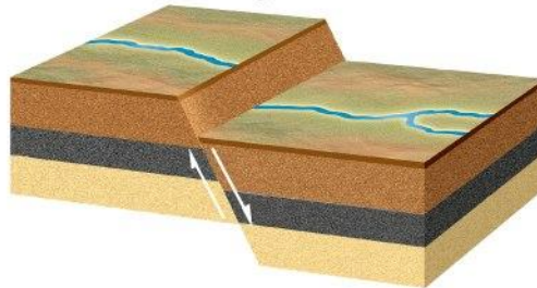
Normal faulting
