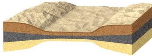
Stretching
