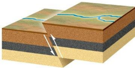
Reverse faulting
