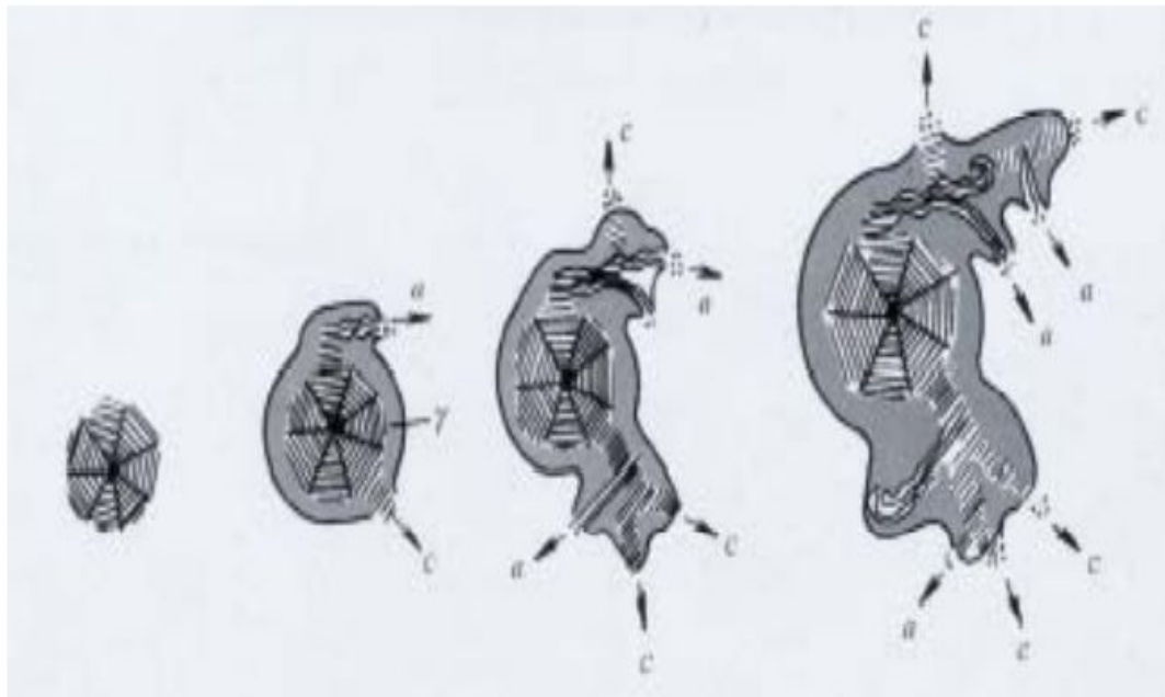
Fig. 4-5: Transformation mechanism from a spheroidal “germ” to vermicular graphite [11]
