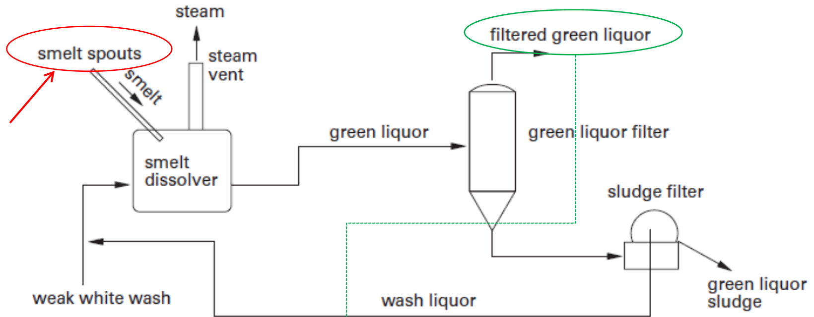
Figure 13.2. Schematic diagram of the green liquor system.
