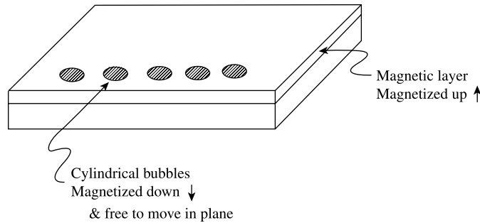
Fig. 15.9 Magnetic bubbles.
