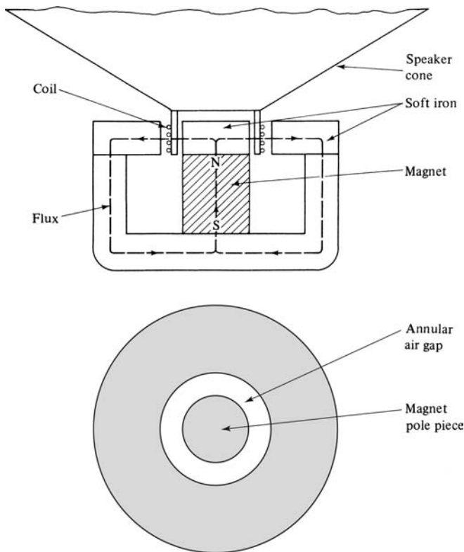
Fig. 14.17 Loudspeaker construction.
