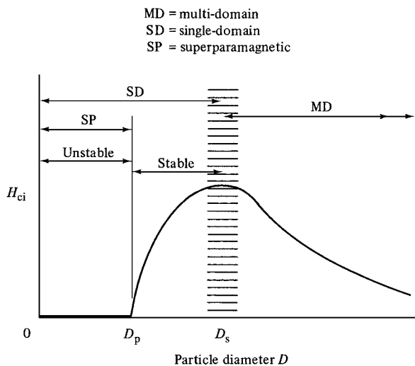
Fig. 11.2 Variation of intrinsic coercivity H_{ci} with particle diameter D (schematic).
