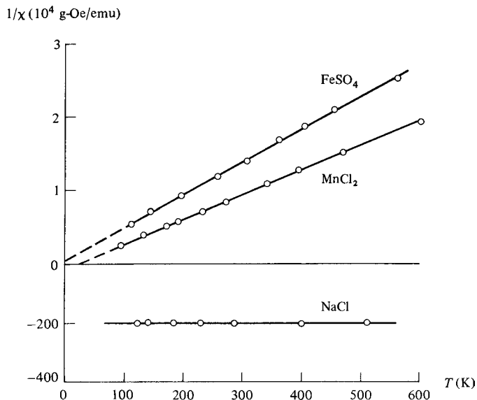
Fig. 3.5 Reciprocal mass susceptibilities of one diamagnetic and two paramagnetic compounds. Note change of vertical scale at the origin.
