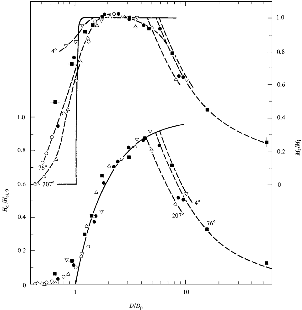
Fig. 11.20 Particle size dependence of the coercivity (lower curve) and retentivity (upper curve) of a Co-Fe alloy. Solid lines are calculated. [E. F. Kneller and F. E. Luborsky, J. Appl. Phys. , 34 (1963) p. 656.]
