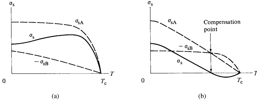
Fig. 6.9 Unusual \sigma_s vs T curves for cubit ferrimagnets.
