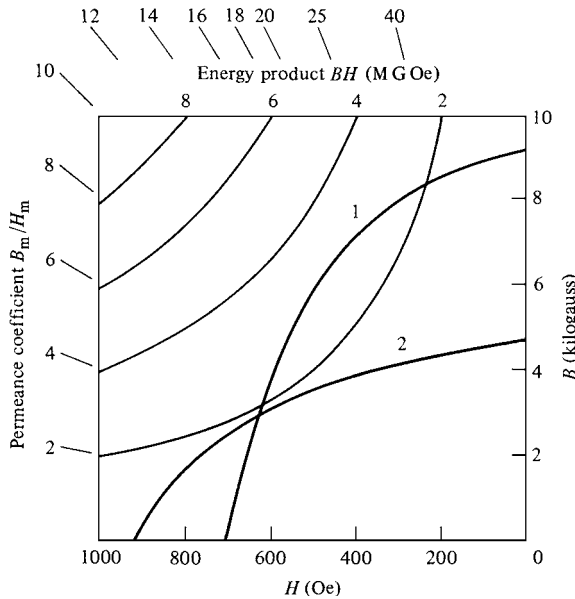
Fig. 14.4 Demagnetization curves (schematic) of two permanent magnet materials denoted 1 and 2. The graph shows also contour lines of constant (BH) , and perimeter marks to allow values of the permeance coefficient to be drawn. Material 1 has (BH)_{max} about 3 MGOe; the value for material 2 is just below 2 MGOe.
