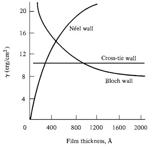
Fig. 11.32 Variation of wall energy with film thickness for various kinds of wall in 80 Permalloy, calculated for exchange constant A = 10^{-6} erg/cm, anisotropy constant K = 1500 ergs/cm 3 , bulk-wall width = 20,000 Å, and bulk-wall energy = 0.1 erg/cm 2 . [M. Prutton, Thin Ferromagnetic Films , Butterworth (1964).]
