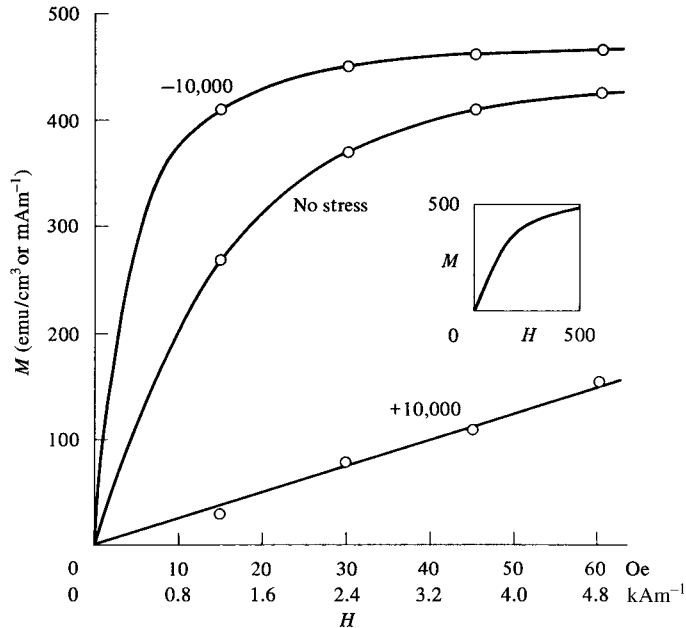
Fig. 8.16 Effect of applied tensile (+) and compressive (−) stress on the magnetization curve of polycrystalline nickel; 10,000 lb/in 2 \approx 69 MPa. [D. K. Bagchi, unpublished.]
