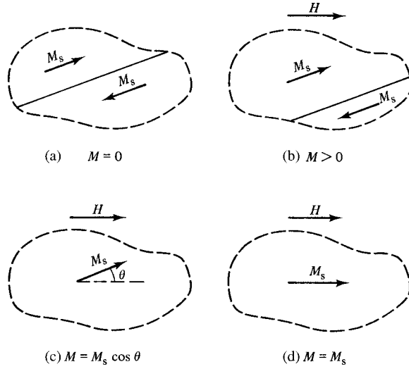
Fig. 4.2 The magnetization process in a ferromagnet.
