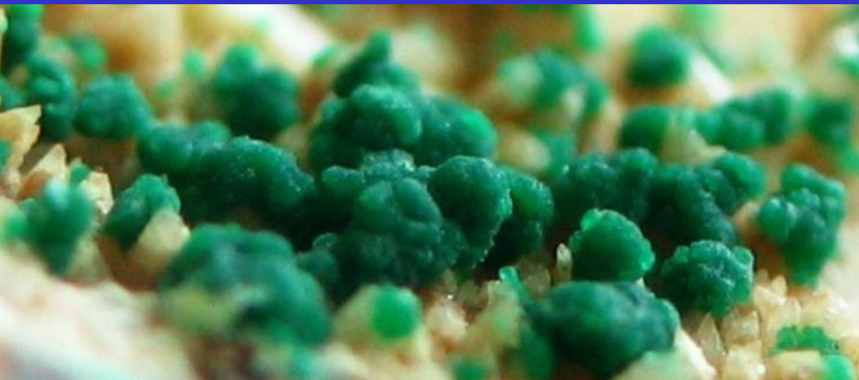
Malaquita \text{Cu}_2(\text{CO}_3)(\text{OH})_2
