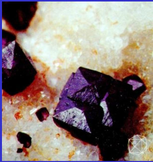
Fluorita
