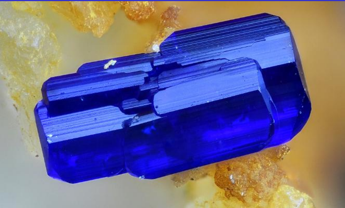
Azurita \text{Cu}_3(\text{CO}_3)_2(\text{OH})_2
