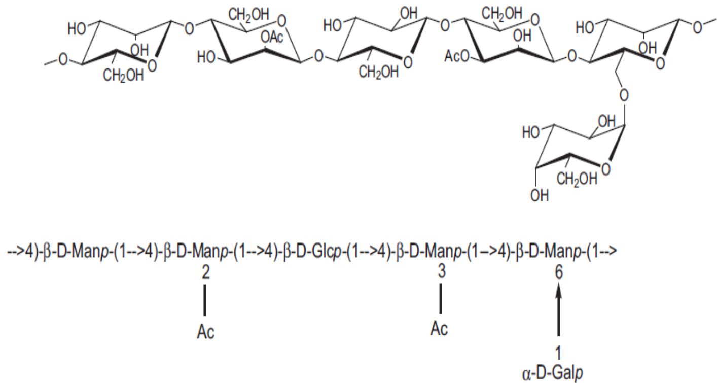
Figure 5.9. Representative structural formula for softwood galactoglucomannan.
