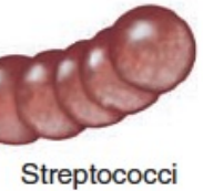
Streptococci
