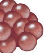
Staphylococci
