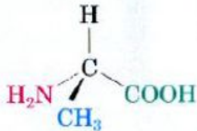
(S)-Alanine [(S)-(+)-2-Aminopropanoic acid] [\alpha]_D = +8.5^\circ
