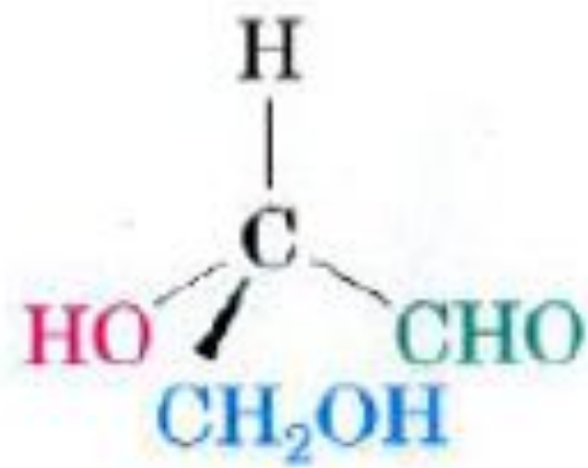
(S)-Glyceraldehyde [(S)-(-)-2,3-Dihydroxypropanal] [\alpha]_D = -8.7^\circ
