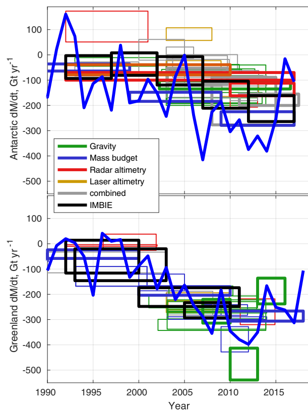
Fig. 3. Mass rates for the Antarctic (top) and Greenland (bottom) ice sheets derived from published studies. The horizontal extent of each rectangle indicates the period that each estimate spans, while the height indicates the error estimate. Studies published between 2011 and 2017 are shown with thin lines, studies published in 2018 and early 2019 with heavier lines. The colour of the lines indicates the type of estimate used, and any estimate that is based explicitly on more than one technique is treated as a ‘combined’ estimate. The IMBIE (Shepherd et al., 2012 for Greenland, Shepherd et al., 2018 for Antarctica) estimates are shown in black. Rectangles are overplotted with annual mass balance estimates from Rignot et al. (2019) for Antarctica and Mouginot et al. (2019) for Greenland, to indicate interannual variability. The studies cited in this plot are described in Supplemental Table I.
