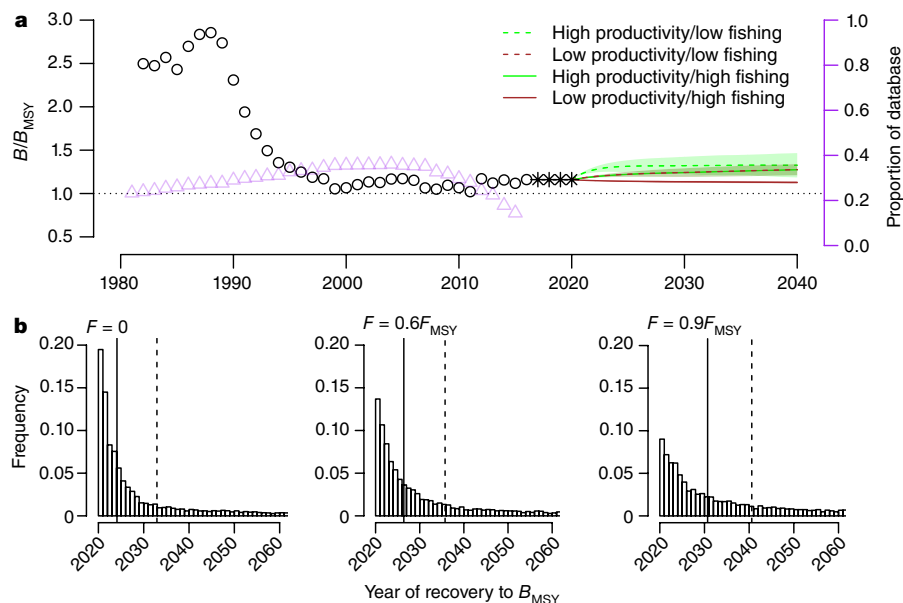
Fig. 4 | Recovery projections for assessed fish stocks. a , Trajectories of exploited fish stock biomass ( B ) relative to the biomass supporting the maximum sustainable yield ( B_{MSY} ; the ratio of which is denoted B/B_{MSY} ) over time based on the scientific assessment of 495 globally distributed fish stocks in the RAM Legacy Stock Assessment Database (version 4.491; https://zenodo.org/record/3676088 ). Open circles indicate the biomass-weighted global average of stock B/B_{MSY} ; asterisks represent years without sufficient data, red and green lines represent four idealized future scenarios ( B_{MSY} values were taken from stock assessments where available and estimated as 50% of the maximum historical biomass otherwise; see Supplementary Information 2). Shading represents the one s.d. range of the simulations. Purple diamonds give the proportion of the database used in the calculation of B/B_{MSY} for each year.
