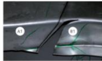
Fracture on real part
