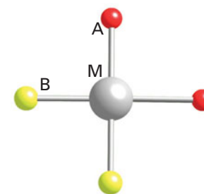
39 cis - [\text{MA}_2\text{B}_2]
