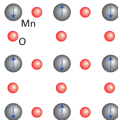
Figure 24.13 The arrangement of electron spins on the \text{Mn}^{2+} ions in the antiferromagnetic state of MnO.
