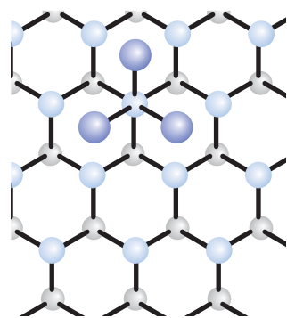
Figure 15.2 The puckered network structure of bismuth. Each Bi atom has three nearest neighbours; the dark shaded atoms indicate next-nearest neighbours from an adjacent pucker sheet. Lightest atoms are furthest from the viewer.
