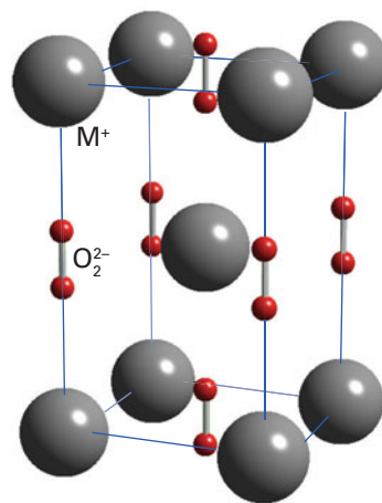
Figure 11.8 The structure of the superoxides \text{MO}_2 of the Group 1 elements.
