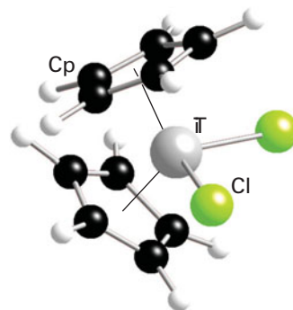
72 [Ti(Cp) 2 (Cl) 2 ]
