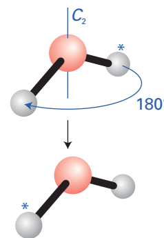
Figure 6.1 An \text{H}_2\text{O} molecule may be rotated through any angle about the bisector of the HOH bond angle, but only a rotation of 180^\circ (the C_2 operation) leaves it apparently unchanged.
