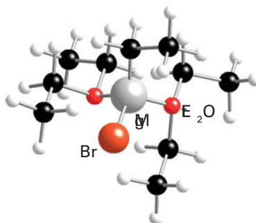
12 \text{MgBr}(\text{OEt})_2
