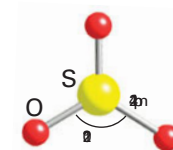
3 \text{SO}_3, D_{3h}
