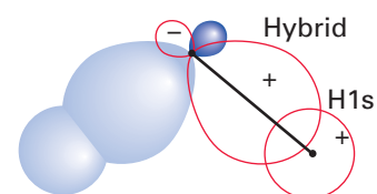
Fig. 2.33 The formation of localized O–H orbitals in \text{H}_2\text{O} by the overlap of hybrid orbitals on the O atom and H1s orbitals. The hybrid orbitals are a close approximation to the \text{sp}^3 hybrids shown in Fig. 2.6.
