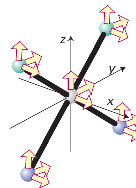
Figure 6.26 The atomic displacements in cis-[PdCl_2(NH_3)_2] with the H atoms ignored.
