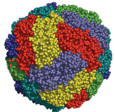
Figure 27.13 The structure of ferritin, showing the arrangement of subunits that make up the protein shell.
