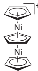
74 [Ni 2 (Cp) 3 ] +
