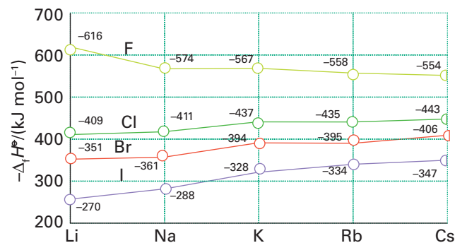
Figure 11.6 The standard enthalpies of formation of the halides of Group 1 elements at 298 K.
