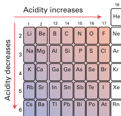
Figure 9.12 The general variation of acidic nature of the oxides of the elements through the periodic table.
