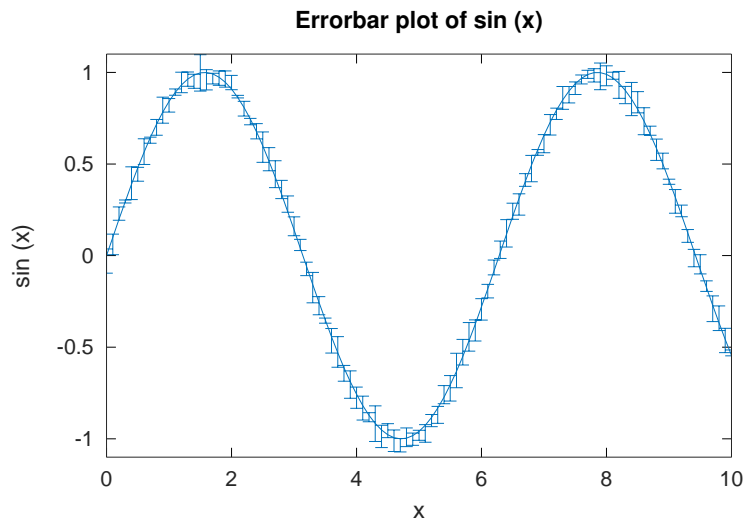
Figure 15.3: Errorbar plot.
