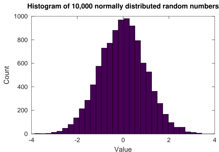
Figure 15.2: Histogram.
