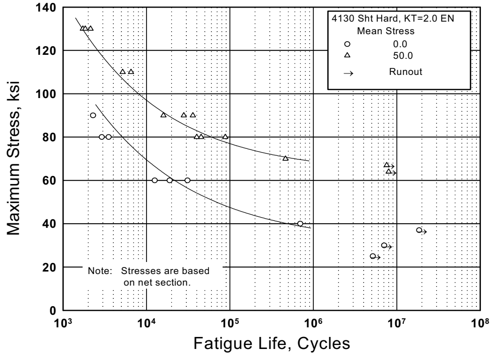
Figure 2.3.1.2.8(g). Best-fit S/N curves for notched, K_t = 2.0 , 4130 alloy steel sheet, F_u = 180 ksi, longitudinal direction.
