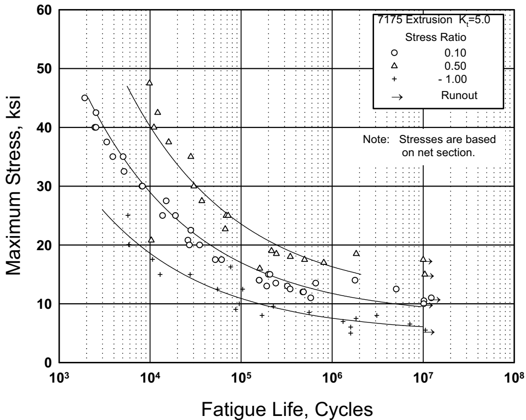
Figure 3.7.8.1.8(c). Best-fit S/N curves for notched, K_t = 5.0 , 7175-T73511 alloy extrusion, longitudinal direction.
