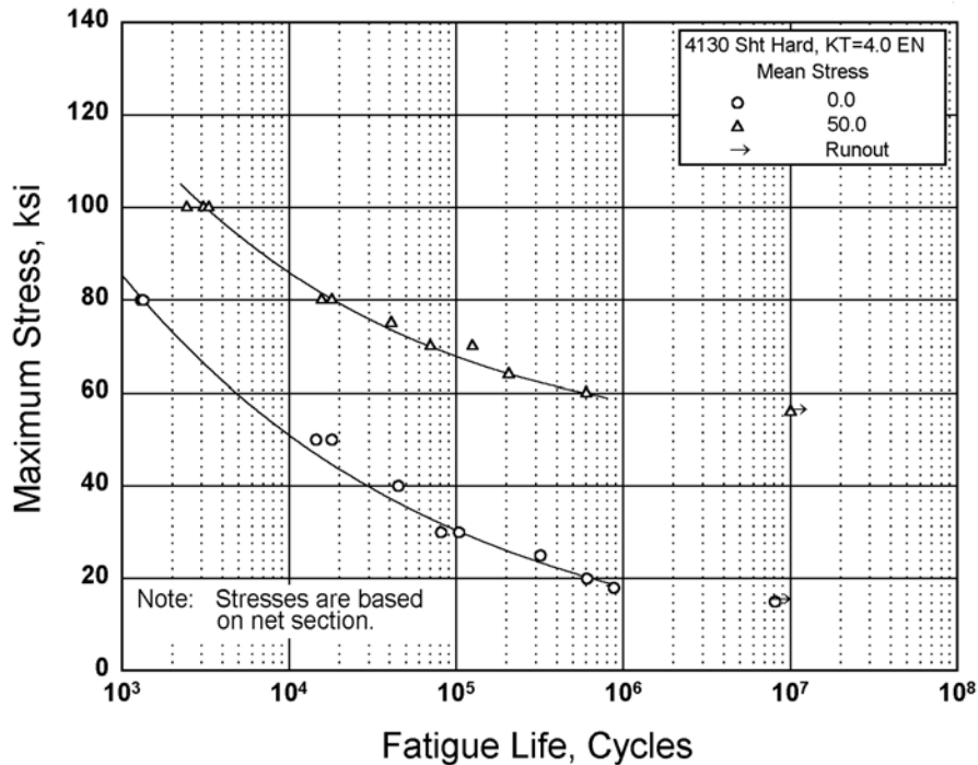
Figure 2.3.1.2.8(h). Best-fit S/N curves for notched, K_t = 4.0 , 4130 alloy steel sheet, F_{iu} = 180 ksi, longitudinal direction.
