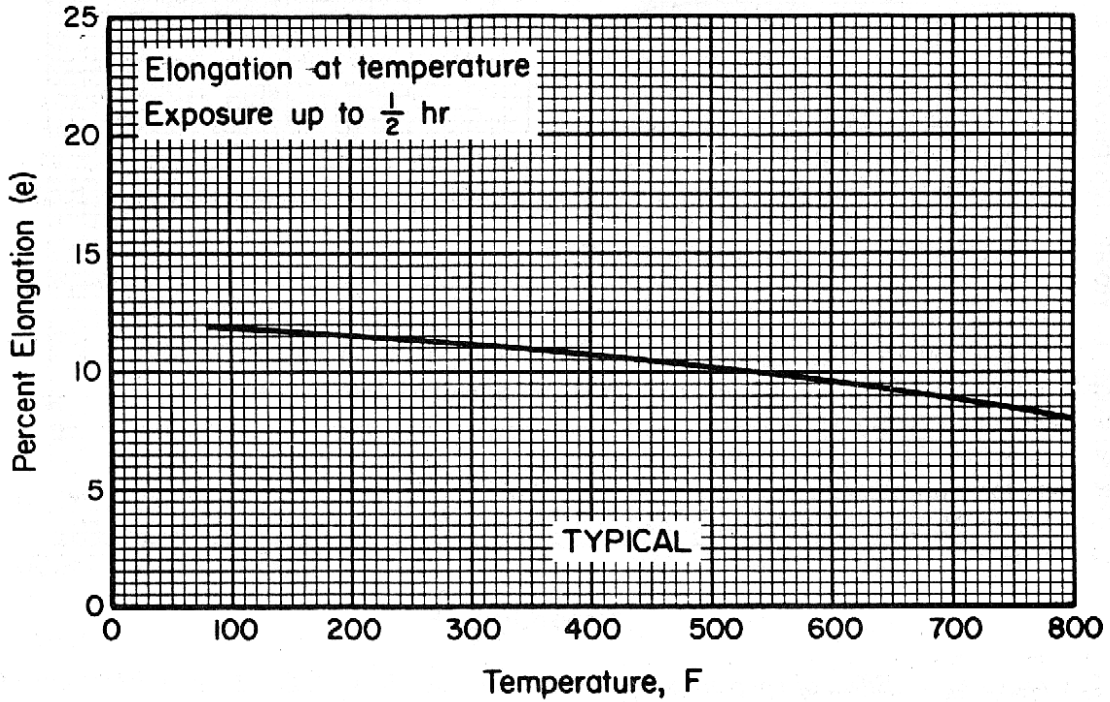
Figure 7.4.1.1.5. Effect of temperature on the elongation (e) of cold worked and aged MP35N bar, F_{iu} = 260 ksi.
