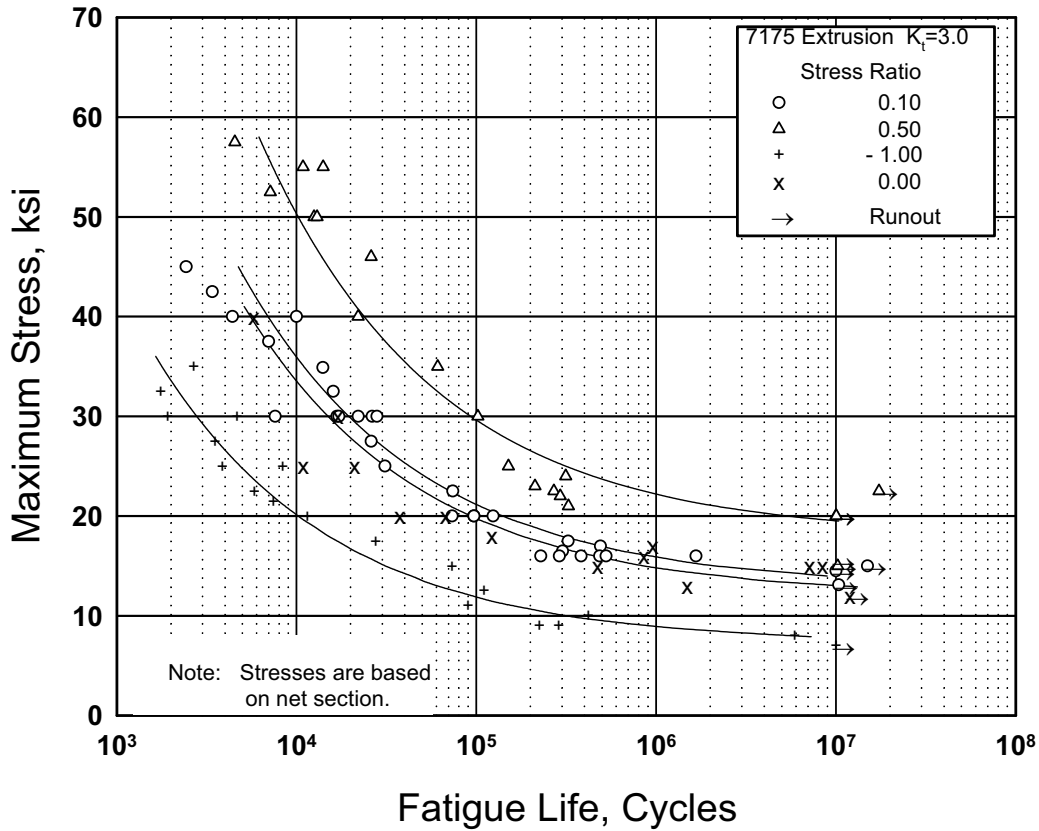
Figure 3.7.8.1.8(b). Best-fit S/N curves for notched, K_t = 3.0 , 7175-T73511 alloy extrusion, longitudinal direction.
