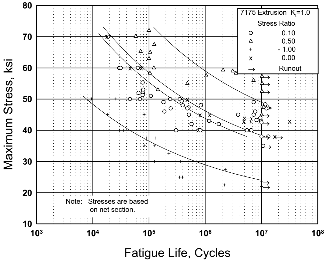
Figure 3.7.8.1.8(a). Best-fit S/N curves for unnotched 7175-T73511 alloy extrusion, longitudinal direction.
