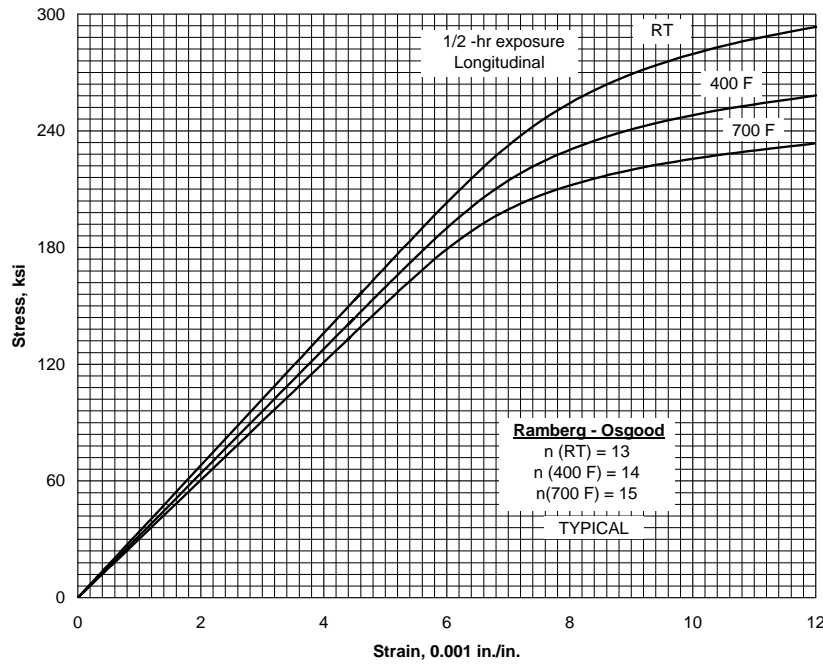
Figure 7.4.1.1.6. Typical tensile stress-strain curves at room and elevated temperatures for cold worked and aged MP35N bar, F_{iu} = 260 ksi.
