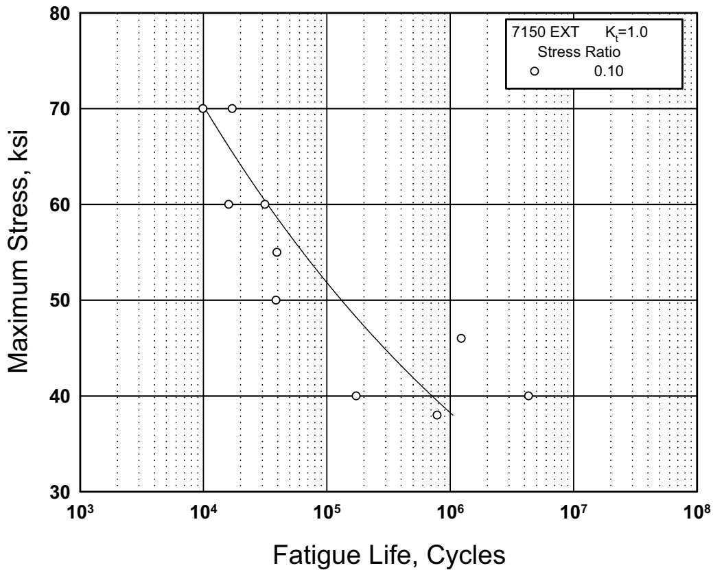
Figure 3.7.7.2.8(b). Best-fit S/N curves for unnotched 7150-T77511 aluminum alloy extrusion, long transverse orientation.
