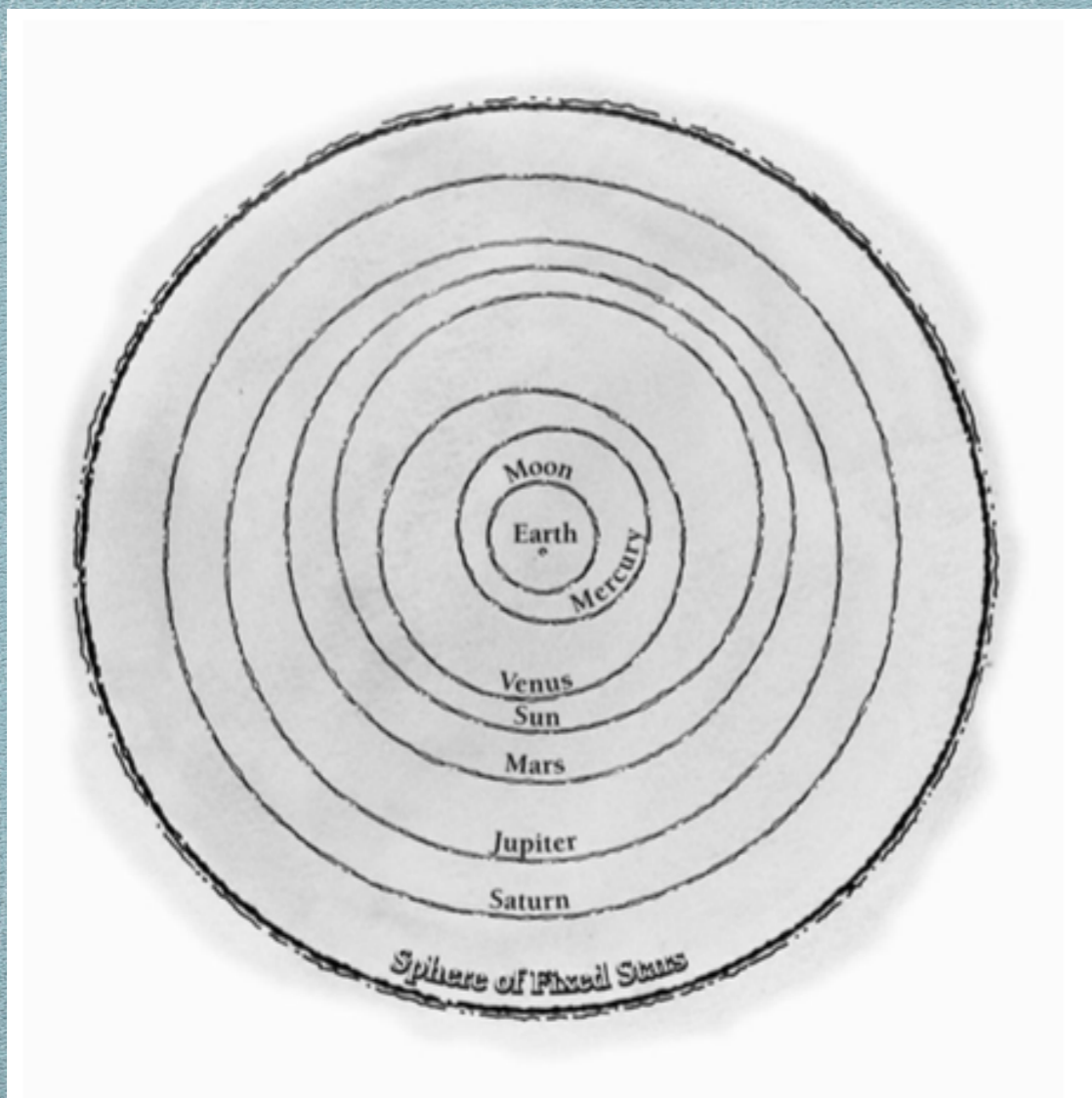
Figure 1.3 An Earth-centered system with the order of the planets as given by Ptolemy. The system ends with the sphere of fixed stars. (Credit: Layne Lundström.)
