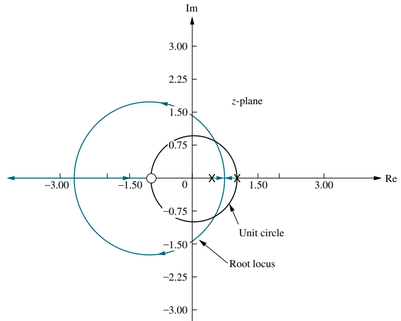
FIGURE 13.22 Root locus for the system of Figure 13.21
