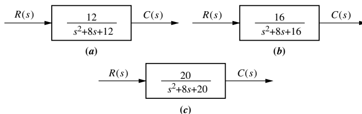
FIGURE 4.12 Systems for Example 4.4
