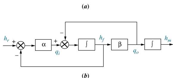
FIGURE P5.38 a. Ktesibios' water clock; b. water clock block diagram (© 1992 IEEE)
