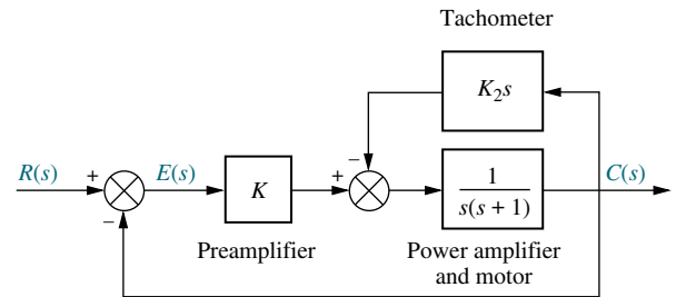
FIGURE P5.51 Position control
