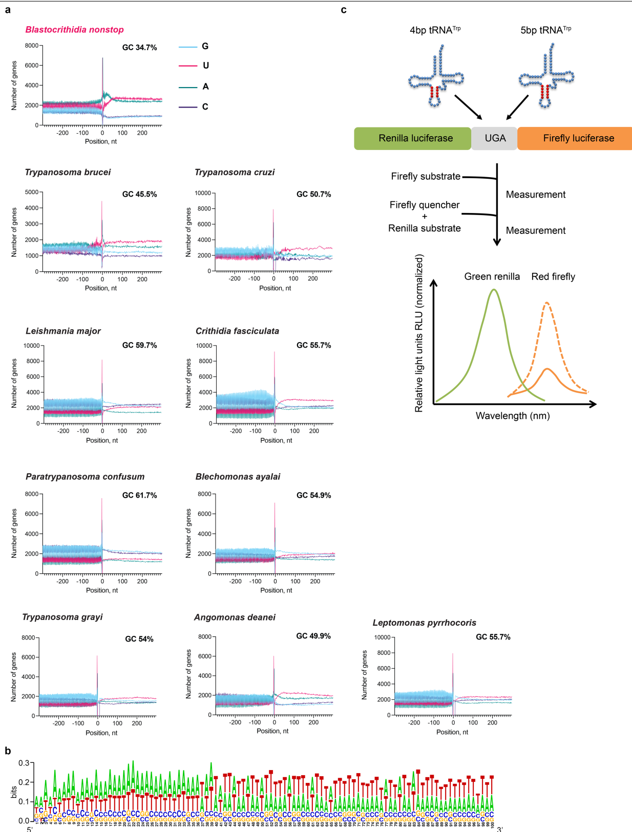
Extended Data Fig. 6 | Stop codon context analysis and schematic of the dual luciferase assay. (a) GC-content around the termination codon position in the 3' ends of protein-coding genes in trypanosomatids. The GC distribution in the B. nonstop genome dramatically differs inside of the coding regions versus the intergenic regions, in contrast to other trypanosomatids. The former are more GC-rich, however, immediately after the 3' end of genes the genome sequences become substantially more A+T-rich. (b) Sequence logo for first 100 nt after the stop codon. A is the most abundant nucleotide in the first
