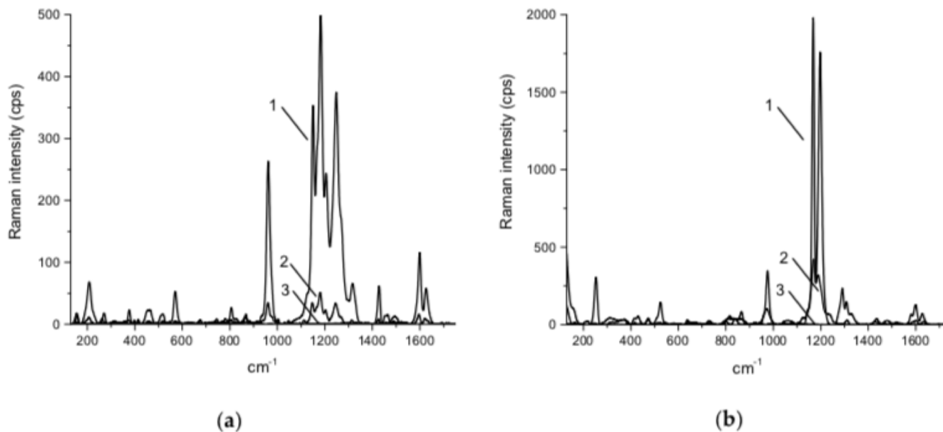
Figure 3. Typical Raman spectra of cream (a) and gel (b) containing curcumin, where 1—Raman spectrum of aggregated curcumin, 2—Raman spectrum of curcumin, dissolved in the base, and 3—Raman spectrum of the base without curcumin.
