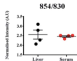
Fig. 4 Calculation of Raman band intensities and intensity ratios pertaining to different biomolecules in liver and serum. Marker bands were chosen for each of the biomolecules; (A) DNA (784 cm -1 ), proteins and lipids (1003, 1451 and 1660 cm -1 ). (B) Ratiometric analysis of two Raman bands – 830 and 854 cm -1 . Each circle in the figure represents an individual mouse. Spectra obtained from a total of 4 mice were used for enumeration. Statistical analysis was performed using Mann–Whitney test where * indicates p < 0.05 .
