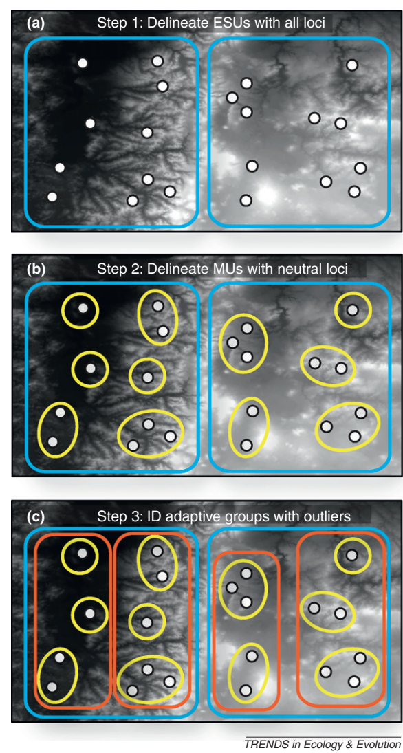
Figure 1. Proposed steps in using genomic data [e.g. single nucleotide polymorphisms (SNPs)] to define conservation units and test for adaptive differentiation among management units (MUs). White circles represent sampling localities, blue outlines are evolutionarily significant units (ESUs), yellow ellipses are MUs, and orange outlines are adaptively similar groups of MUs. The grayscale background is an elevation layer (white is high elevation, black is low elevation).
