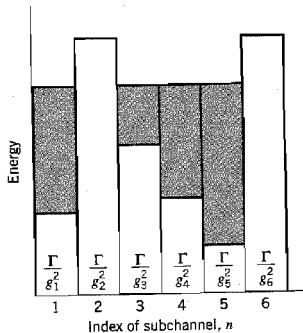
FIGURE 6.56 Water-filling interpretation of the loading problem.
