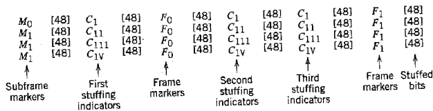
FIGURE 3.21 Signal format of AT&T M12 multiplexer.
