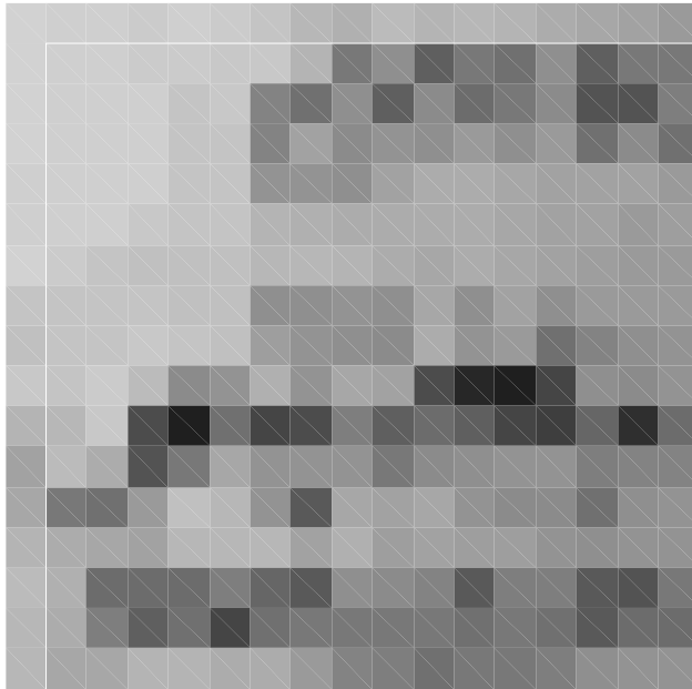
Figure 6.27 16 × 16 macroblock
