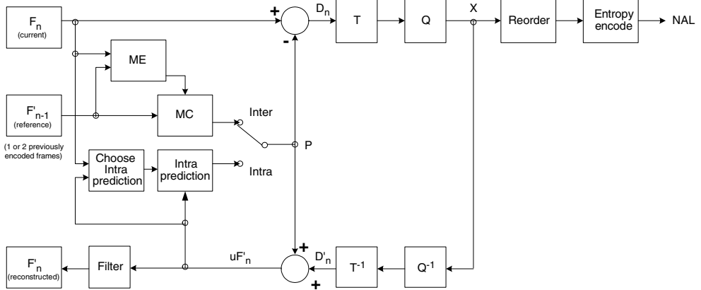
Figure 6.1 H.264 Encoder
