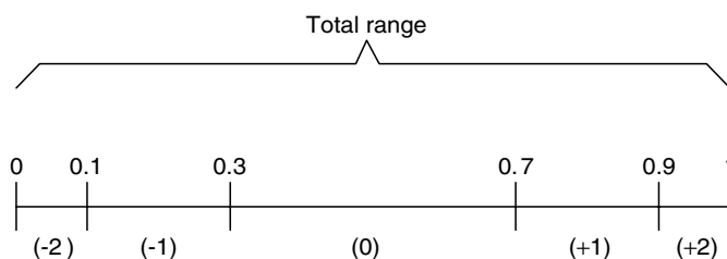
Figure 3.48 Sub-range example
