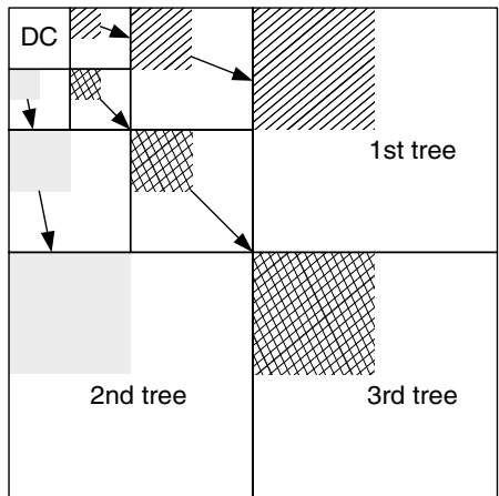
Figure 5.69 Tree-order scanning
