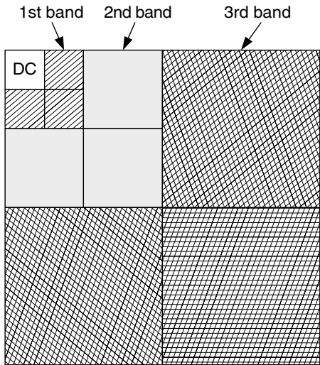
Figure 5.70 Band-by-band scanning
