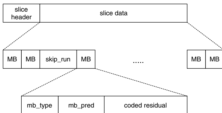
Figure 6.5 Slice syntax
