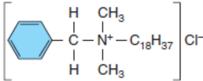
Benzalkonium chloride
