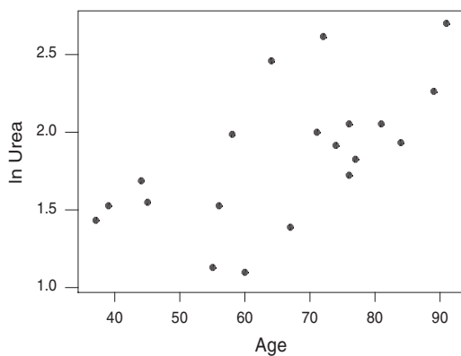
Scatter diagram for In urea and age
