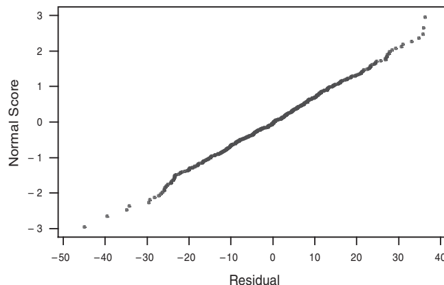
Normal probability plot of residuals for the data in Table 4. Response is Simplified Acute Physiology Score.
