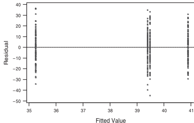
Plot of residuals versus fits for the data in Table 4. Response is Simplified Acute Physiology Score.
