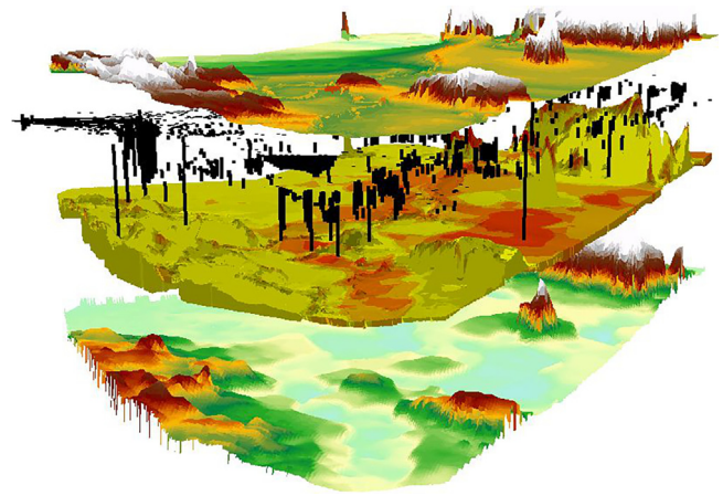
Fig. 8. 3D/4D deposit model: Top level shows current topographic/bathymetric surface, core data is shown on the second level, the isopachyte calculated from cores and sub-bottom data is on the third level, and the reconstructed pre-holocene landscape on the bottom layer (after Sturt et al., 2016, Fig. 7.1).
