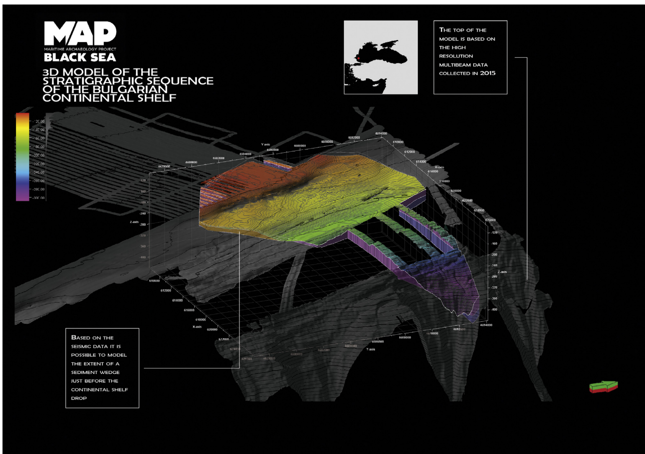
Fig. 16. Computer model of sediment thickness of the surveyed portion of the Bulgarian shelf. Image generated from sub-bottom, swath bathymetry and core data, created by Dr Rodrigo Pacheco-Ruiz.
