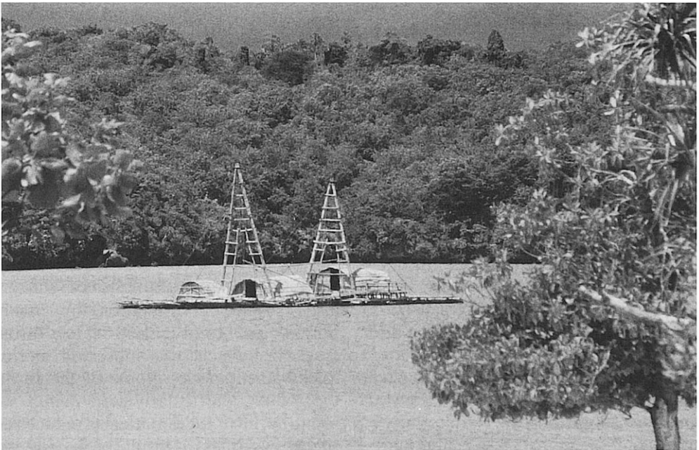
Figure 5. The Nale Tasih 1 in Oeseli Lagoon shortly before sea trials. (Photo: author)
