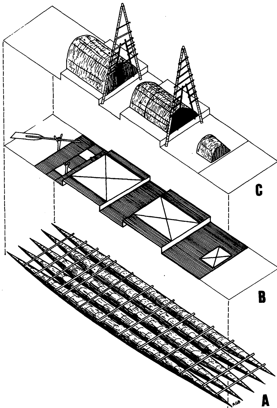
Figure 2. Exploded view of the Nqle Tasih 1 bamboo raft, 23 m long and 5 m wide, showing the arrangement of pontoons (A), decks (B) and superstructures (C). (Drawing: author)
