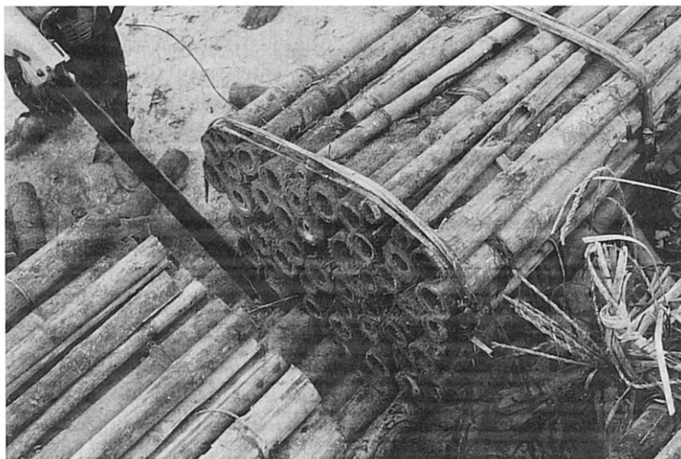
Figure 7. Destructive sampling of bamboo pontoon of Nale Tasih 1 with chainsaw. (Photo: author)
