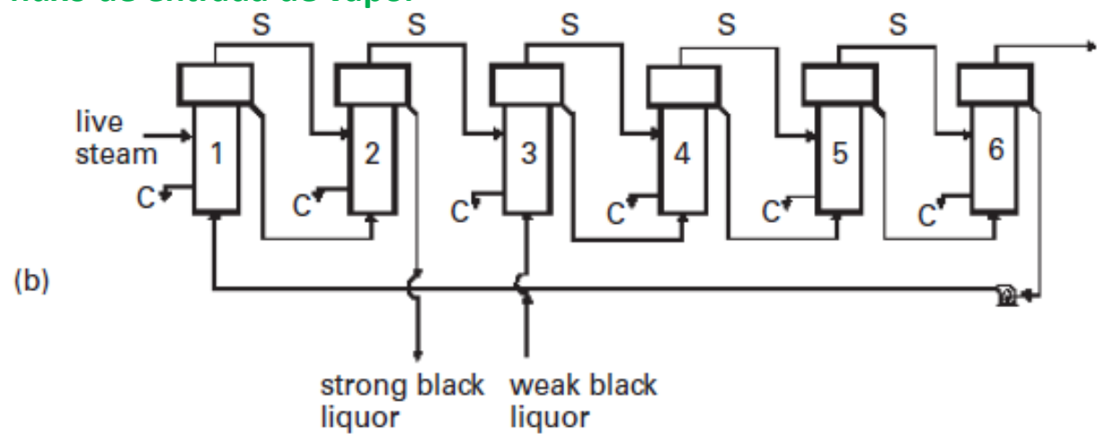
Figure 12.3. Schematic diagram of a counter-current (a), and a mixed co- and counter-current (b), plant respectively. (S is steam and C is condensate).
