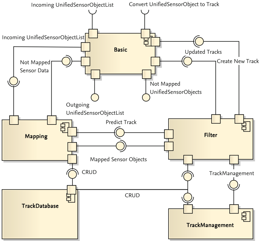
Fig. 5.4 Component diagram of an object fusion module within the sensor fusion layer
