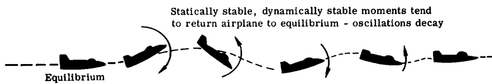
(a) Statically and dynamically stable.
