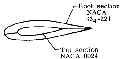
(b) Aerodynamic twist.
