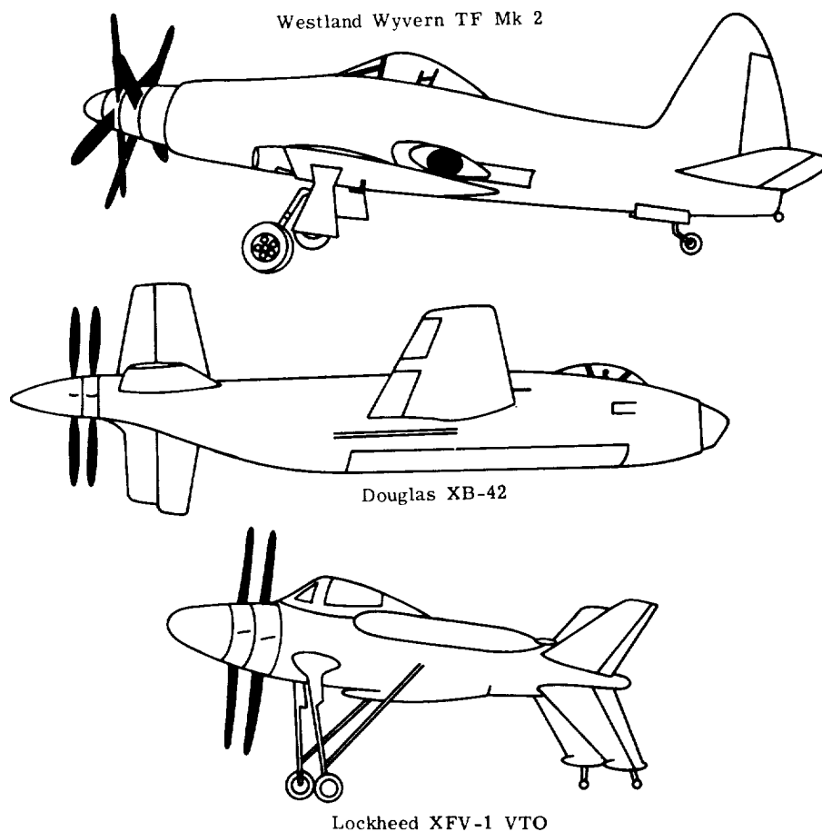
Figure 80.- Contrarotating propellers.
