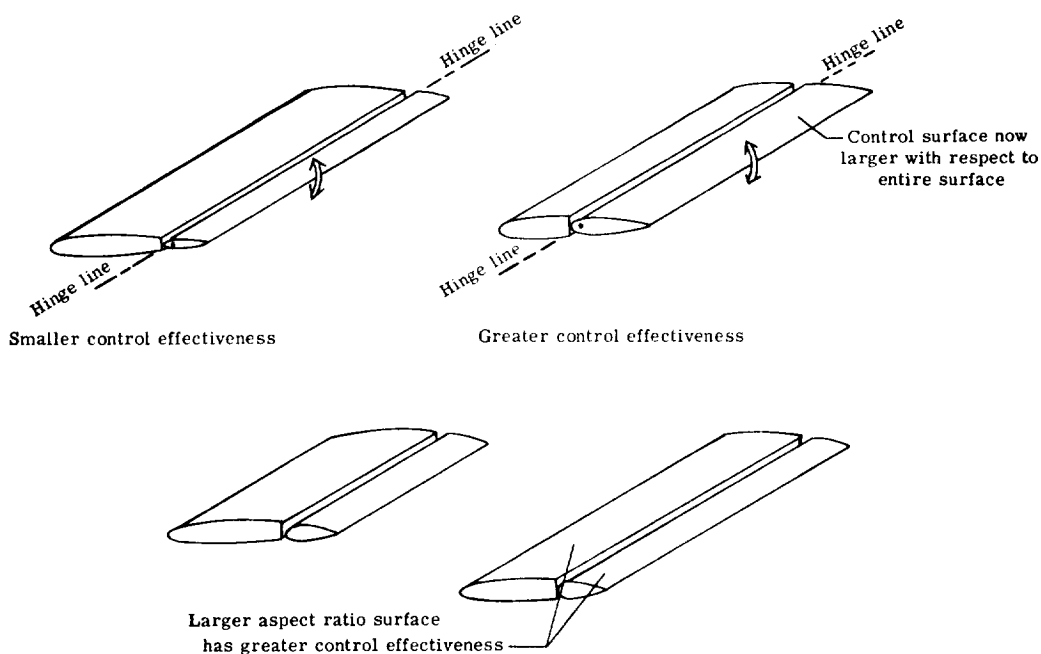
Figure 152.- Control effectiveness.
