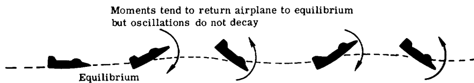
(b) Statically stable; neutral dynamic stability.
