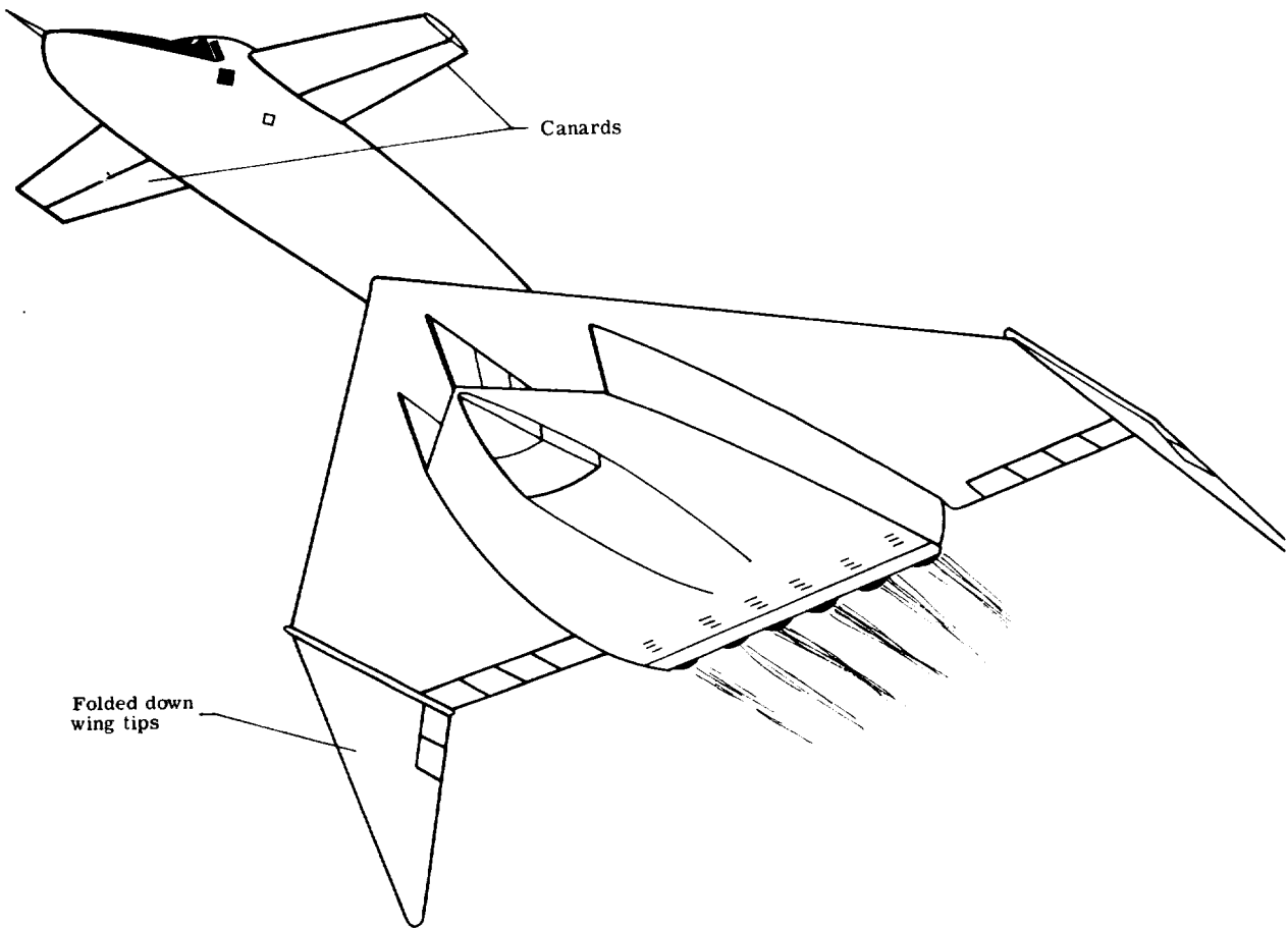
Figure 138.- XB-70 airplane.
