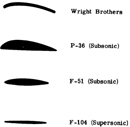
(a) Examples of airfoil shapes.
