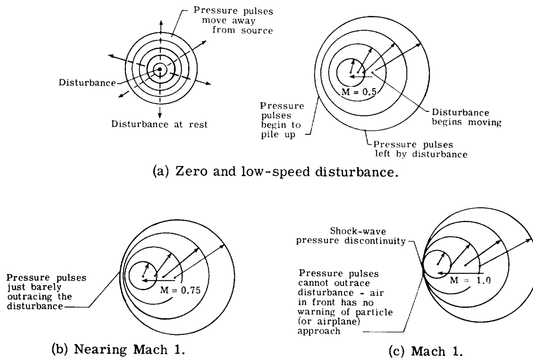
Figure 84.- Shock-wave formation.
