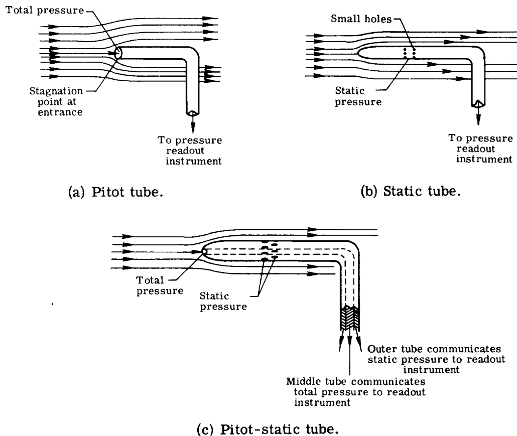
Figure 27.- Pressure measuring devices.
