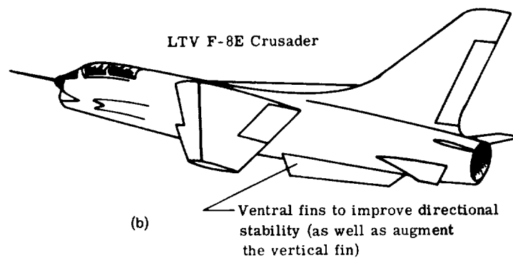
Figure 149.- Dutch roll.
