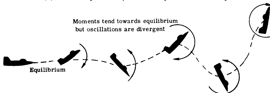
(c) Statically stable; dynamically unstable.
