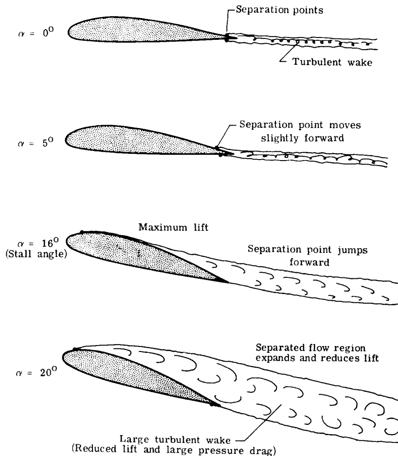
Figure 48.- Stall formation.
