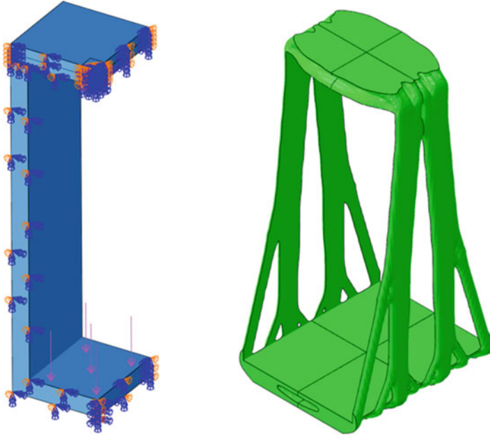
Fig. 17.19 3D cargo sling topology optimization example. Courtesy Mahmoud Alzahrani and Dr. Seung-Kyum Choi, Georgia Institute of Technology
