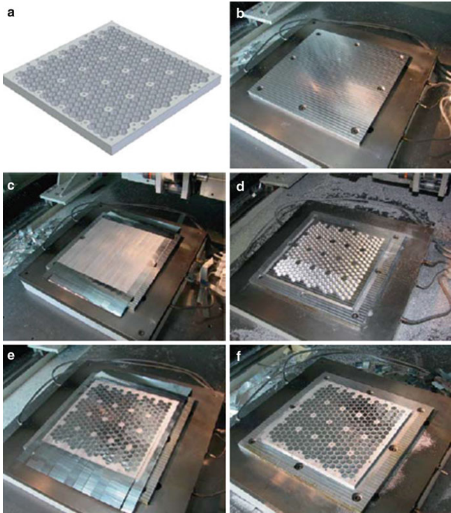
Fig. 9.8 Fabrication procedure for a honeycomb structure using UAM
