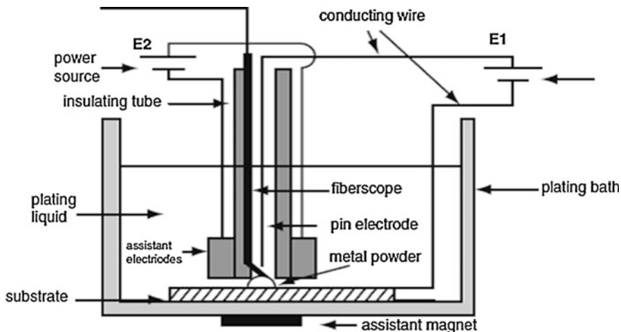
Fig. 11.10 Schematic of an electrochemical liquid deposition system [22] (MATERIALS & DESIGN by Zongyan He, Jack G. Zhou and Ampere A. Tseng. Copyright 2000 by Elsevier Science & Technology Journals. Reproduced with permission of Elsevier Science & Technology Journals in the format Textbook via Copyright Clearance Center.)
