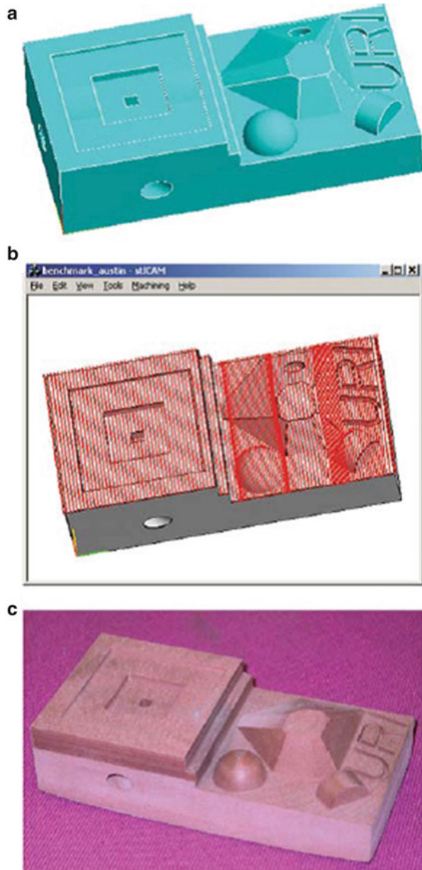
Fig. 14.7 Finish machining using adaptive raster milling of a copper-filled polyamide part made using polymer laser sintering. (a) CAD model, (b) tool paths, (c) machined part (© Emerald Group Publishing Limited, from “Raster Milling Tool-Path Generation from STL Files,” Xiuzhi Qu and Brent Stucker, Rapid Prototyping Journal , 12 (1), pp. 4–11, 2006)
