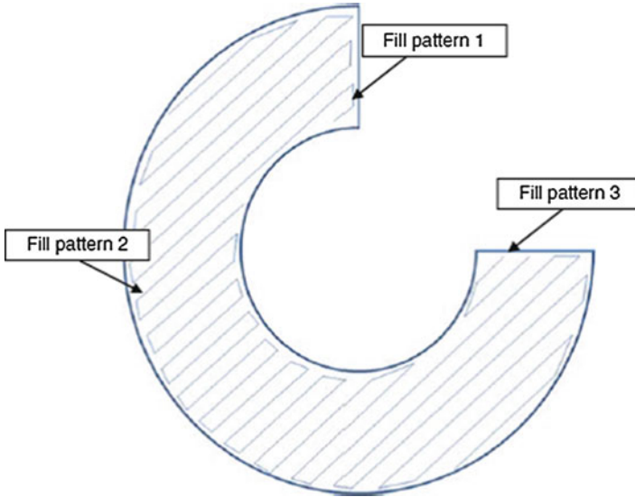
Fig. 6.3 A typical fill pattern using an extrusion-based system, created in three stages (adapted from [4])
