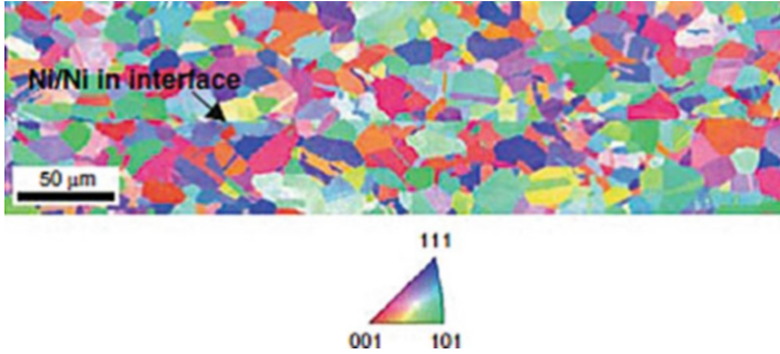
Fig. 9.15 An image of several inverse pole figures of contiguous areas along a well-bonded Ni-Ni interface stitched together. The grains in the image are color coded to reflect their orientation (for color version, see Acta Materialia by Brent L. Adams, Clayton Nylander, Brady Aydelotte, Sadegh Ahmadi, Colin Landon, Brent E. Stucker, G.D. Janaki Ram. Copyright 2008 by Elsevier Science & Technology Journals. Reproduced with permission of Elsevier Science & Technology Journals in the format Textbook via Copyright Clearance Center.)
