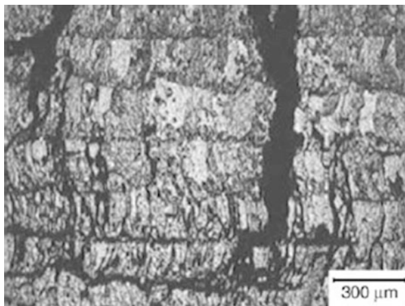
Fig. 10.13 Cracks in a TiC LENS deposit due to residual stresses [4] (SCRIPTA MATERIALIA by Weiping Liu, and J. N. DuPont. Copyright 2003 by Elsevier Science & Technology Journals. Reproduced with permission of Elsevier Science & Technology Journals in the format Textbook via Copyright Clearance Center)
