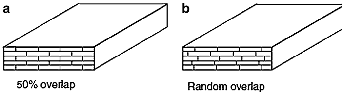
Fig. 9.13 Schematic illustrating (a) 50 % foil overlap and (b) random foil overlap in UAM
