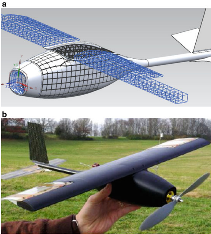
Fig. 17.10 Lattice structure-based UAV design. (a) lattice structure designs for fuselage and wings. (b) assembled UAV ready for test flight
