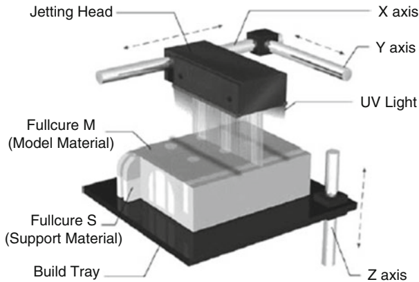
Fig. 2.3 Printer technology used on an AM machine (photo courtesy of Stratasys)
