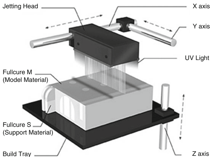
Fig. 7.14 Stratasys Polyjet build process [64]
