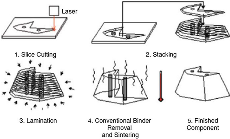
Fig. 9.4 CAM-LEM process (Courtesy CAM-LEM, Inc.)
