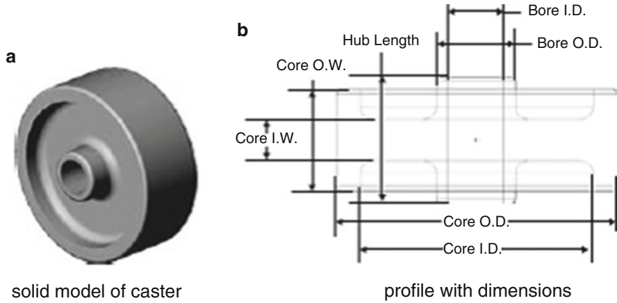
Fig. 13.4 Model of steel caster wheel
