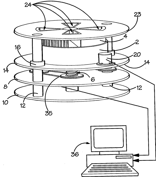
Fig. 8.2 Schematic of a spiral growth manufacturing BJ machine
