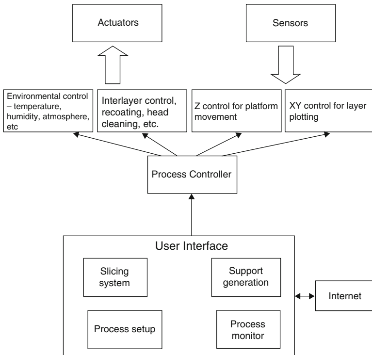
Fig. 2.1 General integration of an AM machine
