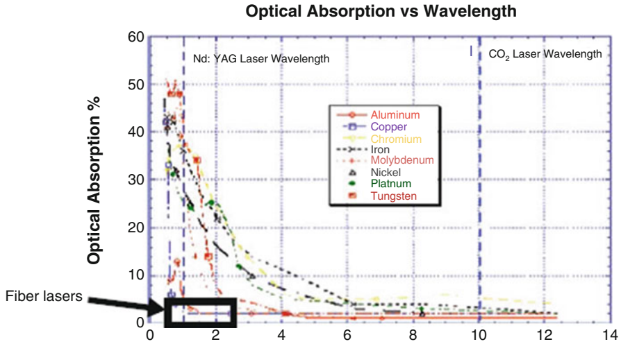
Fig. 5.13 Optical absorption % (absorptivity) of selected metals versus wavelength (units are micrometers) (courtesy: Optomec)
