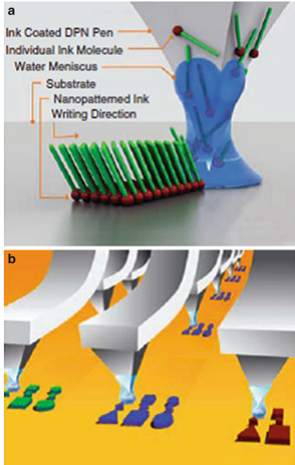
Fig. 11.3 (a) A schematic showing how an AFM tip is used to write a pattern on a substrate. (b) An illustration of a 2D array of print heads (55,000 per \text{cm}^2 ) [7] (courtesy NanoInk)
