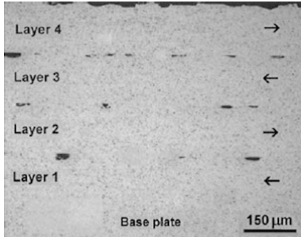
Fig. 9.9 A UAM part made from four layers of Al 3003 foils. LWD is determined by calculating the bonded interface divided by the total interface ( arrows show the sonotrode traveling direction for each layer ). “Effect of Process Parameters on Bond Formation during Ultrasonic Consolidation of Aluminum Alloy 3003,” G.D. Janaki Ram, Yanzhe Yang and Brent Stucker, Journal of Manufacturing Systems , 25 (3), pp. 221–238, 2006
