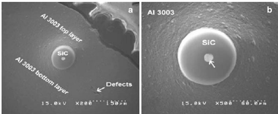
Fig. 9.16 SEM microstructures of Al 3003/SiC: (a) SiC fiber embedded between Al 3003 layers showing a lack of defects near the fiber and (b) the same SiC fiber at a higher magnification showing excellent bonding near the fiber. © Emerald Group Publishing Limited, “Use of Ultrasonic Consolidation for Fabrication of Multi-Material Structures,” G.D. Janaki Ram, Chris Robinson, Yanzhe Yang and Brent Stucker, Rapid Prototyping Journal , 13 (4), pp. 226–235, 2007
