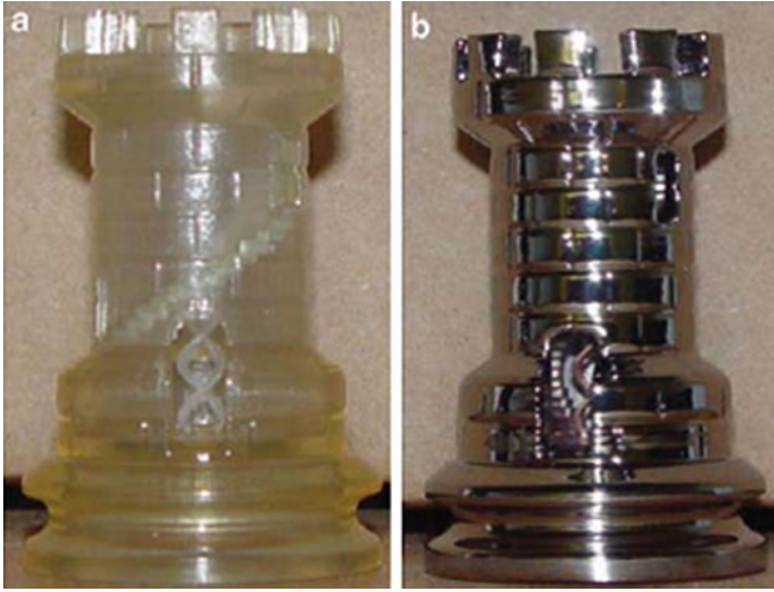
Fig. 14.10 Stereolithography part (a) before and (b) after chrome plating (Courtesy of Aircraft Plating)
