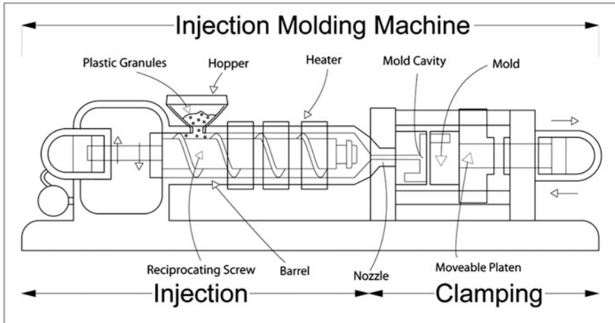
Fig. 18.1 A simple IM machine setup as drawn by Rockey [3]
