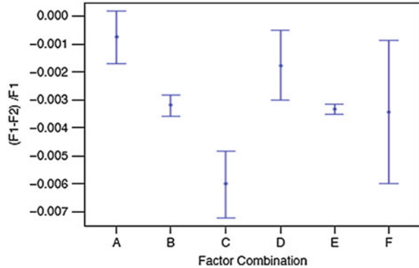
Fig. 14.16 Ninety-five percent confidence intervals for variation in shrinkage for stainless steel (RapidSteel 2.0) infiltration by bronze (Factor combinations are: (a) 10 Torr, 80 %; (b) 10 Torr, 95 %; (c) 10 Torr, 110 %; (d) 800 Torr, 80 %; (e) 800 Torr, 95 %; (f) 800 Torr, 110 %)
