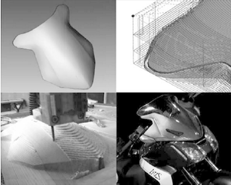
Fig. 15.12 DeskProto software being used to derive machine tool paths from STL file data to form a mold for creating the windscreen of a motorcycle
