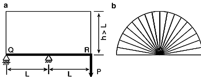
Fig. 17.16 Michell truss layout (b) for simple loaded plate example (a)
