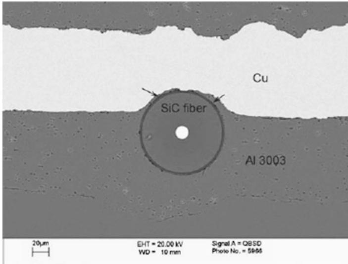
Fig. 9.17 SiC Fiber embedded between copper and aluminum using UAM. Black arrows denote regions where the softer Al extruded around the fiber during embedment, resulting in displacement of the fiber away from the interface into the Al base material
