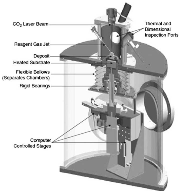
Fig. 11.9 The LCVD system developed at Georgia Tech
