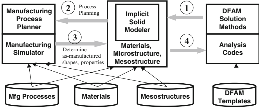
Fig. 17.13 DFAM system and overall structure
