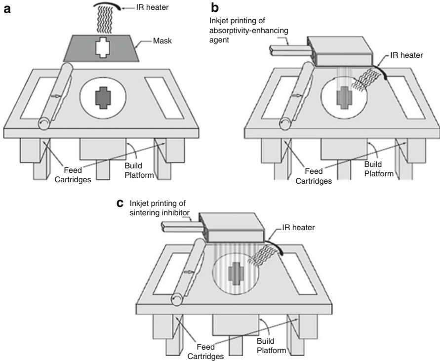
Fig. 5.18 Three different approaches to line- and layer-wise powder bed fusion processing (a) mask-based sintering, (b) printing of an absorptivity-enhancing agent in the part region, and (c) printing of a sintering inhibitor outside the part region
