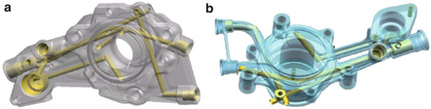
Fig. 17.8 Diesel front plate example. (a) Original design. (b) Redesigned for additive manufacturing
