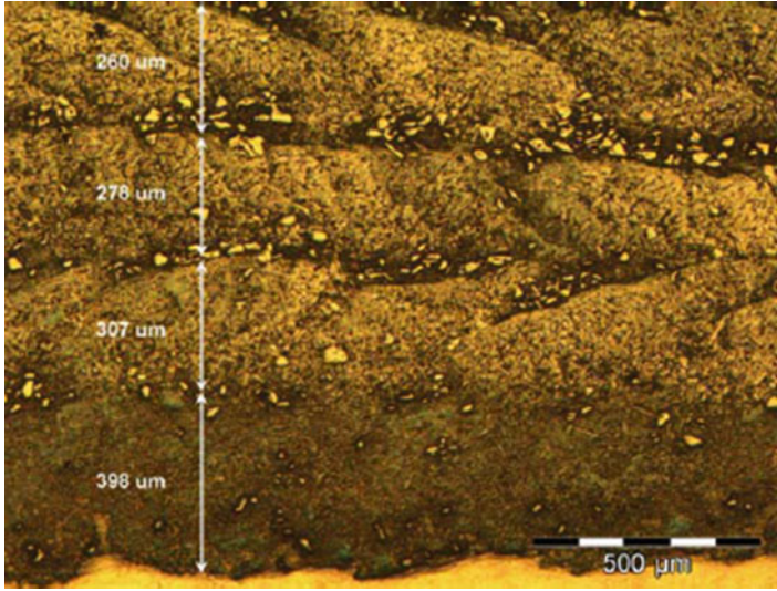
Fig. 10.2 LENS-deposited Ti/TiC metal matrix composite structure (four layers on top of a Ti substrate)
