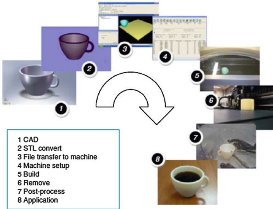
Fig. 3.1 The eight stages of the AM process
