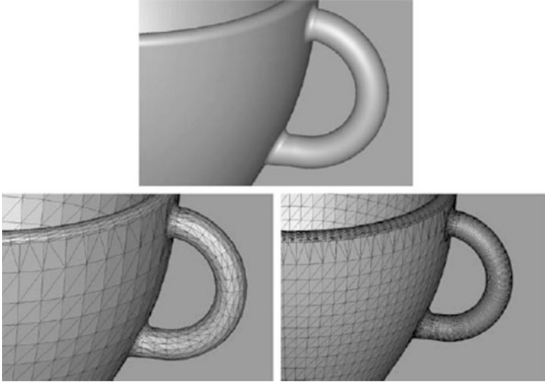
Fig. 15.2 An original CAD model converted into an STL file using different offset height (cusp) values, showing how the model accuracy will change according to the triangle offset
