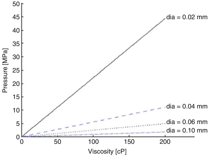
Fig. 7.13 Pressure required to overcome wall friction for printing through nozzles of different diameters
