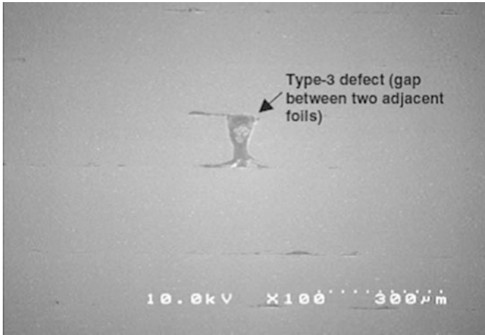
Fig. 9.12 Type-3 defect observed between adjacent foils (Note the morphology of the Type-1 defects between layers indicate that this micrograph is upside-down with respect to build orientation)
