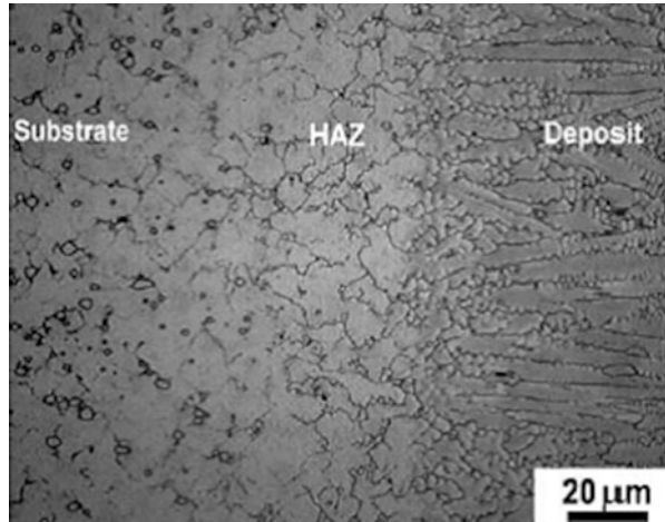
Fig. 10.12 CoCrMo LENS deposit on a wrought CoCrMo substrate of the same composition (deposit occurred from the right of the picture)
