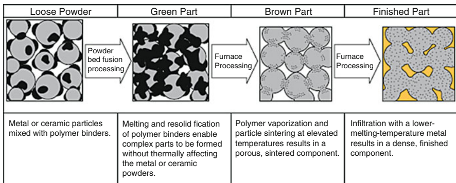
Fig. 5.6 Indirect processing of metal and ceramic powders using PBF
