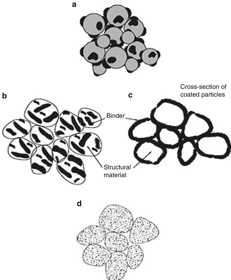
Fig. 5.4 Liquid phase sintering variations used in powder bed fusion processing: (a) separate particles, (b) composite particles, (c) coated particles, and (d) indistinct mixtures. Darker regions represent the lower-melting-temperature binder material. Lighter regions represent the high-melting-temperature structural material. For indistinct mixtures, microstructural alloying eliminates distinct binder and structural regions
