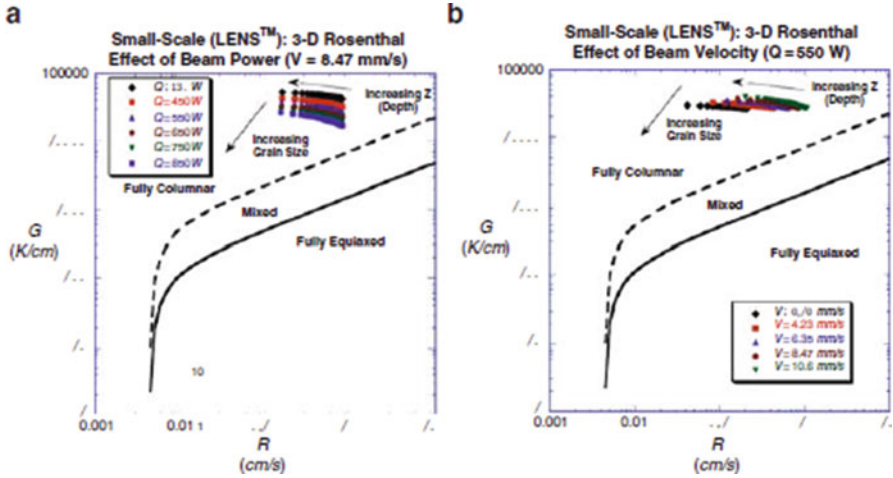
Fig. 10.15 Process maps showing microstructures predicted by the 3D Rosenthal solution for a lower-powered (LENS-like) directed energy deposition system for Ti–6Al–4V (MATERIALS SCIENCE & ENGINEERING. A. STRUCTURAL MATERIALS: PROPERTIES, MICROSTRUCTURE AND PROCESSING by Srikanth Bontha, Nathan W. Klingbeil, Pamela A. Kobryn and Hamish L. Fraser. Copyright 2009 by Elsevier Science & Technology Journals. Reproduced with permission of Elsevier Science & Technology Journals in the format Textbook via Copyright Clearance Center)
