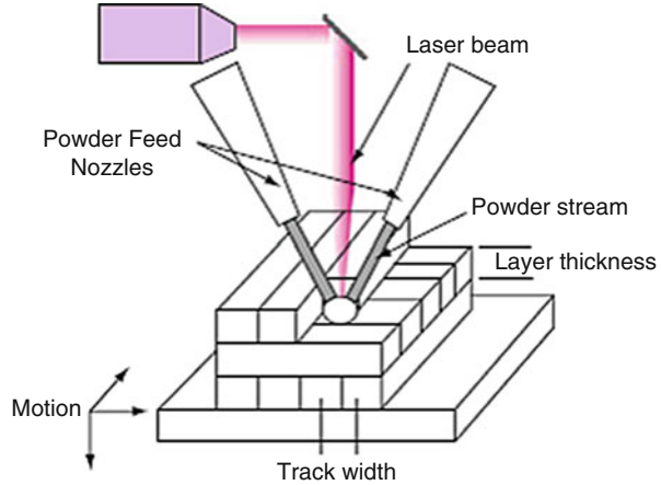
Fig. 10.1 Schematic of a typical laser powder DED process
