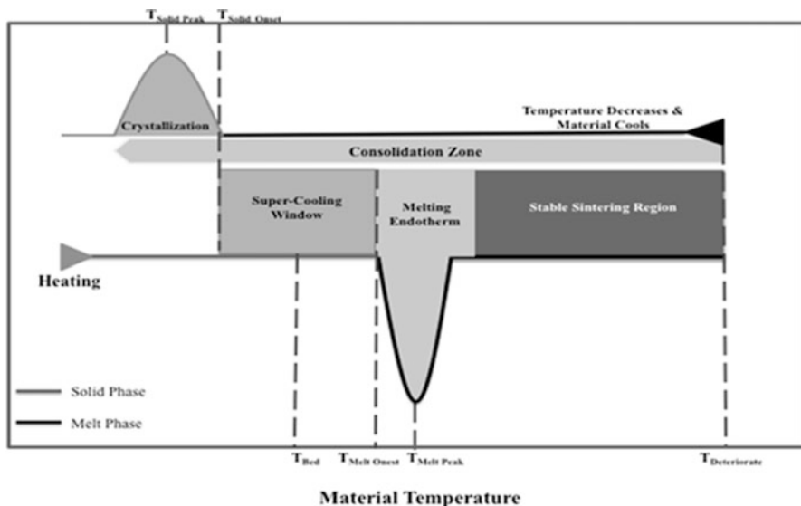
Fig. 5.11 Melting and solidification characteristics for an idealized polymer DSC curve for polymer laser sintering (courtesy: Neil Hopkinson, Sheffield University)
