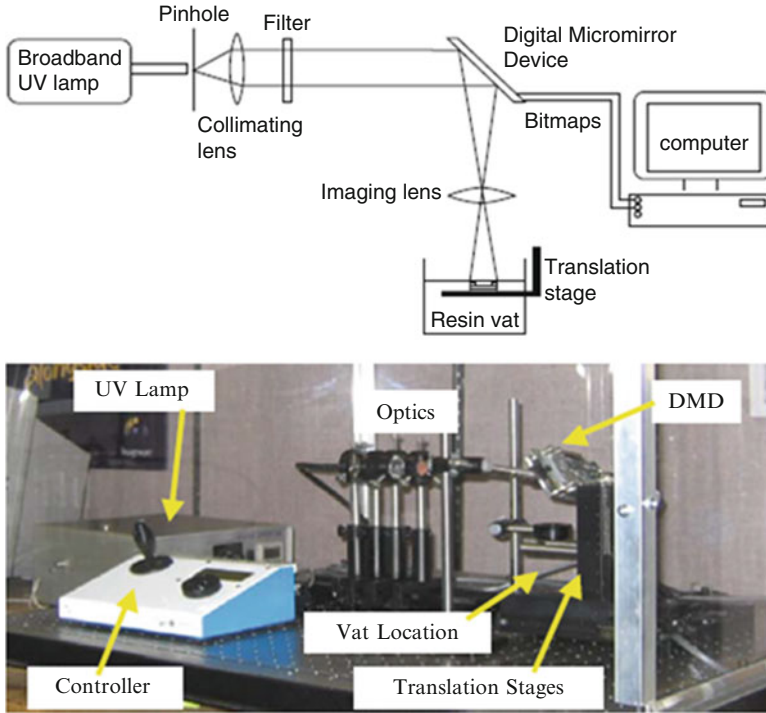
Fig. 4.15 Schematic and photo of mask projection VP machine
