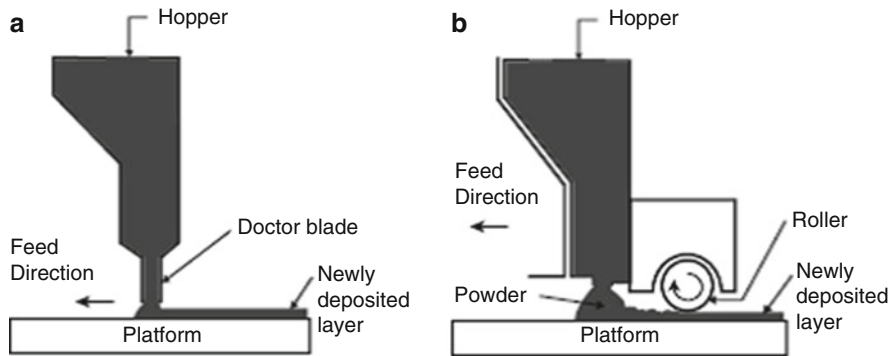
Fig. 5.10 Examples of hopper-based powder delivery systems [6]
