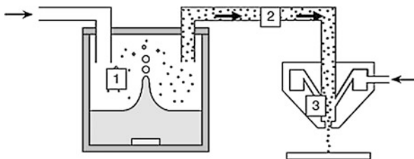
Fig. 11.4 Aerosol Jet System. (1) Liquid material is placed into an atomizer, creating a dense aerosol of tiny droplets 1–5 \mu\text{m} in size. (2) The aerosol is carried by a gas flow to the deposition head (with optional in-flight laser processing). (3) Within the deposition head, the aerosol is focused by a second gas flow and the resulting high-velocity stream is jetted onto the substrate creating features as small as 10 \mu\text{m} in size (Courtesy of Optomec)
