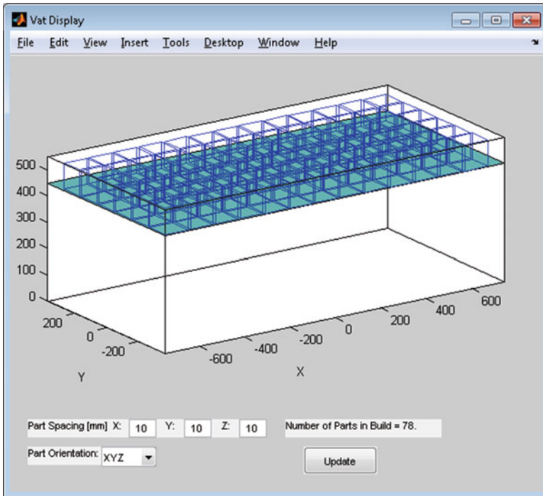
Fig. 13.10 Layout of parts on the machine platform
