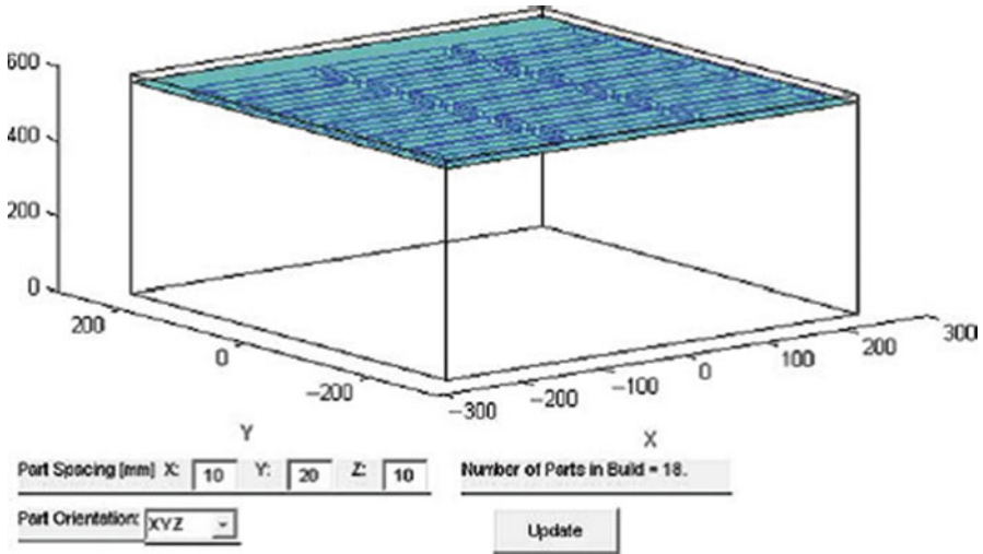
Fig. 16.5 SLA-7000 vat with 18 parts laid out on the platform
