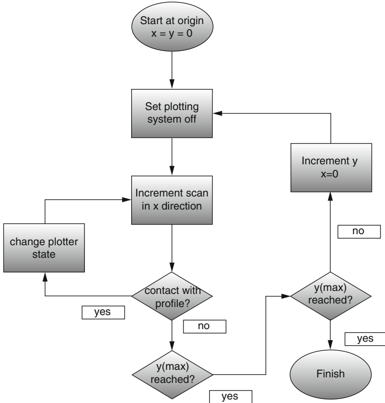
Flowchart 15.3 Algorithm for filling in a 2D profile based on vectors generated using Flowchart 15.2 and a raster scanning approach. Assume the profile fits inside the build volume, the raster scans in the X direction, and lines increment in the Y direction
