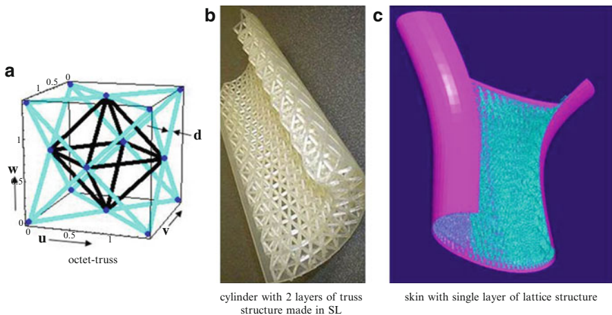
Fig. 17.9 Octet-truss unit cell and example parts with octet-truss mesostructures
