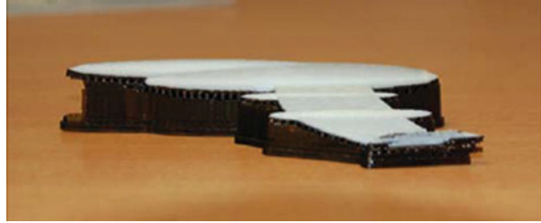
Fig. 14.3 Flat FDM-produced aerospace part. White build material is ABS plastic and black material is the water-soluble WaterWorks™ support material (Courtesy of Shapeways. Design by Nathan Yo Han Wheatley.)
