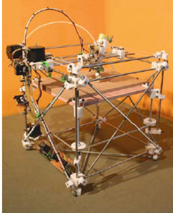
Fig. 6.10 The RepRap “Darwin” machine that is capable of making some of its own parts
