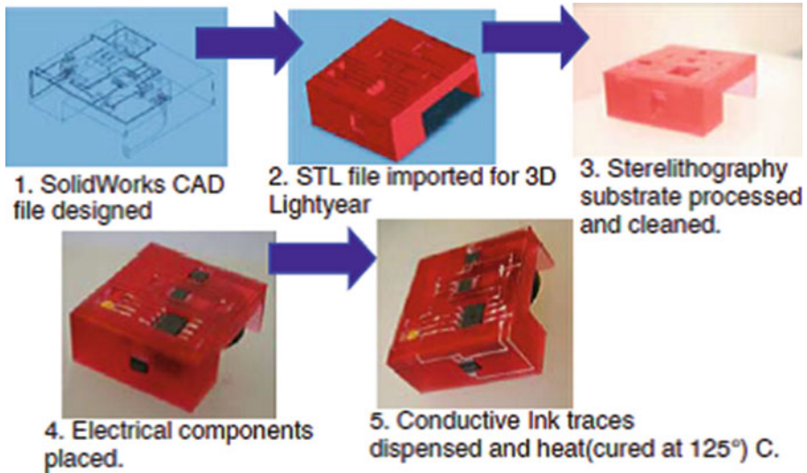
Fig. 17.7 Fabrication of a magnetic flux sensor using VP and DW (courtesy of W.M. Keck Center for 3D Innovation at The University of Texas at El Paso)
