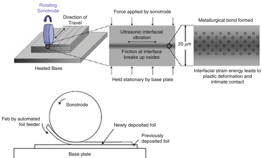
Fig. 9.7 Schematic of ultrasonic consolidation
