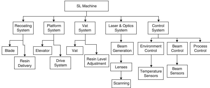
Fig. 4.8 Subsystems for SL technology
