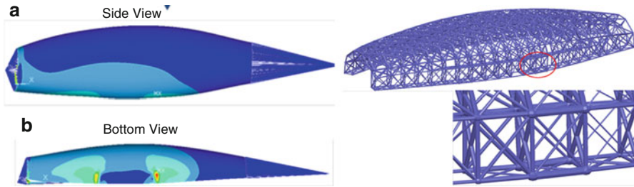
Fig. 17.17 SMS method results on UAV fuselage design problem
