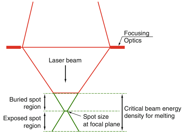
Fig. 10.4 Schematic illustrating laser optics and energy density terminology for directed energy deposition
