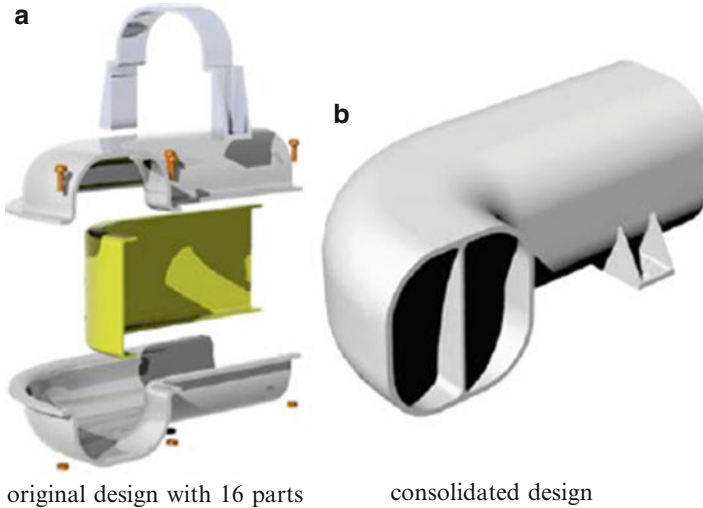
Fig. 17.2 Aircraft duct example
