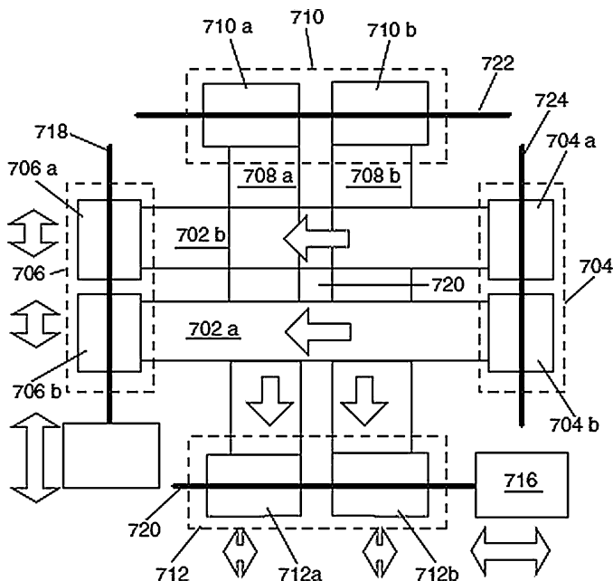
Fig. 11.8 Schematic aperture apparatus for direct write thermal spray (US patent 6576861). Foils 702a, b and 708a, b are in constant motion and are adjusted to allow different amounts of spray to reach the substrate through hole 720 in the center
