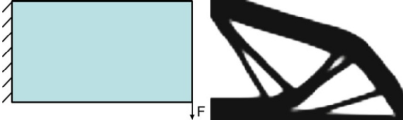
Fig. 17.18 Simple topology optimization example
