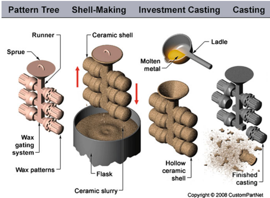
Fig. 18.6 Schematic of the investment casting process. Courtesy of CustomPart at custompartnet.com
