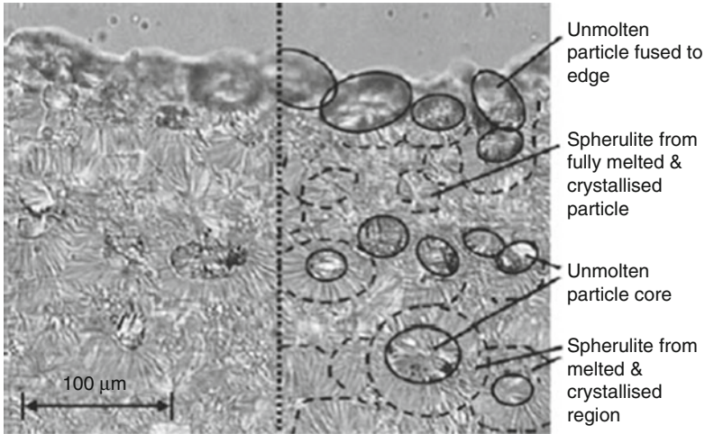
Fig. 5.3 Typical pLS microstructure for nylon polyamide (Materials Science & Engineering, A. Structural Materials: Properties, Microstructure and Processing by Zarringhalam, H., Hopkinson, N., Kamperman, N.F., de Vlieger, J.J. Copyright 2006 by Elsevier Science & Technology Journals. Reproduced with permission of Elsevier Science & Technology Journals in the format Textbook via Copyright Clearance Center) [5]
