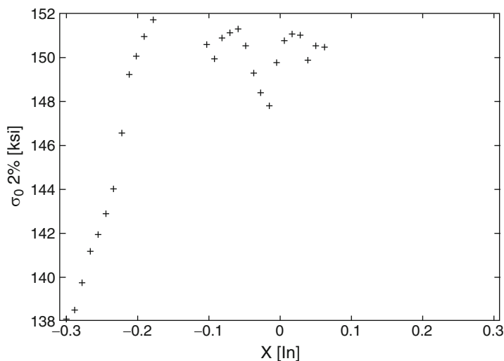
Fig. 10.11 Yield strength at various locations along the tensile bar from Fig. 10.10 representing the mechanical properties for different combinations of Ti-6-4 and Ti-22-23 (courtesy Optomec)
