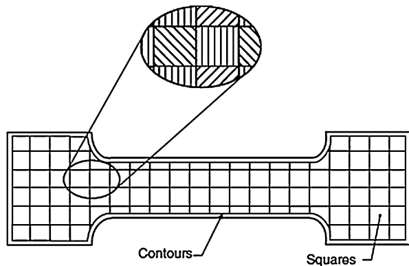
Fig. 5.7 Scan strategies employed in PBF techniques
