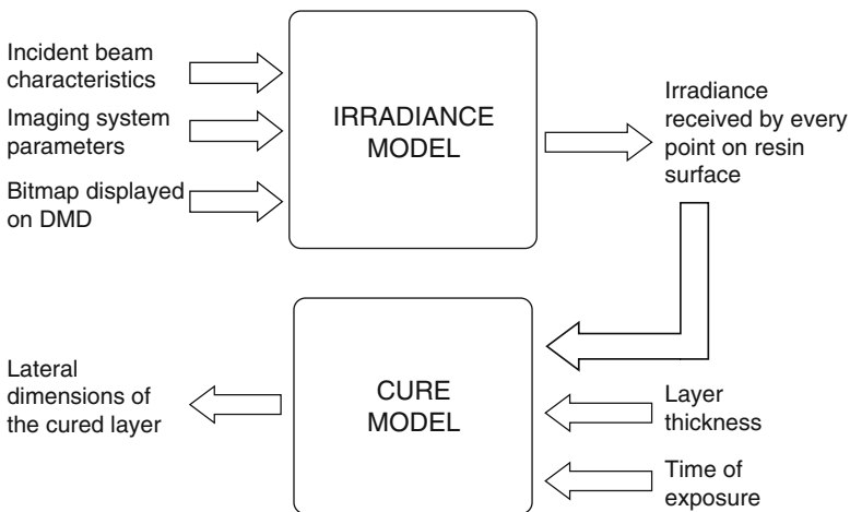
Fig. 4.17 Model of the MPVP process
