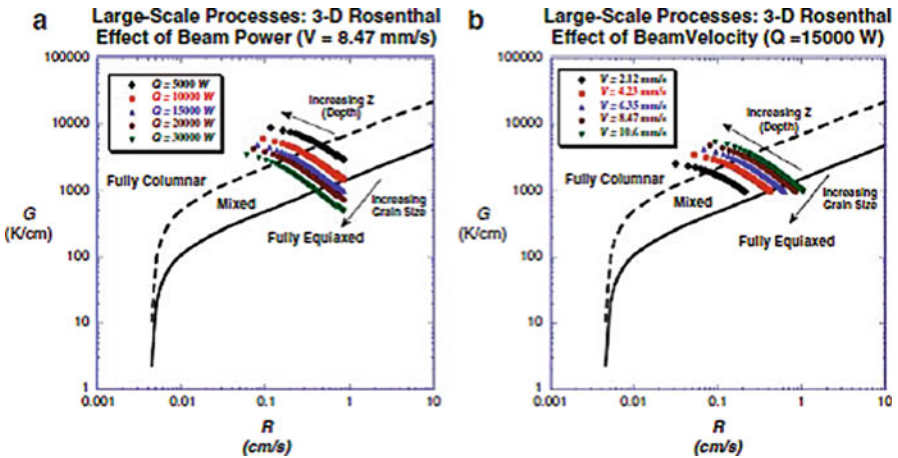
Fig. 10.16 Process maps showing microstructures predicted by the 3D Rosenthal solution for a higher-powered (AeroMet-like) directed energy deposition system for Ti–6Al–4V (MATERIALS SCIENCE & ENGINEERING. A. STRUCTURAL MATERIALS: PROPERTIES, MICROSTRUCTURE AND PROCESSING by Srikanth Bontha, Nathan W. Klingbeil, Pamela A. Kobryn and Hamish L. Fraser. Copyright 2009 by Elsevier Science & Technology Journals. Reproduced with permission of Elsevier Science & Technology Journals in the format Textbook via Copyright Clearance Center)
