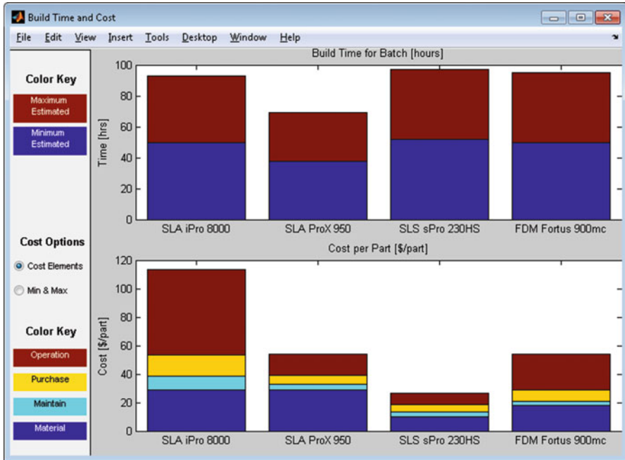
Fig. 13.11 Build time and cost results for the example
