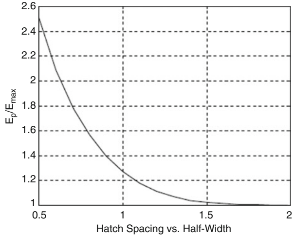
Fig. 4.14 Plot of (4.27): exposure ratios vs. size ratios
