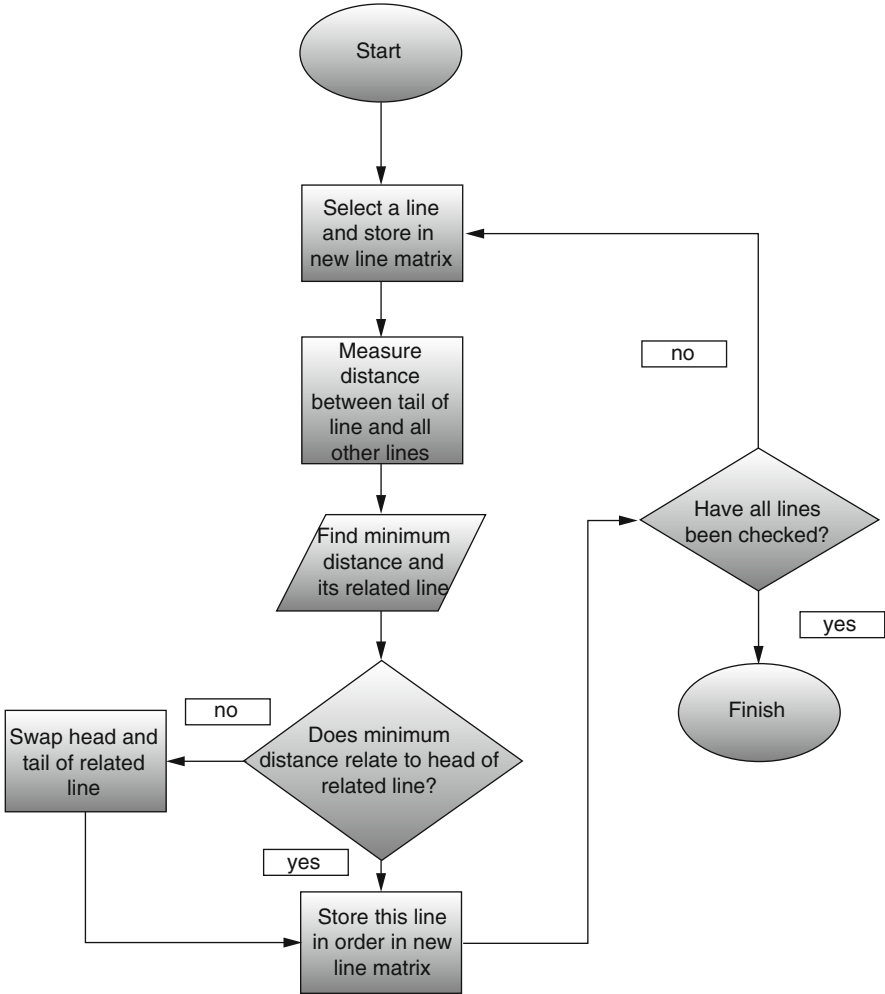
Flowchart 15.2 Algorithm for ordering the line intersections into complete outlines. This assumes there is only a single contour in each plane (adapted from [4])
