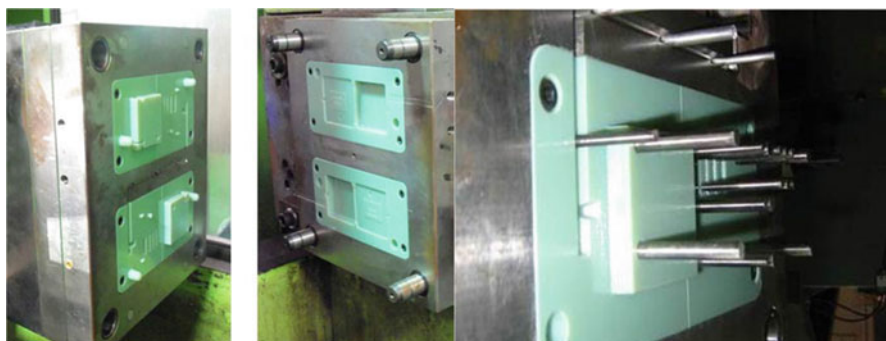
Fig. 18.3 Polyjet inserts for a two cavity mold set, showing a close-up of the ejector pins (courtesy Stratasys)
