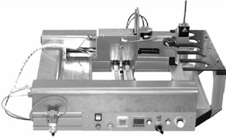
Fig. 19.7 The EnvisionTEC Bioplotter. Note the interchangeable extrusion head system and the extensive use of stainless steel in the fabrication
