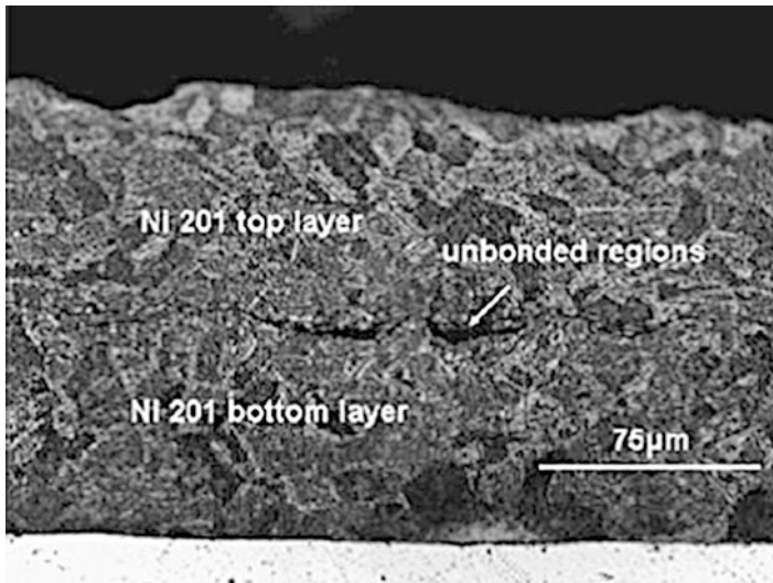
Fig. 9.14 Ultrasonically consolidated Ni 201 foils
