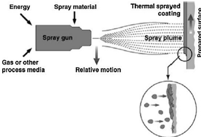
Fig. 11.7 General apparatus for thermal spray [15] (Courtesy of and (C) Copyright Sulzer Metco. All rights reserved)
