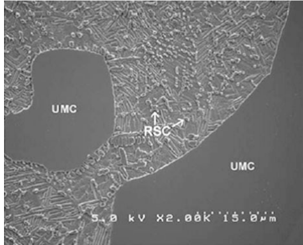
Fig. 17.4 Sixty percent CP-Ti, 40 % TiC composite made using LENS. The ratio of un-melted carbides (UMCs) to resolidified carbides (RSCs) within the Ti matrix is controlled by varying LENS process parameters
