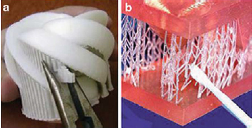
Fig. 14.4 Breakaway support removal for (a) an FDM part (courtesy of Jim Flowers) and (b) an SLA part (Courtesy Worldwide Guide to Rapid Prototyping web site. © Copyright Castle Island Co., All rights reserved. Photo provided by Cadem A.S., Turkey)
