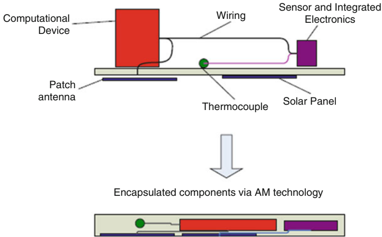
Fig. 9.18 Schematic illustrating the creation of a smart structure using UAM
