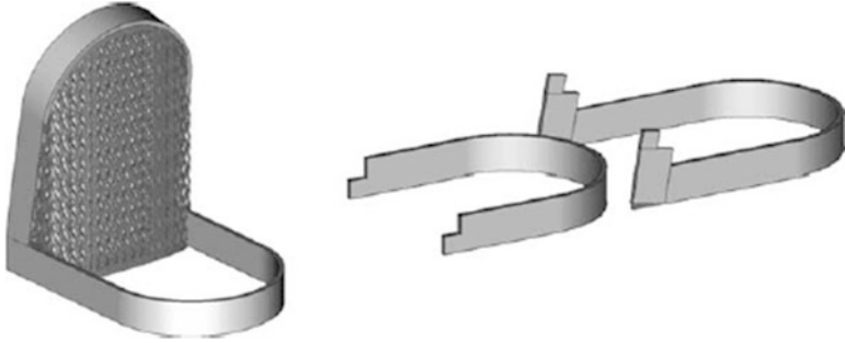
Fig. 3.2 The build on the left (shown with support materials within the arch) can be broken into the two parts on the right , which may be stronger and can be glued together later. Note the reduction in the amount of supports and the reduced build height
