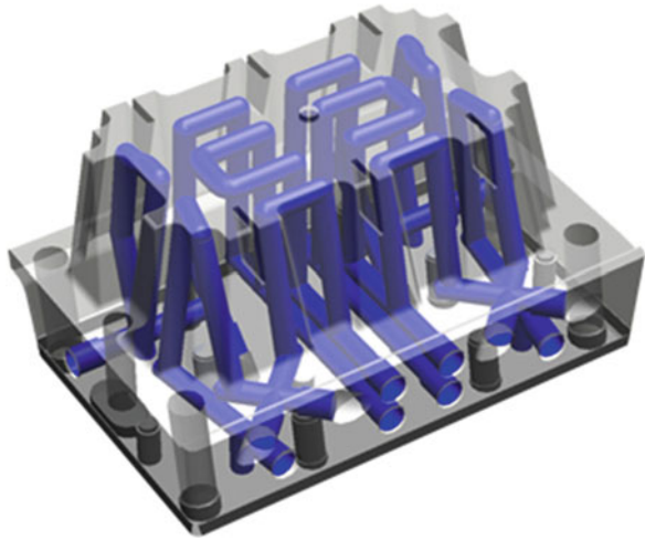
Fig. 18.5 A tool insert design, showing the location of conformal cooling channels
