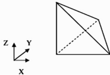
Fig. 15.1 A right-angled triangular pyramid as described by the sample STL file. Note that the bottom left-hand corner coincides with the origin and that every vertex coming out of the origin is of unit length
