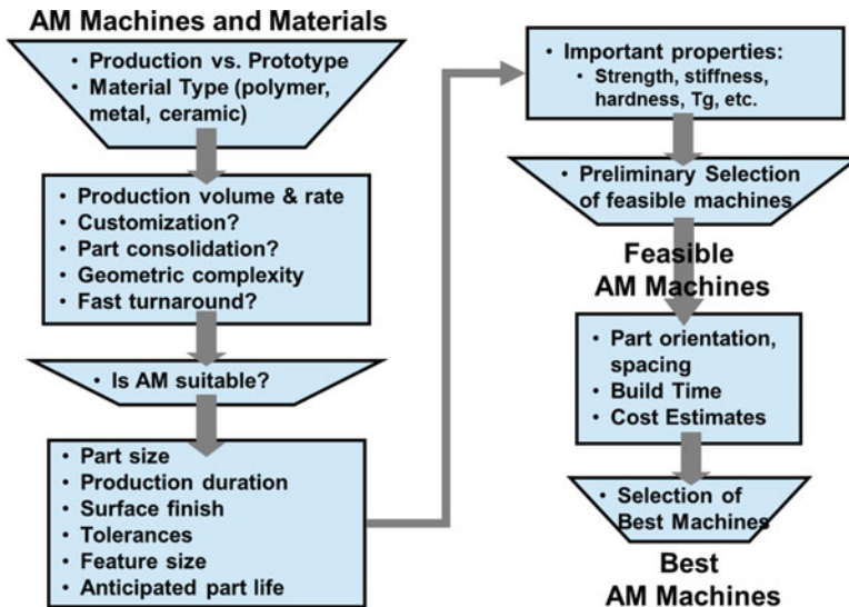
Fig. 13.5 Flowchart of AMSelect operation
