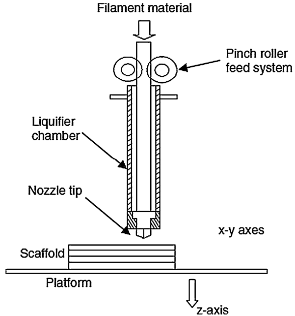
Fig. 6.1 Schematic of extrusion-based systems
