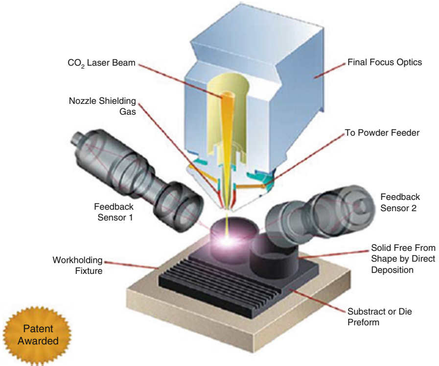
Fig. 10.7 POM DED machine schematic (courtesy POM)
