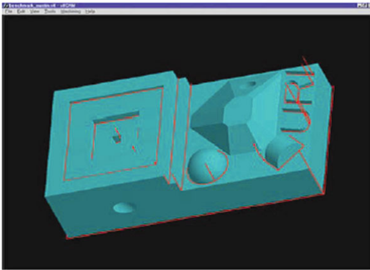
Fig. 14.9 Sharp edge contours identified for milling
