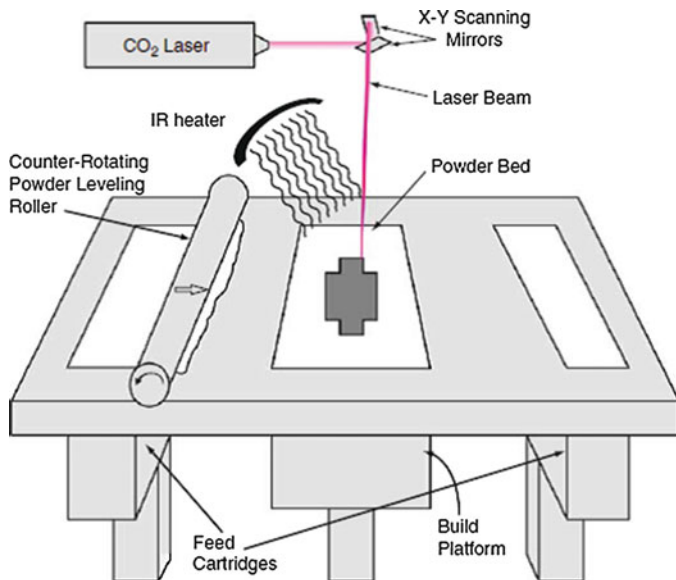
Fig. 5.1 Schematic of the selective laser sintering process
