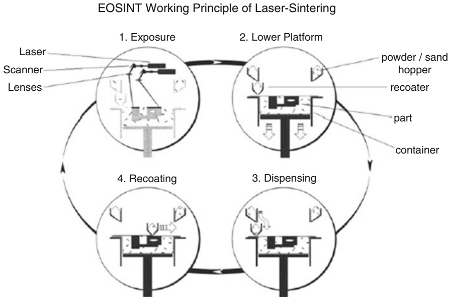
Fig. 5.12 EOSint laser sintering schematic showing the dual-laser system option, hopper powder delivery and a recoater that combines a movable hopper and doctor blade system (courtesy: EOS)
