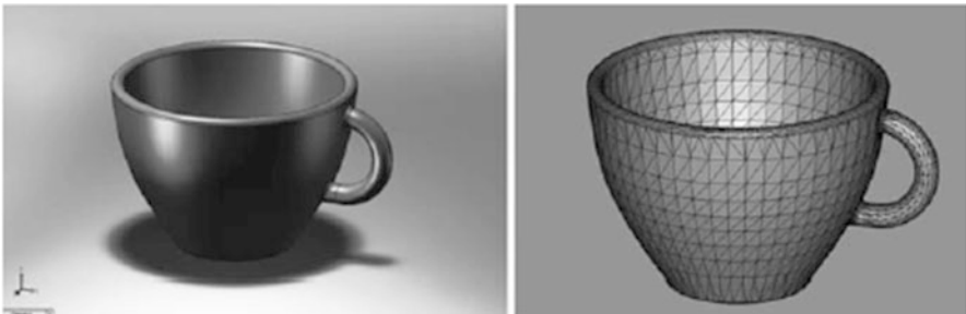
Fig. 2.2 A CAD model on the left converted into STL format on the right
