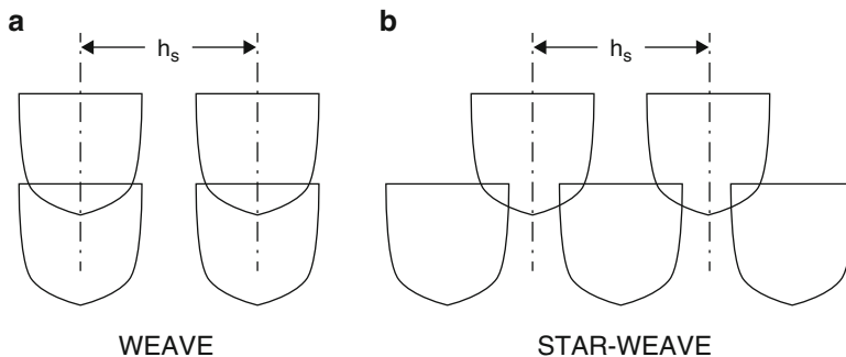
Fig. 4.10 Cross-sectional view of WEAVE and STAR-WEAVE patterns
