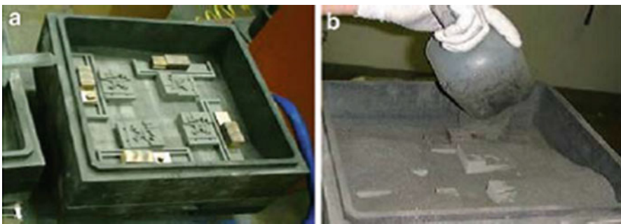
Fig. 14.14 LaserForm ST-100 green parts. (a) Parts are placed next to “boats” on which the bronze infiltrant is placed. The bronze infiltrates through the boat into the part. (b) The parts are often covered in aluminum oxide powder before placing them in a furnace to help support fragile features during debinding, sintering, and infiltration, and to help minimize thermal gradients
