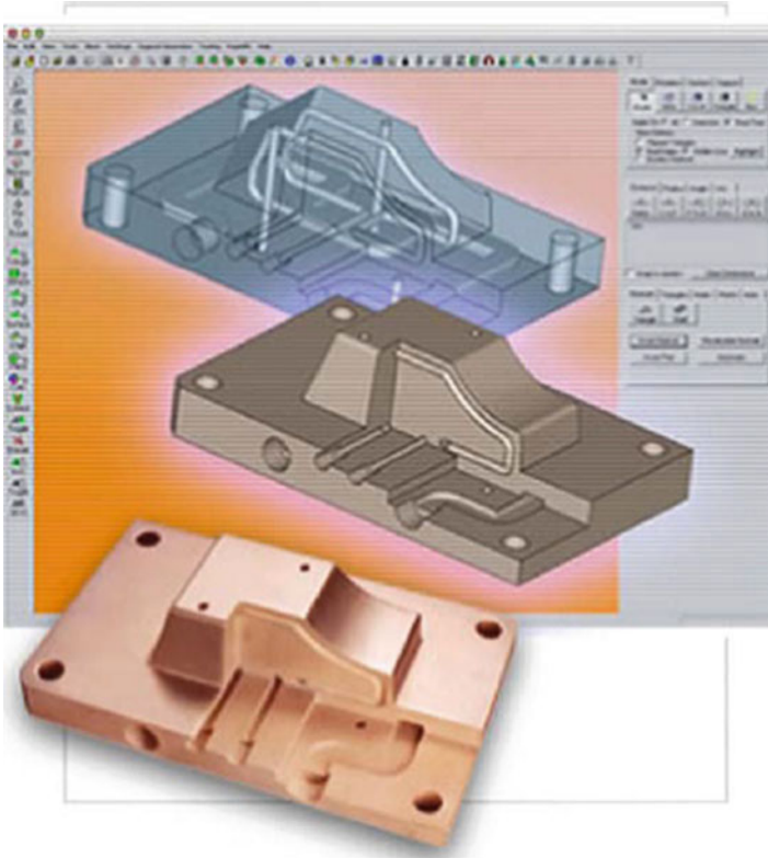
Fig. 14.15 Cross-section of a ExOne ProMetal injection molding tool showing CAD files and finished, infiltrated component with internal conformal cooling channels (Courtesy ProMetal LLC, an ExOne Company)
