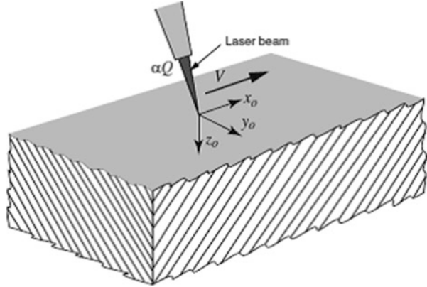
Fig. 10.14 3D Rosenthal geometry considered
