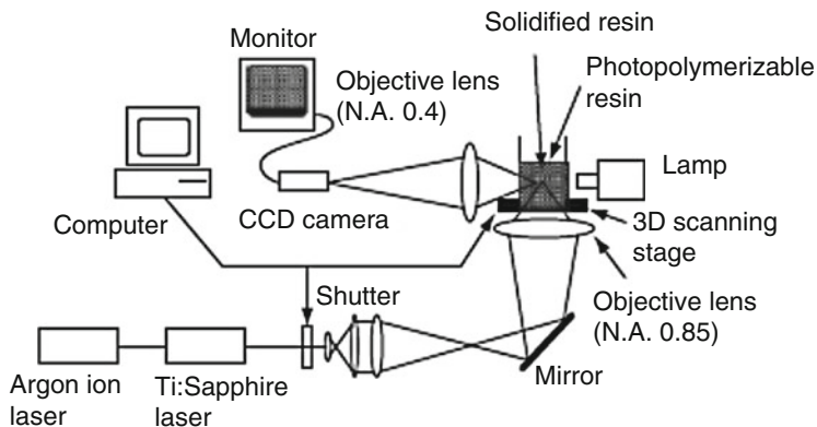
Fig. 4.18 Schematic of typical two-photon equipment
