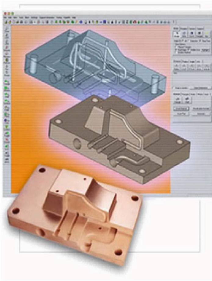
Fig. 8.5 Injection mold with conformal cooling channels fabricated in an ExOne machine (Courtesy ExOne Company)
