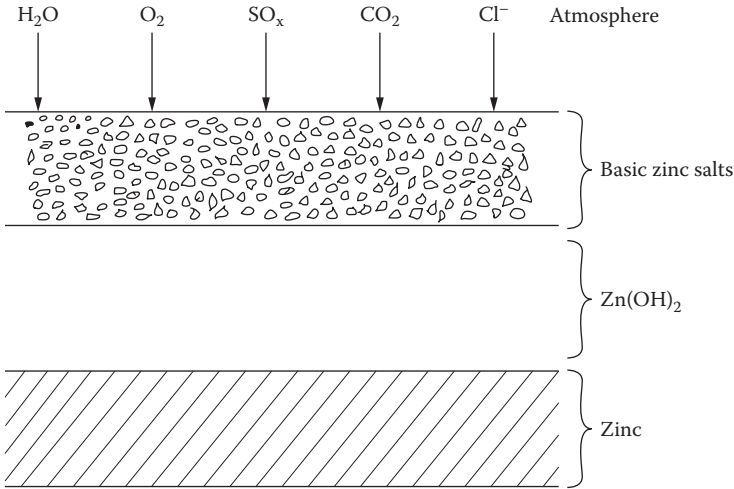
FIGURE 4.2 Corrosion products formed on zinc during atmospheric exposure. (Source: From Reference 5.)
