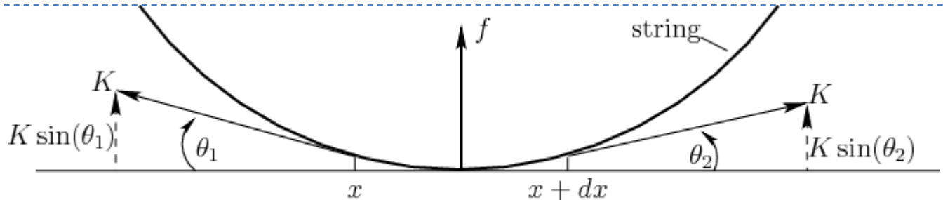
Force diagram for length dx string element
