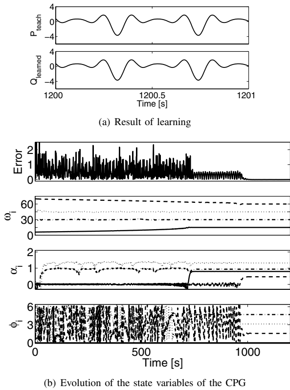
Fig. 2. Figure 2(a) shows the input signal to learn, P_{\text{teach}} , in the upper graph and the result of learning Q_{\text{learned}} in the lower graph. It is obvious that the network correctly learned the input pattern. Figure 2(b) shows the evolution of the state variables of the generic CPG during learning of an input signal ( P_{\text{teach}} = 0.8 \sin(15t) + \cos(30t) - 1.4 \sin(45t) - 0.5 \cos(60t) ) and the evolution of the error of learning. The upper graph is a plot of the error, defined by \text{error} = \|P_{\text{teach}} - Q_{\text{learned}}\| . The 3 other graphs show the evolution of the frequencies, \omega_i , the amplitudes, \alpha_i and the phases, \phi_i . The variables for each oscillator are plotted, variables of oscillator 0 are the plain lines, variables for oscillator 1 are the dotted-dashed lines, variables for oscillator 2 are the dotted lines and the dashed lines represent oscillator 3. The initial conditions are \alpha_i(0) = \phi_i(0) = 0 , x_i(0) = 1 , y_i(0) = 0 \forall i , \mu = 1 , \gamma = 8 , \epsilon = 0.9 , \eta = 0.5 and \tau = 2 . The frequencies \omega_i(0) are uniformly distributed from 6 to 70.
