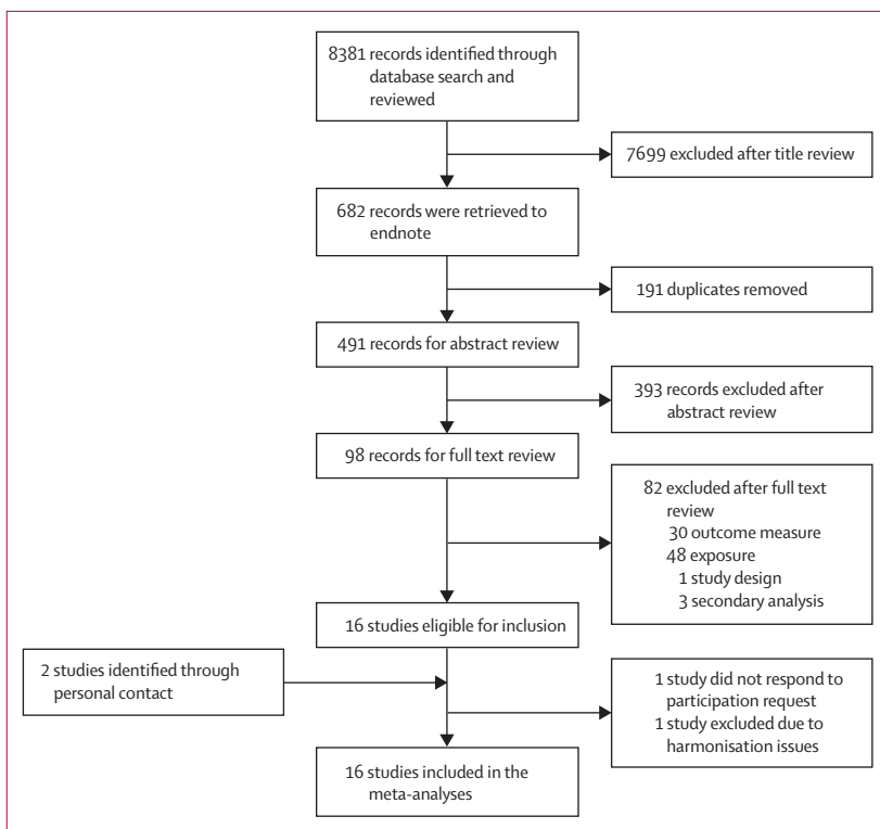
Figure 1: Study selection
