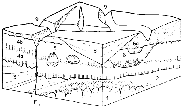
Fig. 5.5 Example of extrusive rock associations: for explanation, see text. F=fault.
