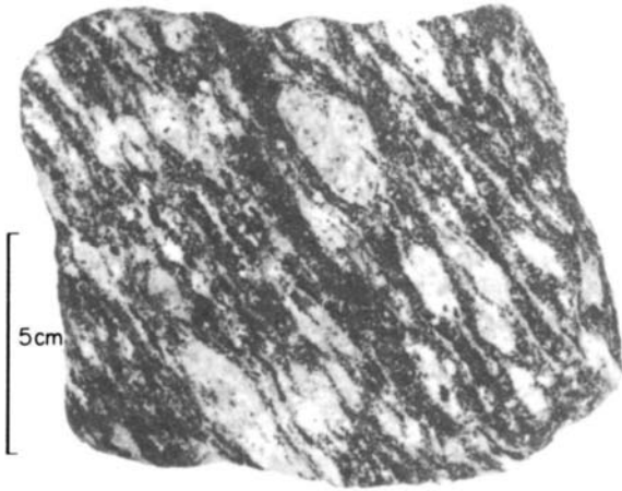
Fig. 7.9 Biotite-gneiss, Sutherland, showing foliation and augen-structure.
