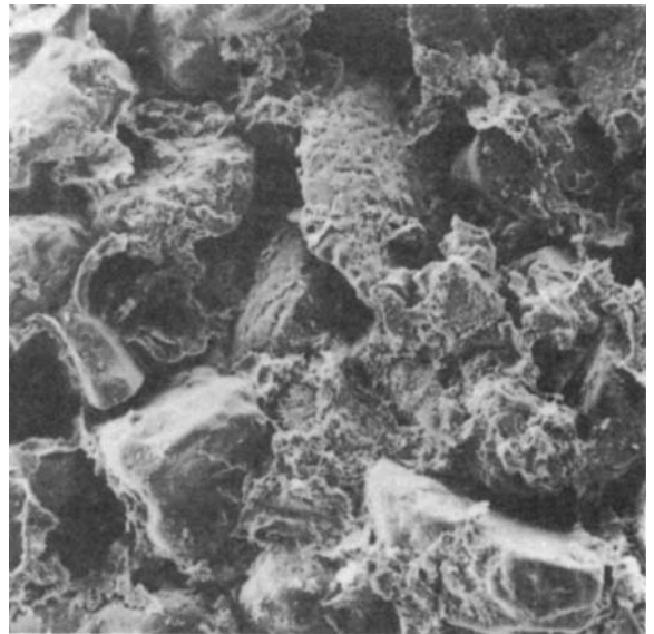
Fig. 6.10 Argillaceous sandstone as seen with an electron microscope: clay occupies the pore space. ( \times 100 ). Photograph by L. Dobreiner.
