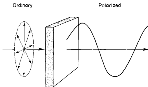
Fig. 4.11 Ordinary light (diagrammatic), composed of many vibrations in planes containing the direction of the ray (double-headed arrows represent double amplitude of vibrations) enters a crystal and is polarized, vibrations in one plane only being transmitted.
