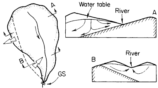
Fig. 18.1 On the left, a map of a catchment: solid line=topographic divide; broken line=ground-water divide; arrows indicate underflow . Two vertical cross-sections illustrate the geological structures that result in this underflow; arrows indicate movement of ground-water. GS=gauging station for measuring river flow.
