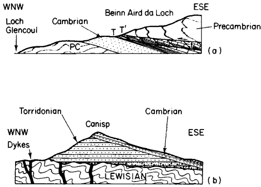
Fig. 2.6 The Precambrian of N.W. Scotland (Glencoul) (a) Precambrian thrust (T and T') over Cambrian that is unconformable on Precambrian. (b) Cambrian unconformable on Precambrian Torridonian, itself unconformable on Precambrian Lewisian. Two types of unconformity are shown: the old land surface at the base of the Torridonian, and the tilted plane of marine denudation on which the Cambrian rests. (c) Map of location.
