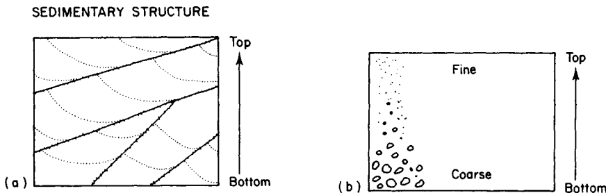
Fig. 2.1 Sedimentary structure. Indications of 'way-up' from small scale structures preserved in sediments: (a) current-bedding in a sandstone; heavy lines are erosion surfaces which truncate the current-bedded layers (dotted); the latter are asymptotic to the surface on which they rest (see also Fig. 3.19). (b) Graded bedding (see text). Note, the grains that constitute a sediment must be derived from rock that is older than the sediment the grains are forming.
