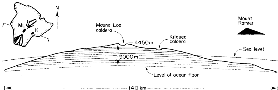
Fig. 5.4 A vertical section through the shield volcano of Mauna Loa, Hawaii, with silhouette of Mount Rainier drawn to the same scales. Sketch map of Hawaii shows recent lava flows and line of vertical section. (Data from Stearns, 1966.)
