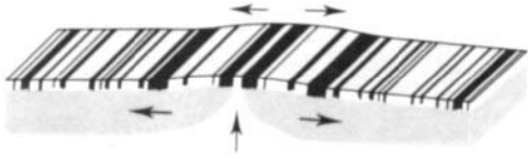
Fig. 1.15 Symmetrical pattern of magnetic stripes in oceanic crust at a spreading ridge (diagrammatic). Black stripes, normal polarity; white stripes, reversed polarity. The rocks at the ends of the diagram are about 8 my older than basalt rising in the centre.
