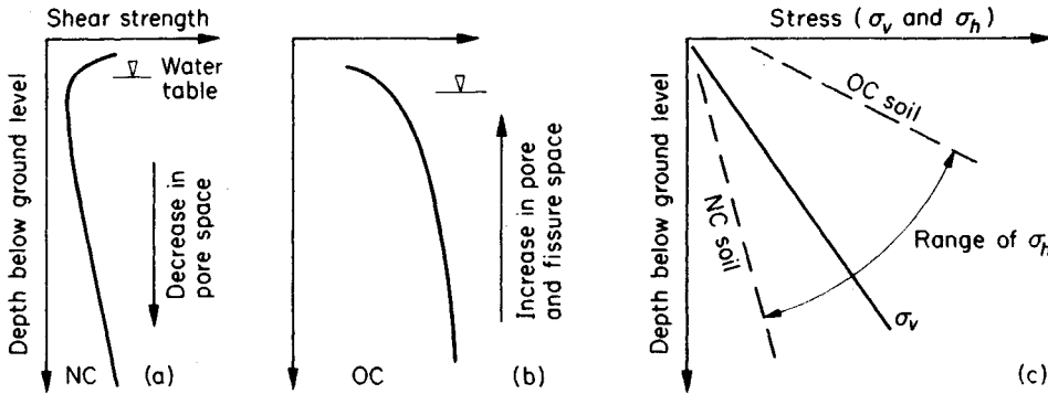
Fig. 9.6 Variation of strength of soils, and stress with depth. Increased strength above water table in (a) is associated with capillarity (see Fig. 9.23). NC=normally consolidated, OC=over-consolidated, \sigma_v and \sigma_h = in-situ stress in the vertical and horizontal directions. The ratio (\sigma_h/\sigma_v) = K_0 .
