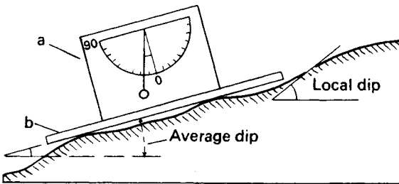
Fig. 12.8 Clinometer (a) with base plate (b) for 'averaging' dips.
