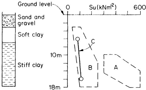
Fig. 11.4 Measurements of undrained shear strength ( S_u ). A=range as measured using bore-hole Penetrometer (cf. Fig. 10.20). B=range from 38 mm dia. and 98 mm dia. triaxial samples (cf. Fig. 9.11). C=results from 865 mm bore-hole Plate Bearing Test (cf. Fig. 10.16) (Marsland, 1971).
