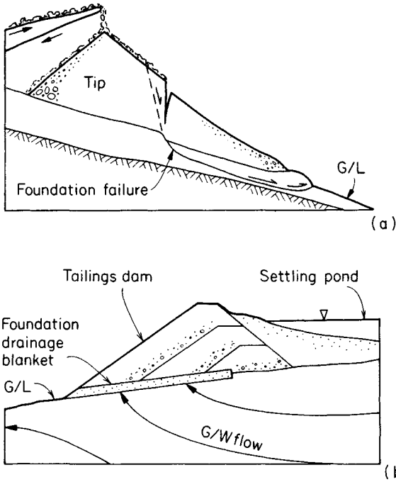
Fig. 16.26 (a) Simple tipping and associated danger of foundation failure (see also Fig. 14.20). (b) Tailings dam and appropriate drainage for controlling ground-water.
