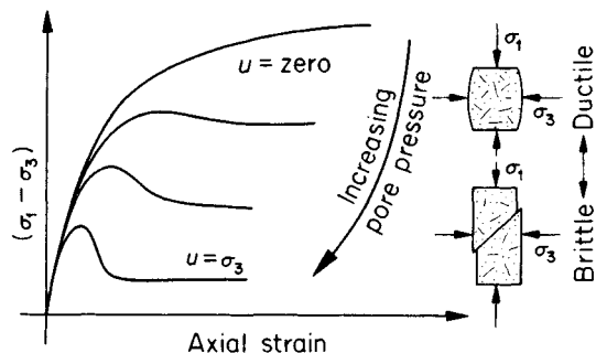
Fig. 9.20 Graphs showing the transition from brittle to ductile failure in rock as a function of pore water pressure ( u ): \sigma_3 the same for all tests. (From Robinson, 1959.)
