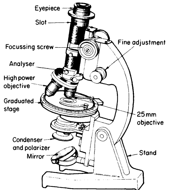
Fig. 4.13 A petrological microscope.
