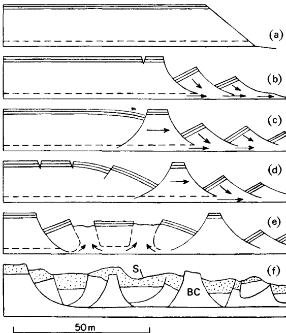
Fig. 14.11 Failure of Turnagain Heights cliffs, Alaska. (a)–(e), as developed in model tests; (f) final situation as observed in the field (after Seed, 1967). S=sands and gravel; BC=Bootlegger Clay.
