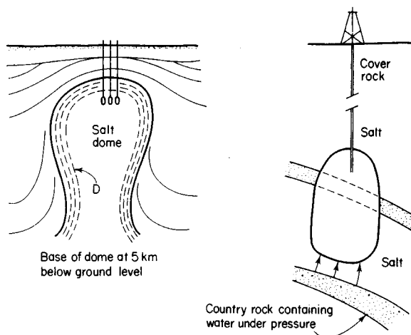
Fig. 15.17 General disposition of storage caverns in a salt dome and (right) detail of problems arising from inclusions of material other than salt (Lechler, 1971 and Hardy et al. , 1984). D=most disturbed zone (see also Fig. 6.21c).
