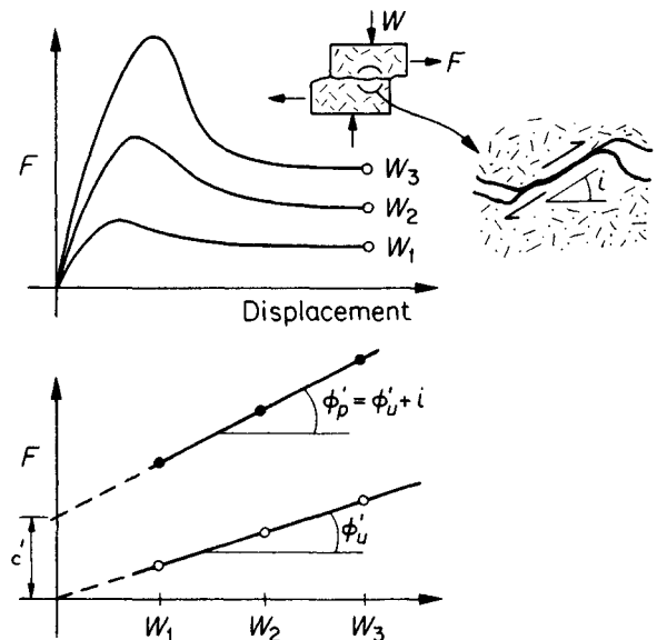
Fig. 9.25 The response of a rough surface to displacement. Note that the inclination ( i ) of an asperity may increase the resistance to shear ( F ) and causes surfaces to dilate. c' = cohesion, \phi' = angle of shearing resistance (see text).
