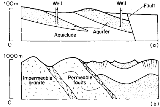
Fig. 13.10 Characteristic aquifers: (a) as strata, (b) as zones associated with faulting, and tensile fracturing on fold crests.
