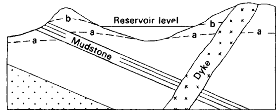
Fig. 15.4 Water-tight reservoir assured by sedimentary and igneous aquicludes. a = original water level; b = water level after impounding.
