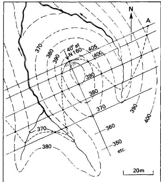
Fig. 12.14 Location of concealed boundary as defined using stratum contours (see text).
