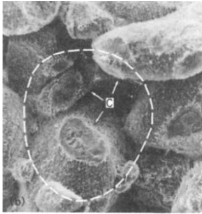
Fig. 6.9 (a) Penrith sandstone in thin section, showing enlargement of grains by new growth of quartz. ( \times 12 ). See also Fig. 6.2. (b) Cemented sandstone as seen with an electron microscope. c = cemented contact areas for a grain that has been removed ( \times 75 ). Photograph by L. Dobreiner.
