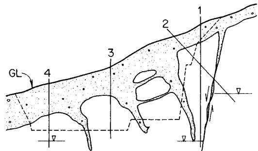
Fig. 18.7 Vertical section through a hillside and outline of proposed quarry (broken line). The ground was investigated using four bore-holes and bedrock was assumed to have a surface that followed the general shape of ground level. See text.
