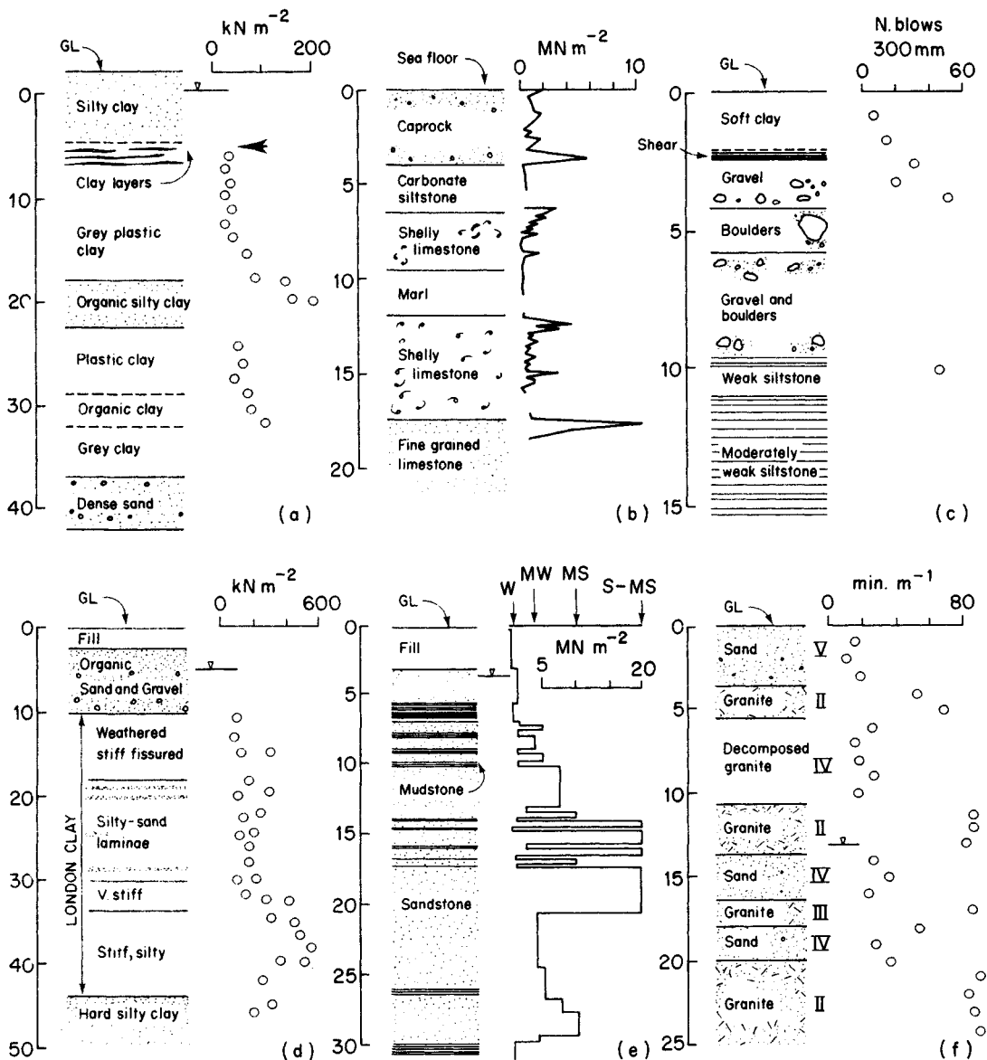
Fig. 18.10 Six vertical profiles, recording the geology beneath foundations and illustrating the variety of techniques that may be used to describe the strength of the ground (see text).
