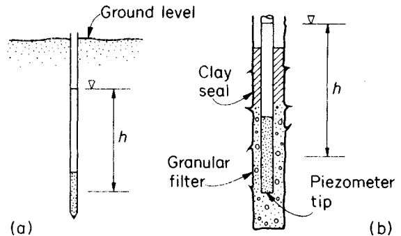
Fig. 10.15 Two examples of a stand-pipe piezometer. (a) Can be driven into the ground and need not require a bore-hole; (b) is an installation in a bore-hole. The fluid pressure = unit weight of water \times h .
