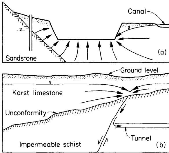
Fig. 16.7 Excavations influenced by remote sources of water.
