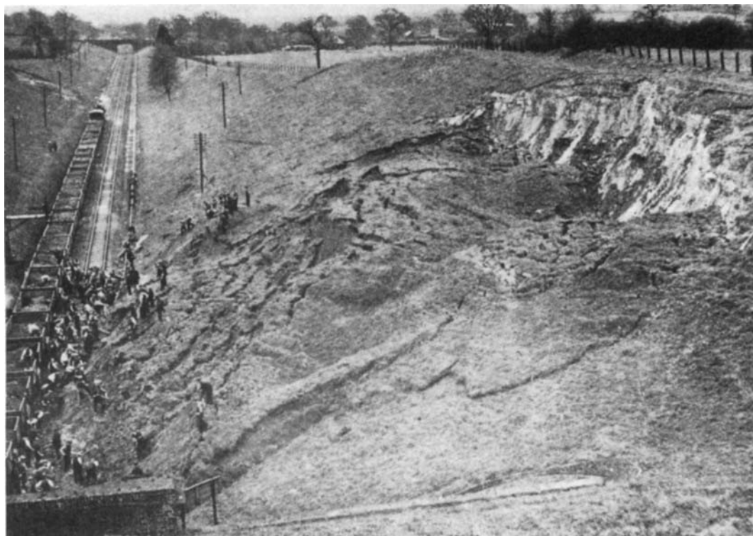
(f) Sevenoaks slip in Weald Clay, an example of failure of a man-made slope (reproduced by permission of the Chief Engineer, British Rail).
