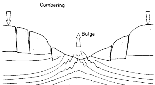
Fig. 8.17 Valley bulging and associated movement (cambering) of the valley sides (see also Figs 14.10 and 16.12).
