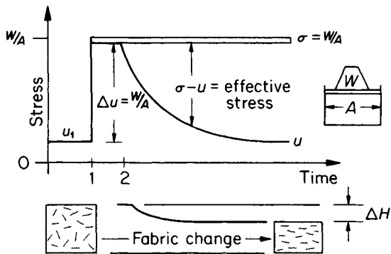
Fig. 9.8 Consolidation of soil (see also Fig. 9.7) 1=application of load ( W ). 2=start of pore fluid drainage.
