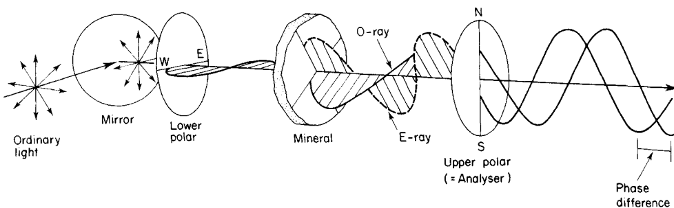
Fig. 4.14 Passage of light through microscope (diagrammatic): plane of polarization is 'E-W' for lower polar, and 'N-S' for upper polar, but may also be 'N-S' and 'E-W' respectively.
