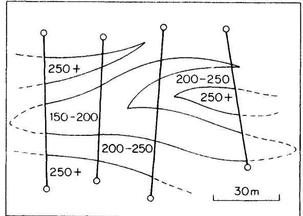
Fig. 12.6 Iso-resistivity map showing four traverse lines along which values for the apparent resistivity of the ground were measured: values in ohm-metres. High resistivity indicates poor rock (Oliveira et al. , 1974.)
