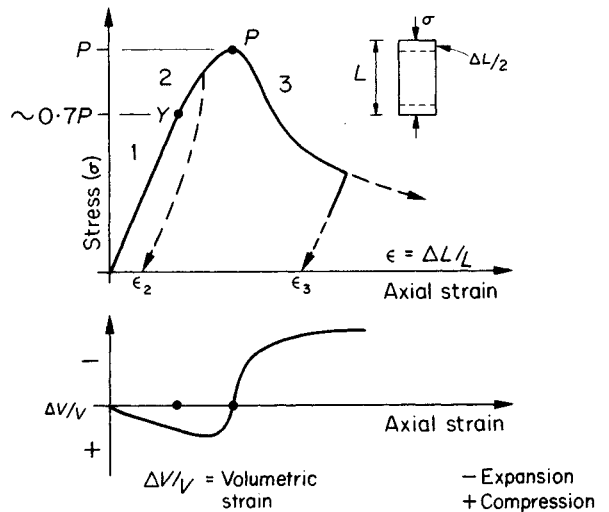
Fig. 9.13 Stress-strain curve for rock. Note: axial strain for complete failure is usually less than 1%. Y = yield stress, P = peak strength (see text).
