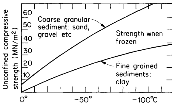
Fig. 17.16 Likely strength for frozen ground. The temperature for brines ranges from -30^{\circ} to -50^{\circ}\text{C} and that for liquid nitrogen is -196^{\circ}\text{C} . (Data from British Oxygen Co., U.K.)
