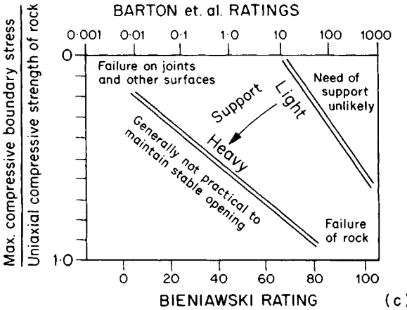
Fig. 16.21 Essential elements of classifications of rock masses by (a) Bieniawski, (b) Barton et al. References cited give details and support recommendations. (c) Approximate relationships for large excavations: boundary stress = stress on roof or walls or excavation (from Hoek, 1981).
