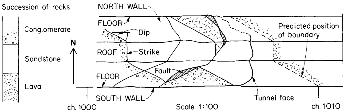
Fig. 16.20 Example of a simple tunnel log. (ch=chainage) and prediction. Such plans can be cut out and the walls folded down to make a simple 3-dimensional model of tunnel geology (see also Face Logs: Fig. 10.7).
