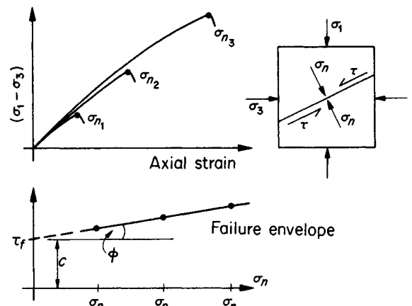
Fig. 9.16 Coulomb failure envelope. \sigma_n = stress normal to failure surface. \tau = shear stress along the failure surface.
