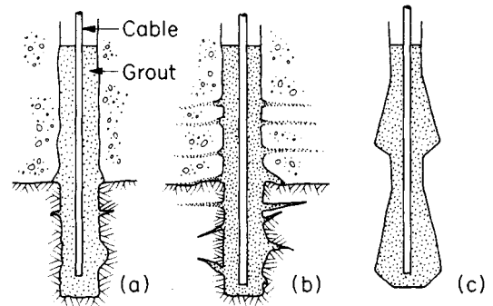
Fig. 17.20 Anchorages for cables: (a) grouted bore-hole, (b) bore-hole grouted under pressure to fill fractures in rock and coarse permeable horizons in the overlying drift, (c) under-reamed. (a) and (b) are suitable for use in soil and rock, (c) is suitable for stiff to very stiff clays and weak rock.
