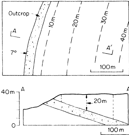
Fig. 12.3 Ischore map for thickness of overburden above a deposit of sand and vertical cross-section.
