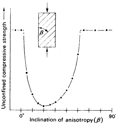
Fig. 11.5 Influence of anisotropy on strength (Donath, 1961)
