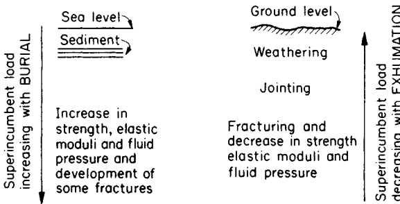
Fig. 9.1 Effect of loading and unloading on the properties of sediments.
