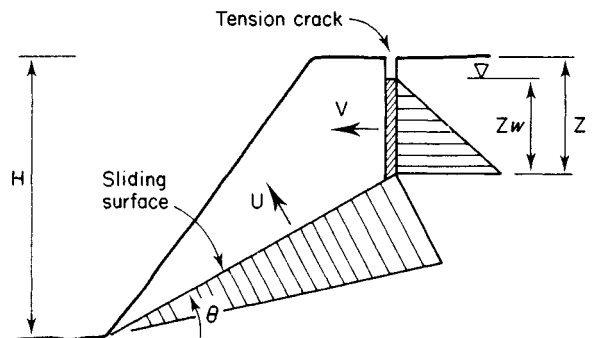
Fig. 14.7 Forces produced by water confined in a tension crack and along a planar sliding surface.
