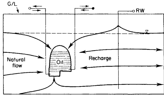
Fig. 15.19 Vertical section showing oil retained by ground-water flow towards a chamber. Below the oil is a water sump. RW=recharge well when required to create a lateral water barrier. Broken line=original water table.
