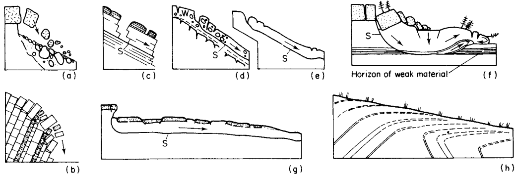
Fig. 14.1 Some common slope movements: S=sliding surface, W=weathered zone (see also Table 14.1 and text).
