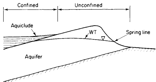
Fig. 13.11 Unconfined outcrop of scarpface with dip-slope confined beneath aquiclude.
