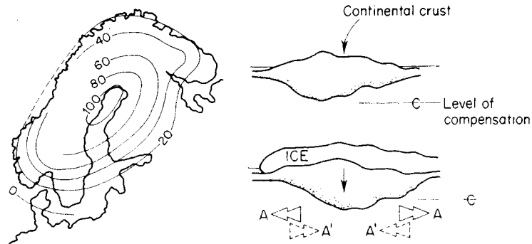
Fig. 2.20 Post-glacial uplift of Scandinavia (in metres). A, signifies the migration of material in the asthenosphere following ice loading. When the ice load is removed isostasy restores the level of compensation at a rate permitted by the return of material in the asthenosphere (A'). (From Woldstedt, 1954.) The present rate of uplift is 2 mm/year in southern Sweden and 9 mm/year in central Sweden.
