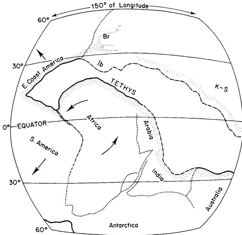
Fig. 2.12 Late Jurassic framework for the Alpine orogeny (based on Smith, Hurley and Briden, 1981; Ager, 1975; Jenkyns, 1980). Ib, Iberia; Br, Britain; K-S, Kazakhstan-Sinkiang.
