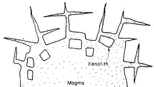
Fig. 5.14 Schematic vertical cross-section of a plutonic intrusion at depth, stopping country-rock. Xenolith=slab of country-rock enclosed in the mass near its walls and roof. Small inclusions of country-rock have been softened and dispersed in the igneous rock as it cooled slowly, locally modifying its composition near its contacts. Thus a granite may grade into quartz-diorite and diorite at its margin.
