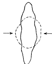
Fig. 7.7 Change of shape of a grain, e.g. quartz, under stress, original grain shown by dotted outline. Stress lowers the melting point, especially where grains touch; solution takes place there with redeposition along directions at right angles to the maximum stress direction (arrowed).
