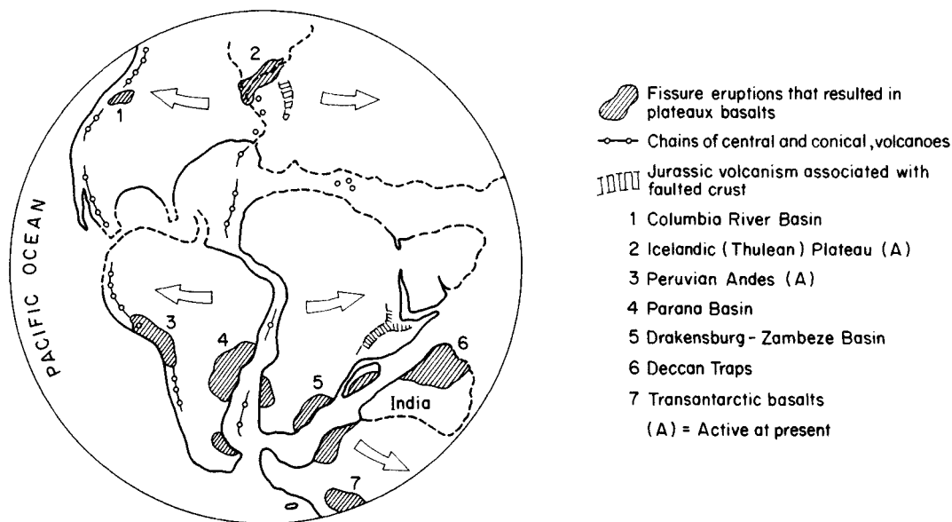
Fig. 2.13 Major volcanic centres of Late Mesozoic and Cenozoic age. (Position of continents is that of Late Jurassic: 150 my ago.)
