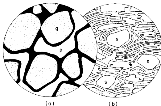
Fig. 6.1 Two sedimentary rocks, in thin section. (a) Sandstone with iron cement (black) coating the sand grains (g); p, pore ( \times 30 ). (b) Compacted clay with silt (s). Stipple = smaller crystals of clay mineral and new minerals formed by precipitation from pore water during compaction ( \times 1000 ).
