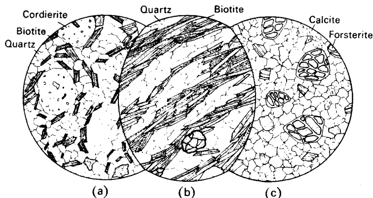
Fig. 7.4 Metamorphic rocks in thin section: (a) Biotite-cordierite-quartz-hornfels; the rounded cordierite contains many inclusions. (b) Mica-schist with garnets. (c) Forsterite-marble (all \times 15 ).
