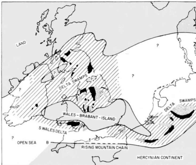
Fig. 2.11 Probable geography of north-west Europe in Coal Measure times (after L.J. Wills and D.V. Ager, 1975). Present day coalfields shown in black, under-ground extensions dotted; they lie to the north of the Hercynian mountain front.
