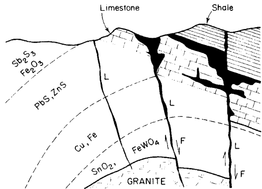
Fig. 5.27 Vertical section diagrammatically illustrating lodes (L) emanating from an intrusion at depth, with zoning of mineral deposits (see text) and solution in limestone F = fault, black = massive mineral deposit.
