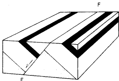
Fig. 8.25 Normal strike fault (FF) with dip in opposite direction to that of strata, and repeating the outcrop of some beds.
