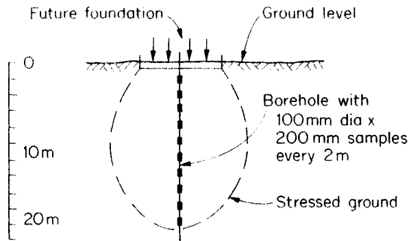
Fig. 11.1 Some limitations with sampling. The total volume of samples is approximately 1/250 000th of the stressed ground. See also Fig. 10.1.
