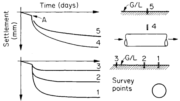
Fig. 16.24 Nature of settlements associated with tunneling. Prior to 'A' tunnel face is approaching the survey points. At 'A' it is beneath them. After 'A' it is moving away from them.
