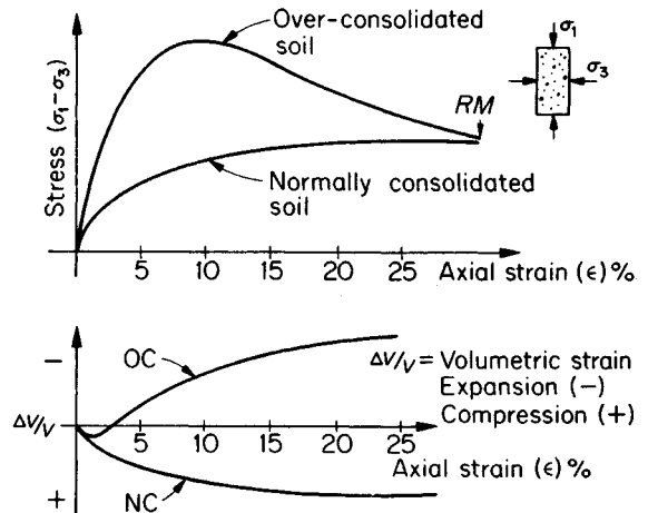
Fig. 9.15 Stress-strain curves for a drained soil, with representative strains: Note large strains required. Normally consolidated soils can exhibit a peak if their fabric is well developed, or strengthened with inter-particle bonds.
