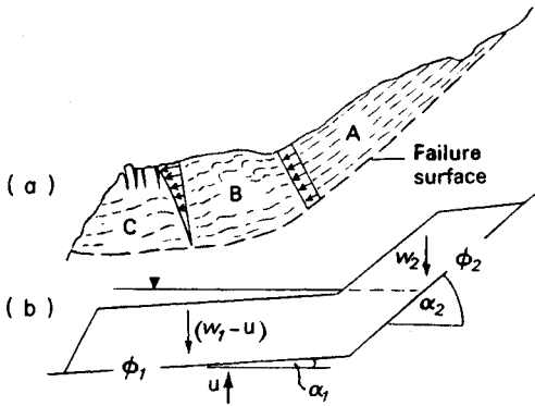
Fig. 14.16 (a) General character of the slide (after Muller); arrows show relative velocities of movement. (b) Section analysed by Jaeger (1969); W = weight of rock and reservoir water above rock; u = uplift pressures; \phi = angle of friction; \alpha = dip of sliding surface.
