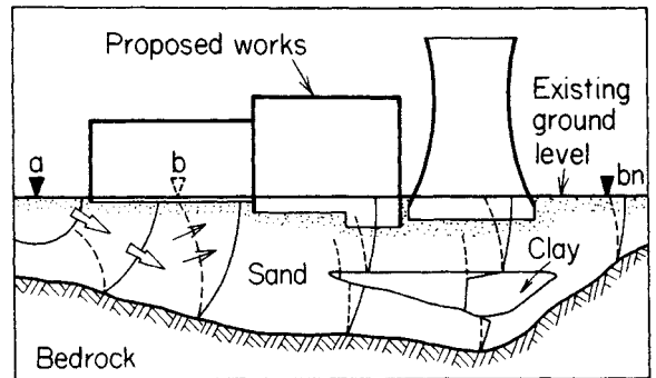
Fig. 10.18 Seismic investigation of ground beneath a proposed power station. A seismic source at a emits shock waves whose direct and reflected accelerations (solid lines and broken lines in the figure) are detected by geophones located along a line from b to bn. The dynamic characters of the overburden and bedrock may be deduced from the velocity of the waves, and those returned by bedrock and other surfaces including the boundaries of the buried valley filled with clay, reveal the stratigraphy and structure of the site (p. 176).
