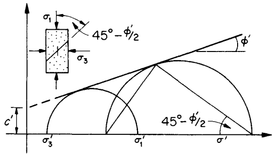
Fig. 9.18 Mohr-Coulomb failure envelope for soil.
