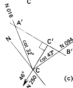
Fig. 12.12 Use of apparent dips for calculation of true dip (see text).
