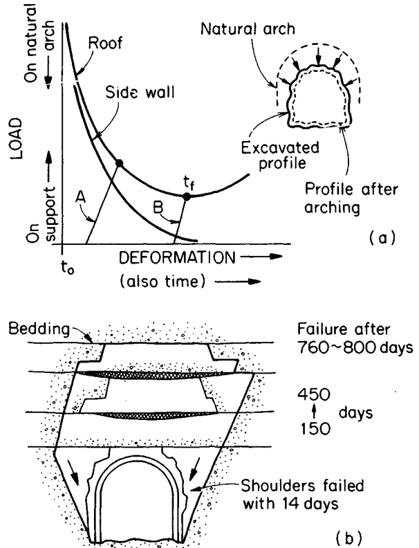
Fig. 16.19 (a) Load on excavation boundary. From t_0 \rightarrow t_f a ground arch is forming. At t_f the deformation is too great and the ground arch begins to fail. A = support that is applied too early, or is too stiff; B = proper support (Deere et al. , 1969). (b) Roof sag and final failure recorded during an experimental tunnel collapse (Ward, 1978). This behaviour agrees with the general form of the curves proposed by Deere and shown in (a) above.
