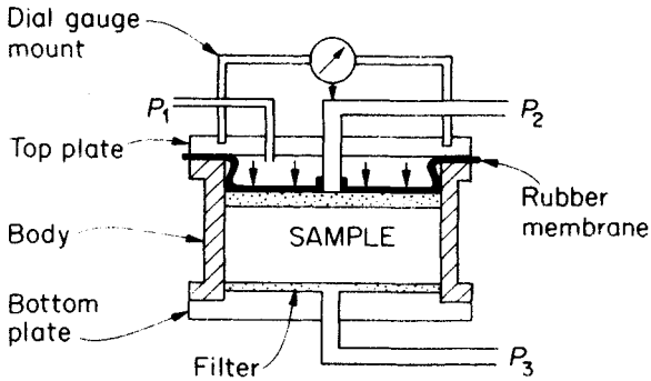
Fig. 11.7 Rudiments of a Rowe Cell (Rowe and Bardon, 1966). The sample is loaded by hydraulic pressure P_1 , and consolidated by drainage via P_3 . Pore pressures can be measured at both ends of sample via P_2 and P_3 . Dial-gauge measures change in sample thickness.
