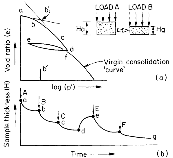
Fig. 17.12 The consolidation of a sediment and its response to unloading. (a) with respect to effective stress and (b), with respect to time (see also Fig. 9.8).
