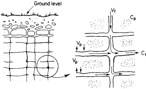
Fig. 13.6 Reaction of ground-water chemistry to host rock environment. Slow moving water in rock pores (velocity V_p , chemical concentration C_p ) and fast moving water in fissures ( V_f ) of composition ( C_f ). V_f \gg V_p and C_p \gg C_f .
