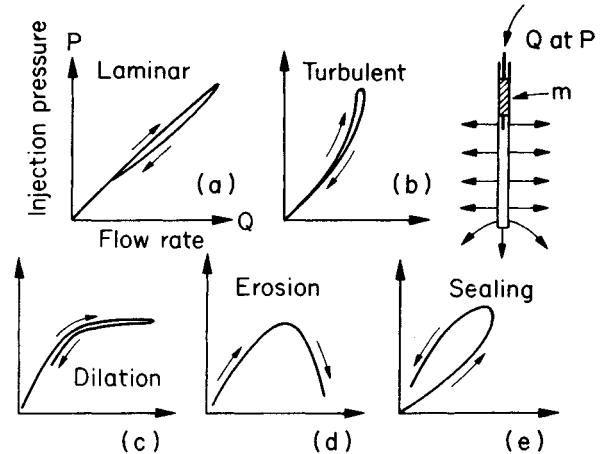
Fig. 17.9 Form of ground response to injection, as recorded from a water absorption test: in each case the ordinate represents injection pressure and the abscissa, flow rate into the ground: based on Housby (1976). The test is conducted over a section of bore-hole isolated by a packer (m): see text.
