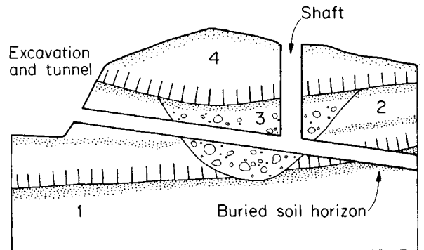
Fig. 16.23 Example of the variations that can be encountered in volcanic rocks. Strong lavas 1, 2 and 4 contain weak zones, profiles of weathered rock, and soil horizons, and moderately strong buried river deposits (3).
