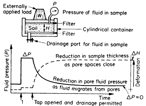
Fig. 9.7 Deformation of soil under load. This test is normally conducted in apparatus called an oedometer (see Fig. 11.6). \Delta P =changes in fluid pressure. \Delta H =changes in sample thickness. 1=Load applied whilst tap is shut and drainage prevented. Fluid pressure increased and small, reversible, elastic shortening occurs.
