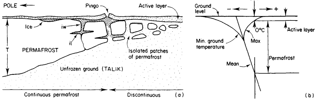
Fig. 3.6 Permafrost. (a) Vertical profile through ground containing permafrost. Thickness of permafrost ( T ) may be 1000\text{ m}+ . (b) Temperature distribution with depth. As ground temperature fluctuates between summer maximum and winter minimum, so a depth of ground ( 0.5 to 3.0\text{ m}+ ) is seasonally frozen and thawed (the active layer). iw = ice wedge; il = ice lense. Based on data from Brown (1970) and Stearns (1966).
