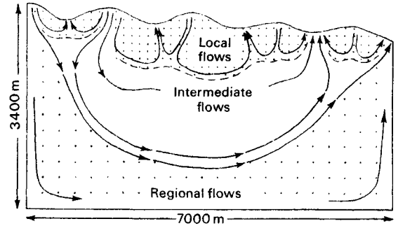
Fig. 13.3 Theoretical distribution of flow (after Toth, 1963): illustrating the relatively rapid circulation of ground-water near surface (local flows), deeper, slower circulation and the very slow circulation of regional flows at great depth.
