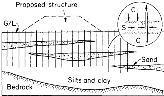
Fig. 17.3 Vertical drains, with detail illustrating how such drains encourage permeable horizons of silt and sand (S) to drain the less permeable material, clay (C).
