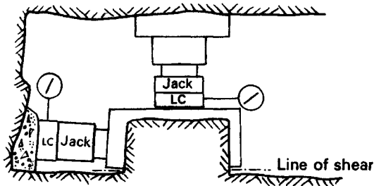
Fig. 10.19 Direct shear test: arrangement for use in situ. Displacement gauges not shown. LC = load cell. Area of shear approximately 1 m 2 .
