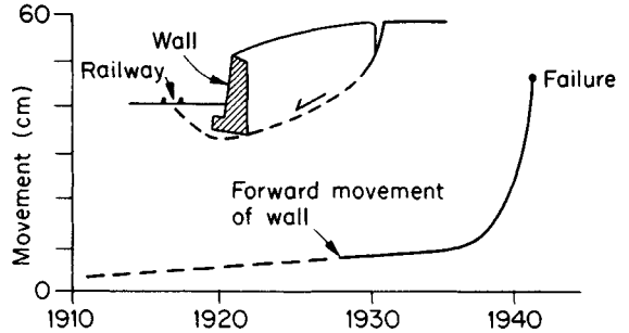
Fig. 9.27 Example of slope movement over a period of 30 years (after Skepton, 1964).
