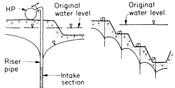
Fig. 17.2 Dewatering point (HP=header pipe) and example of staged excavation.
