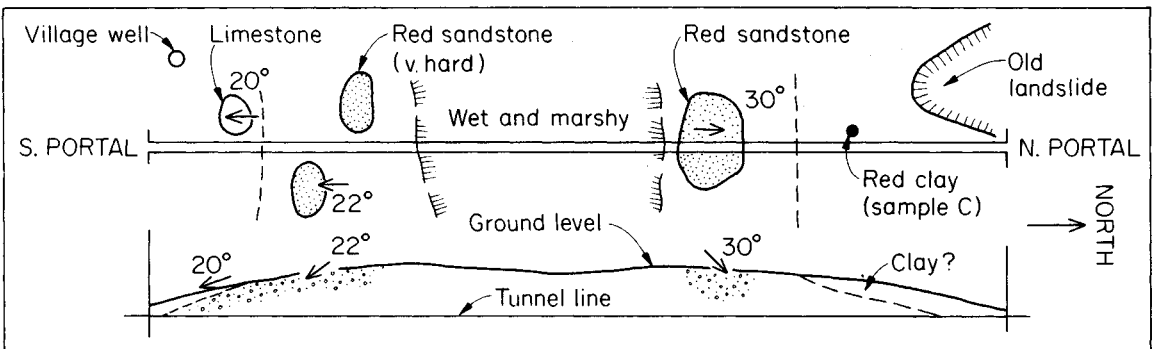
Fig. 12.9 Engineer's record from a surface traverse survey for a tunnel: sketch map, and sketch section below.
