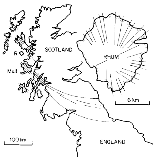
Fig. 5.8 Tertiary dyke swarms of the British Isles, with inset showing the radial dykes of Rhum (R). (Data from Geol. Survey. G.B. 1961. )
