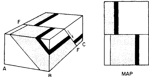
Fig. 8.23 Effect of normal dip fault (FF) on dipping strata, and appearance of this effect as recorded on a map.
