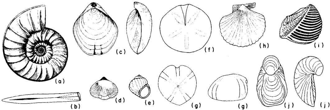
Fig. 2.14 Mesozoic fossils: \times \frac{1}{2} except (a). Ammonite: (a) Asteroceeras (Jur), (b) A belemnite. Brachiopods: (c) Terebratula (Cret), (d) Rhynchonella (Jur). Gastropod: (e) Paludina (Cret). Echinoids: (f) Clypeus (Jur), (g) Micraster (Cret). Lamelli-branths: (h) Pecten (Jur), (i) Trigonina (Jur), (j) Gryphaea (Jur).
