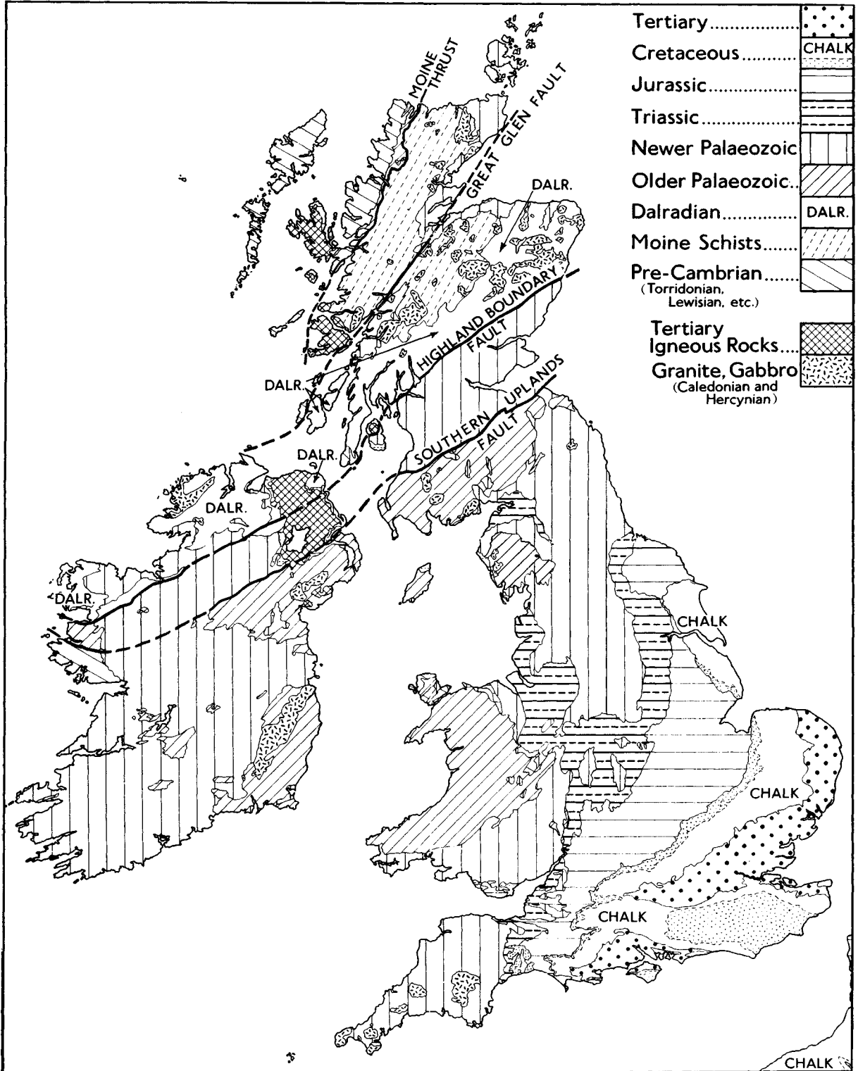
Fig. 2.18 Outline geological map of the British Isles. Scale approximately 1:5 000 000.
