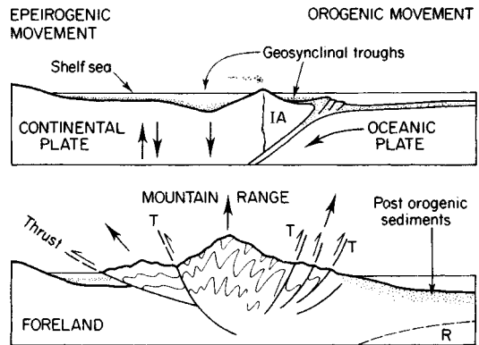
Fig. 2.3 An example of the relationship between epeiric seas, geosynclines and plate tectonics. IA = Island Arc; R = remnant of oceanic plate; T = thrust. Large arrows represent the directions of movement.
