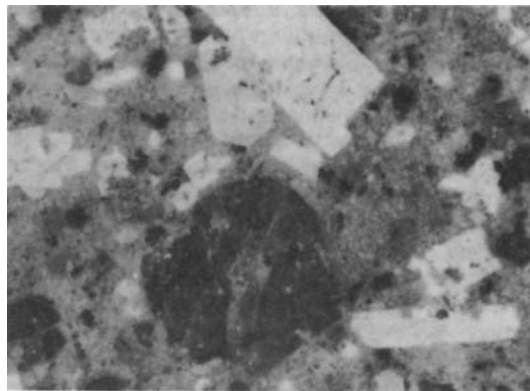
Fig. 5.25 Polished surface of quartz-porphry. Cornwall ( \times 3 ). Feldspar, white; quartz, grey; biotite, black.
