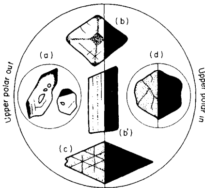
Fig. 4.34 Some accessory minerals in thin section ( \times 15 ). (a) Zircon (at greater magnification than other minerals shown). (b) Chiastolite cross-section, (b') long section. (c) Sphene. (d) Garnet, showing isotropic character under crossed polars.
