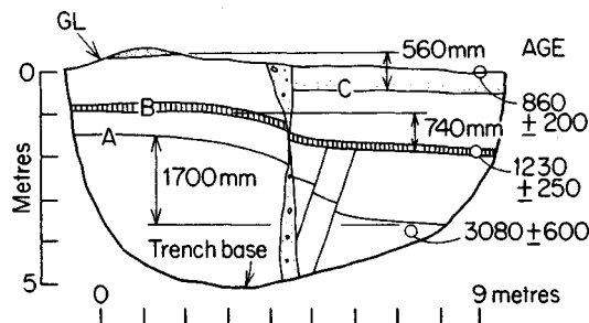
Fig. 18.15 Trial pit in Recent lacustrine sediments where fault displacements record former earthquakes. Dates provided by C^{14} and given in years since present. The event that broke layer A displaced it by 1700–740 mm, i.e. 960 mm; that for B by 740–560 mm (from Clark et al. , 1972).
