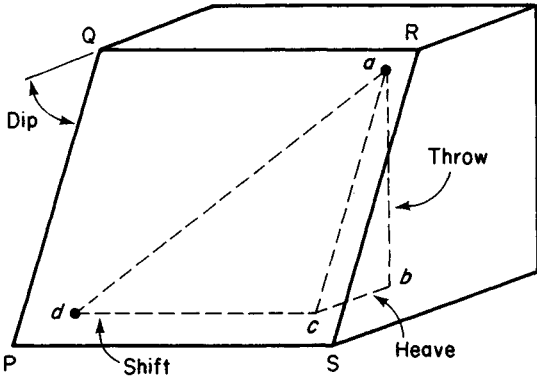
Fig. 8.22 Components of fault displacement. PQRS=fault surface. ad =total slip; ab =throw; bc =heave; cd =shift or strike slip being along the strike of the fault surface; ac =dip slip being along the dip of the fault. The points a, c, d lie on the fault surface.
