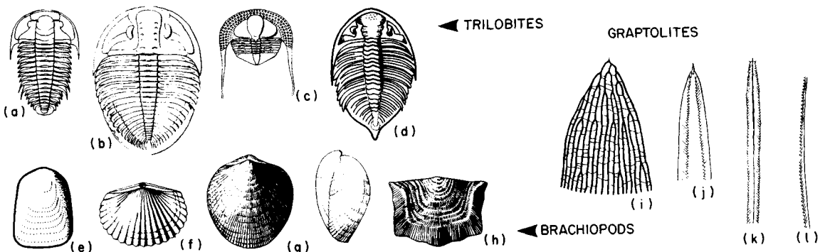
Fig. 2.8 Older Palaeozoic fossils (approximately half life size). Trilobites: (a) Olenus (Cam); (b) Ogygia (Ord); (c) Trinucleus (Sil); (d) Dalmanites (Sil). Brachiopods: (e) Lingula (Cam); (f) Orthis (Cam); (g) Atrypa (Sil); (h) Leptaena (Sil). Graptolites: (i) Dictyonema (Cam); (j) Didymograptus (Ord); (k) Diplograptus (Ord); (l) Monograptus (Sil).
