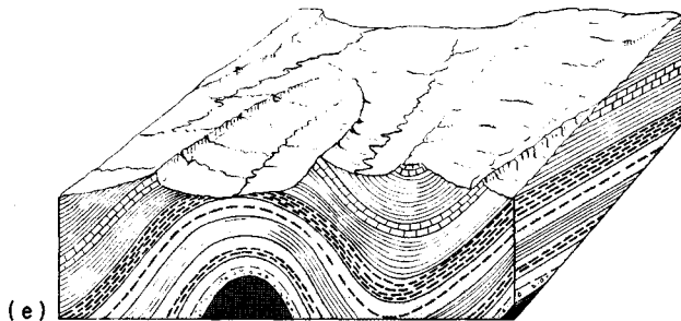
Fig. 8.10 Diagrams to illustrate plunge. (a) Upright plunging synform; (b) synform with nearly vertical plunge; (c) inclined plunging antiform; (d) antiform with nearly vertical plunge. (e) Block diagram, illustrating plunging folds, with hard beds forming topographical features on a denuded surface. Plunge shown on right hand section.
