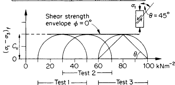
Fig. 9.21 Triaxial test results of the undrained shear strength of soil ( C_u ). Note: \theta = 45^\circ - \phi/2 and when \phi = 0 , \theta = 45^\circ . (\sigma_1 - \sigma_3)_f = difference in principal stresses at failure.
