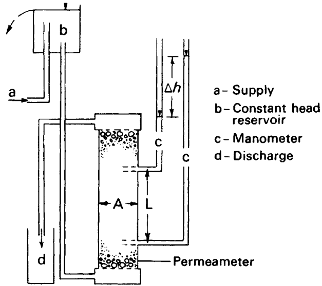
Fig. 11.11 A constant head permeameter for measuring the permeability of granular soils.
