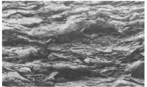
Fig. 6.13 Fissile shale viewed with an electron microscope ( \times 1000 ).
