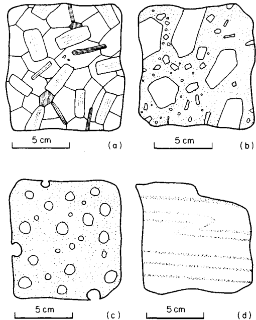
Fig. 5.16 (a) Equigranular texture. (b) Porphyritic texture. (c) Vesicular texture. (d) Flow-structure.
