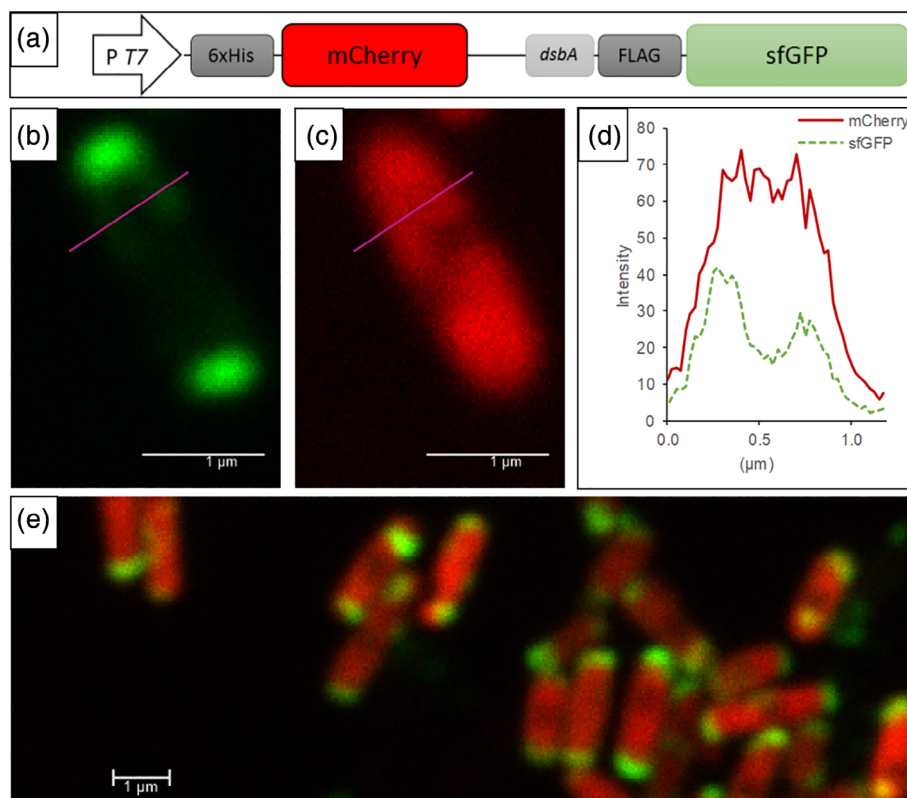
FIGURE 1 Expression system including cytoplasmic mCherry and periplasmic sfGFP (cyto-peri-FP system).
