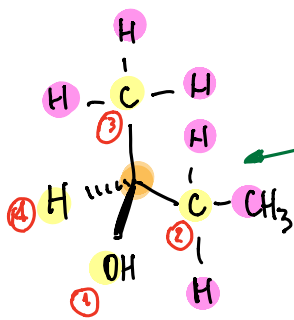
(S)-butan-2-ol
