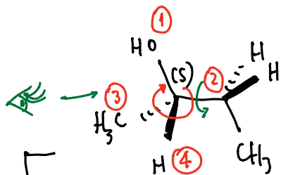
(S)-butan-2-ol
