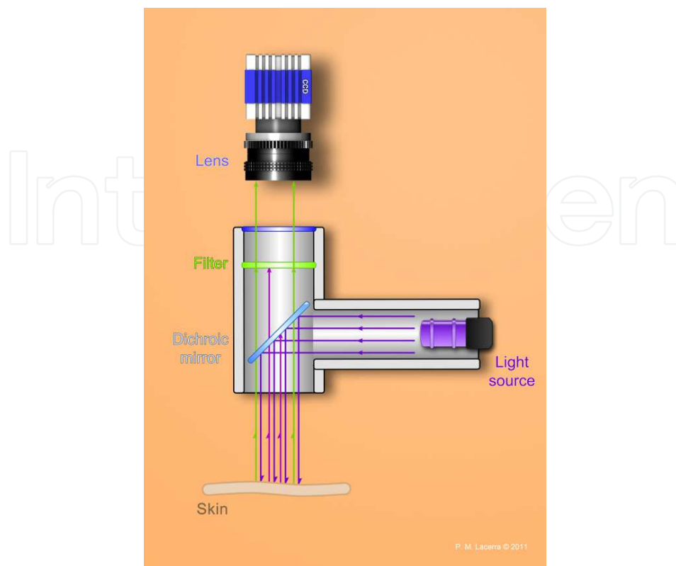
Fig. 4. Configuration of the fluorescence imaging device used.
