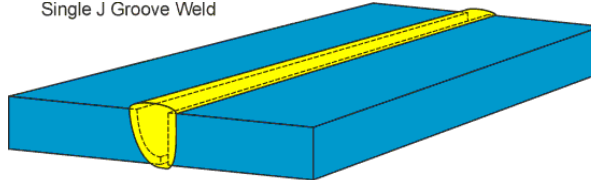
Single J Groove Weld
