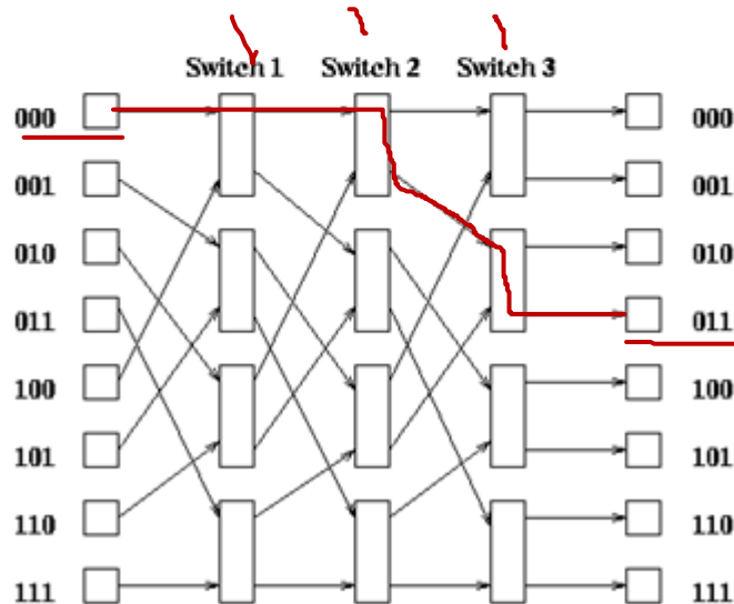
Omega network on 8 processors
