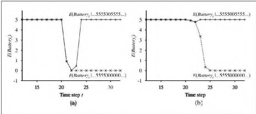
Figure 15.14 (a) (b) Upper curves: trajectory of the expected value of Battery_t for an observation sequence consisting of all Ss except for Os at t = 21 and t = 22 , using a simple Gaussian error model. Lower curves: trajectory with the observation remains at 0 from t = 21 onwards. (b) The same experiment run with the transient failure model. Notice that the transient failure is handled well, but the persistent failure results in excessive pessimism about the battery charge.
