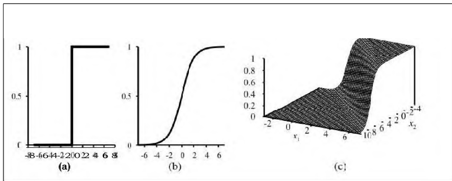
Figure 18.17 (a) The hard threshold function Threshold(z) with 0/1 output. Note that the function is nondifferentiable at z = c . (b) The logistic function, Logistic(z) = \frac{1}{1+e^{-z}} also known as the sigmoid function. (c) Plot of a logistic regression hypothesis h_{\mathbf{w}}(\mathbf{x}) = Logistic(\mathbf{w} \cdot \mathbf{x}) for the data shown in Figure 18.15(b).
