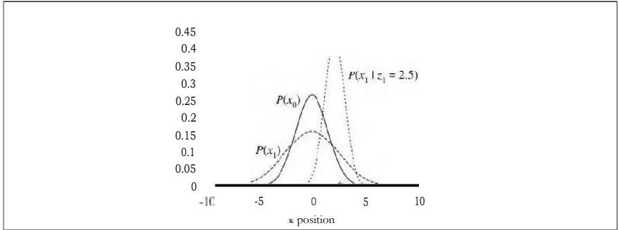
Figure 15.10 Stages in the Kalman filter update cycle for a random walk with a prior given by \mu_0 = 0.0 and \sigma_0 = 1.0 , transition noise given by \sigma = 2.0 , sensor noise given by \sigma_z = 1.0 , and a first observation z_1 = 2.5 (marked on the z-axis). Notice how the prediction P(x_1) is flattened out, relative to P(x_0) , by the transition noise. Notice also that the mean of the posterior distribution P(x_1 | z_1) is slightly to the left of the observation z_1 because the mean is a weighted average of the prediction and the observation.
