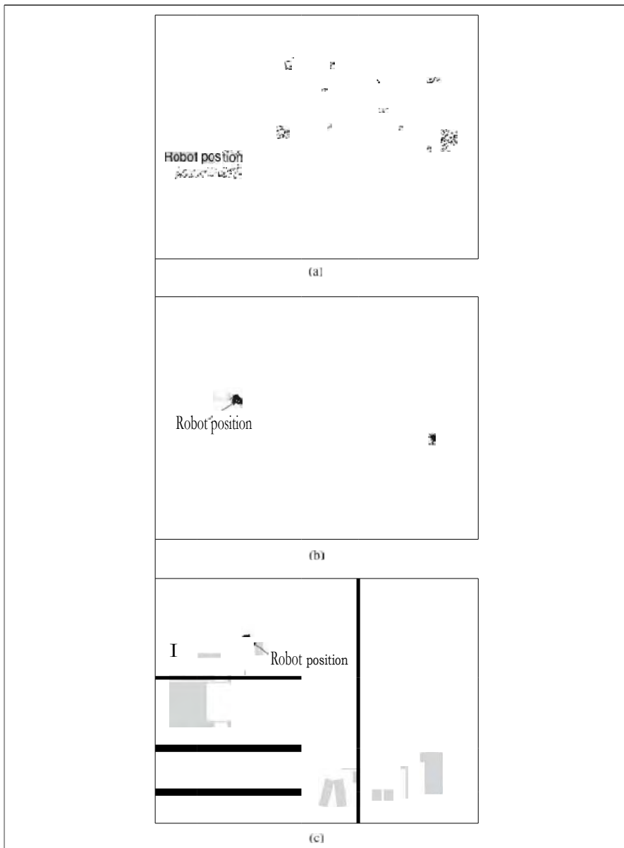
Figure 25.10 Monte Carlo localization , a particle filtering algorithm for mobile robot localization. (a) Initial, global uncertainty, (b) Approximately bimodal uncertainty after navigating in the (symmetric) corridor. (c) Unimodal uncertainty after entering a room and finding it to be distinctive.
