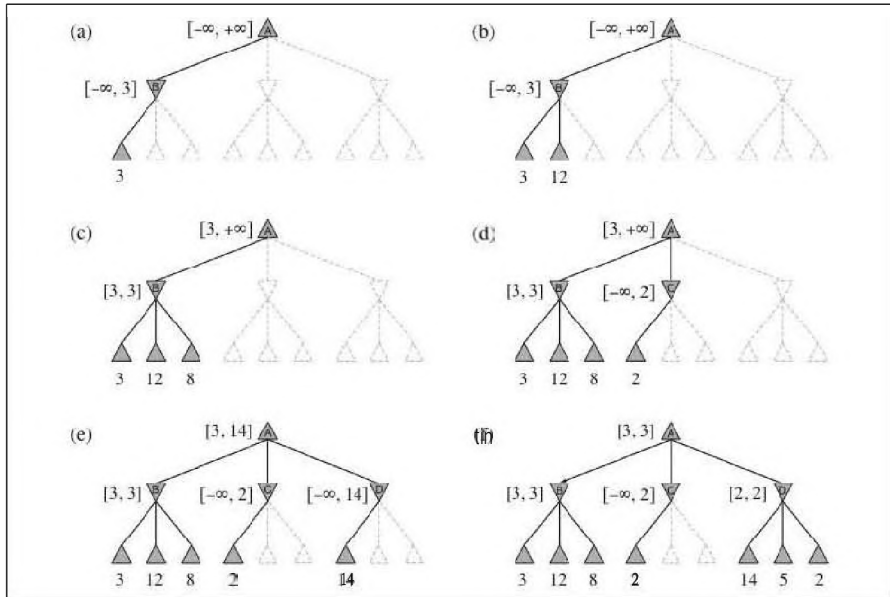
Figure 5.5 Stages in the calculation of the optimal decision for the game tree in Figure 5.2. At each point, we show the range of possible values for each node. (a) The first leaf he low has the value 3. Hence, B , which is a MIN node, has a value of at most 3. (b) The second leaf below B has a value of 12; MIN would avoid this move, so the value of B is still at most 3. (c) The third leaf below B has a value of 8; we have seen all B 's successor states, so the value of B is exactly 3. Now, we can infer that the value of the root is at least 3, because MAX has a choice worth 3 at the root. (d) The first leaf below C has the value 2. Hence, C , which is a MIN node, has a value of at most 2. But we know that B is worth 3, so MAX would never choose C . Therefore, there is no point in looking at the other successor states of C . This is an example of alpha–beta pruning. (e) The first leaf below D has the value 14, so B is worth at most 14. This is still higher than MAX's best alternative (i.e., 3), so we need to keep exploring D 's successor states. Notice also that we now have bounds on all of the successors of the root, so the root's value is also at most 14. (f) The second successor of D is worth 5, so again we need to keep exploring. The third successor is worth 2, so now D is worth exactly 2. MAX's decision at the root is to move to B , giving a value of 3.
