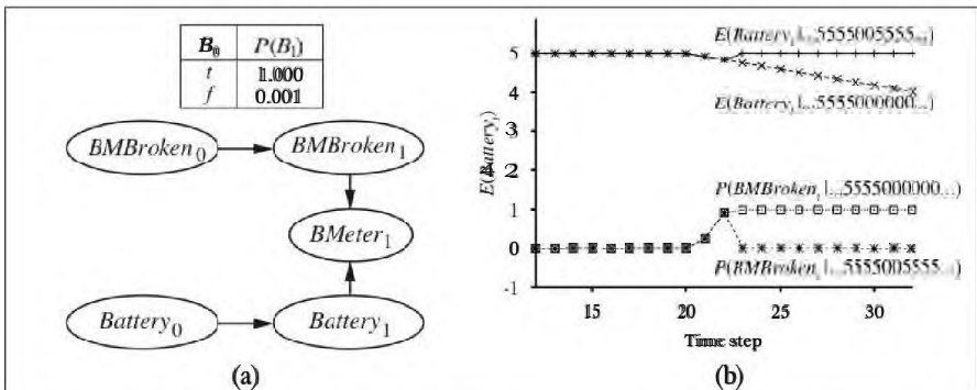
Figure 15.15 (a) A DEDB diagram showing the sensor status variable required for modeling persistent failure of the battery sensor. (b) Upper curves: trajectories of the expected value of Battery_t for the "transient failure" and "permanent failure" observations sequences. Lower curves: probability trajectories for BMBroken given the two observation sequences.
