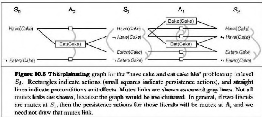
Figure 10.7 The "have cake and eat cake too" problem.
