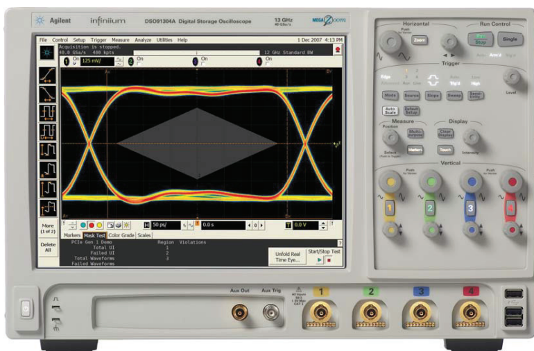
Figure 15. Agilent Infiniium 90000A Series oscilloscope
