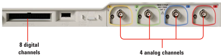
Figure 13. Front panel inputs for the four analog channels and eight digital channels on a mixed-signal oscilloscope
