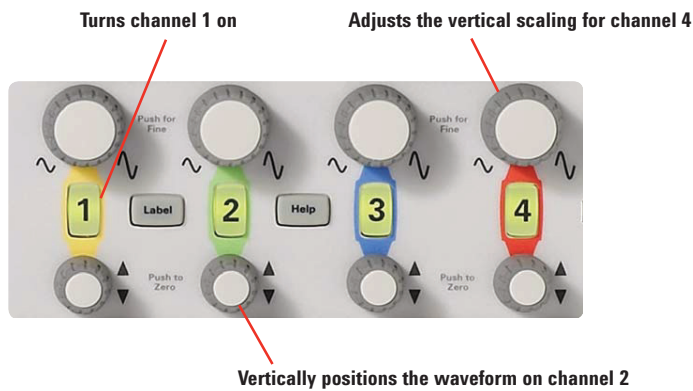
Figure 16. Front panel vertical control section on an Agilent InfiniiVision 2000 X-Series oscilloscope
