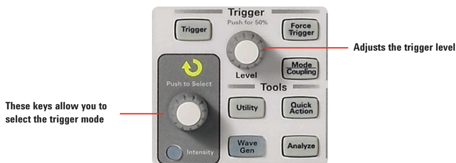
Figure 20. Front panel trigger control section on an Agilent InfiniiVision 2000 X-Series oscilloscope
