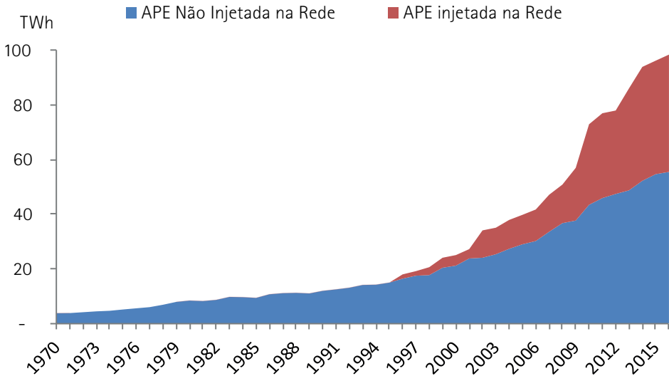
Chart 5.3 - Self Producers Power Plants - APE
