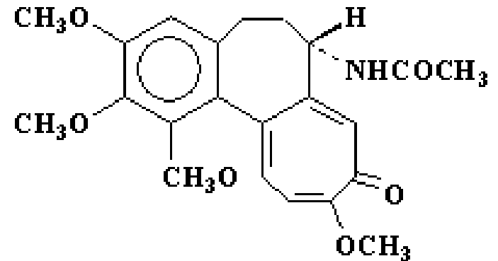
Colchicine C_{22}H_{25}NO_6
