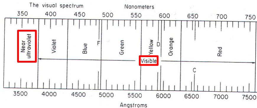
FIGURE 29-5 The visible spectrum.
