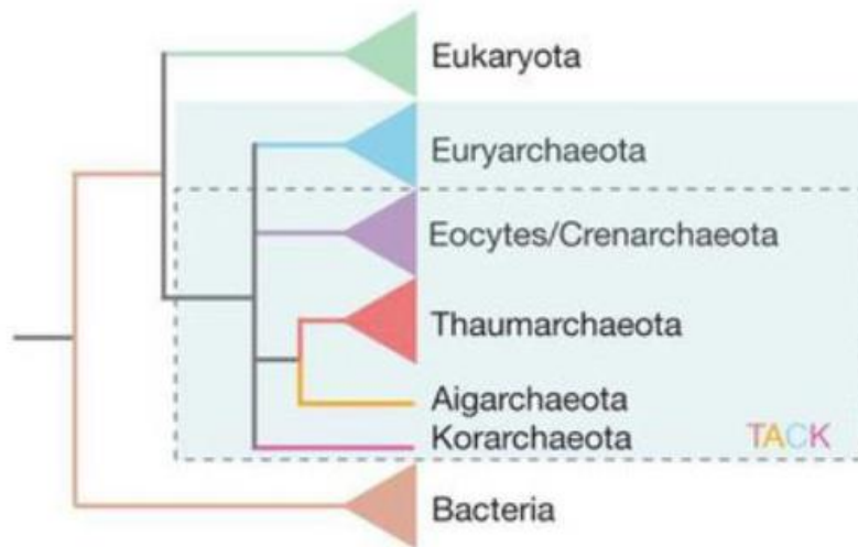
Three-domains hypothesis
