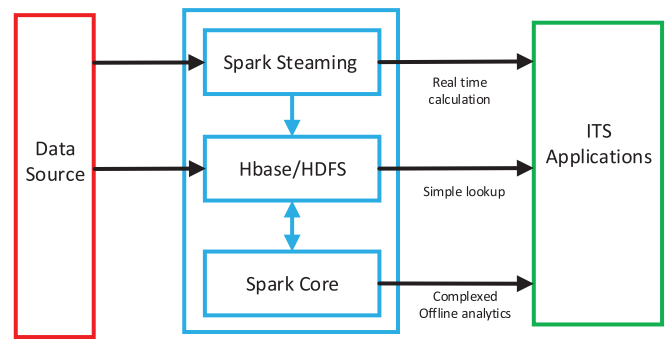
Fig. 6. A typical framework of using Apache Spark platform in ITS.
