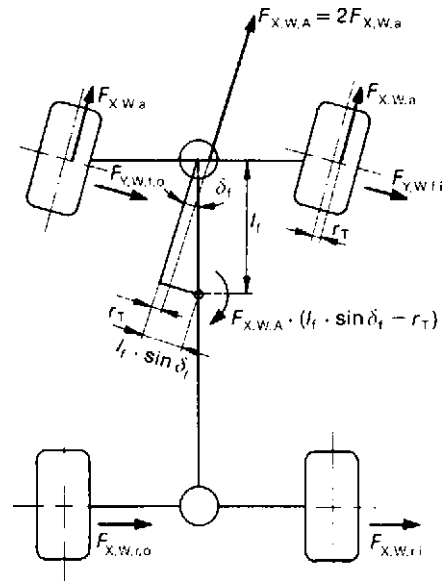
Fig. 10.1-54 With front-wheel drive, an oversteering yawing moment is produced, because the resultant tractive force vector is applied about lever arm l_f \times \sin \delta_f displaced to the centre of gravity of the vehicle.
