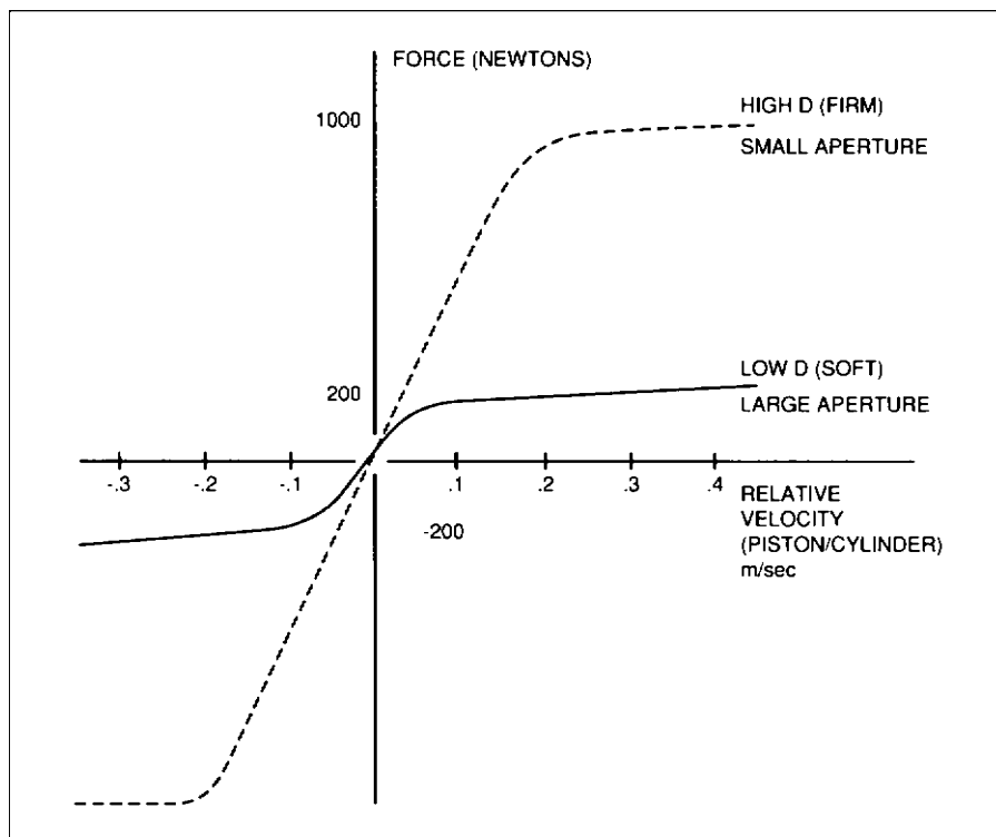
Fig. 13.1-21 Force versus relative velocity of a solenoid-switched aperture shock absorber.
