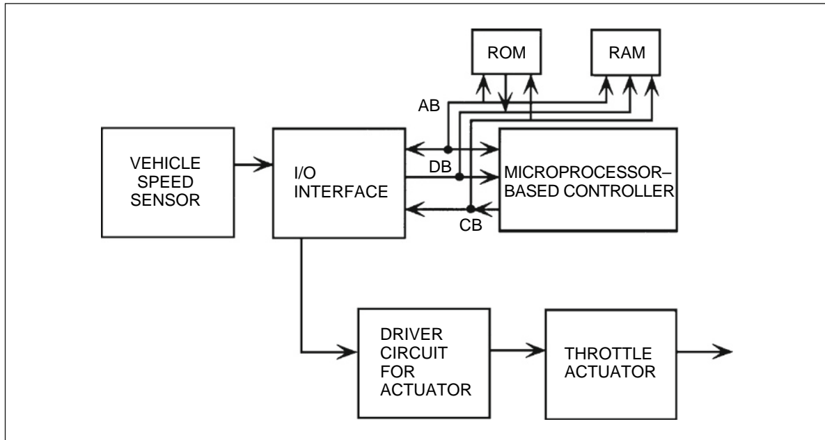
Fig. 13.1-8 Digital cruise control configuration.
