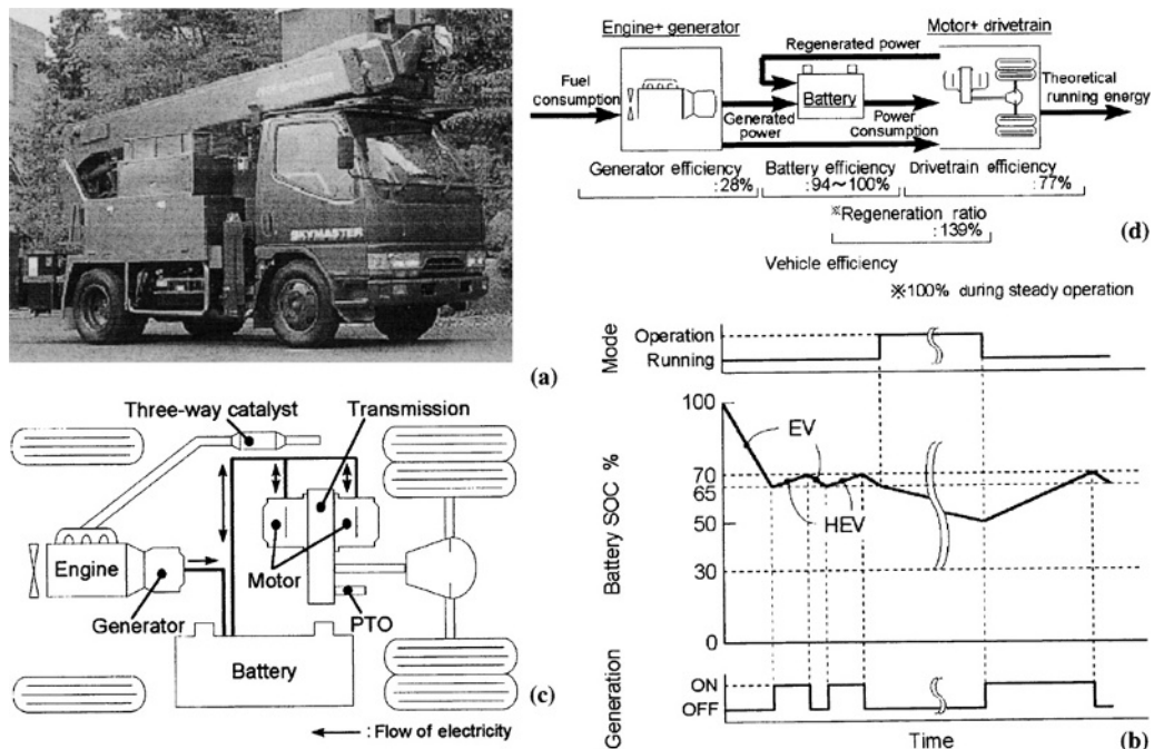
Fig. 7.1-21 Mitsubishi Canter-based hybrid municipal truck: (a) Complete package; (b) hybrid drive; (c) operating modes; (d) unit efficiencies.
