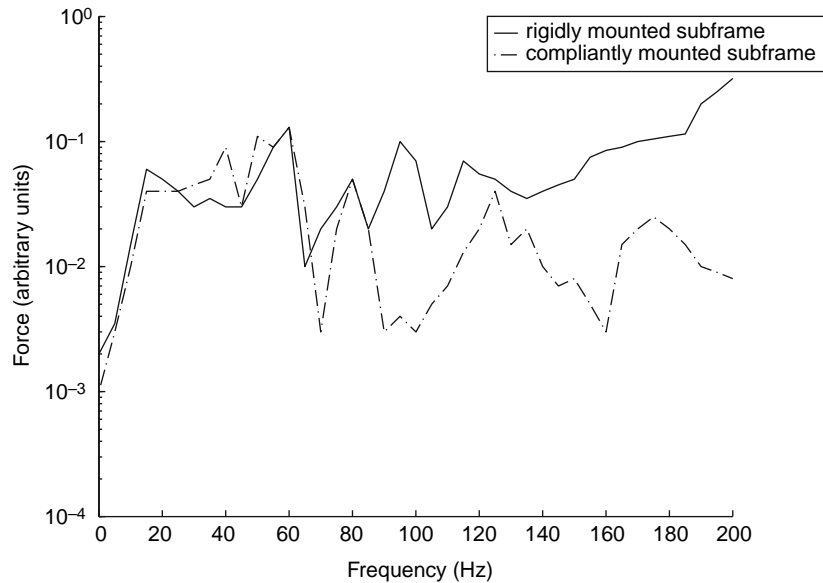
Fig. 21.1-7 The beneficial effects of the compliant subframe: data taken from Hardy (1997).
