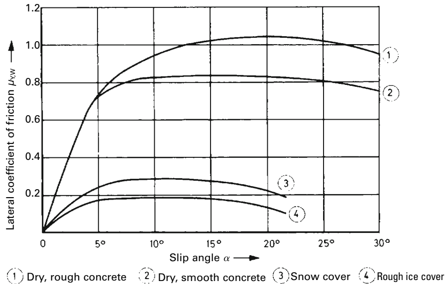
Fig. 10.1-43 Lateral coefficients of friction \mu_{Y,W} as a function of slip angle and road condition, shown for an '82 series' summer tyre with around 90% deep profile. The ice temperature is around -4^\circ\text{C} . The vertical force F_{Z,W} was kept constant during the measurements to obtain the dimensionless values of \mu_{Y,W} . The maximum at \alpha = 20^\circ on a very skid-resistant road can be seen clearly. The further \mu_{Y,W} sinks, the further it moves towards smaller angles.
