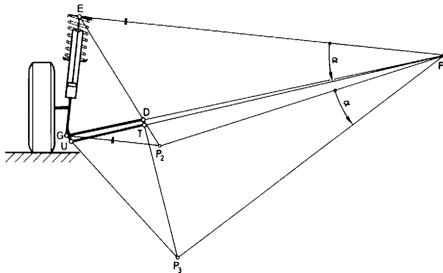
Fig. 9.1-48 The tie rod can also lie under the control arm when the steering arm points inwards.
