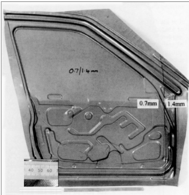
Fig. 18.1-40 Tailer welded door inner blank showing thicker frontal area allowing deletion of separate reinforcement panel. 17
