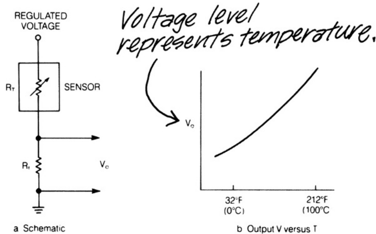
Fig. 23.1-12 Coolant temperature sensor.
