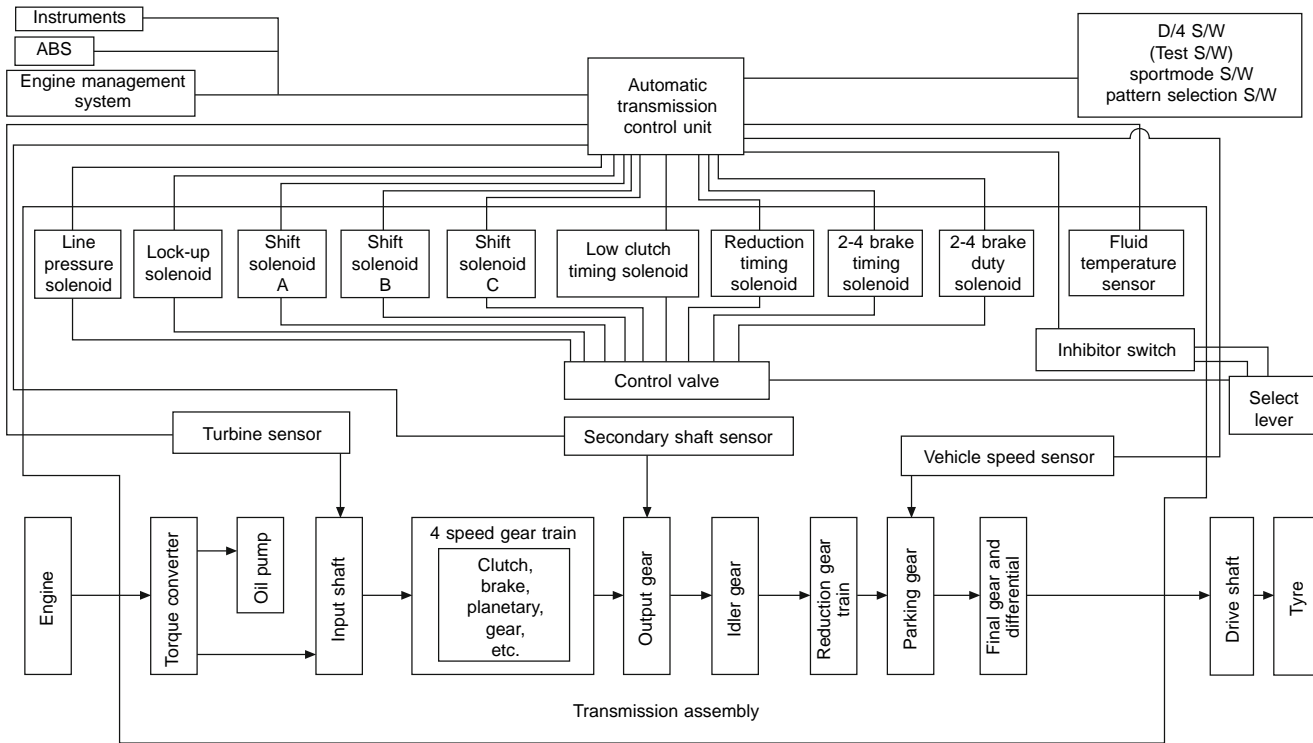
Fig. 5.1-24 Control block diagram (courtesy of Jatco).
