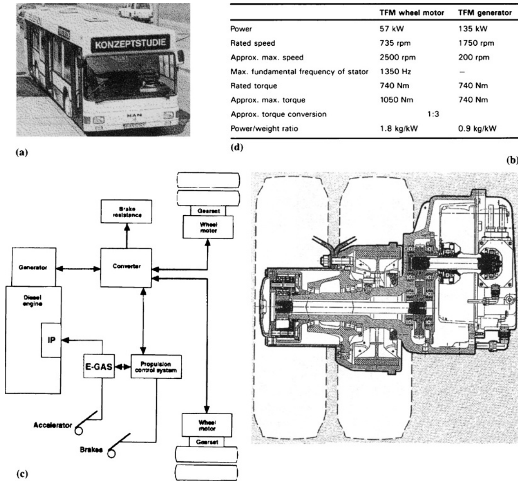
Fig. 7.1-20 MAN/Voith concept city bus: (a) low floor package; (b) wheel motor; (c) controller; (d) drive characteristics.
