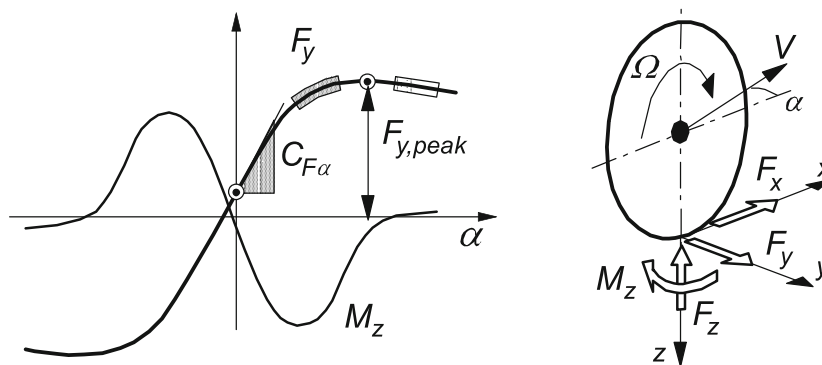
Fig. 11.1-1 Characteristic shape factors (indicated by points and shaded areas) of tyre or axle characteristics that may influence vehicle handling and stability properties. Slip angle and force and moment positive directions.
