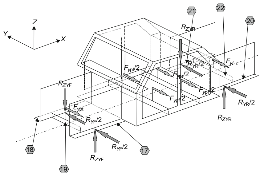
Fig. 16.2-23 Baseline model – lateral loading with additional SSSs.
