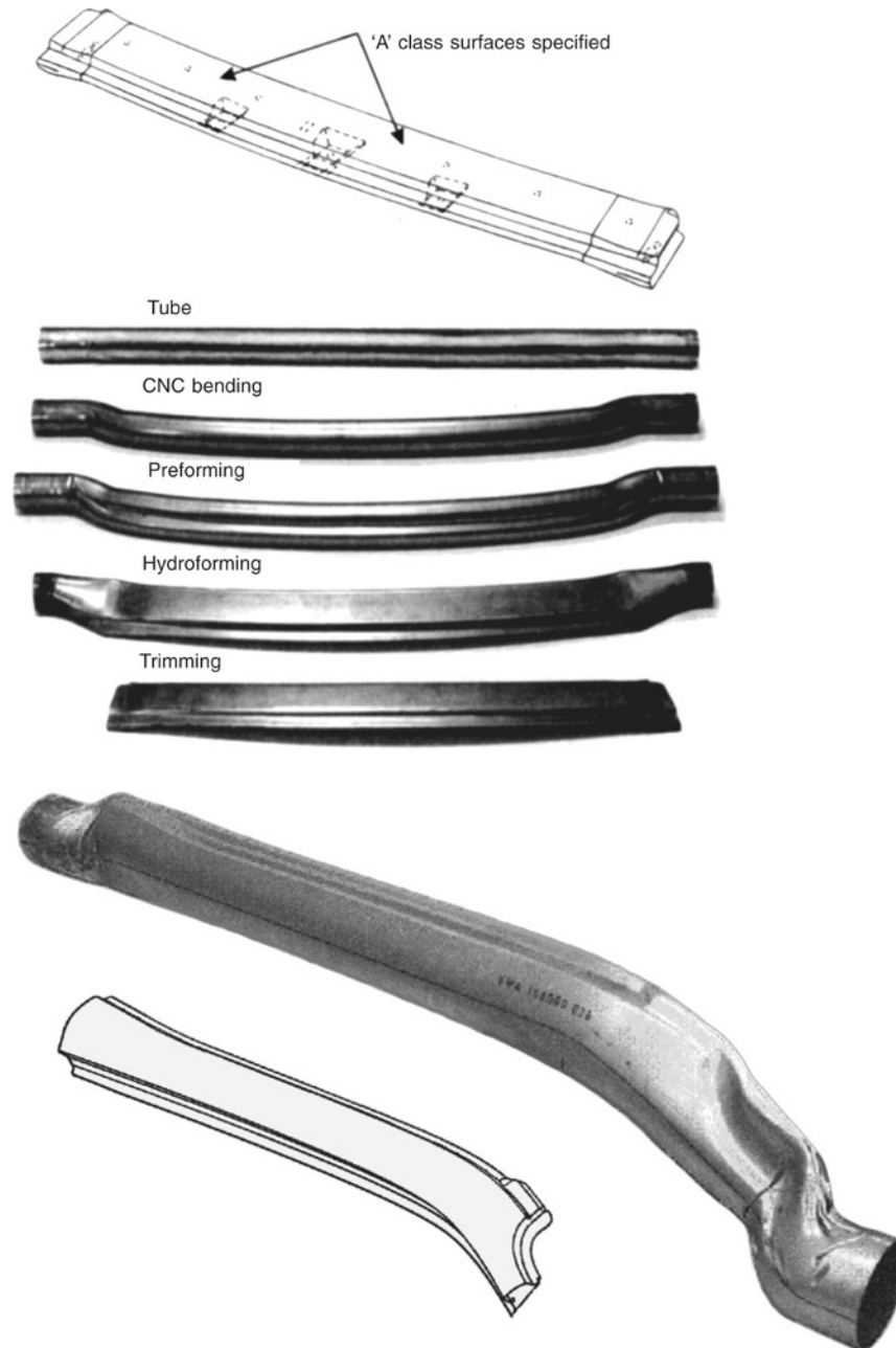
Fig. 18.1-38 Stages in component manufacture by tube hydroforming. 16
