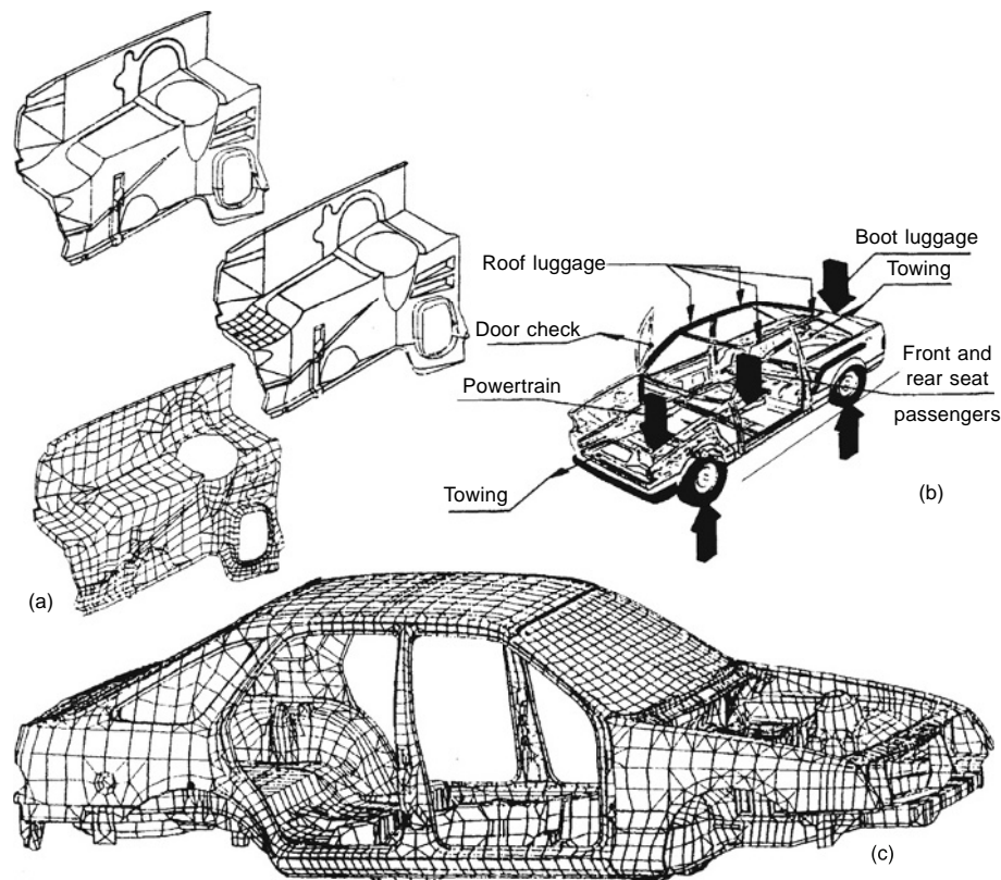
Fig. 18.1-7 FEA of Ford car: (a) steps in producing FEA model; (b) load inputs; (c) global model for body-in-white (BIW).
