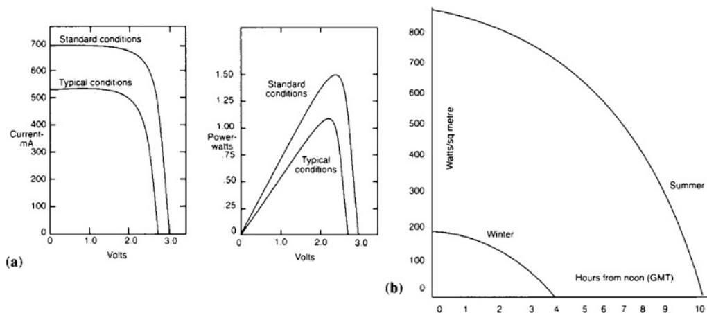
Fig. 6.1-5 Solar cell technology: (a) cell characteristics; (b) solar energy variation.
