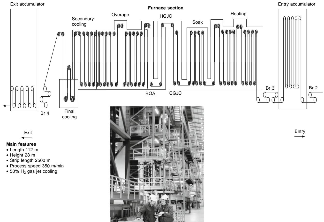
Fig. 18.2-2 (b) Alternative continuous annealing line. (Courtesy of Corus.)
