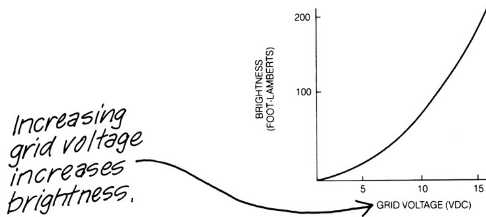
Fig. 23.1-19 Brightness control range for vacuum-fluorescent display.
