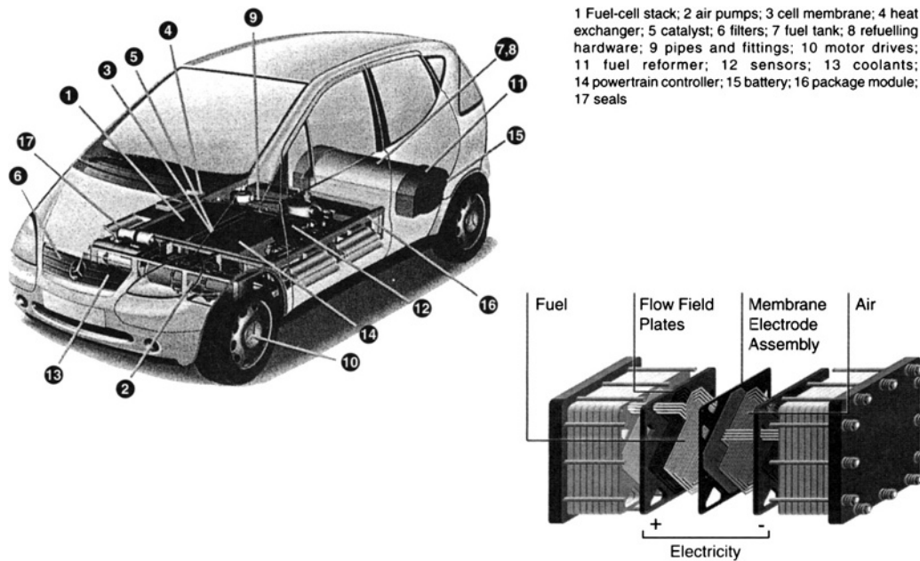
Fig. 6.1-26 D-C Nocar and Ballard PEM fuel cell.
