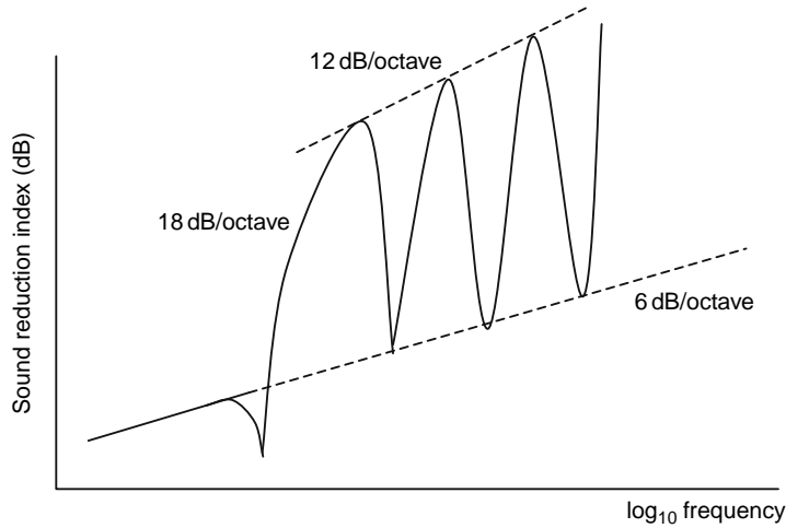
Fig. 21.1-20 Generalised TL curves: after Fahy (1985).
