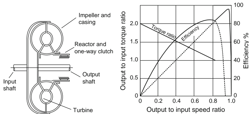
Fig. 5.1-19 Torque converter and characteristics.
