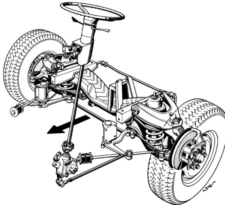
Fig. 8.1-7 Front axle on the VW light commercial vehicle Lt 28 to 35 with an opposed steering square. A cross-member serves as a subframe and is screwed to the frame from below. Springs, bump/rebound-travel stops, shock absorbers and both pairs of control arms are supported at this force centre. Only the anti-roll bar, steering gear, idler arm and the tie-rods of the lower control arms are fastened to the longitudinal members of the frame. The rods have longitudinally elastic rubber bushings at the front that absorb the dynamic rolling hardness of the radial tyres and reduce lift on uneven road surfaces.
