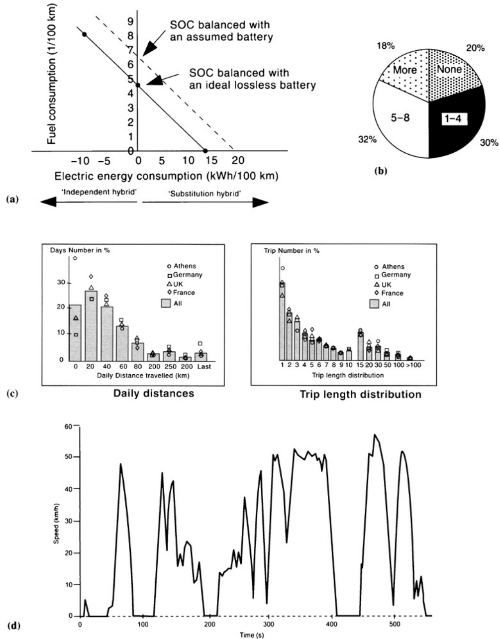
Fig. 7.1-2 HYZEM research programme: (a) characterizing a hybrid powertrain; (b) use of vehicle per day; (c) daily distances and trip lengths; (d) synthetic urban drive cycle.
