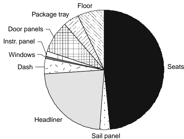
Fig. 21.1-9 The absorption of sound by vehicle interior trim: data taken from Qian and Vanbuskirk (1995).
