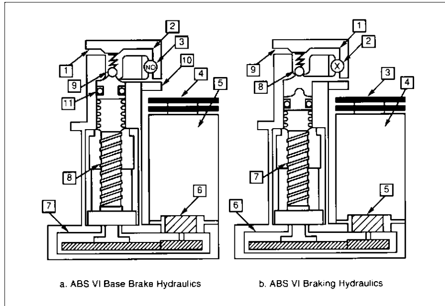
Fig. 13.1-16 Brake pressure modulating mechanism.
