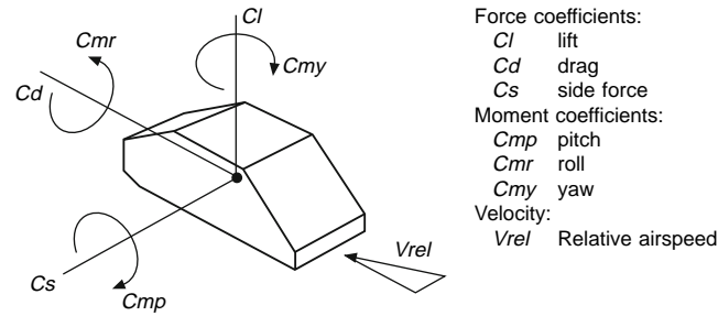
Fig. 19.1-1 Lift, drag, side force and moment axes.
