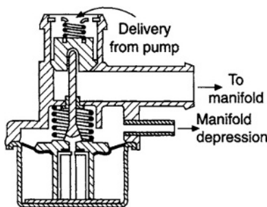
Fig. 3.1-8 AC-Delco gulp valve, for admitting extra air to the induction tract when the throttle is suddenly closed.
