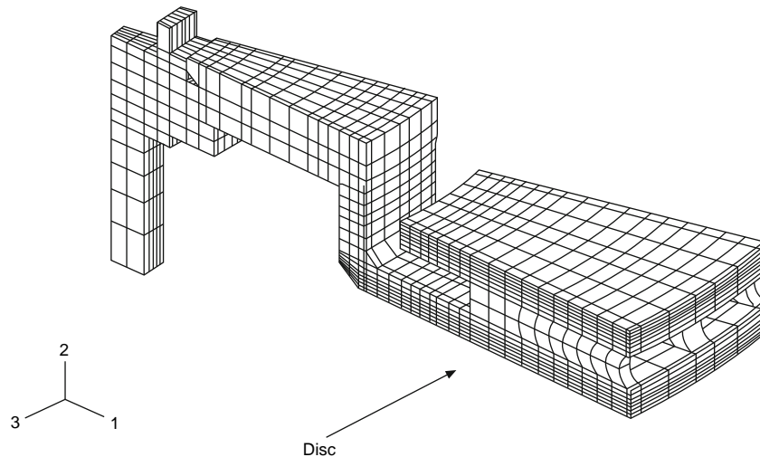
Figure 12.1-23 Finite element model of 10° segment of vented disc and hub.
