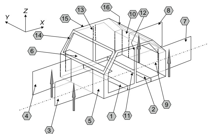
Fig. 16.2-1 Baseline model.
