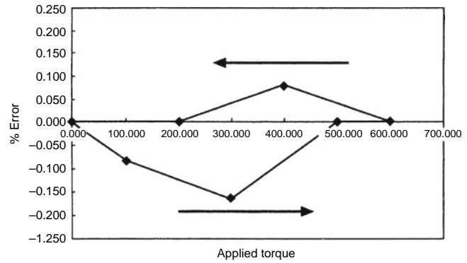
Fig. 2.1-7 Dynamometer calibration error as percentage of full scale.
