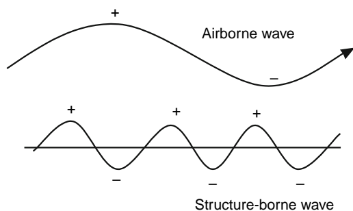
Fig. 21.1-18 Strong coupling between the airborne and structure-borne waves occurs around the coincidence frequency.
