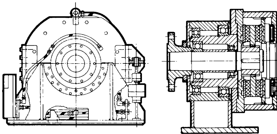
Fig. 2.1-12 Water-cooled friction brake used as a dynamometer.
