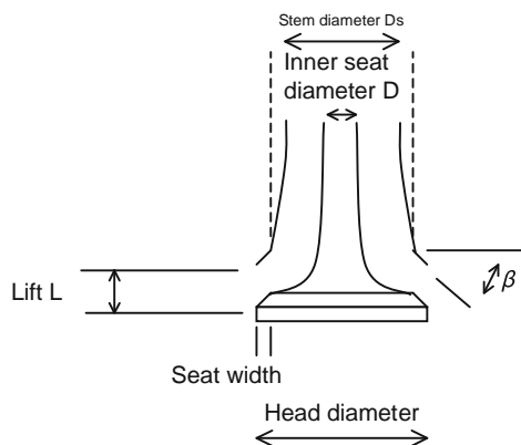
Fig. 22.1-A1 Valve geometry.
