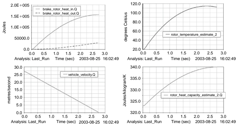
Fig. 15.1-29 Output from the brake temperature model shown in Table 15.1-1 during a 60 mph–0 stop.
