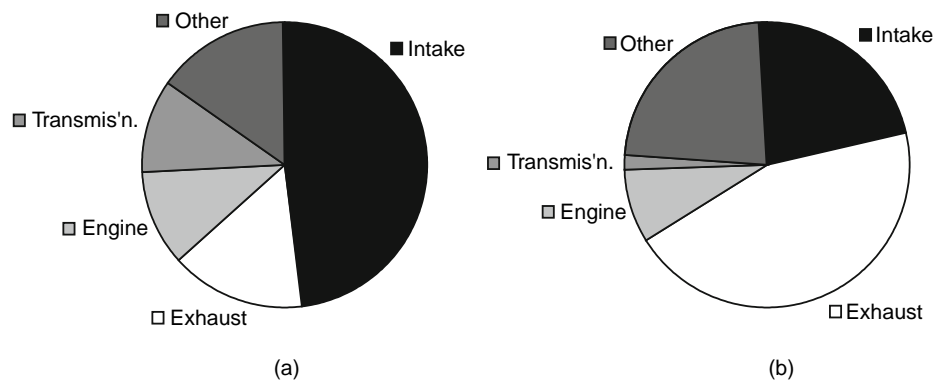
Fig. 22.1-2 Noise source ranking results adapted from Balcombe and Crowther (1993). (a) Results at the start of the pass-by test. (b) Results at the end of the pass-by test.
