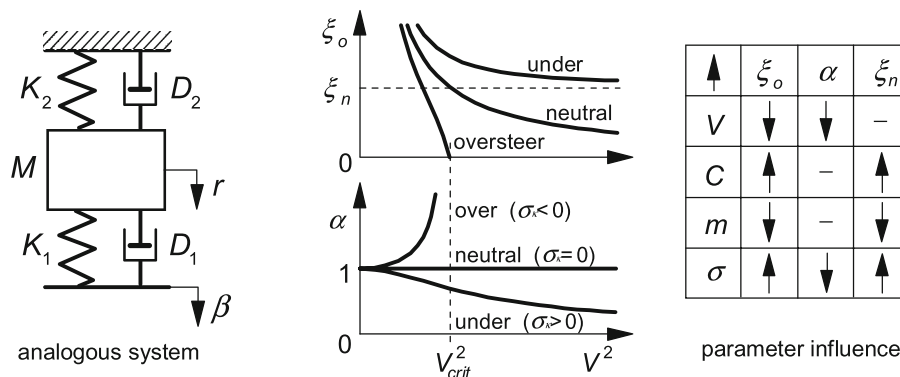
Fig. 11.1-13 The influence of parameters on natural frequency and damping.
