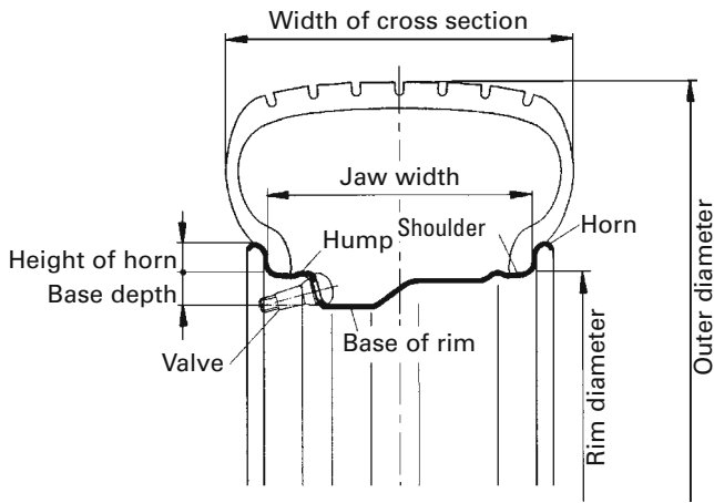
Fig. 10.1-20 Series 55 wide tyre designs, mounted on a double hump rim with the inflating valve shown in Fig. 10.1-6. The actual rim consists of the following:
