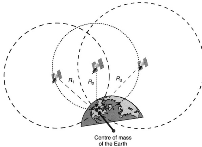
Fig. 14.1-2 3-Dimensional trilateration of GPS satellites.
