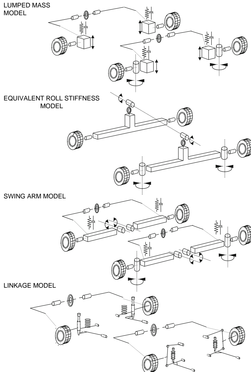
Fig. 15.1-52 Modelling of suspension systems
