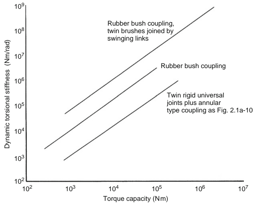
Fig. 2.1a-11 Ranges of torsional stiffness for different types of rubber coupling.
