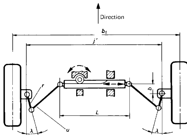
Fig. 9.1-40 The steering is in front of the wheel centre and the triangular linkage behind it, with the inner joints fixed to the ends of the steering rack.
