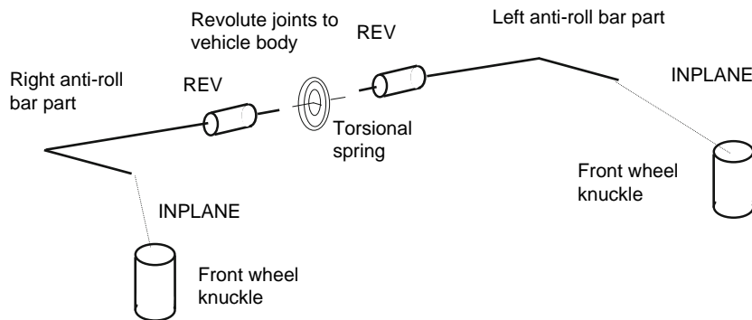
Fig. 15.1-16 Modelling the anti-roll bars using joint primitives.
