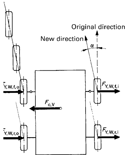
Fig. 10.1-37 Tyres are only able to transfer a lateral force F_{Y,V} acting on the vehicle if they are rolling at an angle to the vehicle. Regardless of whether these are F_{Y,V} or the centrifugal force F_{C,Y} during cornering, the lateral forces F_{Y,W} should be regarded as being perpendicular to the wheel centre plane.
