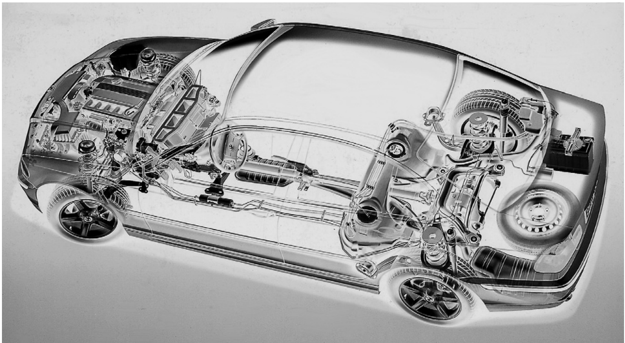
Fig. 8.1-32 Front-mounted engine, rear-mounted drive (BMW 3 series E46, 1998). The manual transmission is flange-mounted on the engine, which is longitudinally positioned over the front axle. The rear-axle differential is driven by means of a propshaft. The fuel tank is situated in front of the rear axle for safety in case of an accident. The battery was placed in the boot in order to achieve a balanced 50:50 axle-load distribution. Fig. 8.1-1 shows the rear axle in detail.
