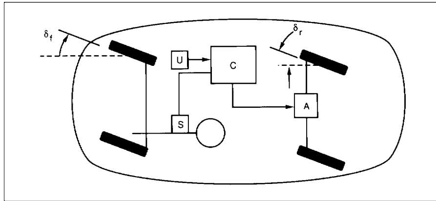
Fig. 13.1-23 4WS Configuration.
