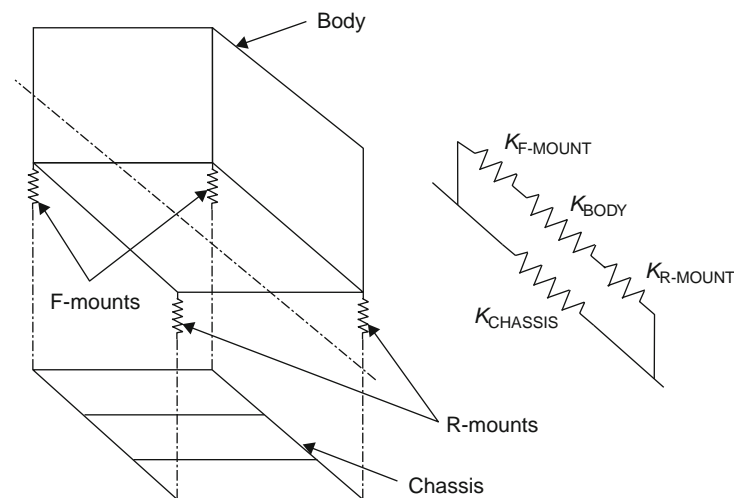
Fig. 16.1-9 Body and body mounts in series in torsion.
