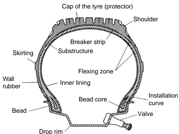
Fig. 10.1-1 Design of a diagonal ply tubeless car tyre with a normal drop rim and pressed-in inflating valve (see also Fig. 10.1-6).
