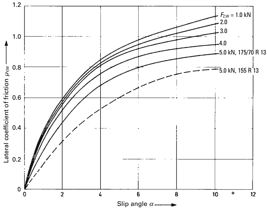
Fig. 10.1-45 Lateral coefficients of friction \mu_{y,w} as a function of the slip angle \alpha and the vertical force F_{z,w} , measured on a dry drum on a 175/70 R 13 82 S tyre at p_T = 2.0 bar. The tyre, which has been inflated in such a manner, carries 395 kg or F_{z,w} = 3.87 kN. In order to indicate the influence of the cross section on the transferable lateral forces the 82 series 155 R 13 78 S tyre was also included.
