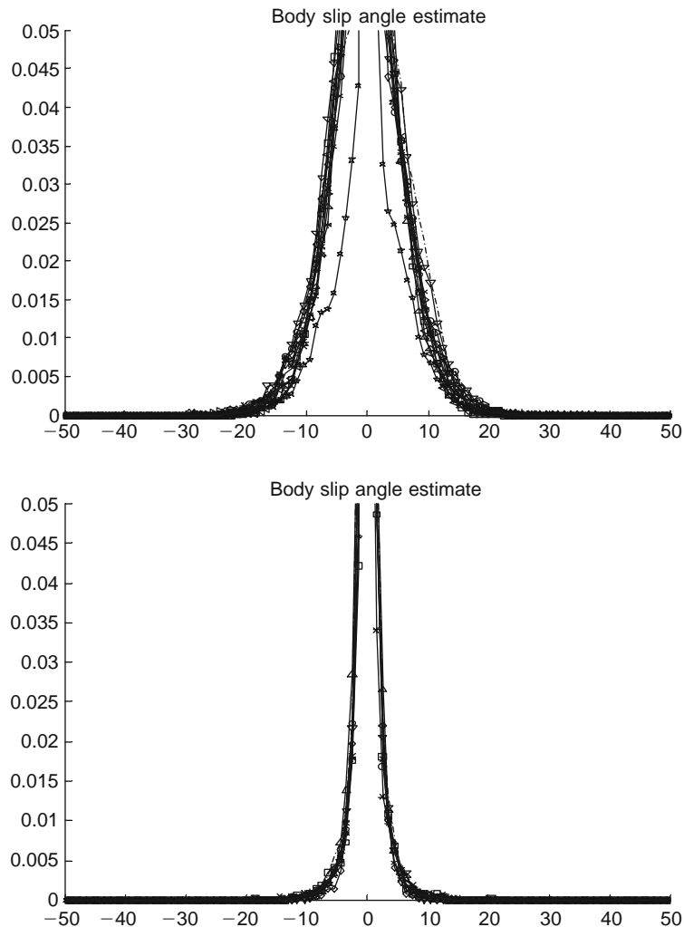
Fig. 15.1-46 Probability density for body slip angle estimates – Greece 2002 (top) and Germany 2002 (bottom) for Petter Solberg, Subaru World Rally Team.
