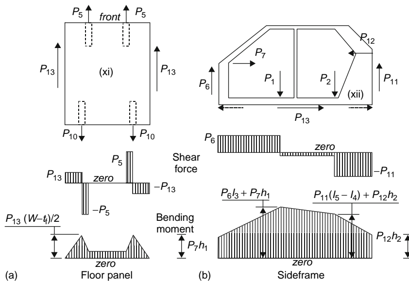
Fig. 16.2-7 Shear force and bending moment diagrams.
