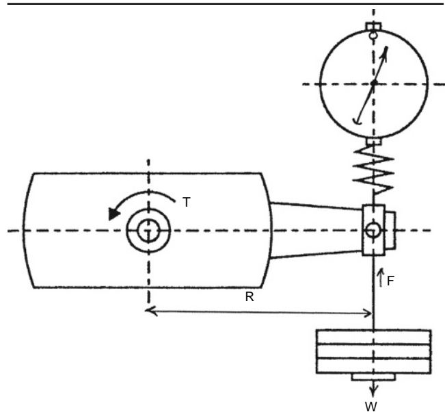
Fig. 2.1-1 Diagram of Froude type, trunnion-mounted, sluice-gate dynamometer measuring torque with dead weights and spring balance.
