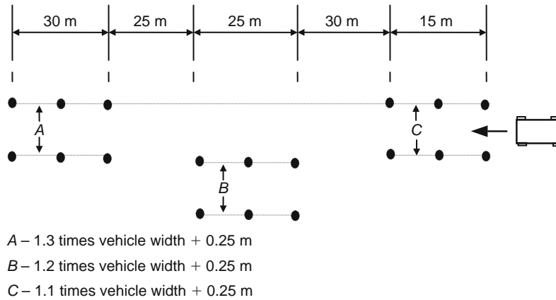
Fig. 15.1-49 Lane change test procedure. (This material has been reproduced from the Proceedings of the Institution of Mechanical Engineers, K2 Vol. 214 'The modelling and simulation of vehicle handling. Part 4: handling simulation', M.V. Blundell, page 74, by permission of the Council of the Institution of Mechanical Engineers.)
