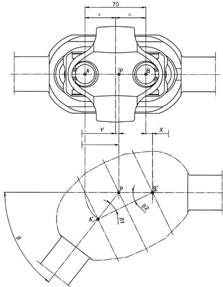
Fig. 8.1-4 Top view of the dual joint (Fig. 8.1-3). The wheel end of the axle is turned about point P in the middle of the steering pivot during steering. The individual joints are constrained at points A and B so that point A is displaced to position A', P is displaced to P' and B is displaced along the drive axle by the distance X to B'. In order to assimilate the variable bending angle \beta resulting from the longitudinal displacement of point B, the mid-point of the joint P is displaced by the distance Y. The adjustment value Y depends on the distance between the joints and the steering angle at which constant velocity is to exist. Where large steering angles can be reached (up to 60^\circ ), there should be constant velocity at the maximum steering angle. The adjustment value Y and the longitudinal displacement X should be taken into consideration in the design of the axle.
