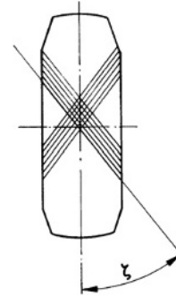
Fig. 10.1-2 The diagonal ply tyre has crossed-bias layers; the zenith angle \xi was 30–40° for passenger cars. The 4 PR design should have two layers in each direction. Smaller angles \xi can be found in racing cars. Rolling resistance, lateral and suspension stiffness are significantly determined by the zenith angle.
