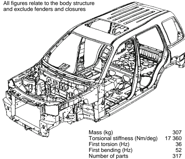
Fig. 18.1-3 Land Rover Freelander with monocoque body and plastic front wings. (Reprinted with permission from SAE paper 1999-01-3181 Copyright 1999 Society of Automotive Engineers Inc.)
