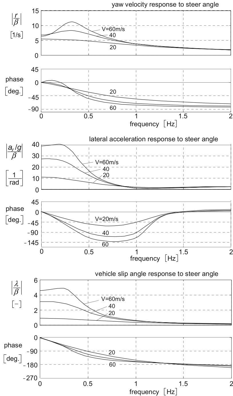
Fig. 11.1-15 Frequency response functions; vehicle parameters according to Table 11.1-1.
