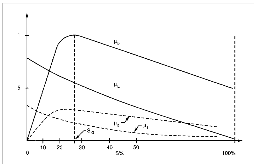
Fig. 13.1-14 Braking coefficients versus tire slip (solid curves for dry road, dashed curves for wet or icy road).
