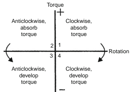
Fig. 2.1-8 Dynamometer operating quadrants.
