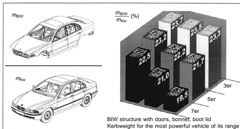
Fig. 18.1-14 Relationship of body-in-white weight to kerbweight. 6
