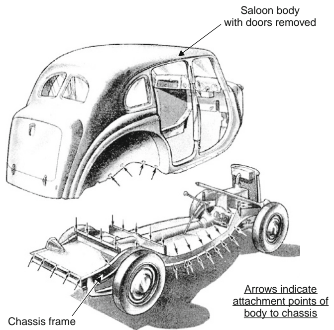
Fig. 16.1-12 Multiple attachments of body to frame.
