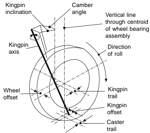
Fig. 17.1-17 Principal features of front steering geometry.
