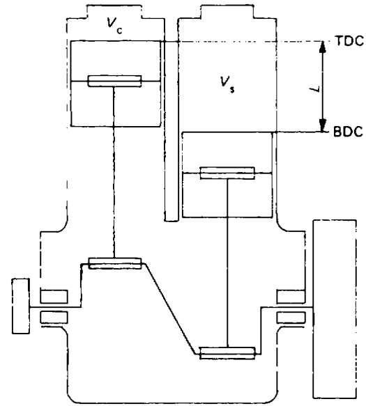
Fig. 1.1-12 Illustration of compression-ratio.
