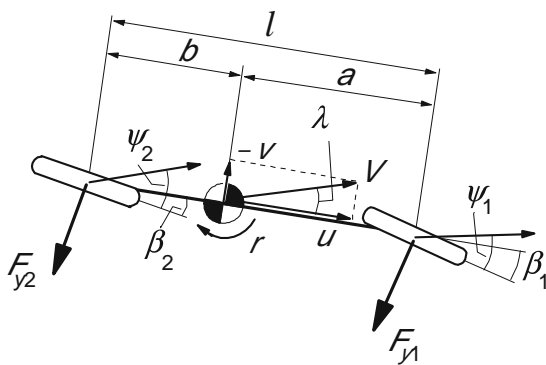
Fig. 11.1-16 ‘Four-wheel’ steering to make slip angle \beta = 0 (Exercise 11.1.2).
