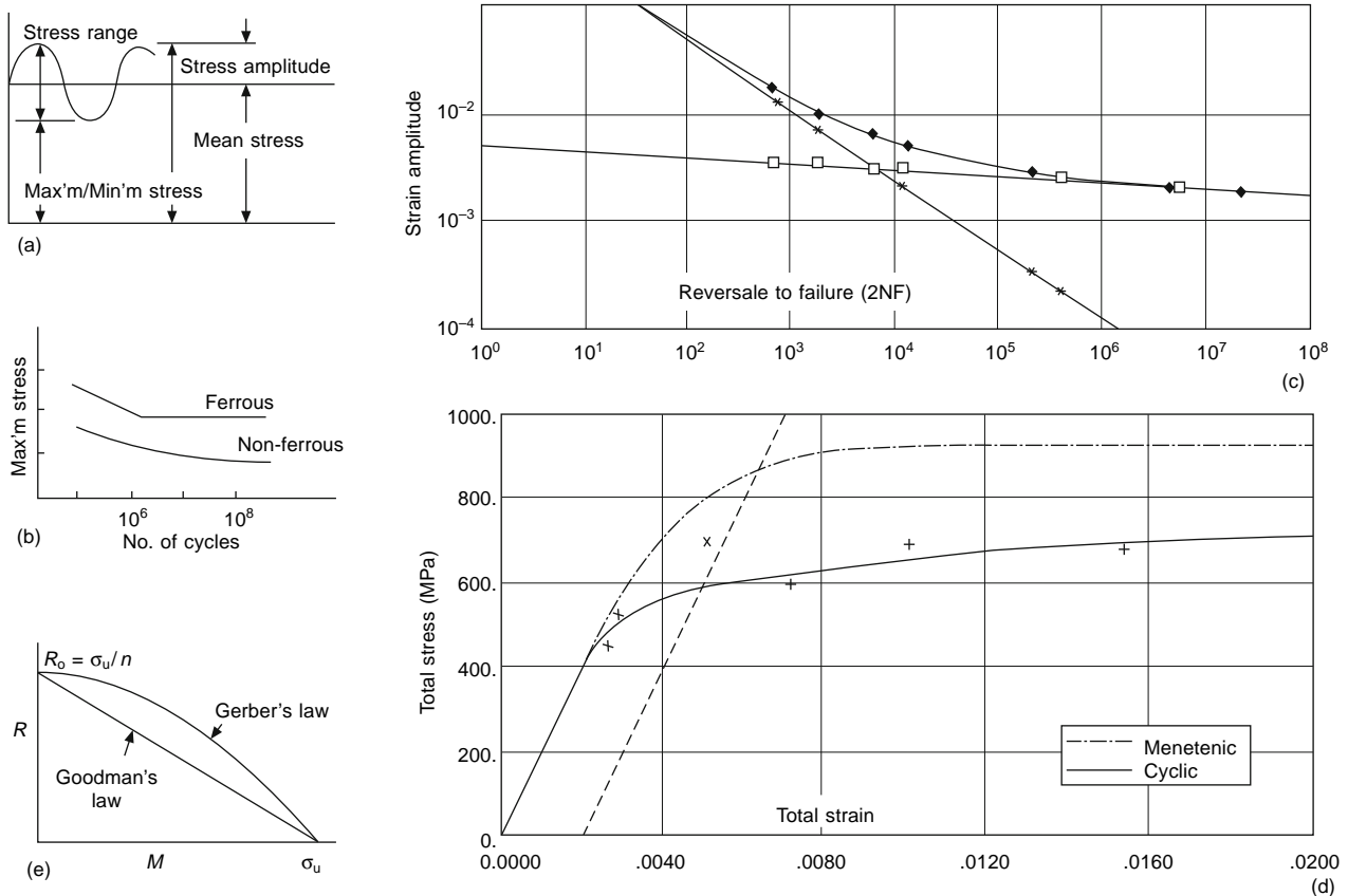
Fig. 18.1-21 Fatigue life evaluation: (a) terminology for cyclic stress; (b) S-N diagram; (c) strain/life curves; (d) dynamic stress/strain curves; (e) fatigue limit diagrams.
