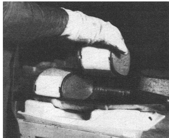
Fig. 3.1-4 Two monolithic catalyst carriers being assembled in series into their casing in the AC-Delco factory at Southampton.
