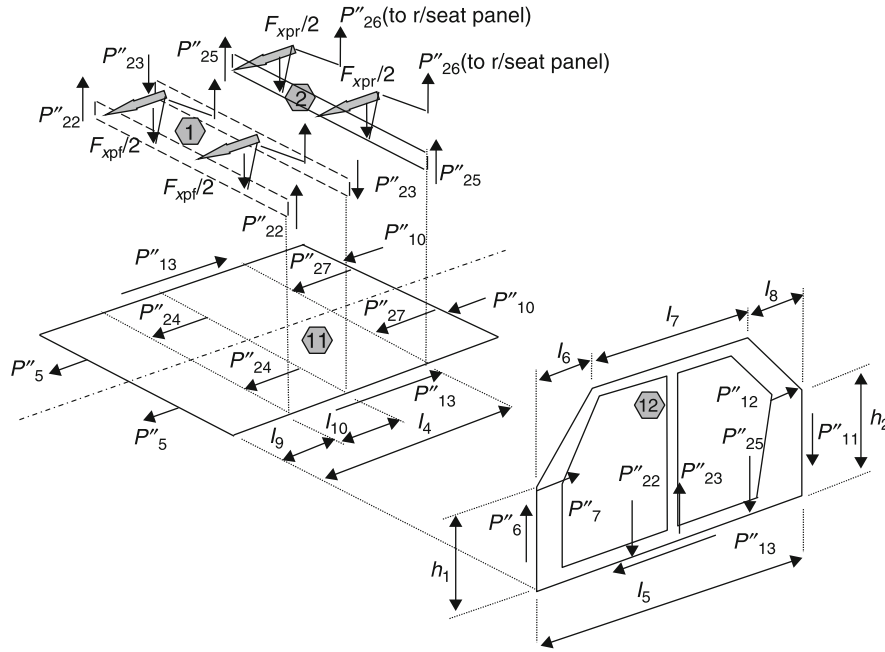
Fig. 16.2-33 Baseline model (floor, sideframe) – braking loads.
