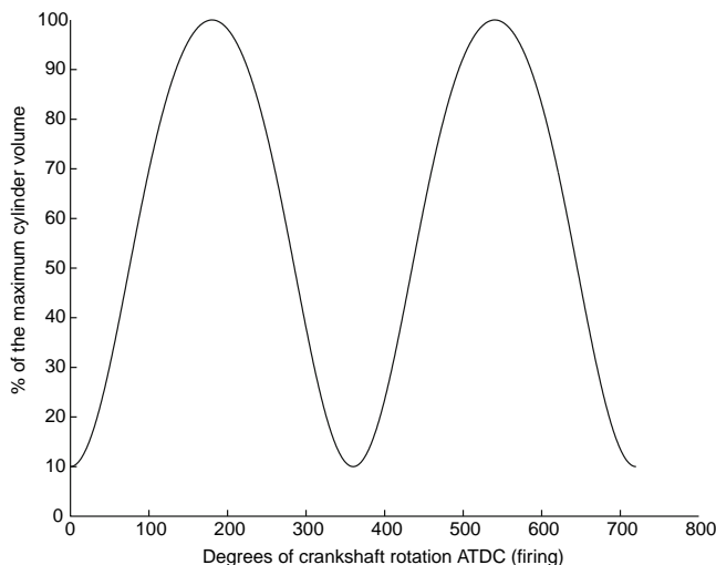
Fig. 22.1-10 Time history of the cylinder volume.
