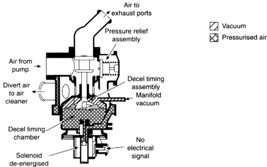
Fig. 3.1-14 The electrically actuated air-control valve, with solenoid energised.
