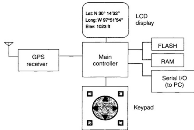
Fig. 14.1-9 Block diagram of basic handheld GPS device.
