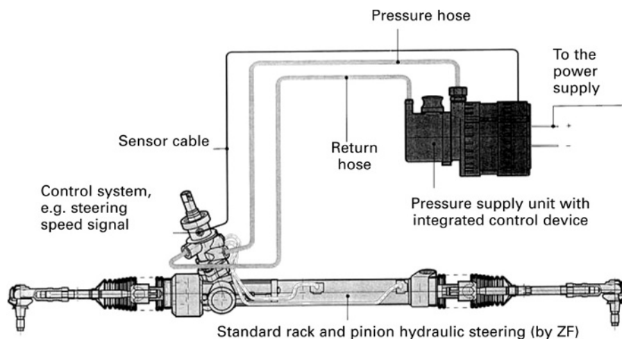
Fig. 9.1-19 Open-centre control system from ZF. The pressure supply unit designed as a modular unit can be fitted with different electric motors (DC motor with or without brushes) and pump fuel feed volumes ( 1.25\text{--}1.75\text{ cm}^3 per rpm) depending on its particular function. Oil tanks for horizontal or vertical installation are also available. Operating pressure is up to 120 bar, with a maximum power consumption of 80 A.
