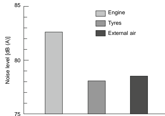
Fig. 19.1-9 Noise sources (Piatek, 1986).
