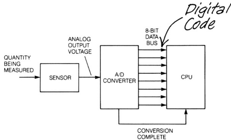
Fig. 23.1-3 Analog-to-digital conversion.
