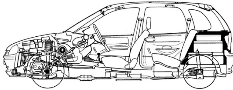
Fig. 8.1-49 Compact power train unit on the Vauxhall Corsa (1997). The engine is transverse mounted with the gearbox on the left. The McPherson front axle and safety steering column can be seen clearly.
