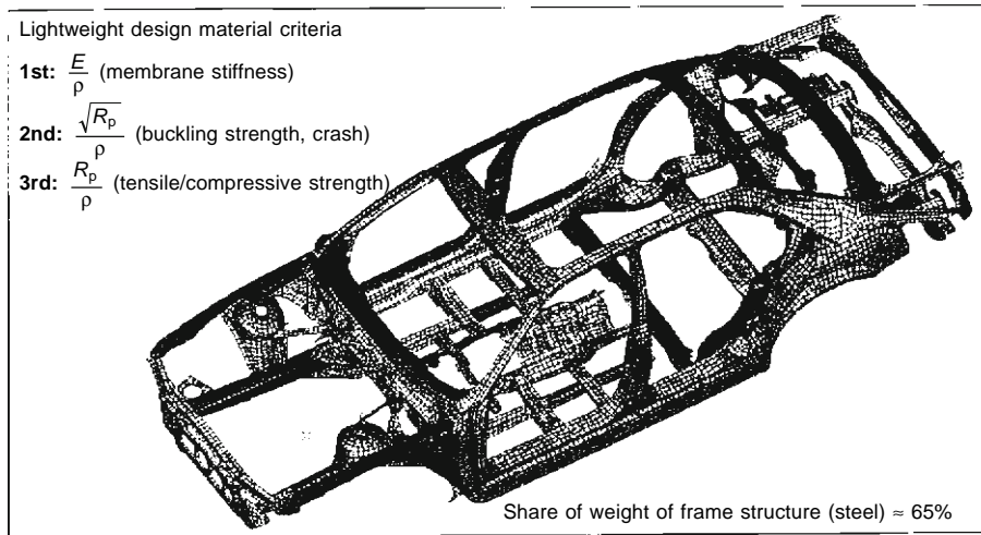
Fig. 18.1-17 Criteria used in the analysis of structural components by BMW. 6
