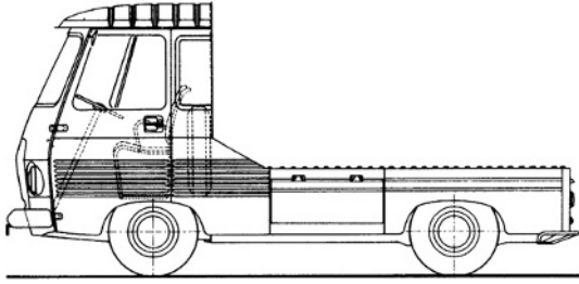
Fig. 8.1-47 The low cargo area on the Peugeot light commercial vehicle J 5/J 7 is achieved due to front-wheel drive and a semi-trailing link axle to the rear (similar to the one in Fig. 8.1-63).
