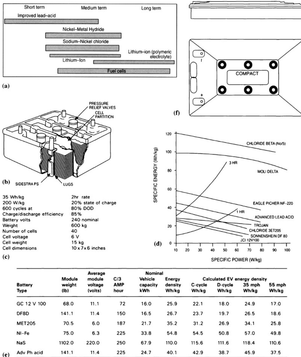
Fig. 6.1-1 The lead-acid battery: (a) development time spans compared; (b) high energy lead-acid battery; (c) parameters of H-E battery; (d) battery characteristics; (e) energy-storage comparisons.
