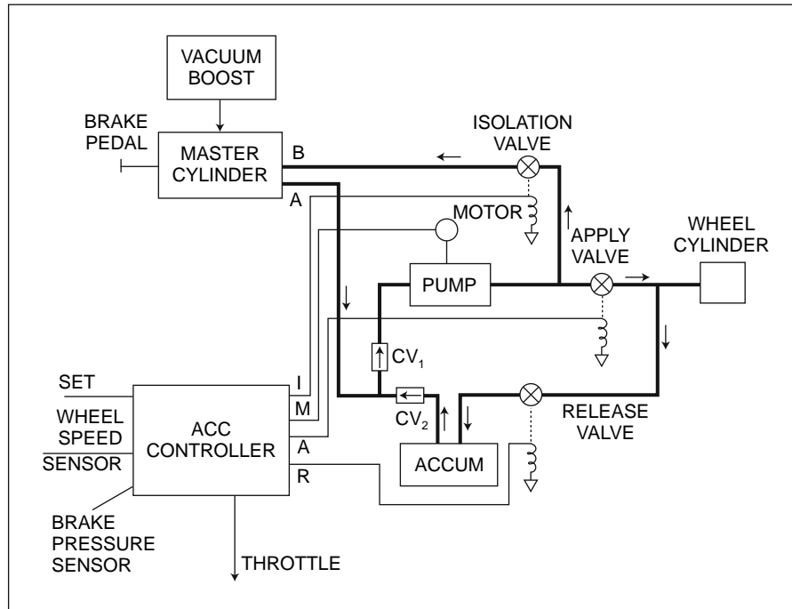
Fig. 13.1-11 ACC emphasizing the automatic braking portion.
