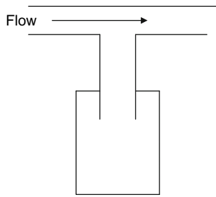
Fig. 22.1-34 The Helmholtz resonator.
