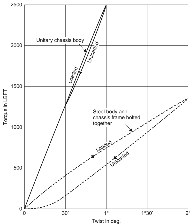
Fig. 16.1-22 Torsion stiffness tests, 1938 and 1939 (Swallow 1938 by permission Council of I.Mech.E.).
