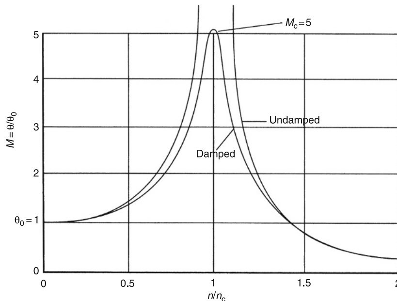
Fig. 2.1a-3 Relationship between frequency ratio, amplitude and dynamic amplifier M .
