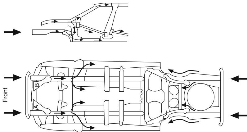
Fig. 17.1-15 Below: plan view of a Toyota frame designed to spread the loads imposed by front and rear end impacts uniformly throughout the structure. The combination of the front transverse member and the diagonal members, A and B, one on each side, triangulate the front end of the frame to constrain it to collapse concertina fashion, as shown in Fig. 17.1-13. Scrap view above: elevation of a different frame, showing how the loads are distributed as viewed in a vertical plane. The triangulation struts shown in this example are fitted in the door frames.
