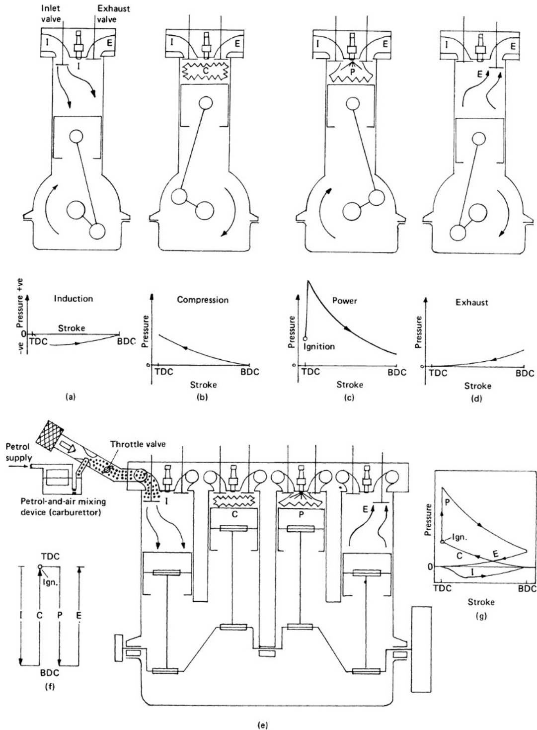
Fig. 1.1-3 Four-stroke-cycle petrol engine.
