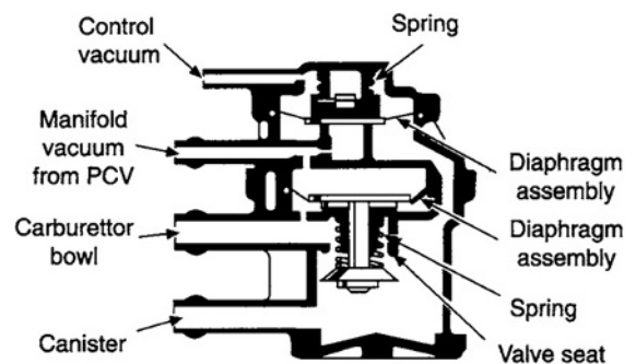
Fig. 3.1-18 Canister control valve type 2 performs the functions not only of the vapour vent valve but also of the purge valve as in Fig. 3.1-15.
