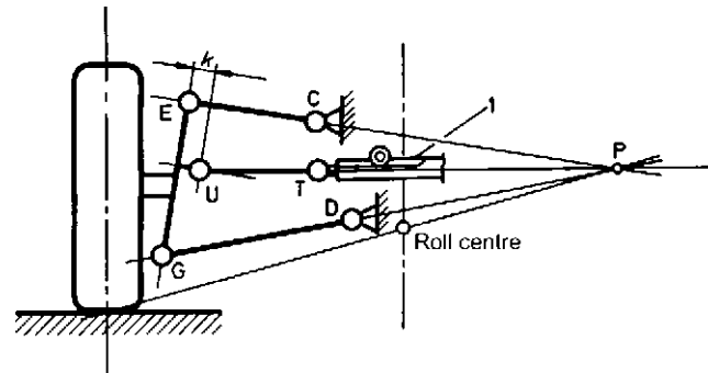
Fig. 9.1-35 Path and movement points necessary for determining the tie rod length and position. The position of the tie rods is given by the connecting line UP (to the pole). The illustration also shows the roll centre R_o .
