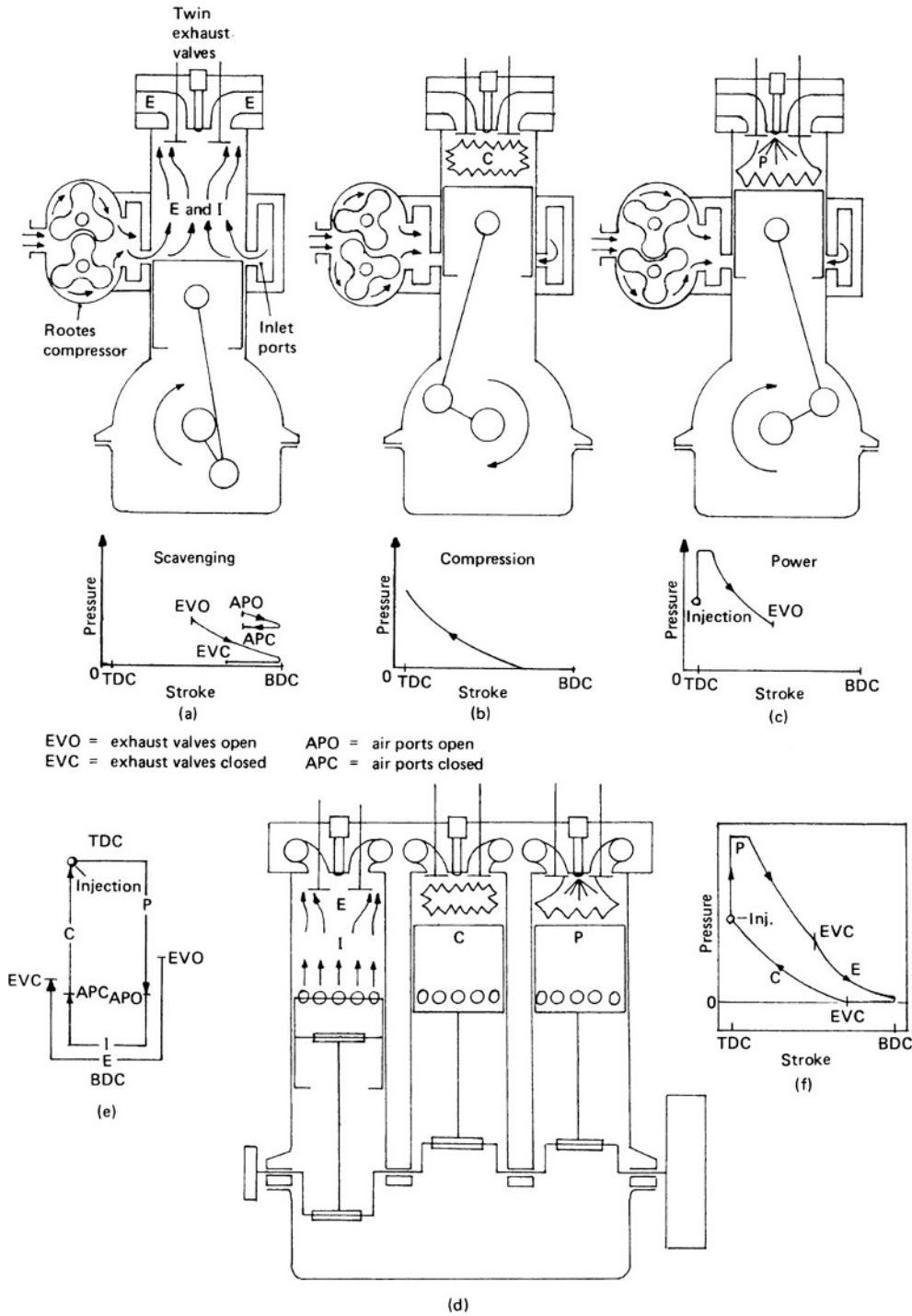
Fig. 1.1-9 Two-stroke-cycle diesel engine.
