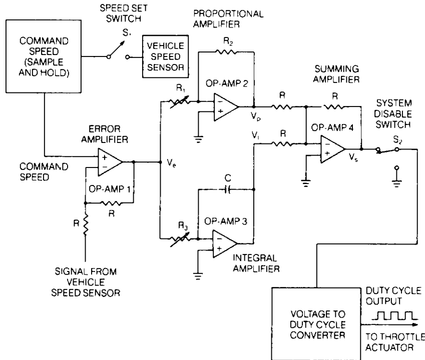
Fig. 13.1-10a Cruise control electronics (analog).
