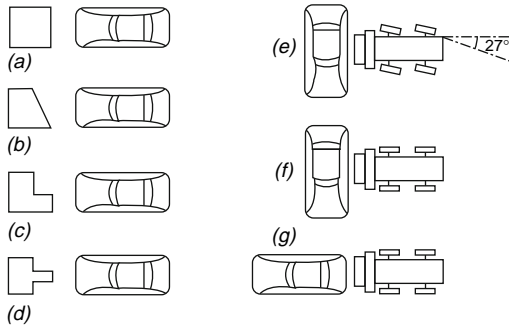
Fig. 17.1-7 Some of the tests done by manufacturers to ensure that the occupants of their vehicles will be, so far as is practicable, safe in the event of an accident. At (a) is the simple basic zero offset frontal impact, at (b) is a 30° offset, at (c) a 40% offset and at (d) a pole impact test. A side impact test for representing an impact between two vehicles moving along lines at right angles to each other is shown at (e) while, at (f), the vehicle that is struck is stationary. Finally, a rear end impact test is shown at (g).
