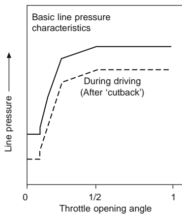
Fig. 5.1-25 Line pressure control strategy (courtesy of Jatco).
