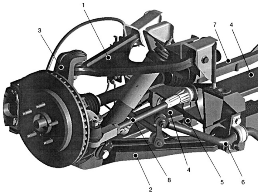
Fig. 8.1-34 Rear axle (left side of wheel) of the Chevrolet Corvette (1998). Links 1, 2 and wheel carrier 3 of the multi-link suspension are made from aluminium in order to reduce the unsprung masses. The plastic leaf spring 4 is mounted at two places on the right and left sides of the body (5) so that it also helps to make the body more resistant to roll. Roll spring stiffness is further increased by stabilizer 6. This is attached to subframe 7, which is also made of aluminium. The design of the wheel carrier 3 on the front and rear axles is the same, but not the wheel links 1 and 2. The toe-in control of the rear axle is exercised very stiffly and precisely, via tie rod 8.
