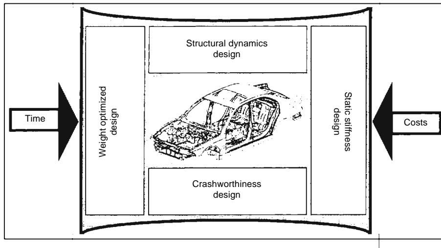
Fig. 18.1-8 Critical areas for body design (after Ludke 6 ).
