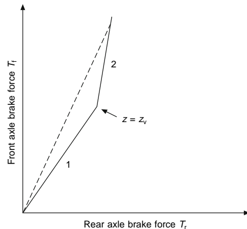
Figure 12.1-20 Typical modulating valve brake force distribution.
