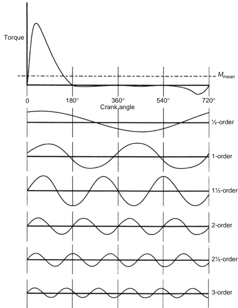
Fig. 2.1a-4 Harmonic components of turning moment, single cylinder four-stroke gasoline engine.
