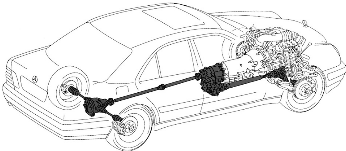
Fig. 8.1-78 Drive train of the four-wheel-drive Mercedes-Benz E class 4MATIC (from 1997). In order to be able to control the drive shafts to the front wheels, an integrated spring-and-shock absorber strut in the shape of a fork on the lower transverse link is used. In the almost identical suspension design of other than off-road varieties, the springs and shock absorbers are separate.
