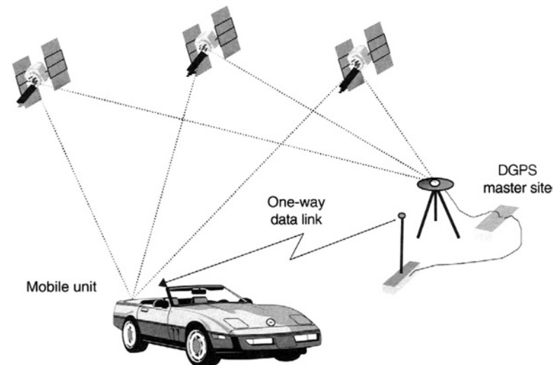
Fig. 14.1-3 Differential GPS positioning.
