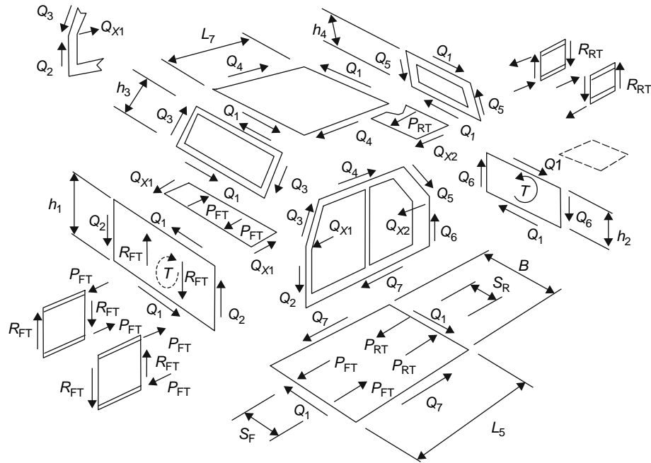
Fig. 16.2-12 Edge forces in the standard sedan in the torsion load case.
