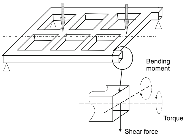
Fig. 16.1-3 Grillage frame.
