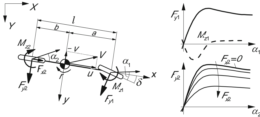
Fig. 11.1-9 Simple car model with side force characteristics for front and rear (driven) axle.
