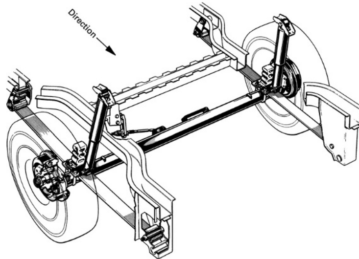
Fig. 8.1-24 The rear axle on a Ford Escort Express delivery vehicle. Single leaf springs carry the axle and support the body well at four points. The shock absorbers (fitted vertically) are located close to the wheel, made possible by slim wheel-carriers/hub units. The additional elastomer springs sit over the axle tube and act on the side members of the body when at full bump.
