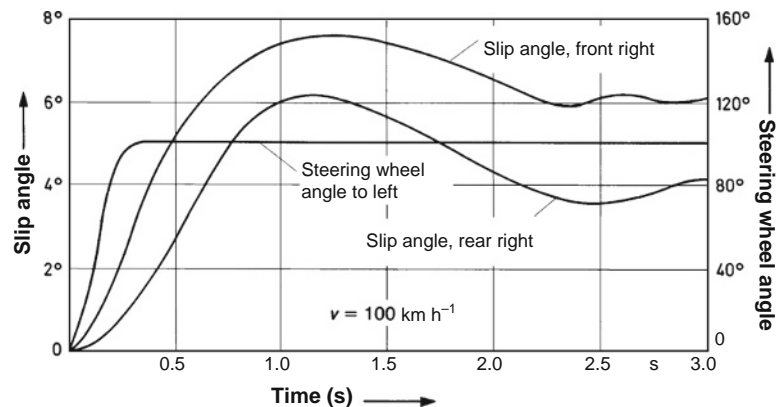
Fig. 9.1-2 Delayed, easily manageable response of the right front wheel when the steering wheel is turned by 100^\circ in 0.2 s, known as step steering input. A slip angle of \alpha_f \approx 7^\circ on both front tyres is generated in this test. The smaller angle \alpha_r on the rear axle, which later increases, is also entered. Throughout the measurement period it is smaller than \alpha_f (x-axis), i.e. the model studied by Mercedes Benz understeers and is therefore easy to handle.
