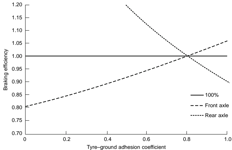
Figure 12.1-13c Brake system efficiency of modified prototype vehicle.
