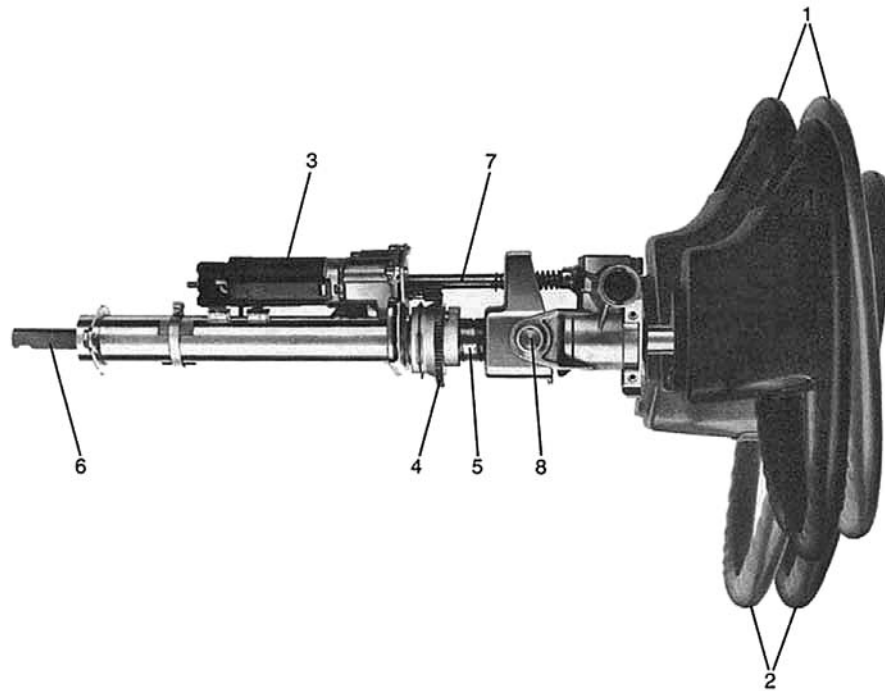
Fig. 9.1-30 Electrically adjustable steering column manufactured by Lemförder Fahrwerktechnik. The electric motor 3 turns a ball nut via the gears 4 and this engages with the grooves 5 of the steering tube and shifts it (position 6) in the longitudinal direction (position 1). To change the height of the steering wheel (position 2), the same unit tips around the pivot 8 by means of the rod 7.
