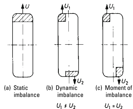
Fig. 10.1-29 Different forms of imbalance U : (a) static, (b) dynamic. The imbalance is equalized in (c).
