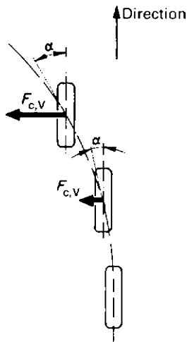
Fig. 10.1-38 The higher the lateral force F_{Y,W} , the greater the tyre slip angle \alpha .
