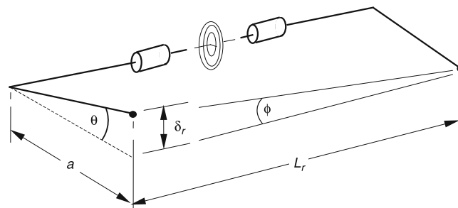
Fig. 15.1-24 Calculation of roll stiffness due to the anti-roll bar.
