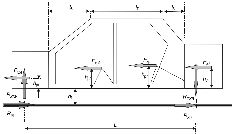
Fig. 16.2-30 Baseline model (side view) – braking loads.
