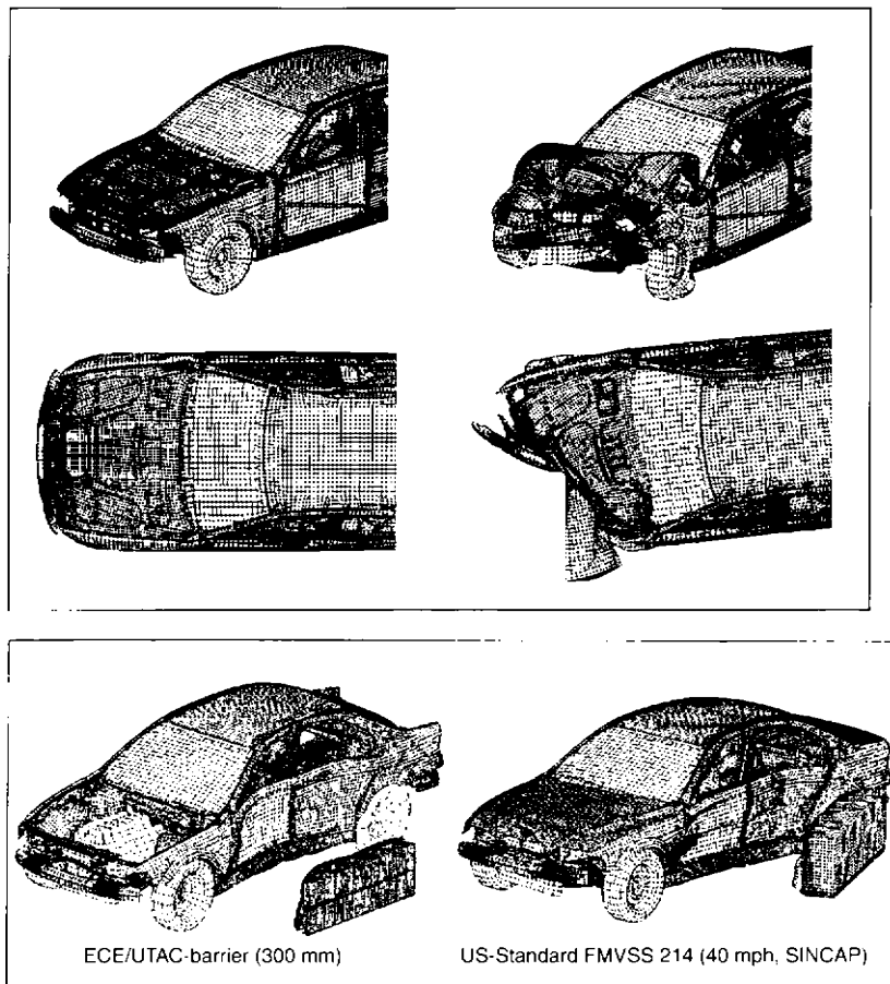
Fig. 18.1-12 Offset barrier (top) and side impact simulations (below). 6
