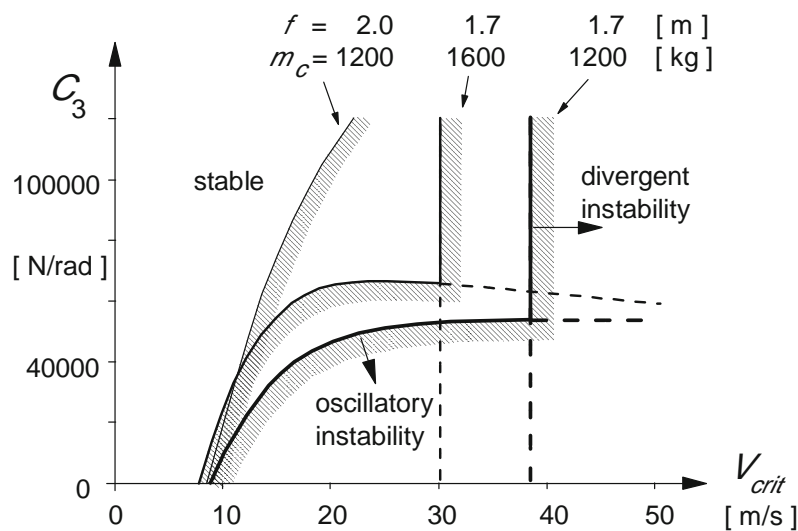
Fig. 11.1-30 Stability boundaries for the car caravan combination in the caravan cornering stiffness vs critical speed diagram. Vehicle parameters according to Table 11.1-1, in addition: h = 2 \text{ m} , g = 2 \text{ m} , k_c = 1.5 \text{ m} ( l_c = m_c k_c^2 ), cf. Fig. 11.1-29.
