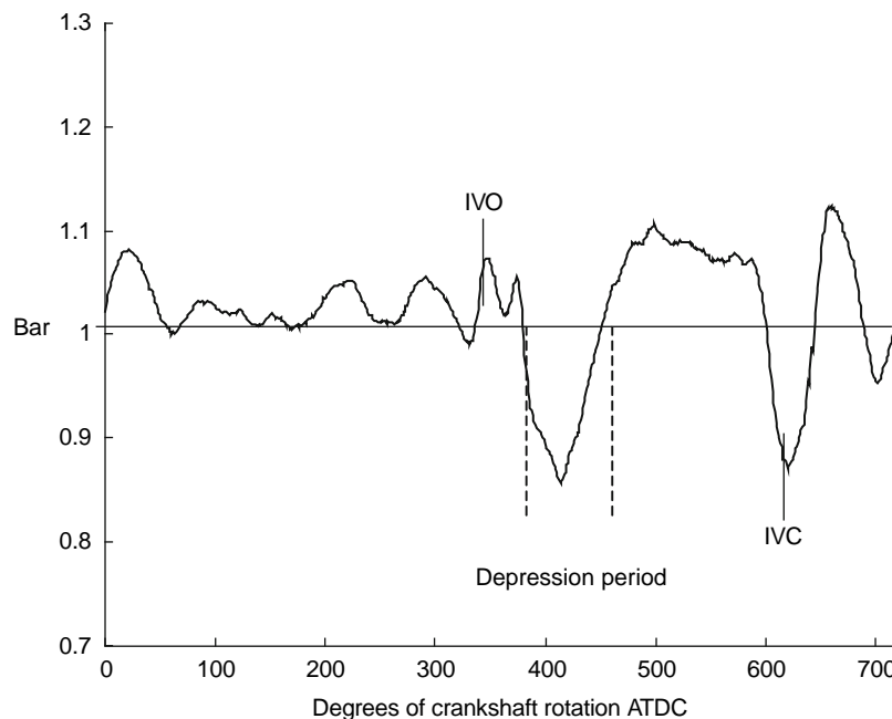
Fig. 22.1-13 Intake port pressure trace, 35% rated speed, full load (Dunkley, 1999).
