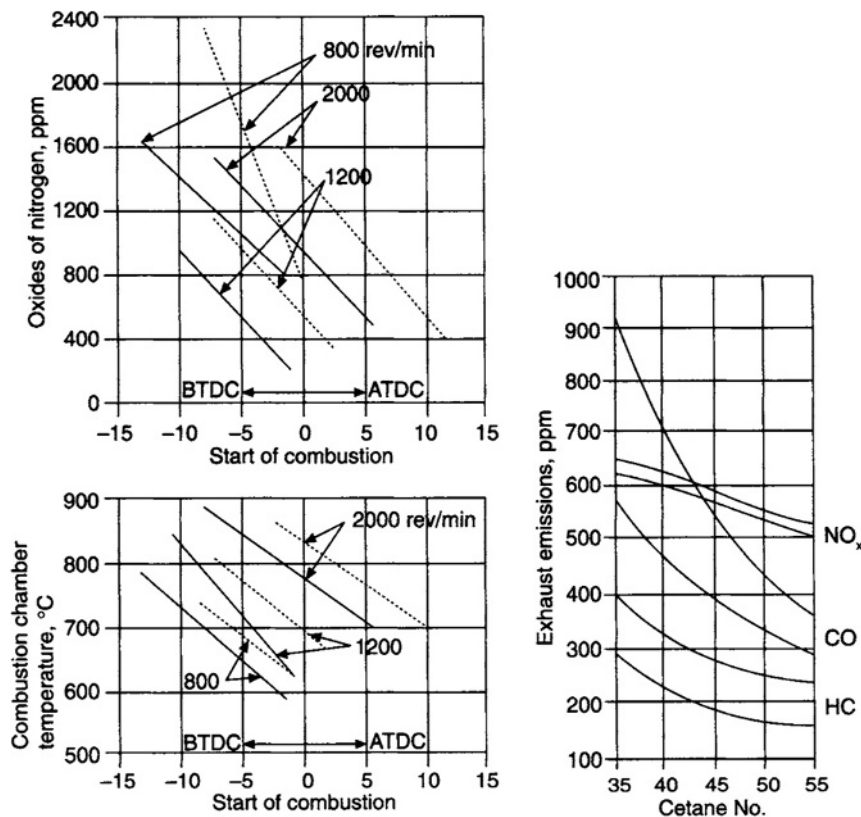
Fig. 3.1-21 (Left) Tests by BP showing how injection timing influences combustion and therefore \text{NO}_x output; (right) the influence of cetane number on the principal emissions.
