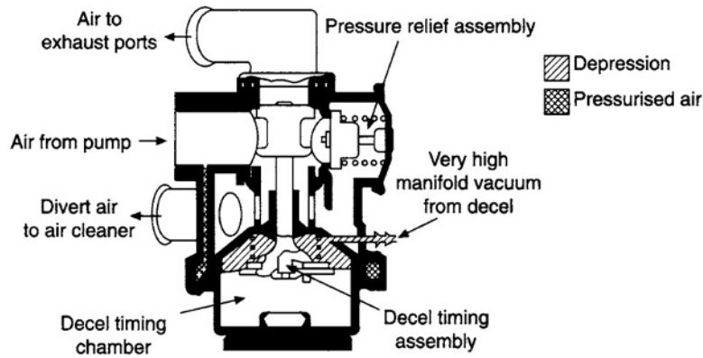
Fig. 3.1-9 Rochester standardised diverter valve, with high manifold depression applied to the diaphragm to divert air from its normal route, which is to the exhaust system, into the air cleaner.
