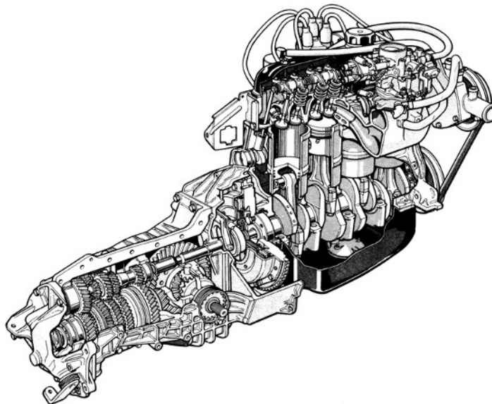
Fig. 8.1-48 In front-wheel drive vehicles the engine can be mounted longitudinally in front of the front axle with the manual gearbox behind. The shaft goes over the transverse differential (illustration: Renault).
