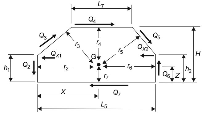
Fig. 16.2-14 Sideframe.
