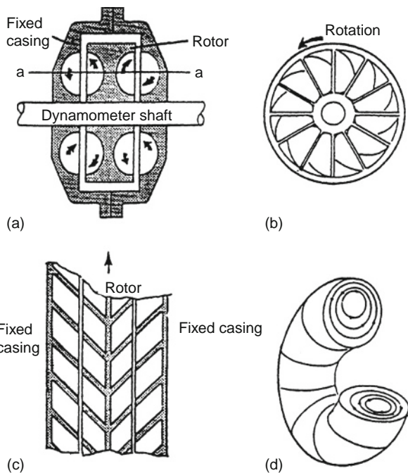
Fig. 2.1-9 Hydrokinetic dynamometer, principle of operation: (a) section through dynamometer; (b) end view of rotor; (c) development of section a-a of rotor and casing; (d) representation of toroidal vortex.
