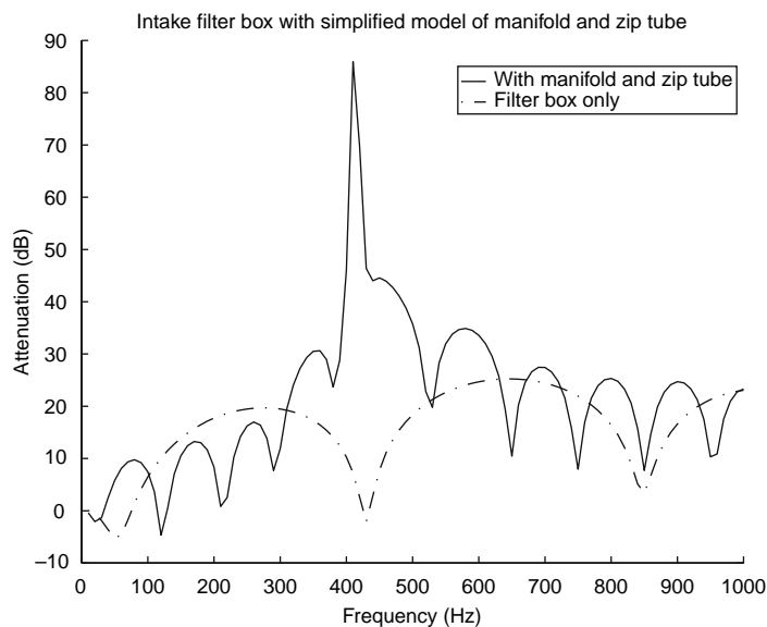
Fig. 22.1-39 The influence of the intake manifold and zip tube calculated using APINEX software.
