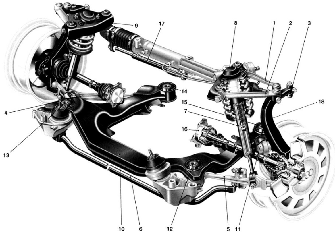
Fig. 8.1-54 Double wishbone front axle assembly of the Audi A4. The Audi A6 of 1997, the Audi A8 (1996) and the VW Passat of 1996 are similar. Four individual transverse 'arms' on each side form what is effectively a double wishbone arrangement which provides lateral and longitudinal wheel location. The two upper members (1 and 2) are attached to the spheroidal graphite iron hollow-section stub-axle post (18) by low-friction ball and socket joints. The track rod (3) provides the steering input through a horizontal extension of this stub-axle post which forms a steering arm. The two lower suspension members consist of the radius arm (4) and the transverse arm (5). This latter must be capable of reacting high loads from the anti-roll bar (6) and spring/damper (7) attachment points. The co-axial spring/damper assembly incorporates a polyurethane rubber bump-stop, as well as the hydro-mechanical tension rod stop. The spring/damper unit (7) and the inner bearings of the upper members (1) and (2) are mounted on the upper suspension bracket.
