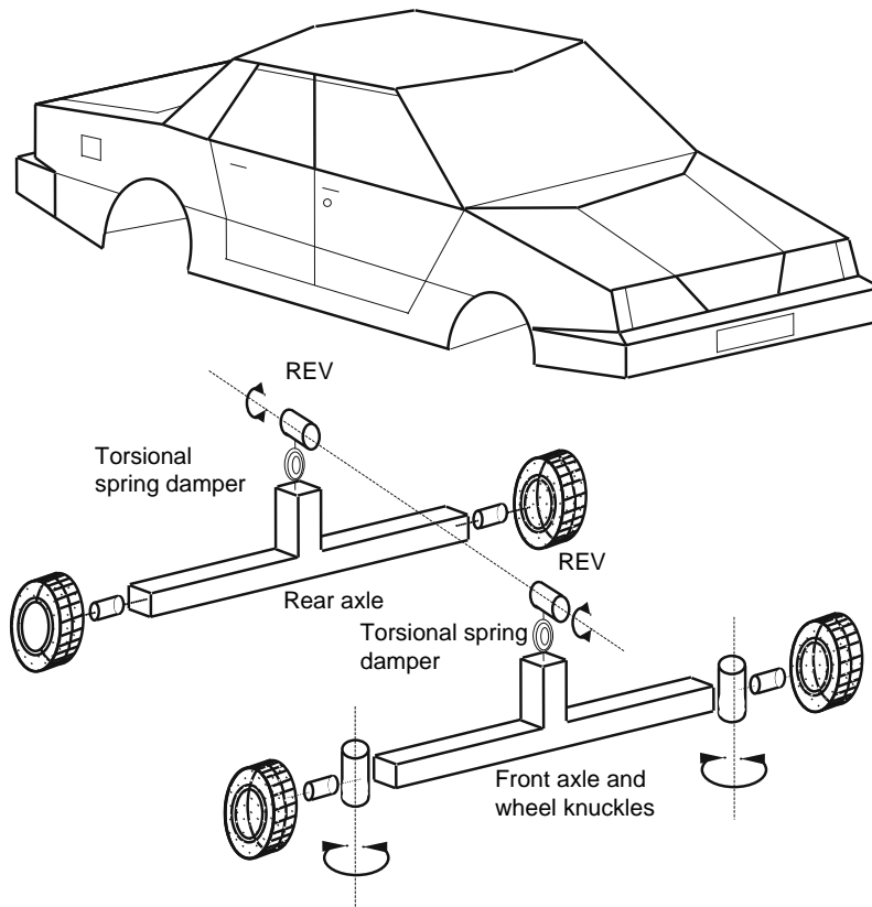
Fig. 15.1-8 Equivalent roll stiffness model approach.
