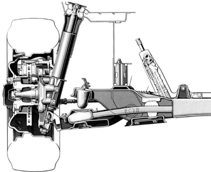
Fig. 8.1-41 Front axle of the Mercedes-Benz Sprinter series (1995). The wheel-controlling strut is screwed on to the wheel carrier, which is, in turn, connected to the lower cross-member by means of a ball joint. Both the vehicle suspension and roll stabilization are ensured by means of a transverse plastic leaf spring mounted on rubber elements. Large rubber buffers with progressive rigidity act as additional springs and bump stops.
