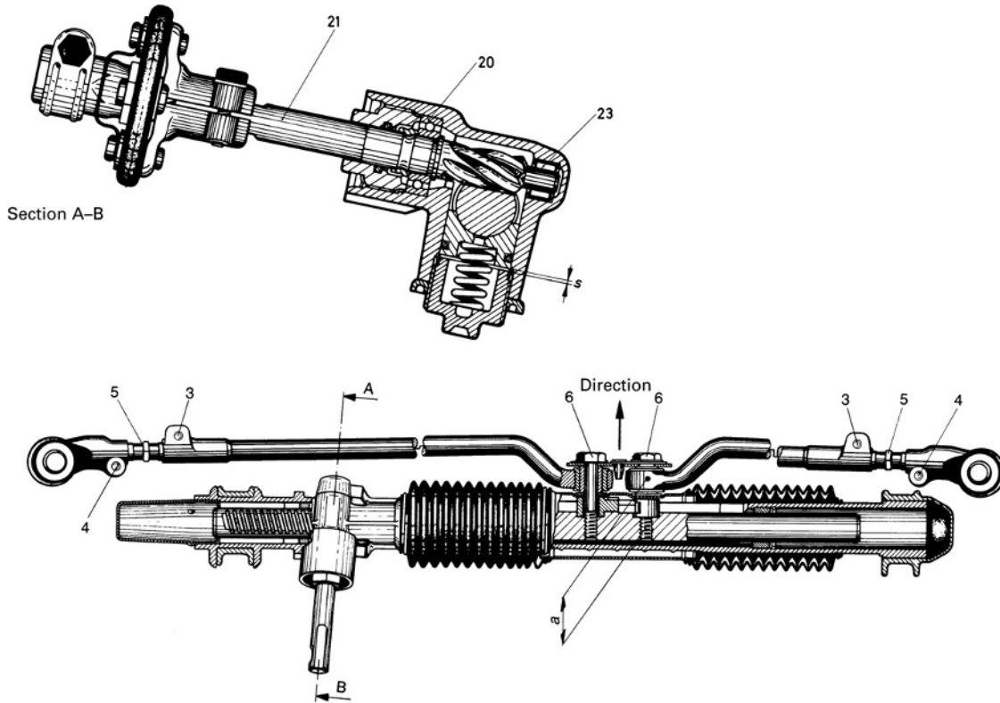
Fig. 9.1-11 Top view of the rack and pinion steering of the front-wheel-drive Opel (Vauxhall) Astra (up to 1997) and Vectra (up to 1996); the steering arms on the McPherson strut point backwards and the steering gear is located relatively high. For this reason the tie rods have to be jointed in the middle and (in order not to come into contact with the gear housing when the wheels are turned) have to be bent. The guide-bearing in the groove of the housing prevents the steering rack from twisting. On the inside, both tie rods have the eye-type joint; the distance a to the steering rack centre, which causes a bending moment, and a torque (when the wheels bump and rebound) is also shown. The two bolts 6 gripping into the steering rack are secured. Once the screws 3 and 4 have been loosened, toe-in to the left and right can be set by turning the connecting part 5. The steering gear has two fixing points on the dashpanel, which are a long way apart and which absorb lateral force moments with minimal flexing. As also shown in Fig. 9.1-10, the pinion is carried by a ball and a needle bearing (positions 20 and 23) and is also pressed onto the steering rack by a helical spring. The illustration shows the possible path s of the rack guide. Figs. 9.1-46–9.1-48 show the reason for the length of the tie rods on McPherson struts and strut dampers.
