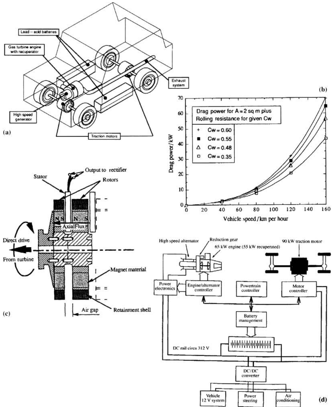
Fig. 7.1-10 Gas turbine hybrid taxi: (a) package; (b) typical steady-state vehicle power consumption; (c) high speed disc alternator; (d) system diagram of the TETLEI vehicle.
