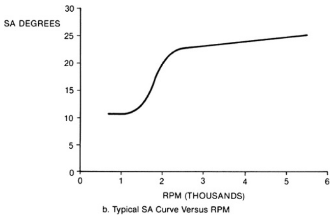
Fig. 4.1-9b Spark advance versus RPM.
