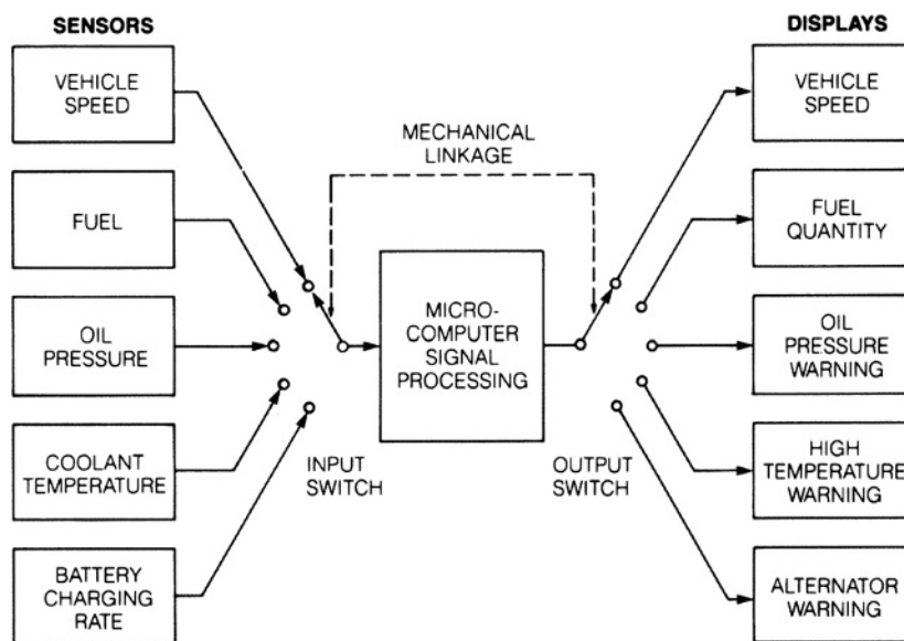
Fig. 23.1-5 Input/output switching scheme for sampling.
