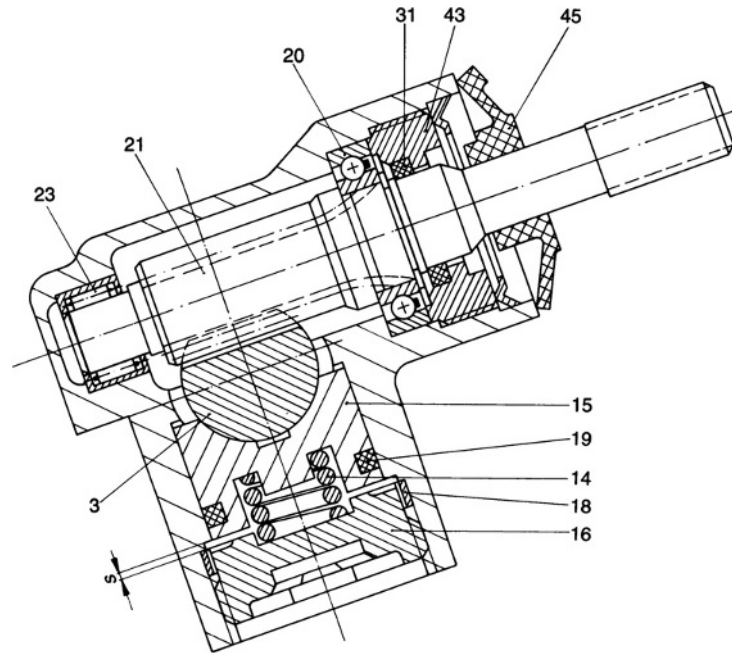
Fig. 9.1-10 Rack- and- pinion steering by ZF; section through pinion gear, bearing and rod guide. The distance ring 18 is used for setting the plays, and the closing screw 16 is tightened against it. The O-ring 19 provides the damping function and prevents rattling noises.
