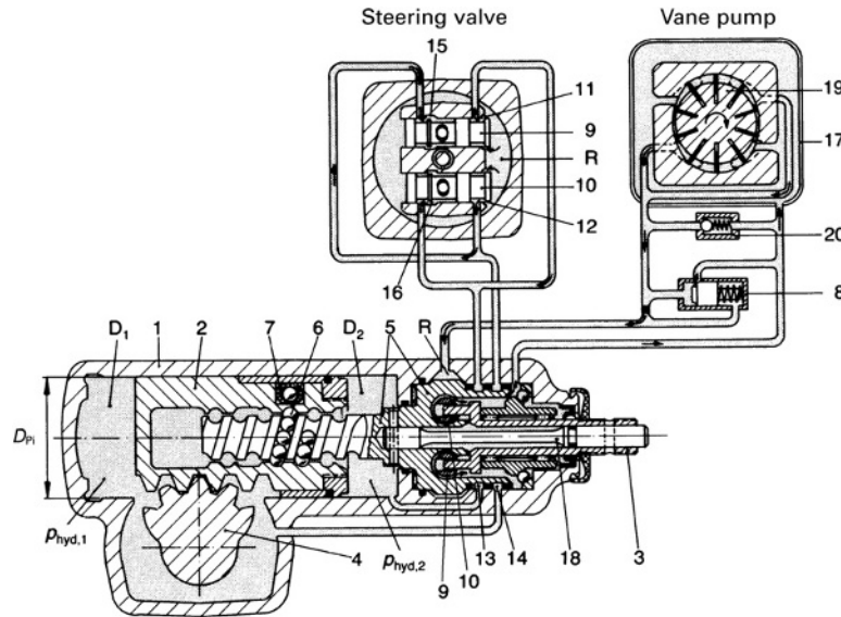
Fig. 9.1-17 Illustration of the principles of the ZF recirculating ball steering in the neutral position (vehicle travelling in a straight line). The steering valve, the working piston and the mechanical gear sit in a common housing. The two valve pistons of the steering valve have been turned out of their operating plane to make the diagram easier to see. The individual parts are:
