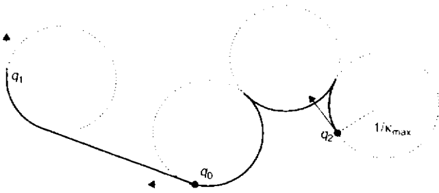
Fig. 14.2-30 Optimal paths for the Reeds and Shepp car.
