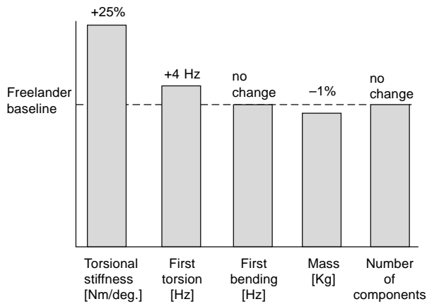
Fig. 18.1-39 Results from the application and proving phase. 16 (Reprinted with permission from SAE paper 1999-01-3181 Copyright 1999 Society of Automotive Engineers Inc.)
