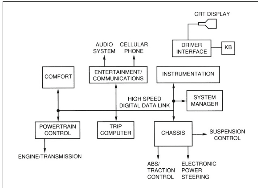
Fig. 23.1-26 Integrated vehicle electronic systems.
