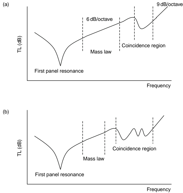
Fig. 21.1-19 Typical panel TL (after Bies and Hansen, 1996). (a) Isotropic panel and (b) orthotropic panel.
