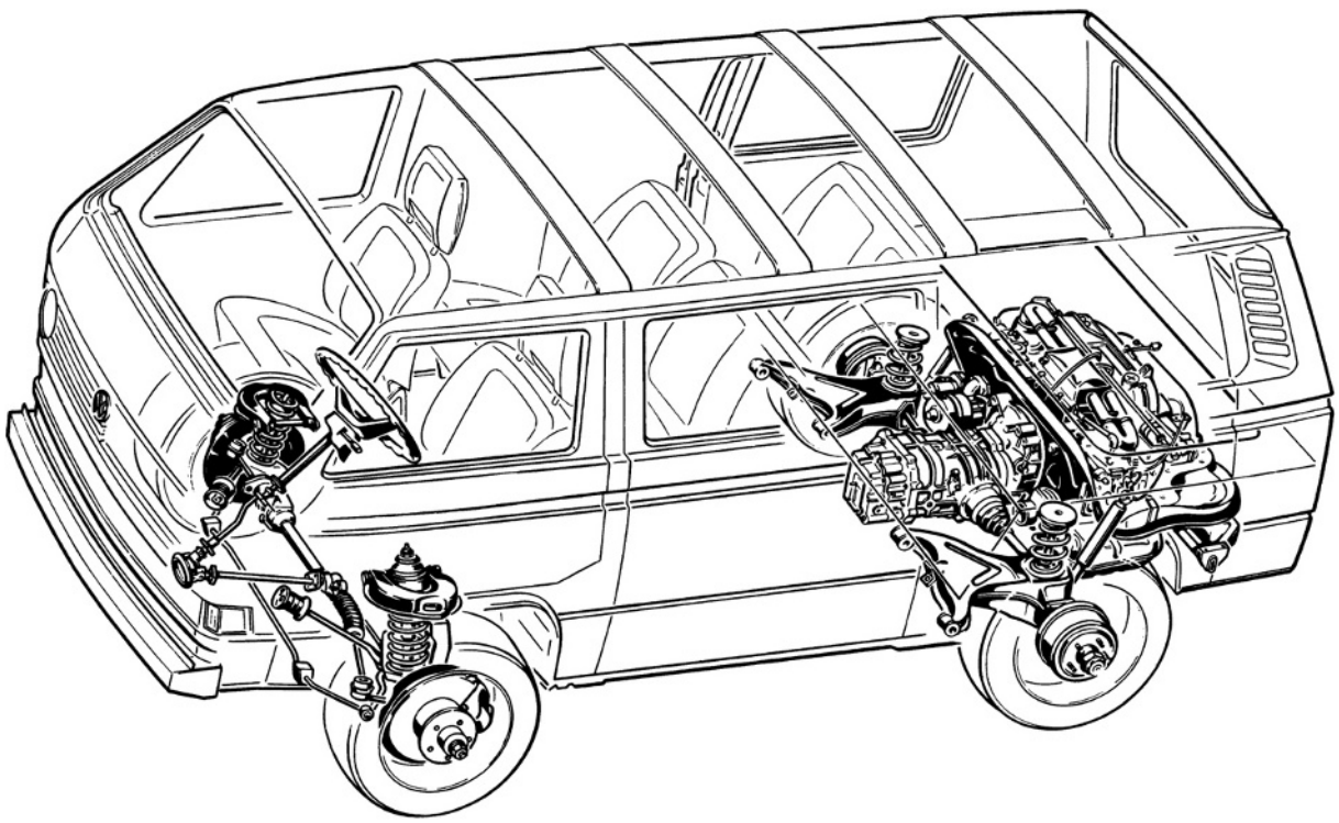
Fig. 8.1-45 VW Transporter, a light truck which could be used either as an eight-seater bus or for transporting goods, and which has the optimal axle load distribution of 50%/50% in almost all loading conditions. The double wishbone suspension at the front, the semi-trailing link rear axle and the rack and pinion steering, which is operated via an additional gear set in front, can be seen clearly. To achieve a flat load floor throughout, VW changed the Transporter to front-wheel drive in 1990.
