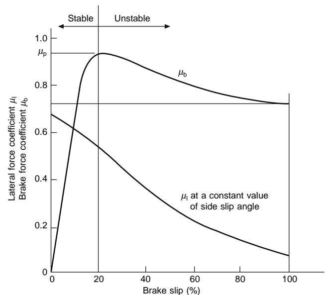
Figure 12.1-7 Brake force against wheel slip.
