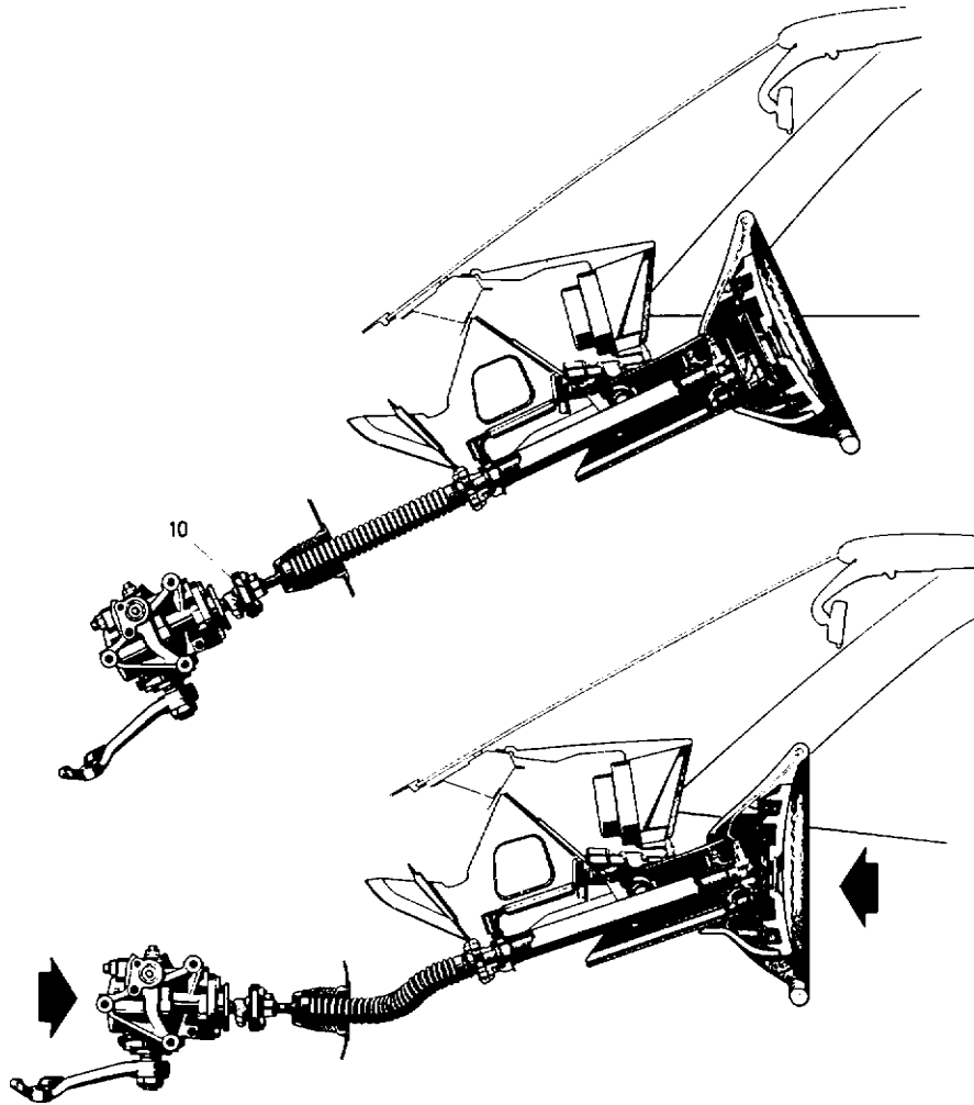
Fig. 9.1-24 Mercedes Benz safety steering tube and dished steering wheel; it is fixed to the recirculating ball steering gear with a compliant 'joint'. The bottom illustration shows the corrugated tube bending out in a head-on crash. The illustration also shows the energy-absorbing deformation of the steering wheel and the flexibility of the steering gear mounting.
