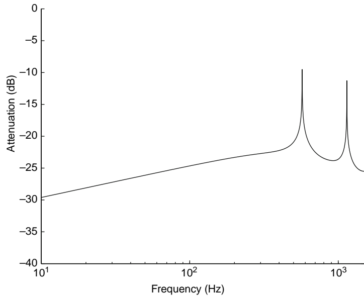
Fig. 21.1-22 Results for a steel box with a surface density of 16 \text{ kg m}^{-2} and l = 0.3 \text{ m} and s = 1 \times 10^8 \text{ N m}^{-1} using Jackson's method (Jackson, 1966).
