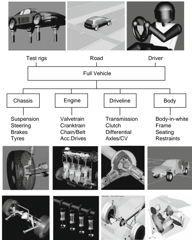
Fig. 15.1-1 Integration of subsystems in a full vehicle model (provided courtesy of MSC.Software).
