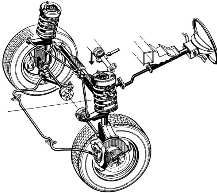
Fig. 8.1-57 Driven McPherson front axle on the Audi 6 (Audi 100, 1991). The dynamic rolling hardness of the radial tyre is absorbed by the rubber bearings, which sit in the lower transverse control arms. The inner sleeves of these bearings take the arms of the anti-roll bar, which also act as a trailing link (classic McPherson construction). To avoid greater toe-in changes when the wheels are at full bump/rebound-travel, centre take-off tie rods are used on the rack and pinion steering higher up and in the centre (Fig. 9.1-39). Together with these rods, the steering damper located on the right is fastened to the end of the steering rack. The engine is mounted longitudinally, which means the drive shafts are of equal length. The development of the axle since 1997 is shown in Fig. 8.1-54.
