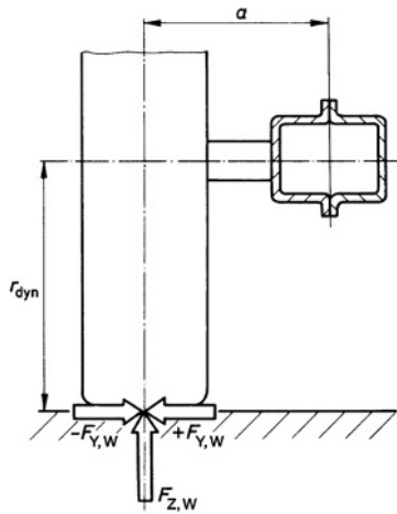
Fig. 8.1-14 On rear axle trailing-link suspensions, the vertical force F_{Z,W} together with the lateral forces F_{Y,W} cause bending and torsional stress, making a corresponding (hollow) profile, e.g. a closed box profile necessary. A force from inside causes the largest torsional moment:
