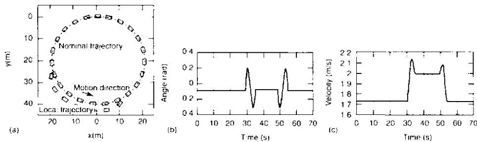
Fig. 14.2-18 Motion and control commands in the "roundabout" scenario: (a) motion, (b) steering angle and (c) velocity controls applied.
