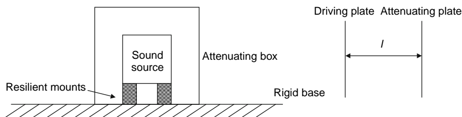
Fig. 21.1-21 Jackson's models (Jackson, 1962).
