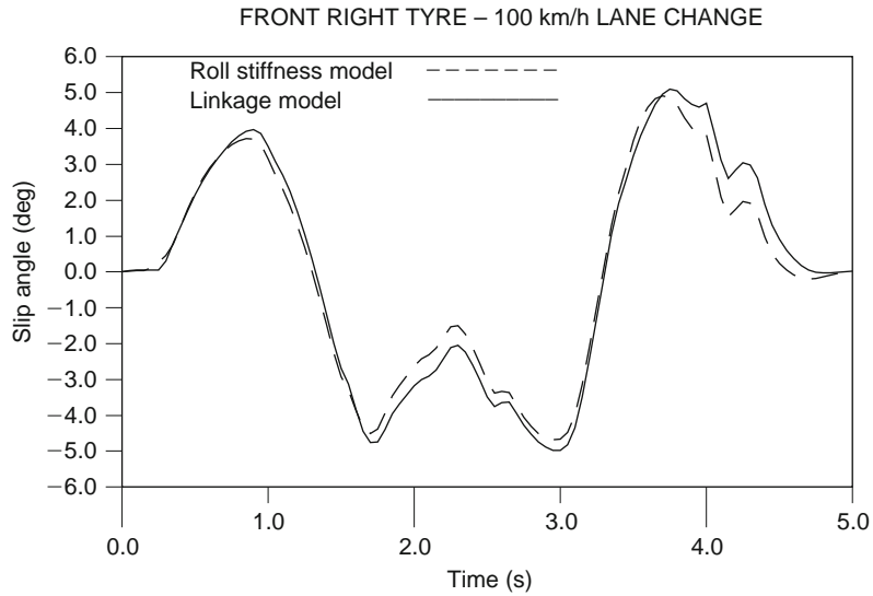
Fig. 15.1-59 Slip angle comparison – linkage and roll stiffness models.
