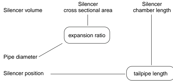
Fig. 22.1-23 Important parameter in flow duct acoustics.
