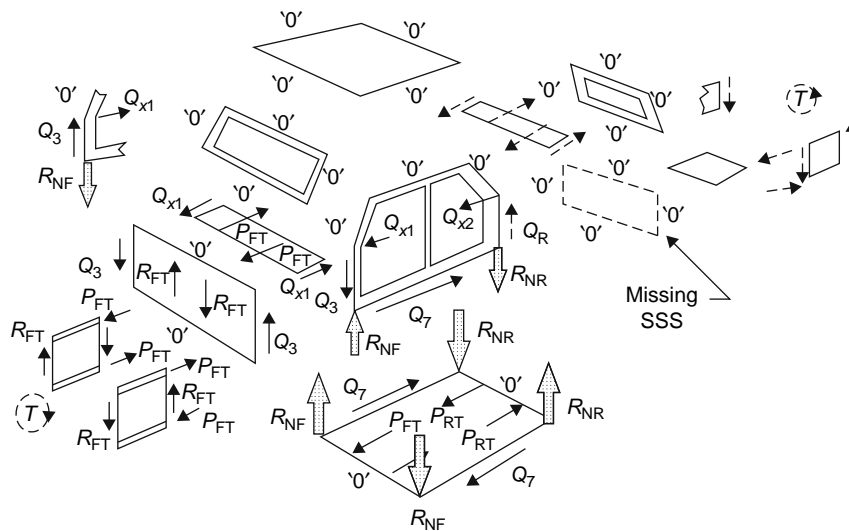
Fig. 16.2-18 Faux sedan in torsion.
