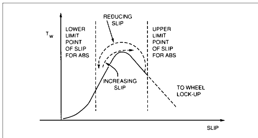
Fig. 13.1-15 Wheel torque versus slip.
