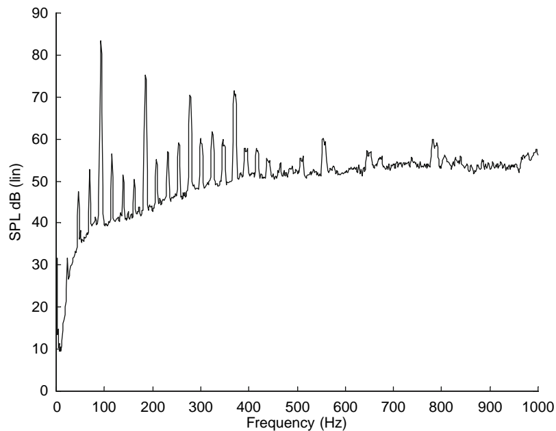
Fig. 22.1-20 Sound pressure levels recorded 500 mm from the exhaust tailpipe of a 1.6-litre four-cylinder gasoline engine running full load at 2800 rev min -1 .
