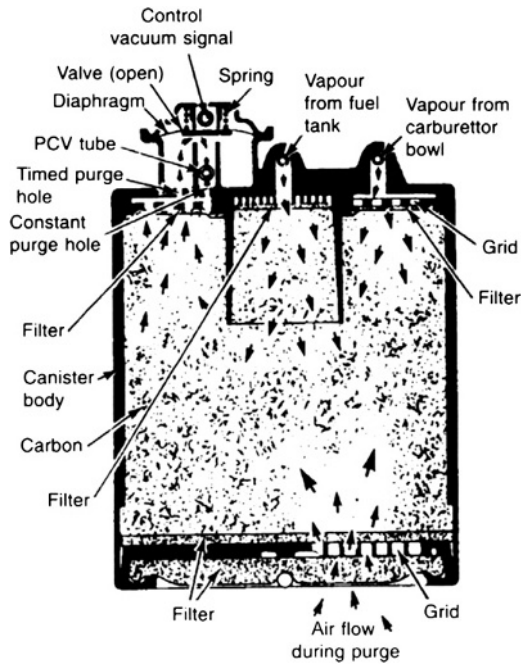
Fig. 3.1-15 A purge valve canister of the open-bottom type.
