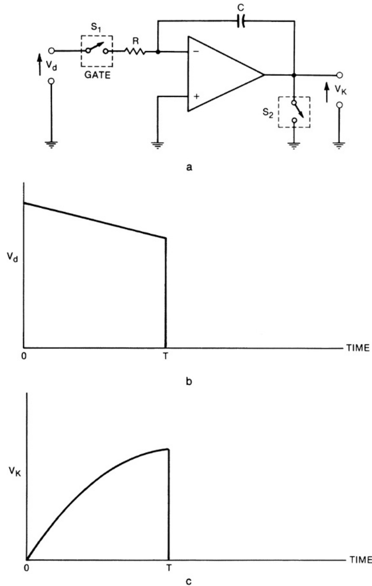
Fig. 4.1-13 Example integrator circuit diagram.
