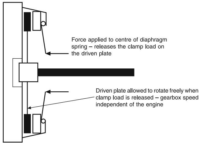
Fig. 5.1-14 Diagram of clutch when released.
