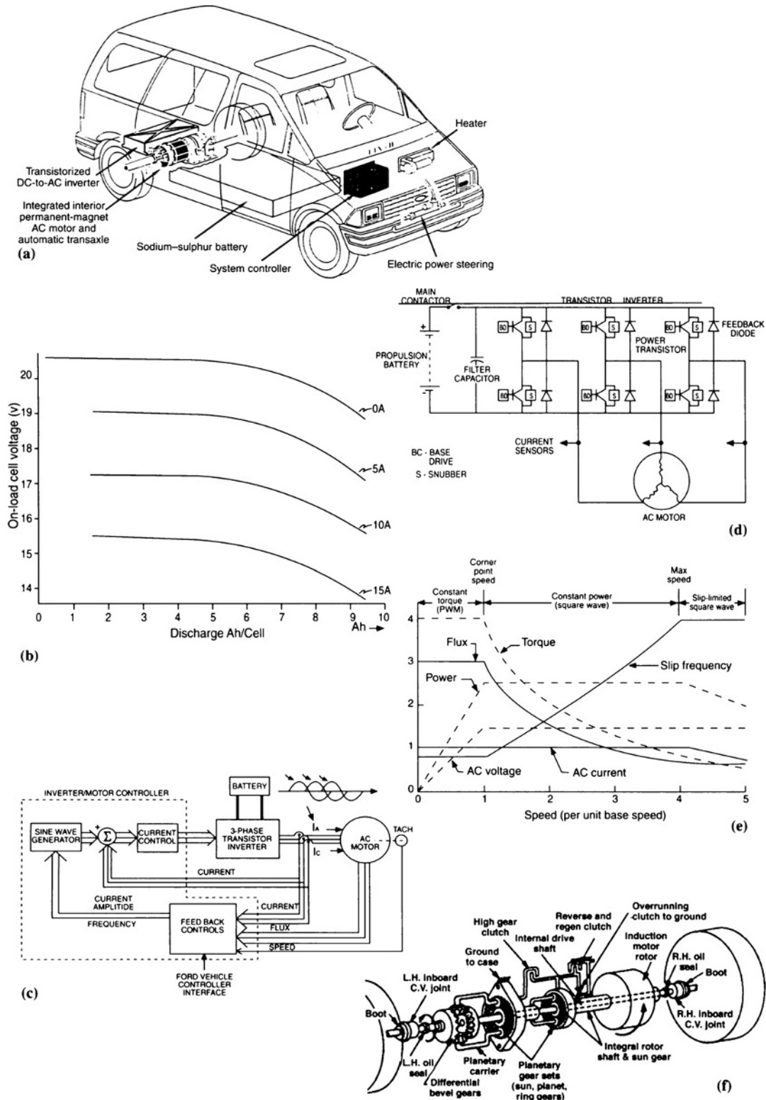
Fig. 6.1-19 Ford EXT 11 EV project: (a) AC-driven Ford Aerostar conversion; (b) discharge performance of s-s cells; (c) AC drive; (d) transistorized inverter; (e) AC control strategy; (f) transaxle drive with coaxial motor.
