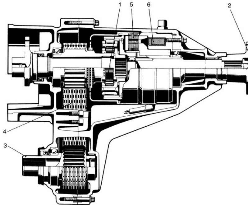
Fig. 8.1-79 The torque coming from the engine is apportioned by the Planet Wheel-Centric Differential 1 in such one, to the rear cardan shaft 2 (64%) and to the front one 3 (36%). The offset to this shaft is bridged-over by the inserted tooth type chain 4. The adaptation of the distribution of driving power is taken over the multiple-disk clutch 5, which is driven (controlled) by the electromagnet. Power Divider A110 of the Fa. ZF (Zahnradfabrik Friedrichshafen).
