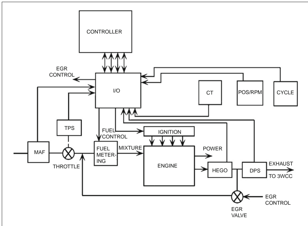
Fig. 4.1-2 Digital engine control system diagram.
