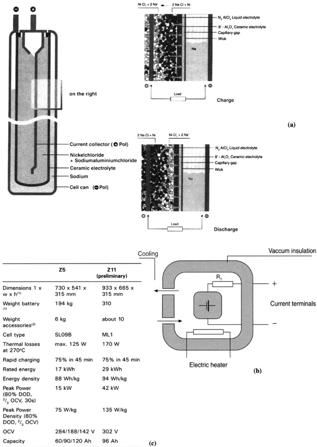
Fig. 6.1-4 ZEBRA battery: (a) cell; (b) cell-box; (c) performance comparison.
