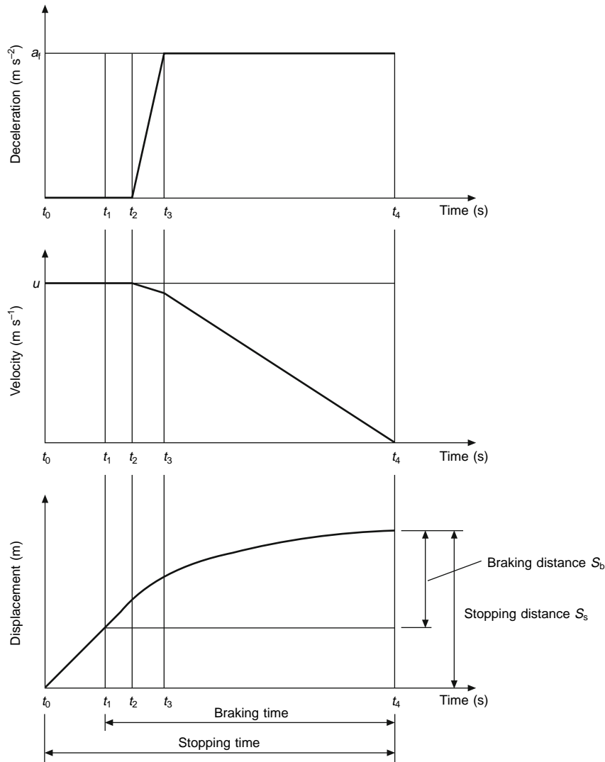
Figure 12.1-5 Four-stage stop simulation.
