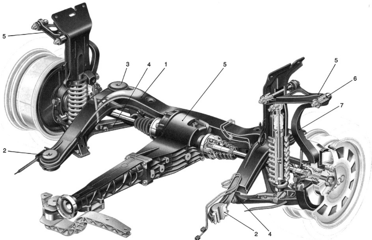
Fig. 8.1-76 Double wishbone rear axle on the Audi A4 Quattro. The suspension subframe 1 is fixed to the body with four widely spaced rubber mountings (items 2 and 3) and houses the differential casing 8 and transverse control arms (items 4 and 5). The springs and shock absorbers are mounted next to the fixings for the upper control arms 7. The location 6 of the wheel hub carrier 5 was raised (long base c , Fig. 8.1-4) and drawn outwards. The lower transverse control arm 4 is fixed to part 1 with widely spaced mountings. These measures ensure a wide boot and low forces, making it easier to attain the desired kinematic characteristics.
