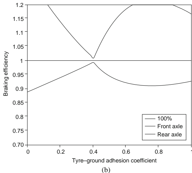
Figure 12.1-19 (a) Adhesion utilization, modified vehicle fitted with deceleration-sensitive pressure, (b) brake system efficiency, modified vehicle fitted with deceleration sensitive.
