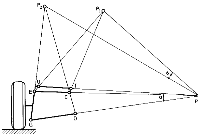
Fig. 9.1-44 A high-location steering gear can involve a tie rod above the upper control arm. The steering arm points backwards and towards the inside in the example.
