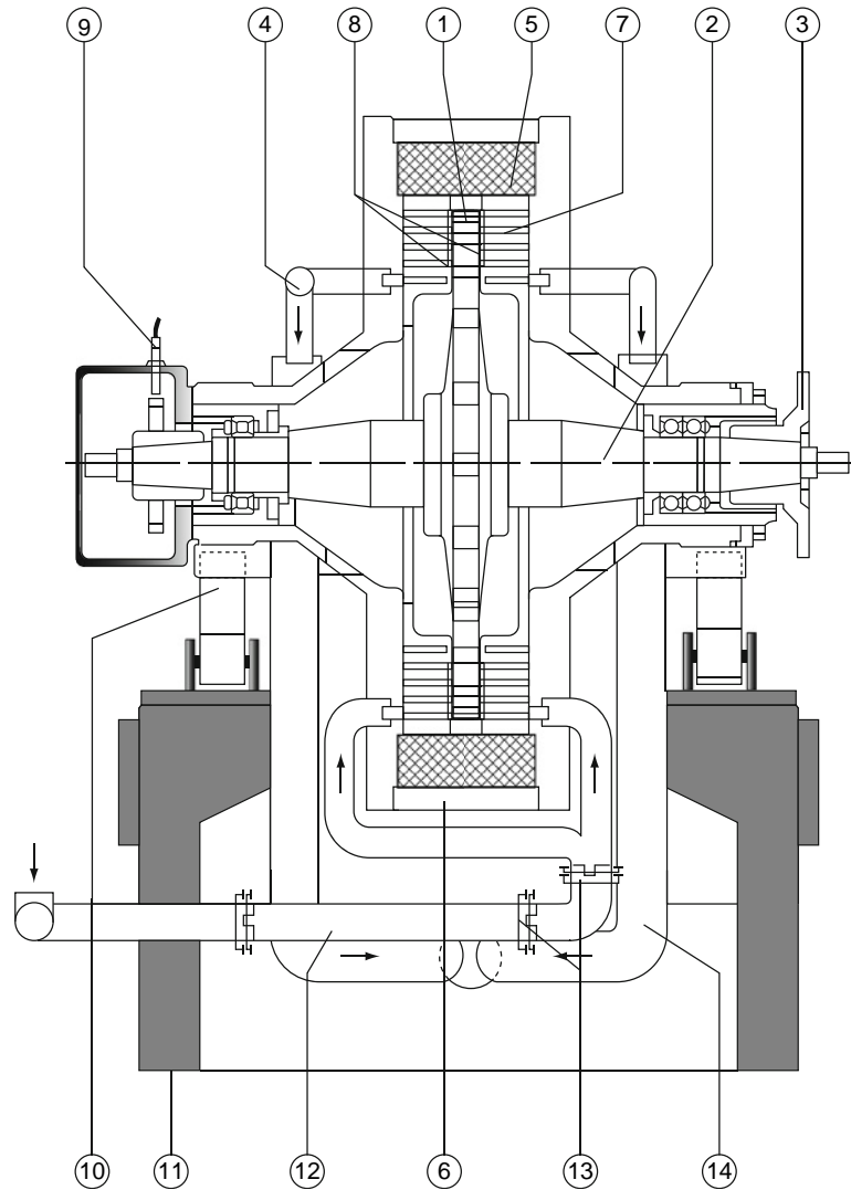
Fig. 2.1-3 Schenck, dry gap, disc type eddy-current dynamometer 1, rotor; 2, rotor shaft; 3, coupling flange; 4, water outlet with thermostat; 5, excitation coil; 6, dynamometer housing; 7, cooling chamber; 8, air gap; 9, speed pick-up; 10, flexure support; 11, base; 12, water inlet; 13, joint; 14, water outlet pipe.
