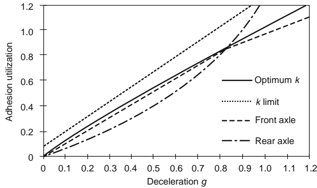
Figure 12.1-13b Adhesion utilization, modified prototype vehicle.
