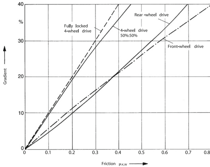
Fig. 8.1-65 Hill-climbing capacity on a homogeneous surface with front, rear-wheel and four-wheel drive, and with locked centre differential and a driving force distribution of 50%/50% on four-wheel drive. Of the cars studied, the front/rear axle load distribution was (Fig. 8.1-36):
