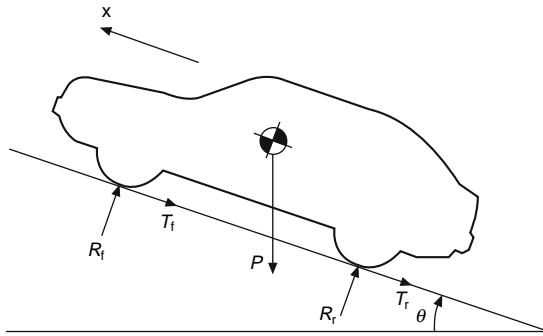
Figure 12.1-6 Free body diagram of a braking vehicle.
