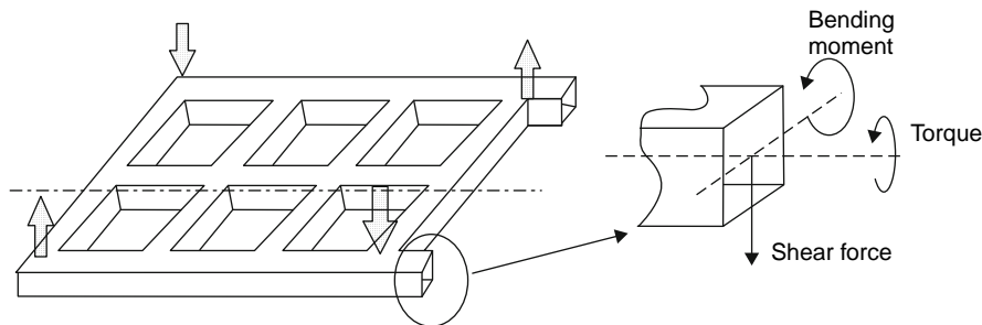
Fig. 16.2-21 Grillage structure.
