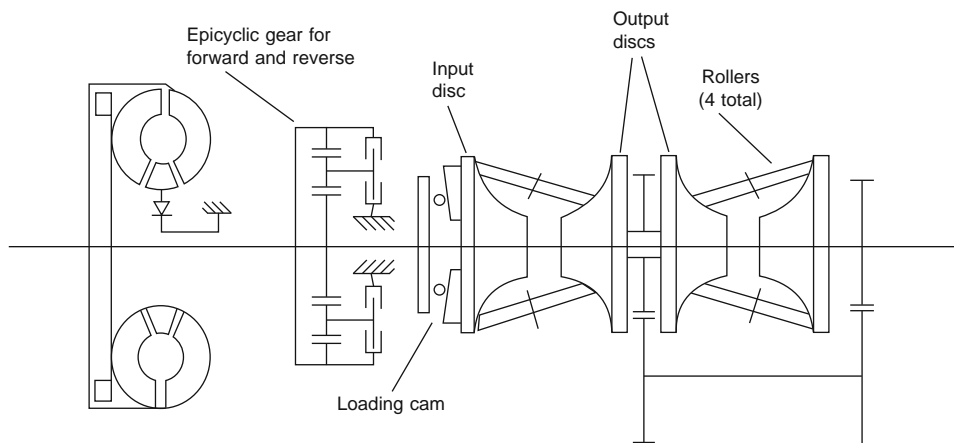
Fig. 5.1-32 A dual-cavity half-toroidal transmission.
