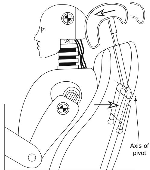
Fig. 17.1-20 The Saab seat designed to prevent spinal damage due to whiplash. At the lower end of the pivoted lever is a pad against which, during a rear end impact, the shoulders push to swing the head rest at the upper end of the lever forwards about the pivot to support the head. Stops, not shown here, limit the motion of the lever.
