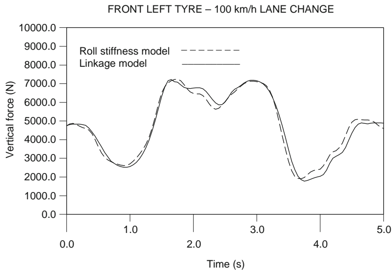
Fig. 15.1-58 Vertical tyre force comparison – linkage and roll stiffness models.
