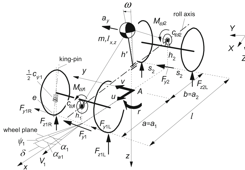
Fig. 11.1-4 Vehicle model showing three degrees of freedom: lateral, yaw and roll.
