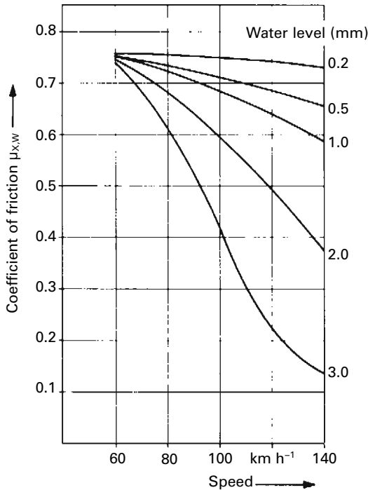
Fig. 10.1-35 Coefficients of friction \mu_{x,w} of a summer tyre with an 8-mm deep profile dependent on speed at different water levels. Hardly any influence can be detected under 60 \text{km h}^{-1} ; at higher speeds and 3-mm water depth, the curve shows a lowering of \mu_{x,w} which indicates the aquaplaning effect.
