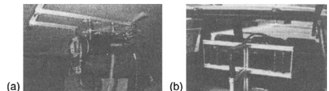
Fig. 14.2-22 Experimental setup for platooning: (a) the linear camera, (b) the first experimental infrared target.
