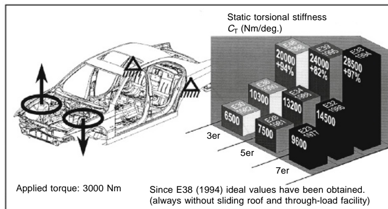
Fig. 18.1-10 Progressive improvement in torsional stiffness shown for successive BMW model generations. 6
