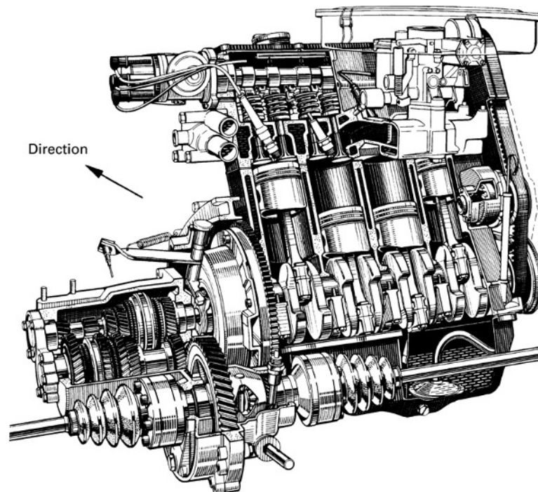
Fig. 8.1-50 Layout of transverse engine, manual gearbox and differential on the VW Polo. Because the arrangement is offset, the axle shaft leading to the left front wheel is shorter than that leading to the right one. The shifter shaft between the two can be seen clearly. The total mechanical efficiency should be around n \approx 0.9 .
