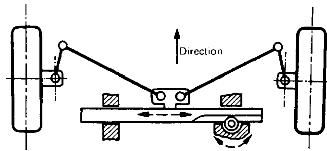
Fig. 9.1-39 The rack-and-pinion steering is behind and above the wheel centre and the steering arms point forward (shown for a right-hand-drive vehicle). For kinematic reasons, the inner tie rod joints are fixed to a central outrigger – known as a central take-off. This type of solution (also shown in Fig. 8.1-57) is necessary on McPherson and strut damper front axles with a high-location steering system as the tie rods have to be very long to avoid unwanted steering angles during jounce.
