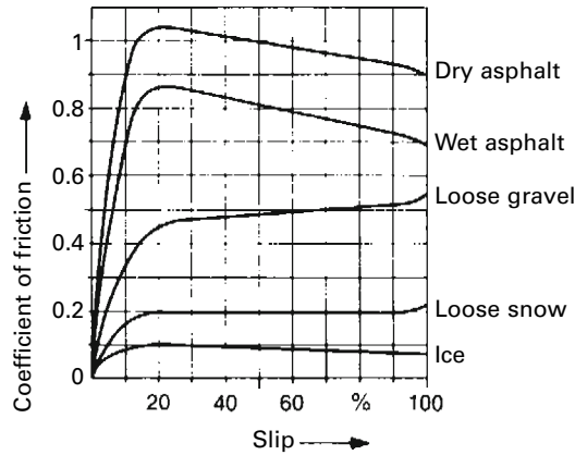
Fig. 10.1-33 Coefficient of friction \mu_{X,W} of a summer tyre with 80–90% deep profile, measured at around 60 km/h and shown in relation to the slip on road surfaces in different conditions (see also Fig. 8.1-64). Wide tyres in the '65 series' and below have the greatest friction at around 10% slip, which is important for the ABS function.
