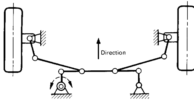
Fig. 9.1-38 'Opposed' 4-bar linkage located behind the wheel centre. The inner tie rod joints can be fixed to the middle part of the intermediate rod or directly to the pitman and idler arm (see Fig. 9.1-12).
