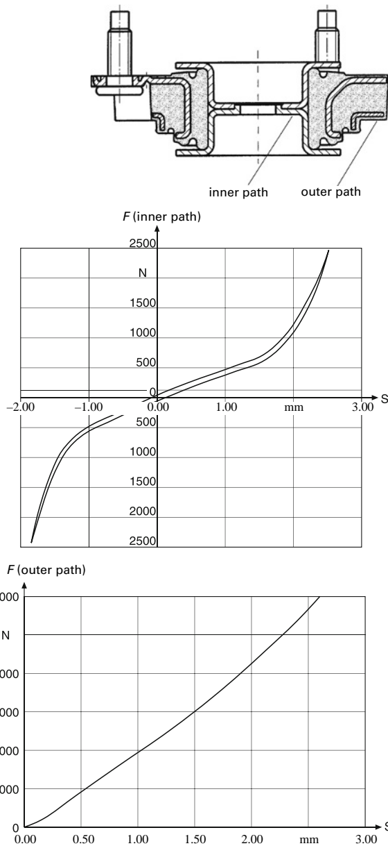
Fig. 8.1-10 The dual path top mount support of the Ford Focus (1998) manufactured by ContiTech Formteile GmbH. The body spring and shock-absorber forces are introduced into the body along two paths with variable rigidity. In this way, it is possible to design the shock-absorber bearing (inner element) in the region of small amplitudes with little rigidity and thus achieve good insulation from vibration and noise as well as improve the roll behaviour of the body. With larger forces of approximately 700 N and above, progression cams, which increase the rigidity of the bearing, come into play. A continuous transition between the two levels of rigidity is important for reasons of comfort. The bearing must have a high level of rigidity in a transverse direction in order to ensure that unwanted displacements and hence changes in wheel position do not occur. The forces of the body springs are directed along the outer path, which has a considerably higher level of rigidity.
