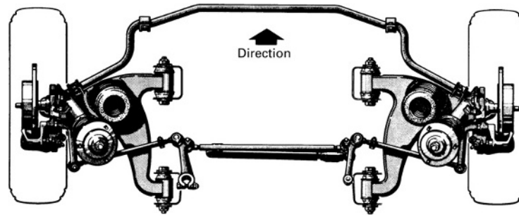
Fig. 9.1-12 Top view of the strut damper front axle on a Mercedes vehicle. The intermediate rod and the tie rods are fixed side by side on the pitman and idler arms and one grips from the top and the other from the bottom into the two levers; the steering square is opposed. The steering damper is supported on the one side at the intermediate rod and on the other side on the suspension subframe. The anti-roll bar is linked to the lower wishbone type control arms whose inner bearings take large rubber bushings. The defined springing stiffness of these bearings, together with the inclined position of the tie rods (when viewed from the top) means that when the vehicle corners, there is a reduction in the steering input, i.e. elastic compliance in the steering, tending towards understeering. The strut dampers are screwed to the steering knuckles; the negative kingpin offset is r_p = -14 mm.
