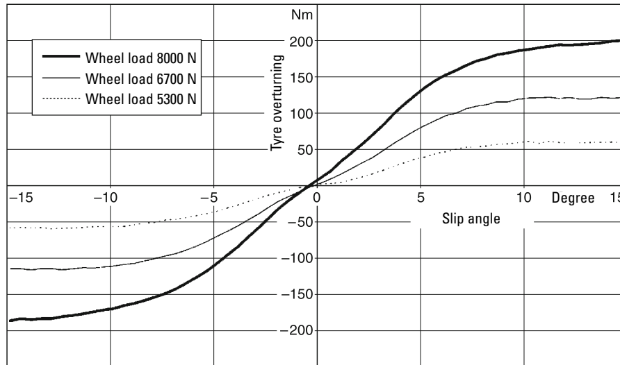
Fig. 10.1-52 Tyre overturning moments M_{X,T,\alpha} on the wheel as a result of the buildup of lateral forces at different slip angles and wheel loads F_{Z,W} ; measurements by Continental on a tyre of type 205/65 R 15 94 V ContiEcoContact CP.
