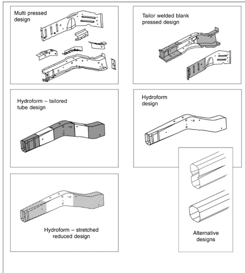
Fig. 18.1-36 Alternative forms of longitudinal section. (Reprinted with permission from SAE paper 1999-01-3181 Copyright 1999 Society of Automotive Engineers Inc.)
