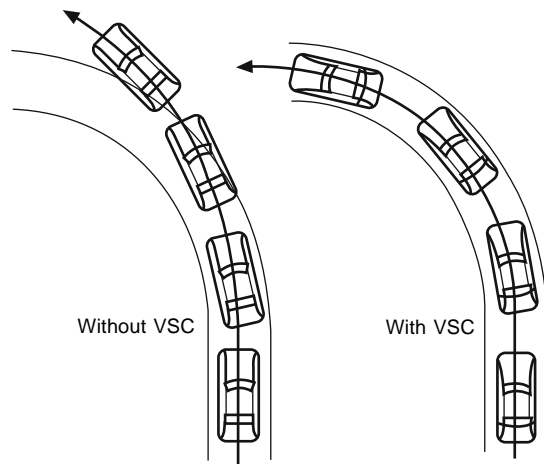
Fig. 17.1-19 Left , diagram showing the path typical of an understeering car driven beyond the limit of adhesion of the wheels on the road compared with, right , one driven in the same manner but equipped with vehicle stability control.
