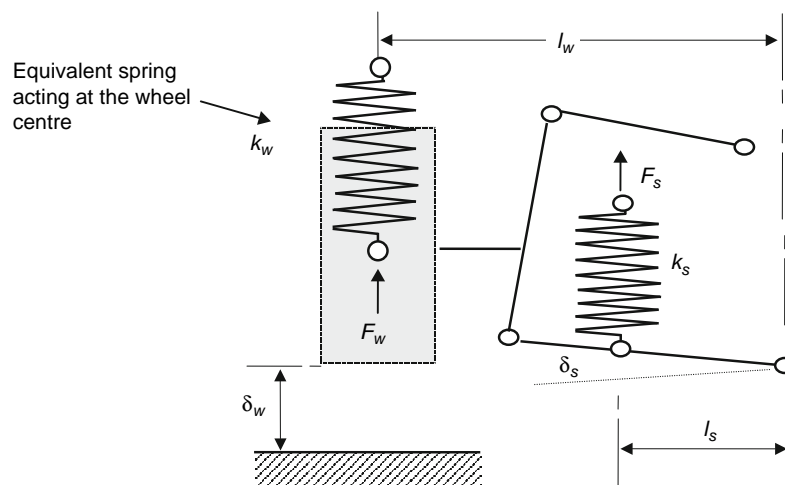
Fig. 15.1-14 Equivalent spring acting at the wheel centre.
