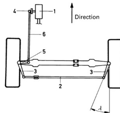
Fig. 9.1-5 On rigid axles, apart from the two steering arms 3, only the tie rod 2, the idler arm 5 and the drag link 6 are needed to steer the wheels. If leaf springs are used to carry the axle, they must be aligned precisely in the longitudinal direction, and lie vertical to the lever 5 when the vehicle is moving in a straight line. Steering arm angle \lambda is an essential factor in the relationship between the outer and the inner curve steering angles.
