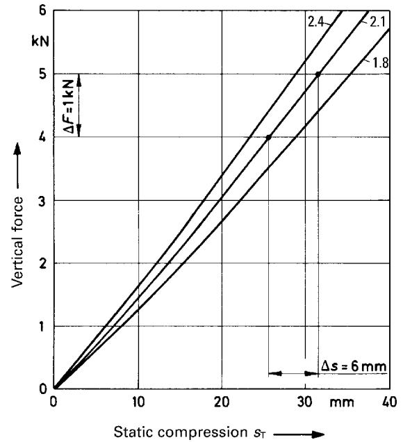
Fig. 10.1-27 The static tyre spring rate c_T is the quotient of the force and the deflection travel shown on the radial tyre 175/70 R 13 80 S at p_T = 1.8 bar, 2.1 bar and 2.4 bar; the example shown gives: c_T = \frac{\Delta F_{Z,W}}{\Delta s_T} = \frac{1000 \text{ N}}{6 \text{ mm}} = 167 \text{ N/mm}
