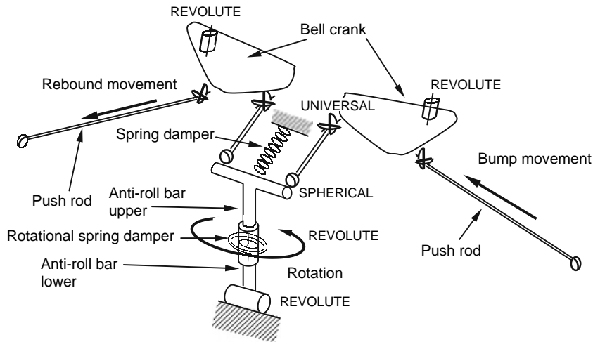
Fig. 15.1-20 Modelling of anti-roll bar mechanism in student race car.
