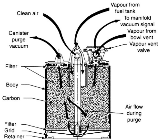
Fig. 3.1-16 Canisters of the closed-bottom type will not let water in at the base, where it could freeze and inhibit the purge action.
