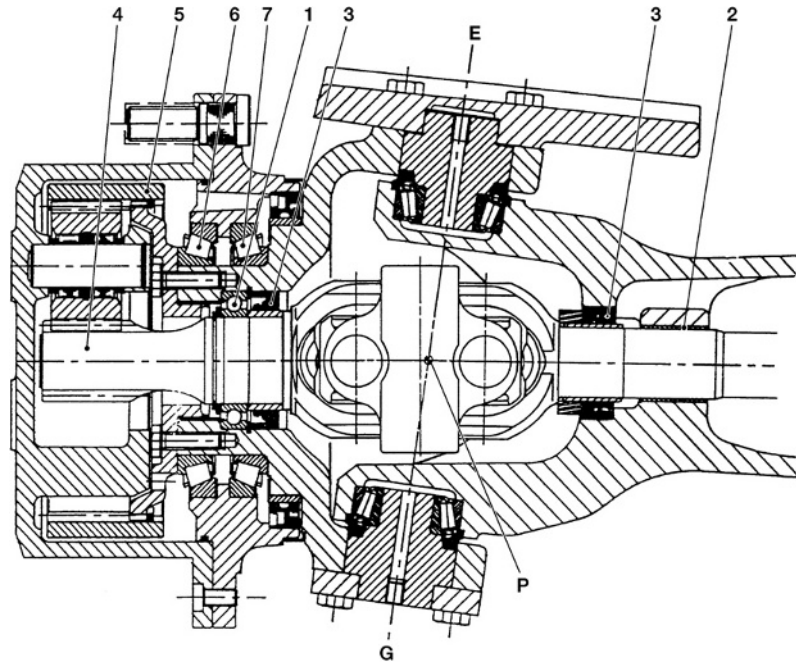
Fig. 8.1-3 Driven, rigid steering axle with dual joint made by the company GKN – Birfield AG for four-wheel-drive special-purpose vehicles, tractors and construction machinery.
