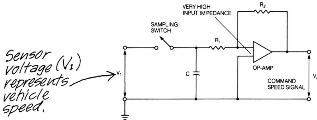
Fig. 13.1-10b Typical sample-and-hold circuit.
