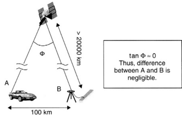
Fig. 14.1-4 Pseudorange correction in DGPS (not to scale).
