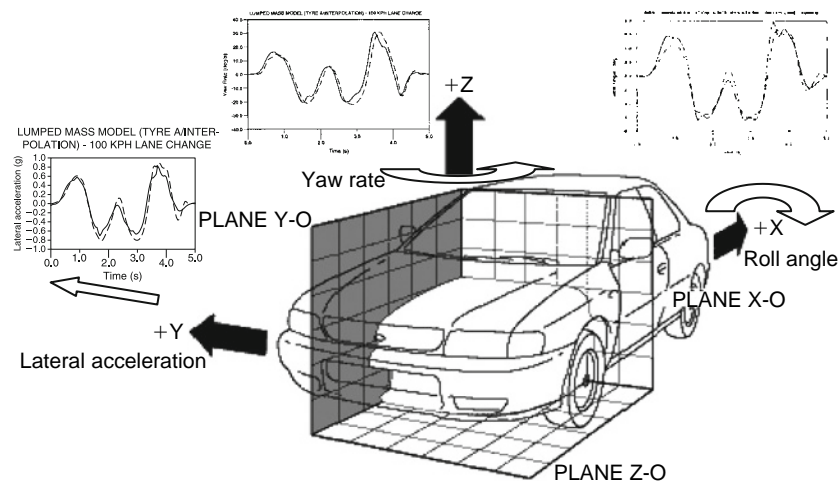
Fig. 15.1-5 Typical lateral responses measured in vehicle co-ordinate frame.
