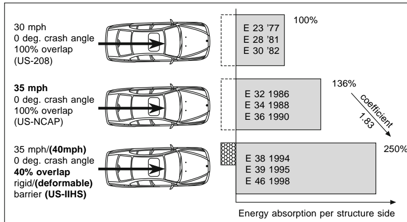
Fig. 18.1-11 Increasingly stringent objectives for crashworthiness. 6
