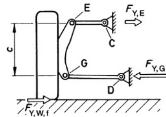
Fig. 8.1-5 On front independent wheel suspensions, the lateral cornering force F_{Y,W,f} causes the reaction forces F_{Y,E} and F_{Y,G} in the links joining the axle with the body. Moments are generated on both the outside and the inside of the bend and these adversely affect the roll pitch of the body. The effective distance c between points E and G on a double wishbone suspension should be as large as possible to achieve small forces in the body and link bearings and to limit the deformation of the rubber elements fitted.
