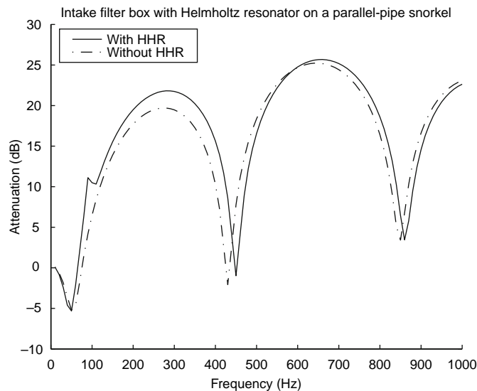
Fig. 22.1-35 Effect of an added Helmholtz resonator calculated using APINEX software.
