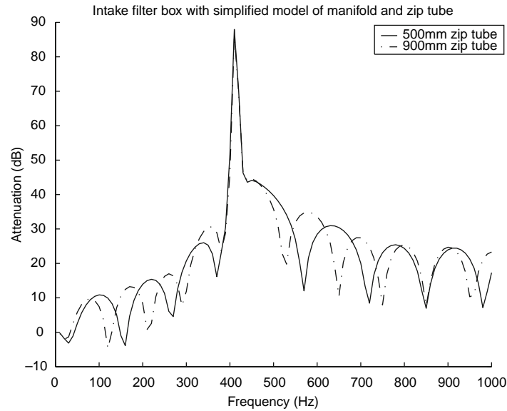
Fig. 22.1-40 Influence of zip tube length calculated using APINEX software.
