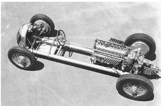
Fig. 16.1-13 Twin tube frame of Auto Union racing car (1934–1937) (courtesy of Deutsches Museum, München).
