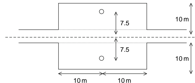
Fig. 22.1-1 The test area defined in ISO 362:1998.
