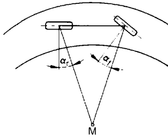
Fig. 10.1-40 If, during cornering, \alpha_f \sim \alpha_r , the handling of a vehicle can be described as neutral.
