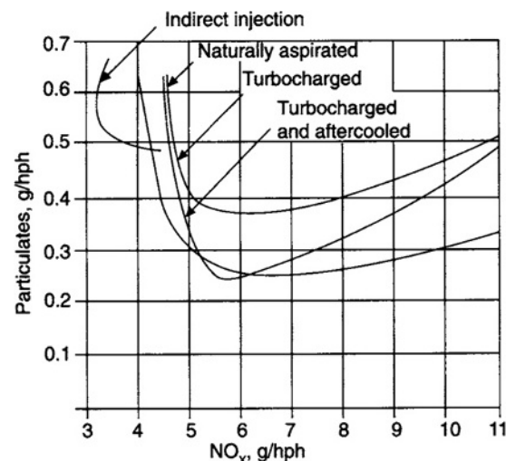
Fig. 3.1-20 Tests done in the late 1980s to demonstrate how NO x increases when measures are taken to reduce particulates in different types of engine.
