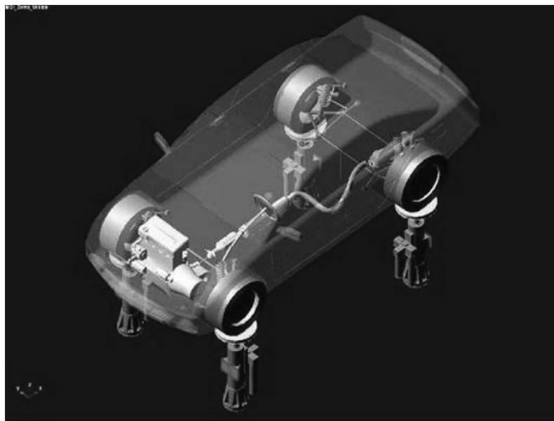
Fig. 15.1-2 A detailed multibody systems vehicle model (provided courtesy of MSC.Software).
