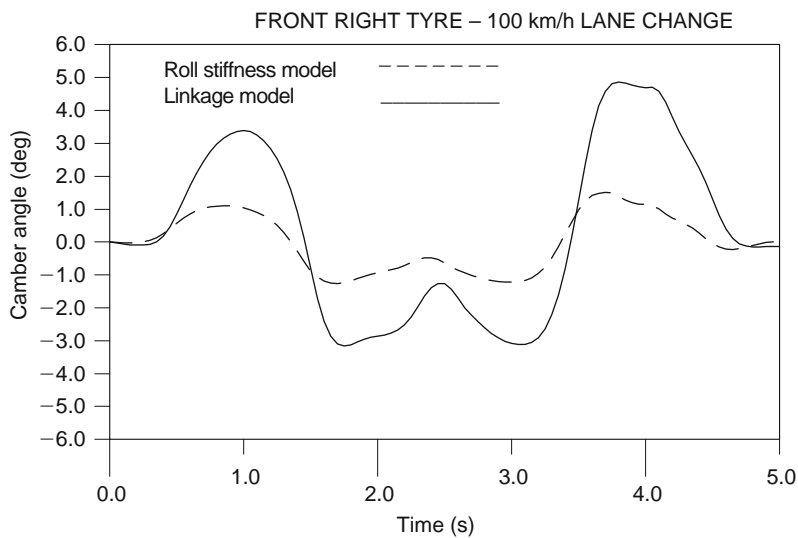
Fig. 15.1-60 Camber angle comparison – linkage and roll stiffness models.
