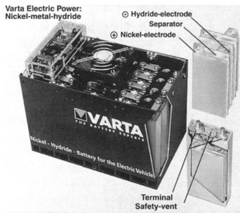
Fig. 6.1-3 Nickel–metal hydride battery.
