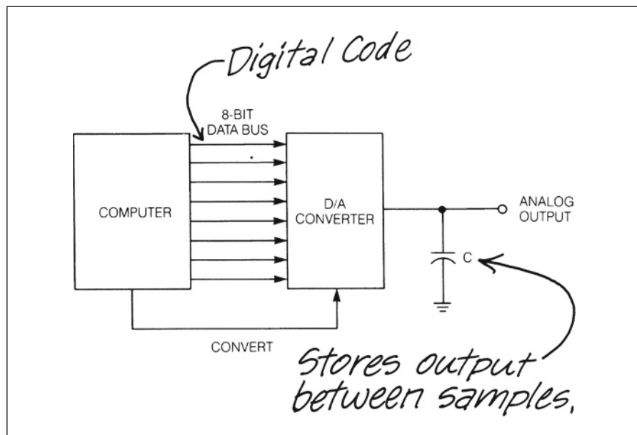
Fig. 23.1-4 Digital-to-analog conversion.
