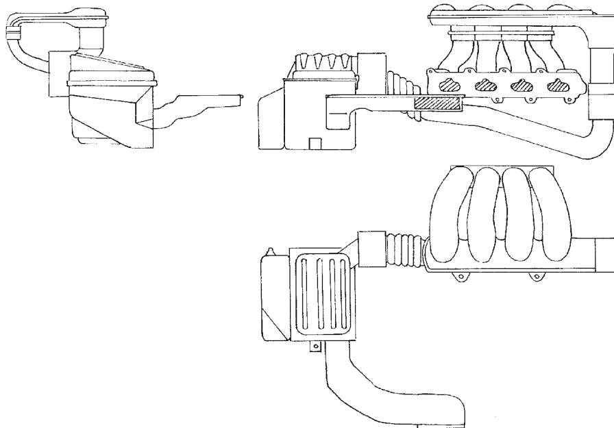
Fig. 22.1-41 An intake system where the design has been optimised using linear acoustic theory.
