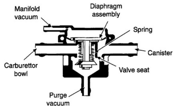
Fig. 3.1-17 The Rochester type 1 canister control valve functions as a simple vapour vent valve.
