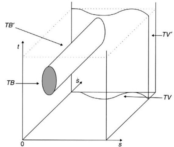
Fig. 14.2-24 ST ; the state-time space of \mathcal{A} .
