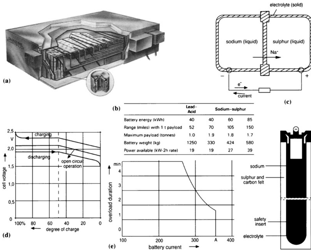
Fig. 6.1-2 Sodium-sulphur battery: (a) battery assembly; (b) projected performances; (c) ABB s-s cell; (d) energy capability; (e) overload capability.
