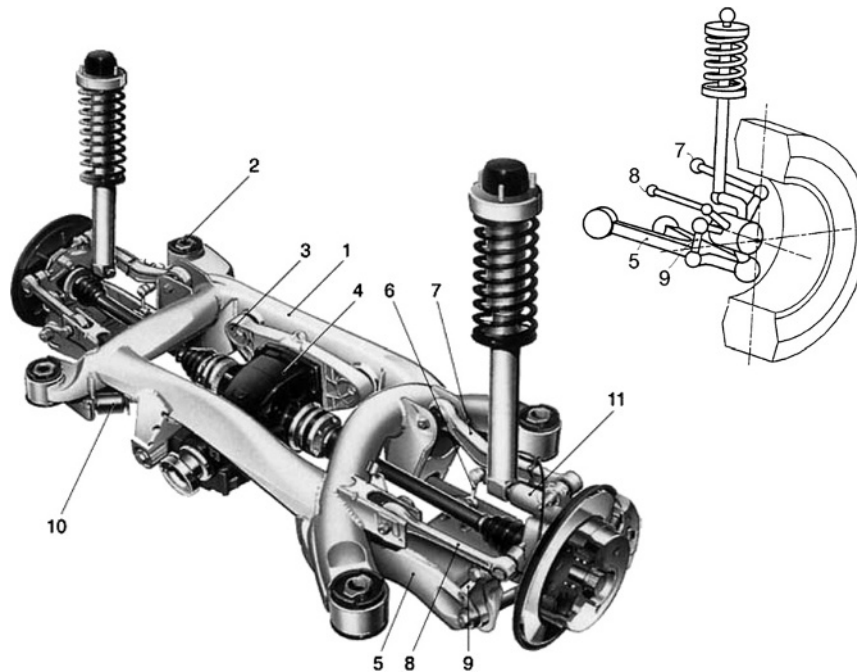
Fig. 8.1-19 Multi-link rear suspension of the BMW 5 series (E39, 1996). For the first time in large-scale car production, mainly aluminium is used for the suspension system derived from the geometry of the BMW 7 series. The subframe (rear-axle support) (1), produced from welded aluminium tubes, is attached to the bodywork by means of four large rubber mounts (2). These are soft in a longitudinal direction for the purposes of riding comfort and noise insulation and rigid in a transverse direction to achieve accurate wheel control. The differential gear also has compliant mounts (3). The wheel carrier is mounted on a U-shaped arm (5) at the bottom and on the transverse link (7) and inclined guide link (8) at the top. As a result of this inclined position, an instantaneous centre is produced between the transverse link and guide link outside the vehicle which leads to the desired brake understeer during cornering and the elastokinematic compensation of deformation of the rubber bearings and components. The driving and braking torque of the wheel carrier (11) is borne by the 'integral' link (9) on the swinging arm (5), which is subject to additional torsional stress as a result. This design makes it possible to ensure longitudinally elastic control of the swinging arm on the guide bearing (10) for reasons of comfort, without braking or driving torque twisting the guide bearings as would be the case with torque borne by pairs of longitudinal links. The stabilizer behind presses on the swinging arm (5) by means of the stabilizer link (6), whereas the twin-tube gas-pressure shock absorber, whose outer tube is also made of aluminium, and the suspension springs provide a favourably large spring base attached directly to the wheel carrier (11). For reasons of weight, the wheel discs are also made of aluminium plate. The wheel carrier is made of shell cast aluminium. The rear axle of the station wagon BMW Tourer is largely similar in design. However, the shock absorber extends from the U-shaped swinging arm in order to allow for a wide and low loading area.
