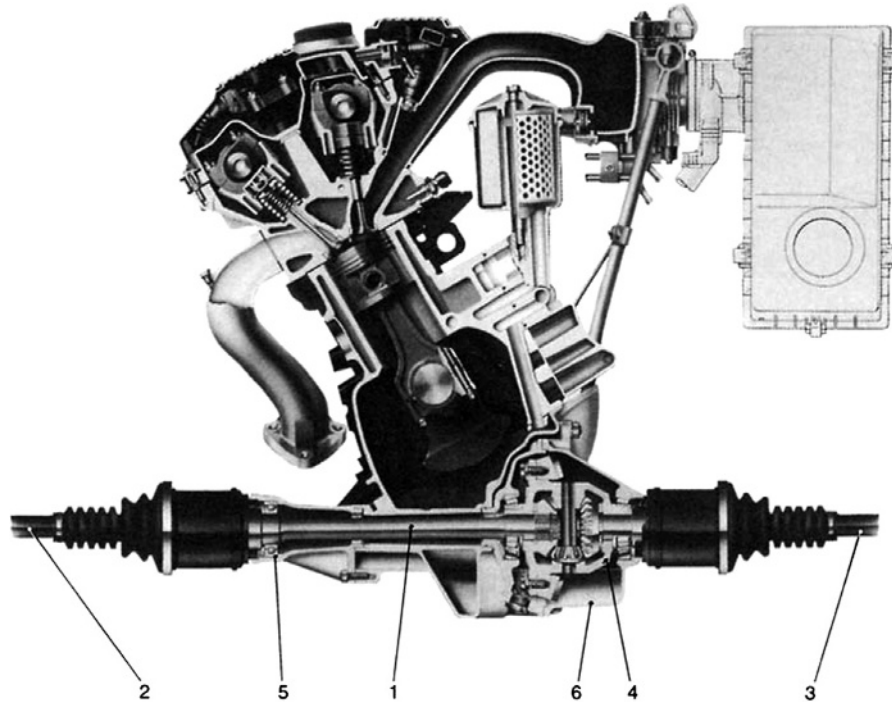
Fig. 8.1-80 Front cross-section view of the engine; and drive axle of a standard four-wheel-drive vehicle (BMW assembly diagram). The basic vehicle has rear-wheel drive and, in order to also be able to drive the front wheels, the front axle power take-off 4 had to be moved into the space of the oil pan. The intermediate shaft 1 bridges the distance to the right inner CV joint and thus ensures drive shafts of equal length to both wheels (items 2 and 3 and Fig. 8.1-51). Part 1 is mounted on one side in the non-lockable differential 4 and on the other side in the outrigger 5. This, and the casing 6, are screwed to the oil pan.
