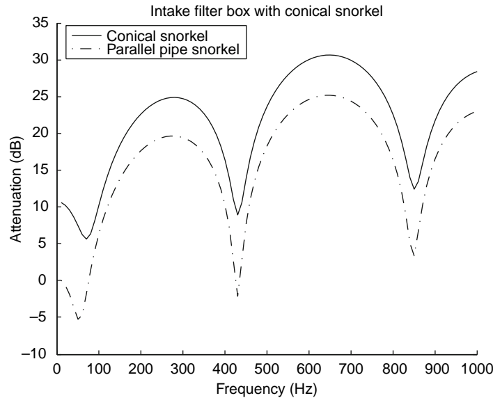
Fig. 22.1-32 Effect of adopting a conical snorkel. Calculated using APINEX software.
