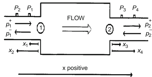
Fig. 22.1-28 Inlet and outlet acoustic fields in a silencer element.
