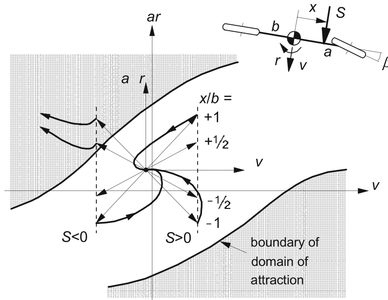
Fig. 11.1-25 Large disturbance in a curve. New initial state vector ( \Delta v , \Delta r ) after the action of a lateral impulse S . Once outside the domain of attraction the motion becomes unstable and may get out of control.
