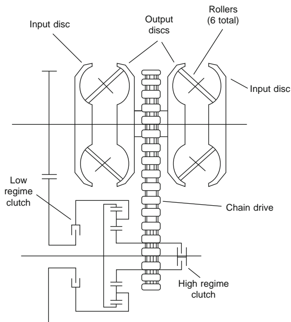
Fig. 5.1-33 Torotrak transmission schematic layout.
