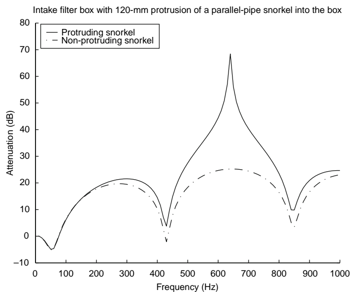
Fig. 22.1-33 Effect of protruding the snorkel into the filter box. Calculated using APINEX software.
