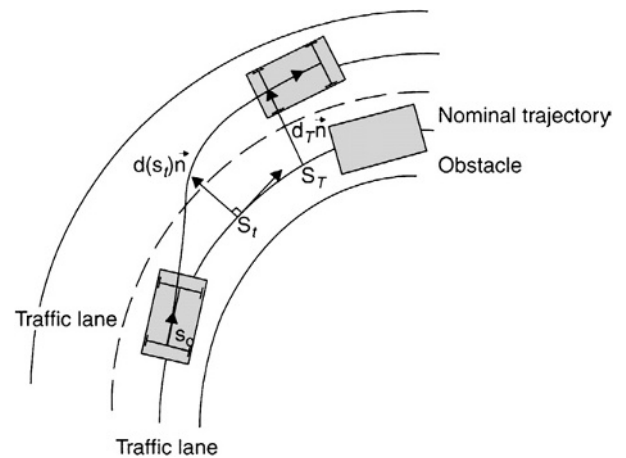
Fig. 14.2-14 Generation of smooth local trajectories to avoid an obstacle.
