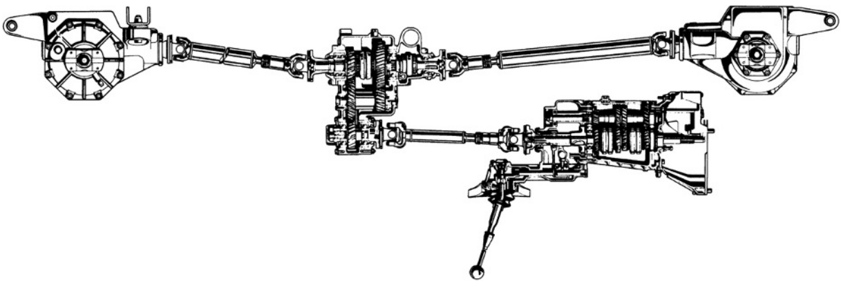
Fig. 8.1-70 Complex power distribution on the Fiat Campagnolo, a four-wheel drive, all-purpose passenger car. The drive moment is transferred from the manual gearbox via a centrally located two-gear power take-off gear to the differentials of the front and rear axles. Efficiency is not likely to be especially good.
