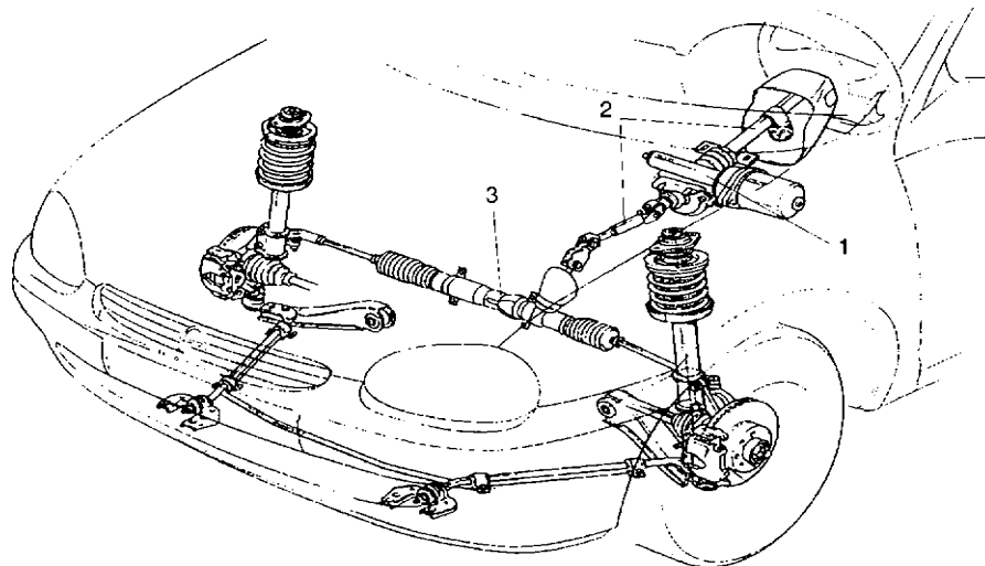
Fig. 9.1-23 Electric power steering system of the Opel Corsa (1997). The individual components are:
