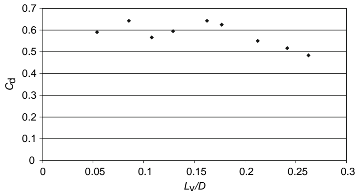
Fig. 22.1-7 Discharge coefficients with respect to reference area given by equation (22.1.50) for the case of inflow through the intake valve (Annand and Roe, 1974).
