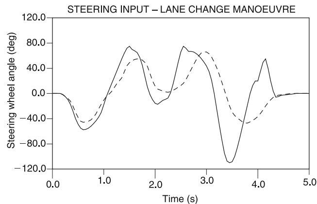
Fig. 15.1-42 Steering input for the lane change manoeuvre at 70 km/h (dashed line) and 100 km/h (solid line).
