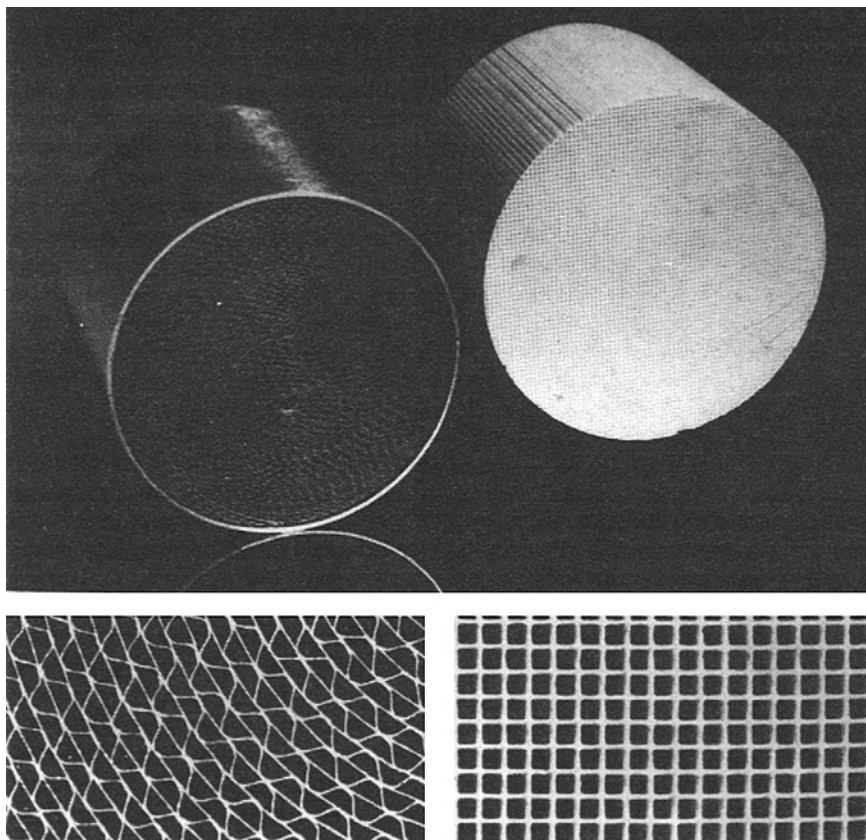
Fig. 3.1-5 Comparison between ceramic and metallic monoliths. The thermal stresses in monoliths comprising alternate strips of plain and corrugated metal foil in looped S-form are considerably lower than those that are simply spirally wound.
