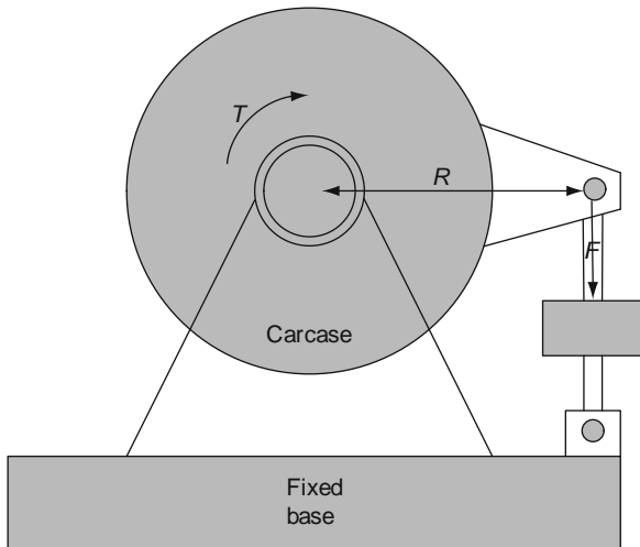
Fig. 2.1-2 Diagram of trunnion-mounted dynamometer measuring torque with a load cell.
