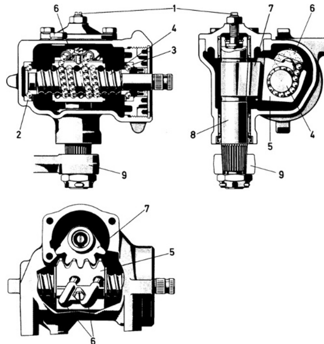
Fig. 9.1-15 Mercedes Benz recirculating ball steering suitable for passenger cars and light vans; today, apart from in a few exceptional cases, this is only fitted as a hydraulic power-assisted version. Pitman arm 9 is mounted onto the tapered toothed profile with a slotted castle nut 11 (Fig. 9.1-24).
