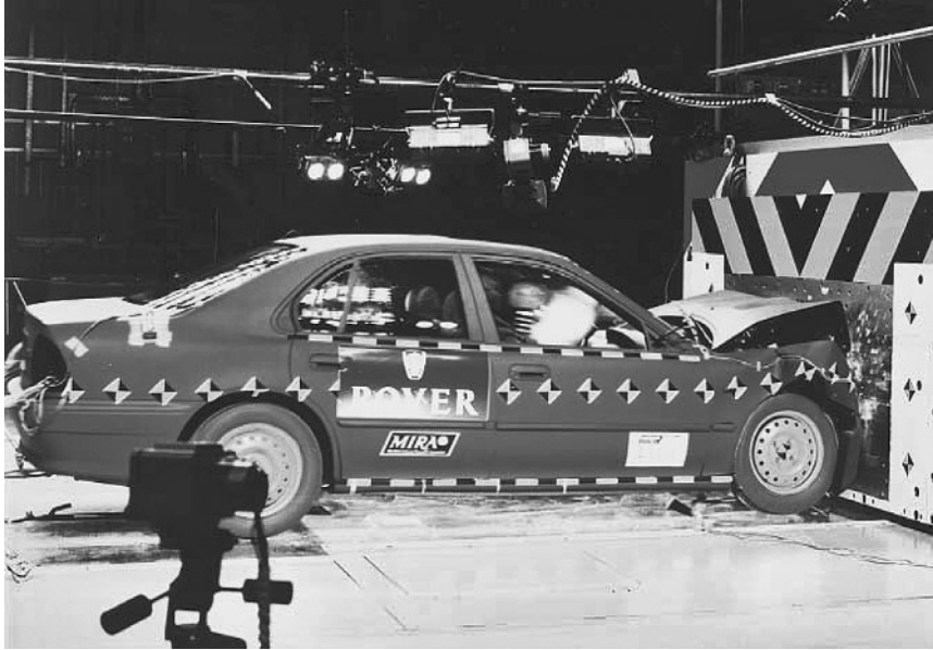
Fig. 17.1-2 For conventional frontal impact tests, the impacted face of the concrete block can be protected with steel plate to reduce the rate of erosion.
