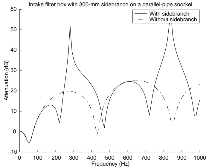
Fig. 22.1-37 The effect of adding a sidebranch resonator calculated using APINEX software.
