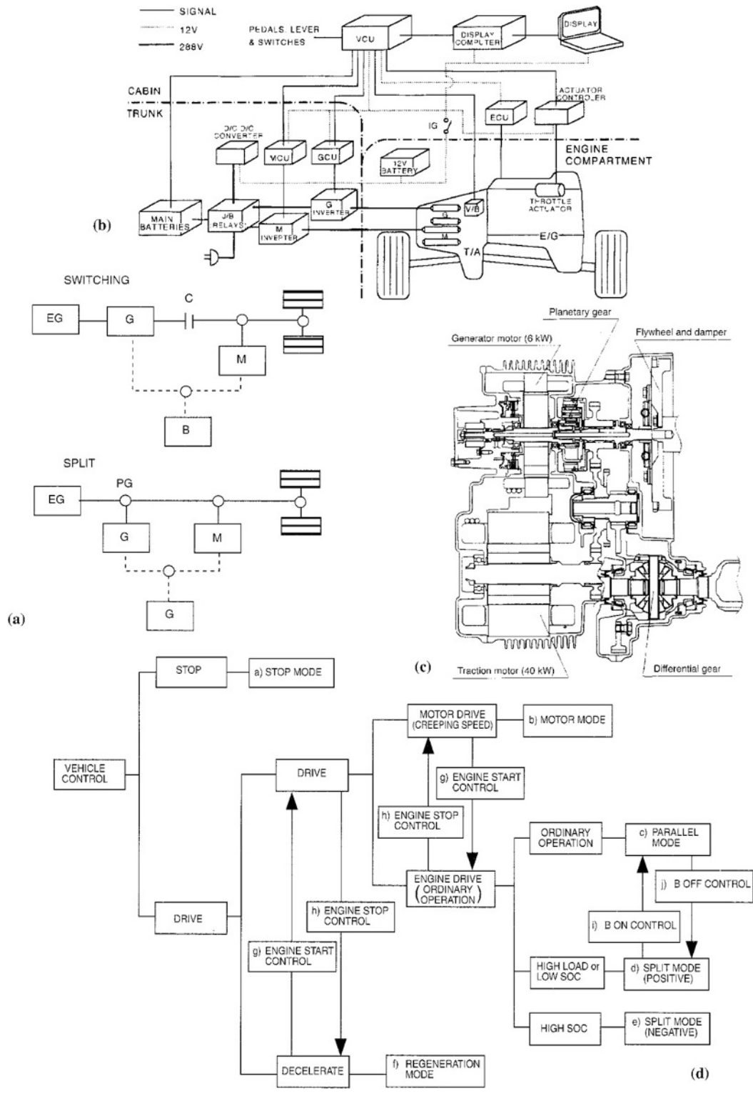
Fig. 7.1-11 Dual system: (a) comparison of switching and split series/parallel hybrid drives, full line is mechanical connection and dotted line electrical; (b) hybrid system; (c) transaxle configuration; (d) control strategy).
