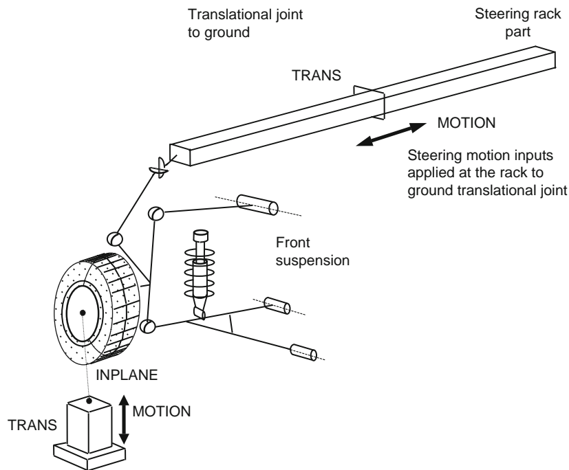
Fig. 15.1-39 Front suspension steering ratio test model.
