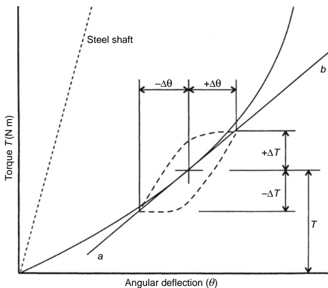
Fig. 2.1a-9 Dynamic torsional characteristic of multiple bush type coupling.
