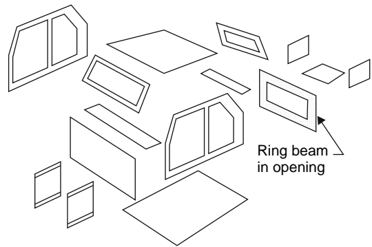
Fig. 16.2-19 Ring frame to remedy faux sedan problem.
