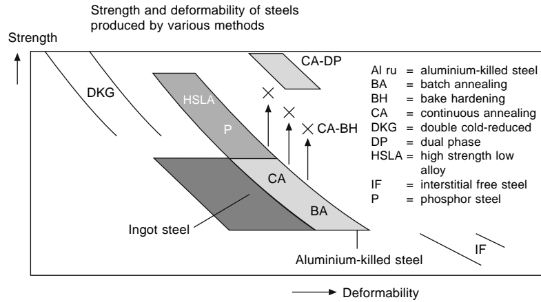
Fig. 18.2-1 Range of flat rolled steel products. (Courtesy of Corus.)
