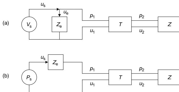
Fig. 22.1-16 Acoustic circuits for flow ducts. (a) Excitation by a fluctuating mass or volume velocity, (b) Excitation by fluctuating pressure or aerodynamic force (after Davies (1996)).
