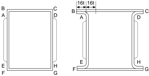
Fig. 17.1-14 Sections through two box section frame side members, one tubular and the other fabricated. Although the swages in their sides weaken them so far as taking side loads is concerned, these loads can be taken mainly in the sections ABCD and EFGH. A useful rule of thumb is that a length equal to 16 multiplied by the thickness of the metal represents the maximum length that is stable on each side of each angle under compression, the measurement being taken from the inner face in each corner or, for the fabricated section, the centres of the bends.
