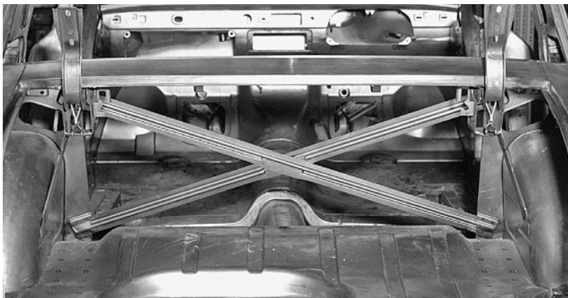
Fig. 16.2-13 Rear seat aperture with diagonal braces (courtesy Vauxhall Heritage Archive).
