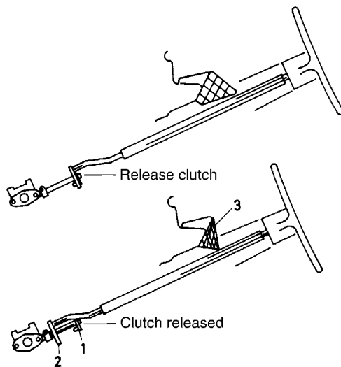
Fig. 9.1-29 'Release clutch' used by VW on steering columns. A half-round plate sits on the short shaft that is linked to the steering pinion gear, and carries the two pins 1 which point downwards. They grip into the two holes of the clutch 2 sitting on the steering tube from the top. The jacket tube is connected to the dashboard via a deformable bracket. As shown in a head-on crash, this part 3 flexes and the pins 1 slide out of part 2.
