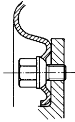
Fig. 10.1-26 Depression design with special springing characteristics on a passenger car sheet metal disc-type wheel. The wheel can be centred using the fixing bolts or by fitting into the tolerated hole (Fig. 10.1-24).
