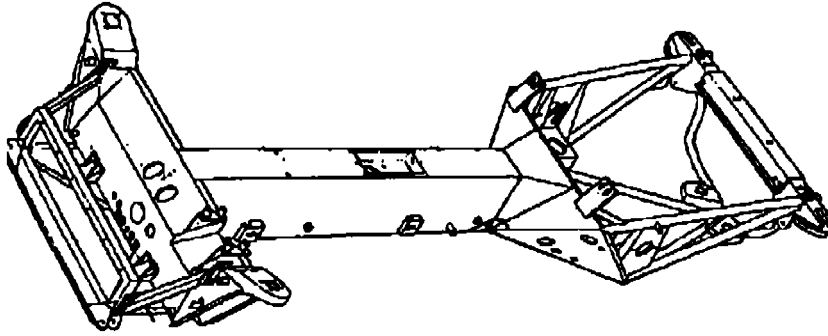
Fig. 16.1-14 Sheet steel backbone chassis (courtesy Lotus Cars Ltd).
