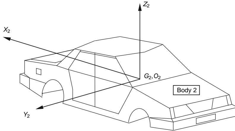
Fig. 15.1-3 Vehicle body reference frame.
