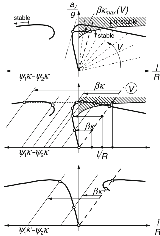
Fig. 11.1-20 Construction of stability boundary (upper diagram, from Fig. 11.1-17). On the isolated branch, a stable range may occur (large steer angle as indicated in middle diagram). The lower diagram shows the case with complete understeer featuring a stable main branch.
