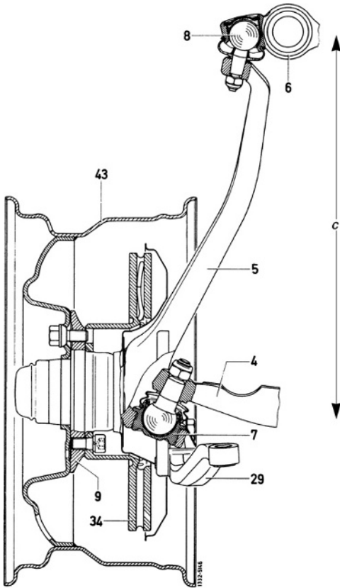
Fig. 8.1-38 Front hub carrier (steering knuckle) on the Mercedes-Benz S class (W40, 1997) with a large effective distance c (see also Fig. 8.1.4). The upper transverse control arm 6 forms the casing for the ball pivot of the guiding joint, whereas the lower supporting joint 7 is pressed into the hub carrier 5. The ventilated brake disc 34 (dished inwards), the wheel hub 9, the double-hump rim 43 with asymmetrical drop centre and the space for the brake caliper (not included in the picture) are clearly shown.
