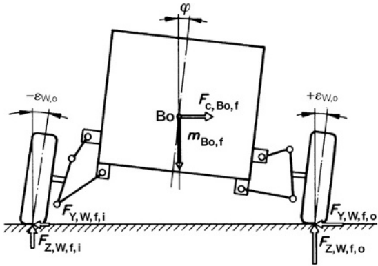
Fig. 8.1-6 If the body inclines by the angle \varphi during cornering, the outer independently suspended wheel takes on a positive camber \varepsilon_{w,o} and the inner wheel takes on a negative camber \varepsilon_{w,i} . The ability of the tyres to transfer the lateral forces F_{Y,W,f,i} or F_{Y,W,f,o} decreases causing a greater required slip angle Equation 10.1.16, m_{Bo,f} is the proportion of the weight of the body over the front axle and F_{c,Bo,f} the centrifugal force acting at the level of the centre of gravity B_o . One wheel rebounds and the other bumps, i.e. this vehicle has 'reciprocal springing', that is:
