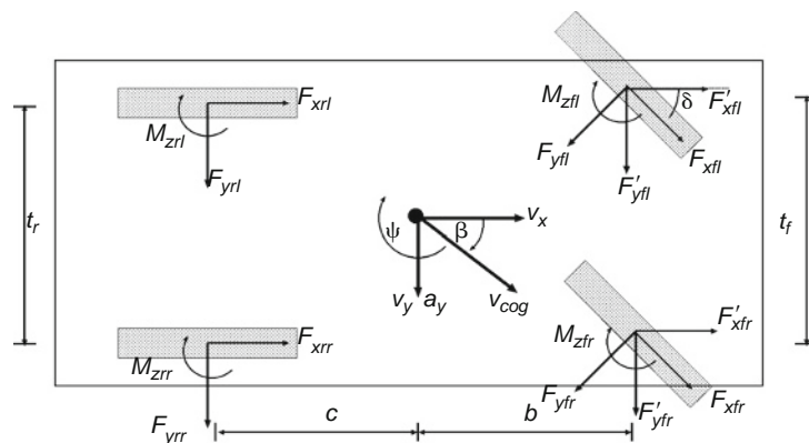
Fig. 15.1-62 Three-degree-of-freedom vehicle model.
