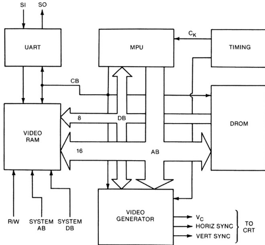
Fig. 23.1-23 CRT-type controller configuration.
