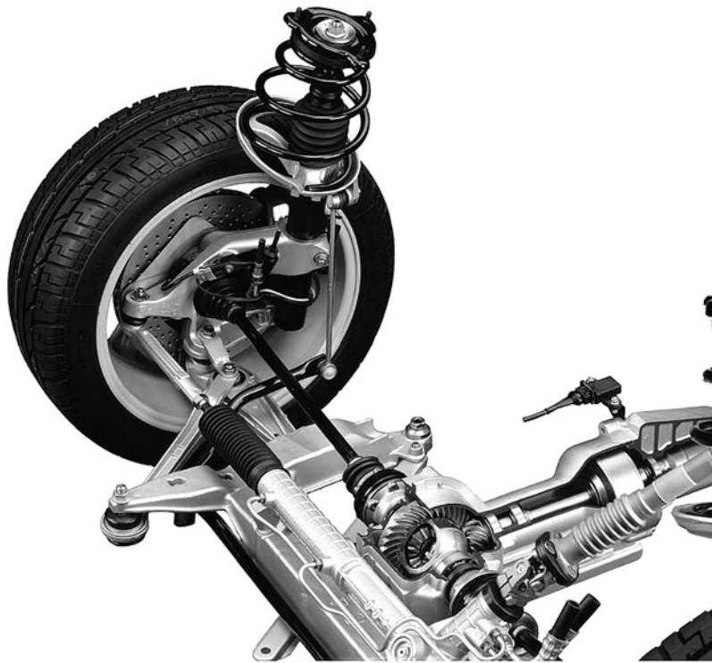
Fig. 8.1-75 Driven front axle of the Porsche 911 Carrera 4 (1996, 1998). The visco clutch is flange mounted directly on the front axle to achieve a better distribution of axle load. With corresponding slip of the rear wheels, up to 40% of the driving torque is transmitted to the front axles. Particular attention was paid during the adjustment of the four-wheel drive to predictable self-steering properties independent of drive distribution and to controllability of the handling characteristics even at the stability limit. Instead of differential locks, specific wheel brake engagements are made in order to retard spinning wheels. Four-wheel drive is integrated into the Porsche Stability Management (PSM), a system for controlling the dynamics of vehicle movement with brake actuation.
