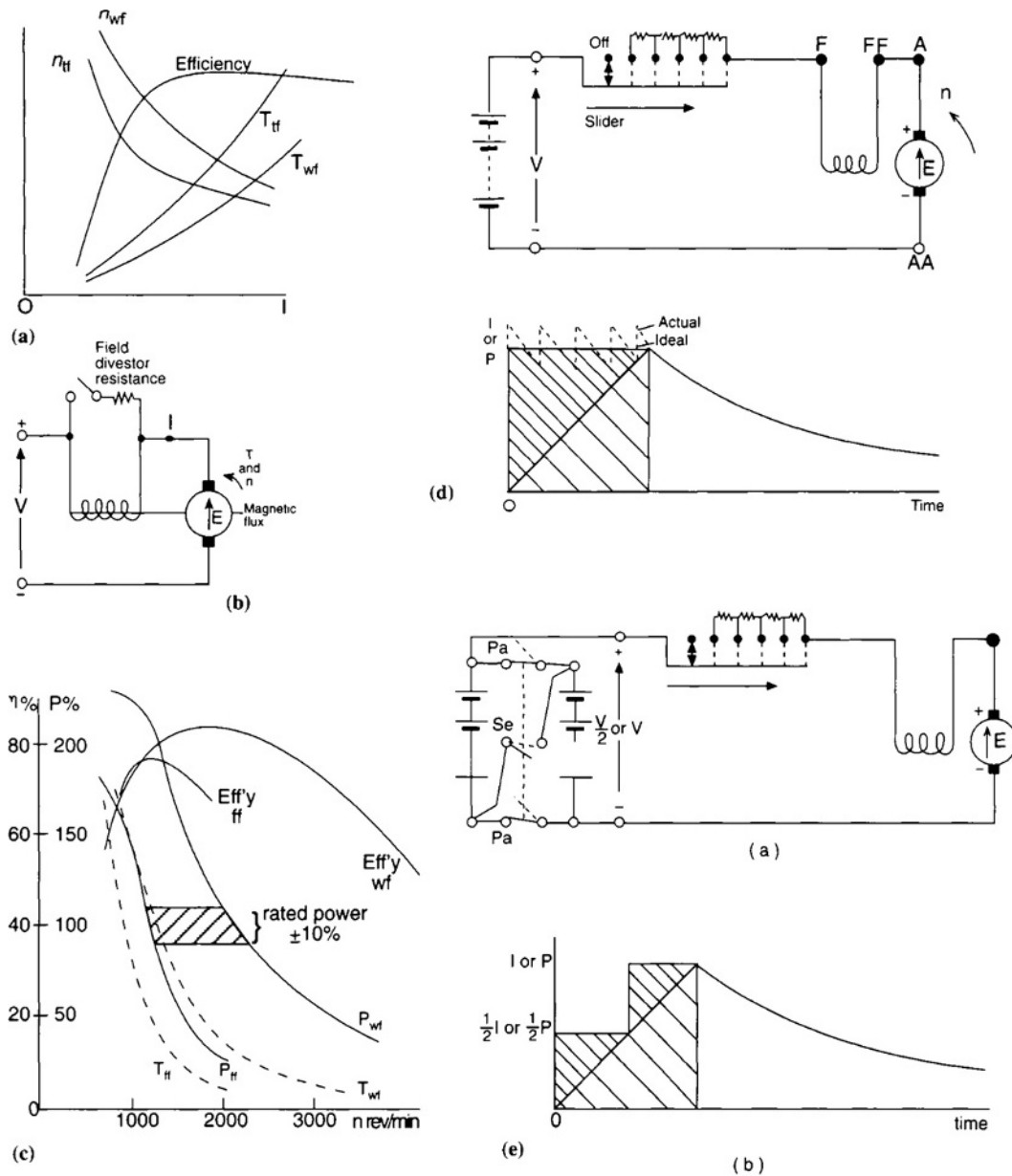
Fig. 6.1-9 Series-wound DC motor: (a) motor characteristics; (b) field diverter resistance; (c) speed-base motor characteristics; (d) rheostatic control; (e) parallel/series battery control.
