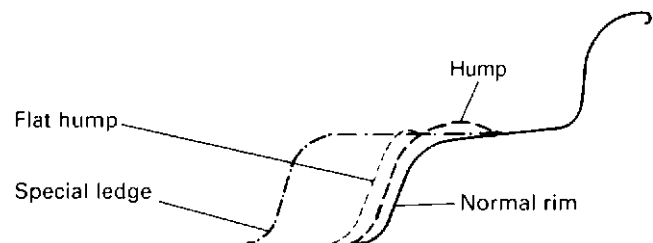
Fig. 10.1-21 Standard rim and contours of the safety shoulders which can be used on passenger cars and light commercial vehicles.
