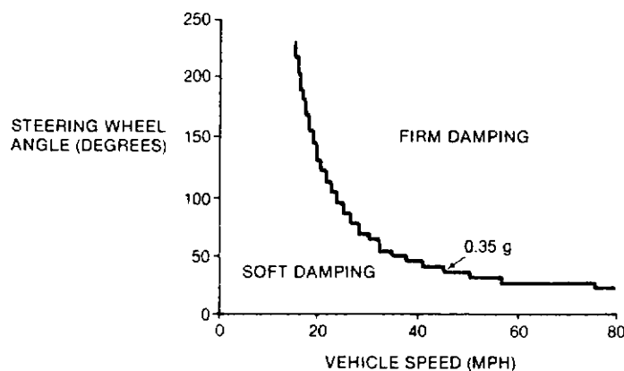
Fig. 13.1-19 Switching threshold versus speed and steering inputs.
