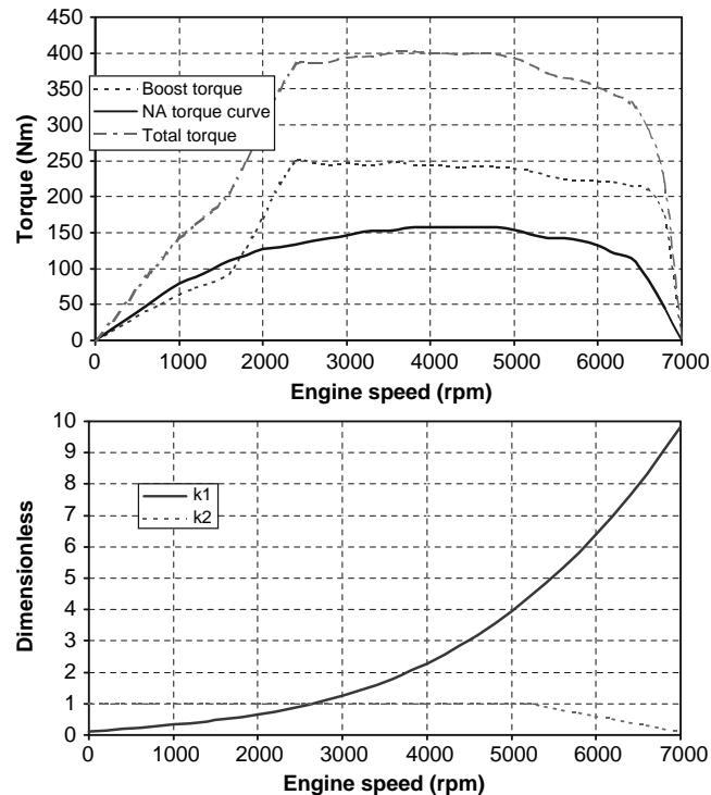
Fig. 15.1-35 Empirical mean-state turbocharger model.
