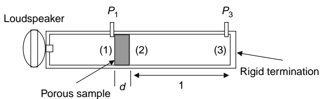
Fig. 21.1-10 Impedance tube method for measuring flow resistivity: after Ingard and Dear (1985).
