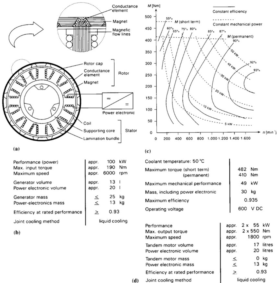
Fig. 7.1-8 Advanced PM motor system: (a) trapezoidal iron conductors; (b) motor performance; (c) motor curve; (d) target performances.
