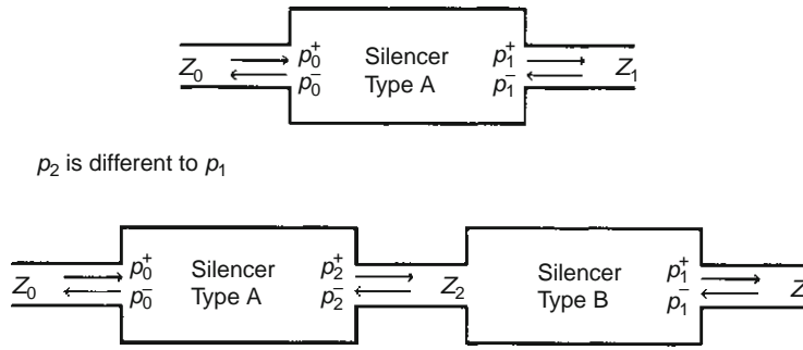
Fig. 22.1-27 The interacting sound fields in a twin-silencer exhaust system.
