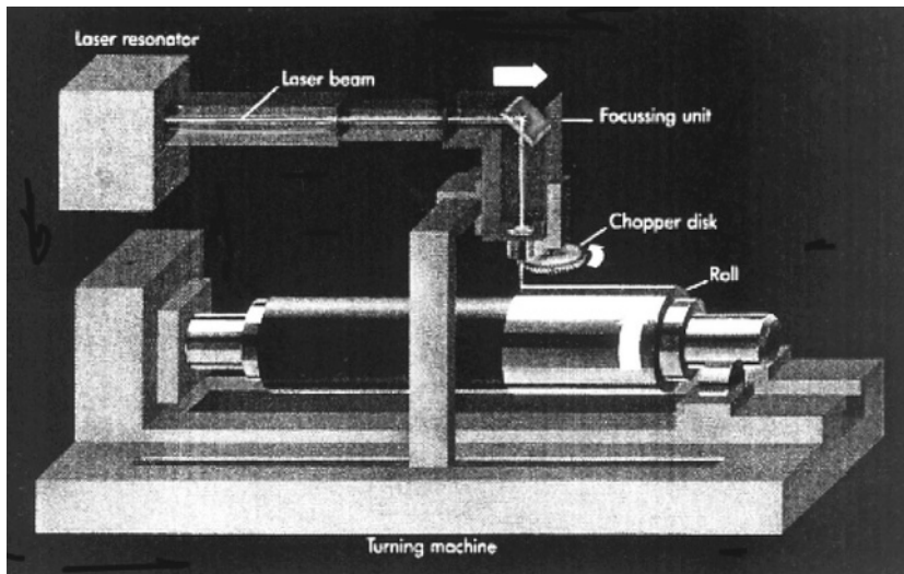
Fig. 18.2-10 Principle of the Lasertex method of roll texturing.
