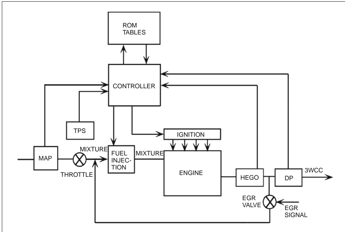
Fig. 4.1-4 Engine control system using the speed-density method.
