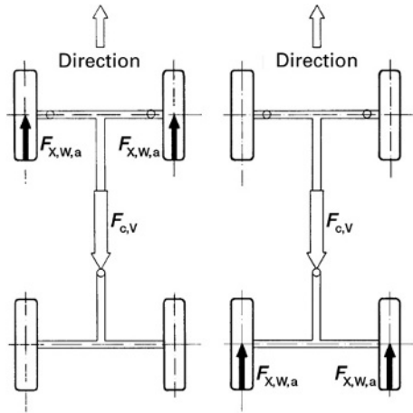
Fig. 8.1-35 On a front-wheel drive (left) the vehicle is pulled. The result is a more stable relationship between the driving forces F_{x,w,a} and the inertia force F_{c,v} . Conversely, in the case of driven rear wheels an unstable condition is theoretically evident; front axle settings ensure the necessary stabilization.
