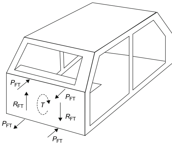
Fig. 16.2-10 Forces on dash panel.
