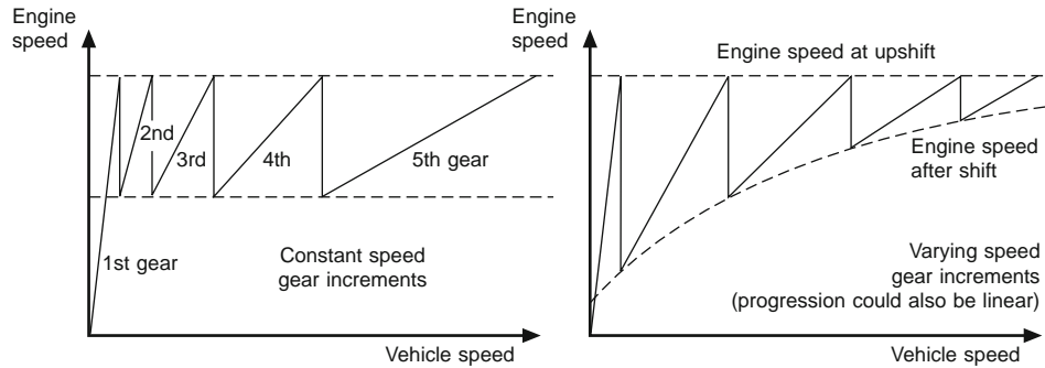
Fig. 5.1-3 Engine speed vs vehicle speed for differing gear ratio progressions.
