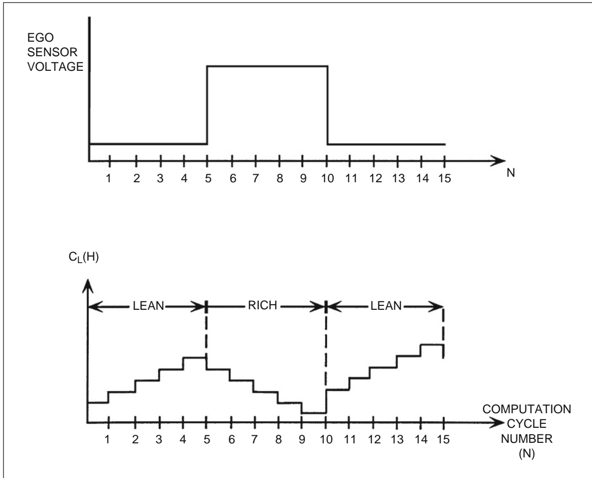
Fig. 4.1-6 Closed-loop correction factor.
