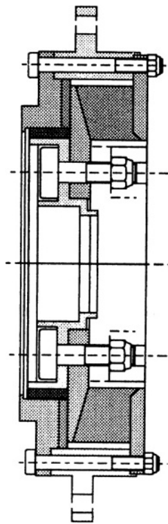
Fig. 2.1a-10 Annular type rubber coupling.
