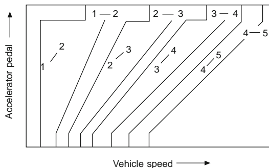
Fig.5.1-23 Shift strategy (courtesy of Jatco).
