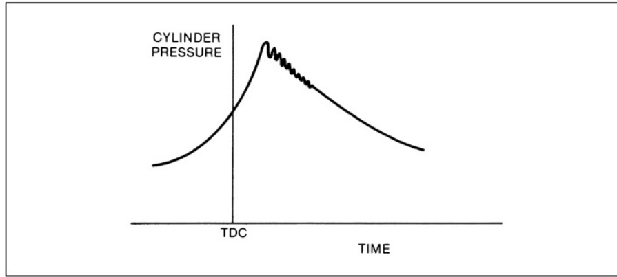
Fig. 4.1-11 Cylinder pressure (knocking condition).
