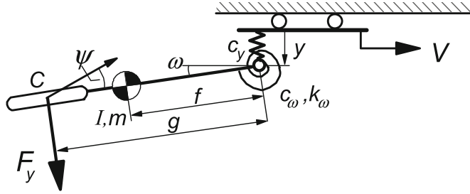
Fig. 11.1-31 On the stability of a trailer (Exercise 11.1.4).
