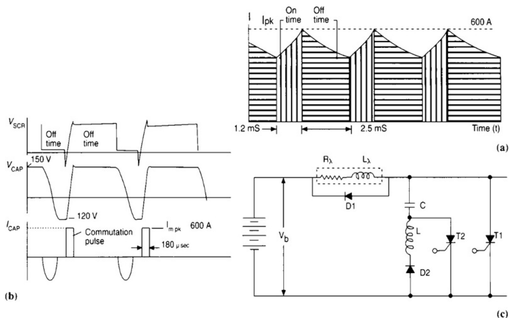
Fig. 6.1-20 Thyristor control: (a) controller pulses: (b) energy storage and reversal: (c) DC chopper circuit.
