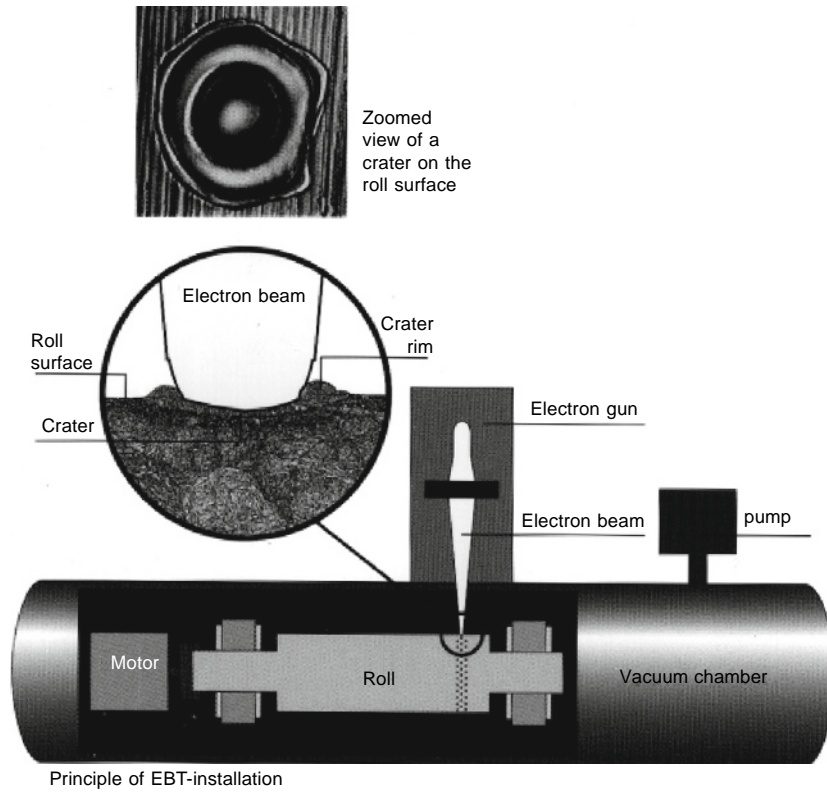
Fig. 18.2-11 Electron beam technology. (Courtesy Sidstahl.).
