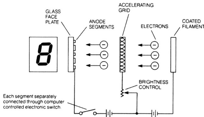
Fig. 23.1-18 Simplified vacuum-fluorescent display configuration.
