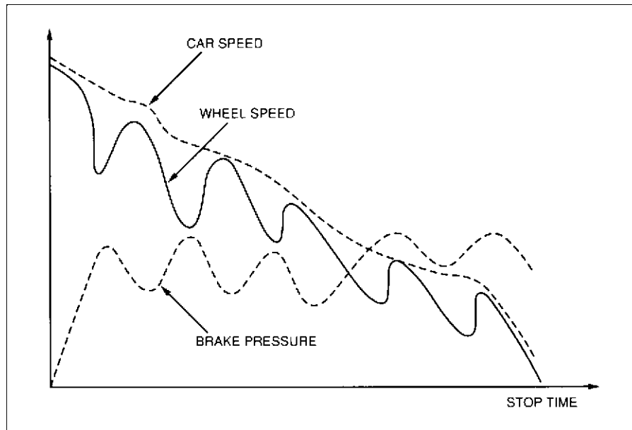
Fig. 13.1-17 ABS braking action.
