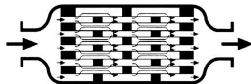
Fig. 3.1-25 Diagram showing how the gas flow is diverted in a particulate trap.
