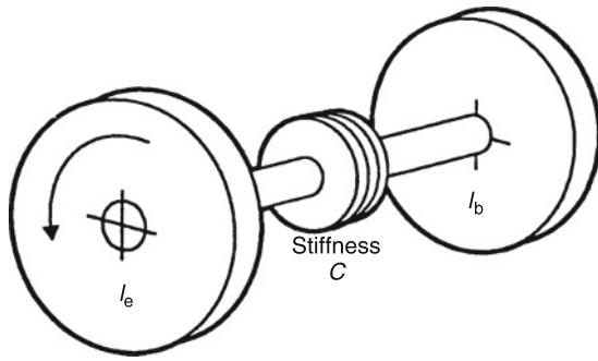
Fig. 2.1a-2 Two mass system (compare with Fig. 2.1a-1).
