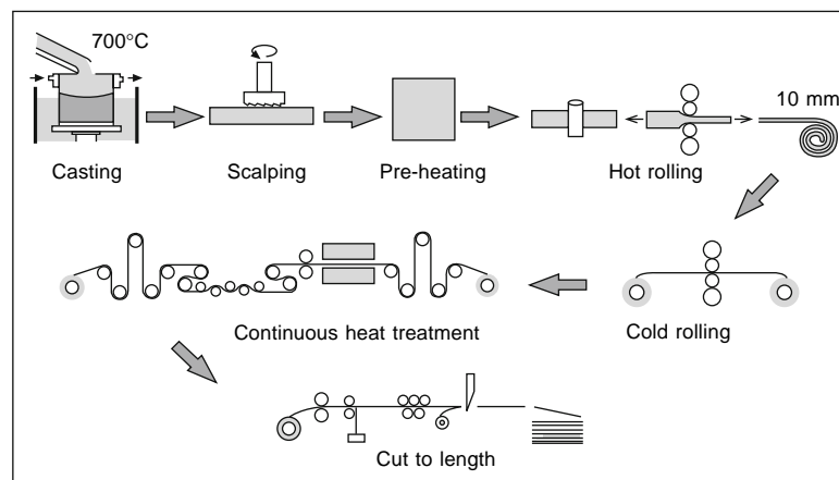
Fig. 18.2-14 Aluminium production process.
