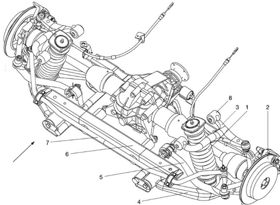
Fig. 8.1-82 Rear axle of the Mercedes-Benz off-road vehicle of the M series. Suspension and damping are ensured by the spring strut (1) whose spring is tapered for reasons of construction space (spring rate gradually increasing from 70 to 140 N/mm), 2 brake disc with integrated drum parking brake, 3 upper transverse link (forged aluminium component), 4 lower transverse link (forged aluminium component), 5 tie rod (forged steel component), 6 integral bearer (subframe), 7 stabilizer, 8 transverse link mounting points.
