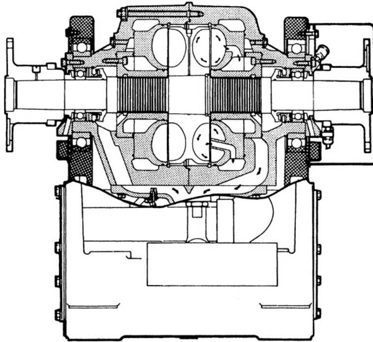
Fig. 2.1-11 Variable fill hydraulic dynamometer controlled by fast acting outlet valve at bottom of the stator.
