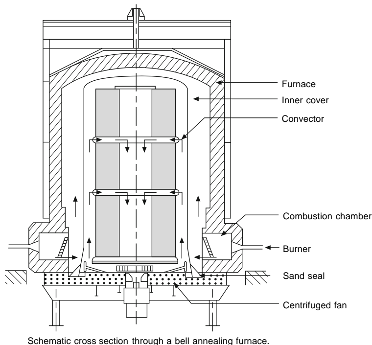
Fig. 18.2-6 Bell annealing furnace showing the vertical positioning of cold reduced coils.
