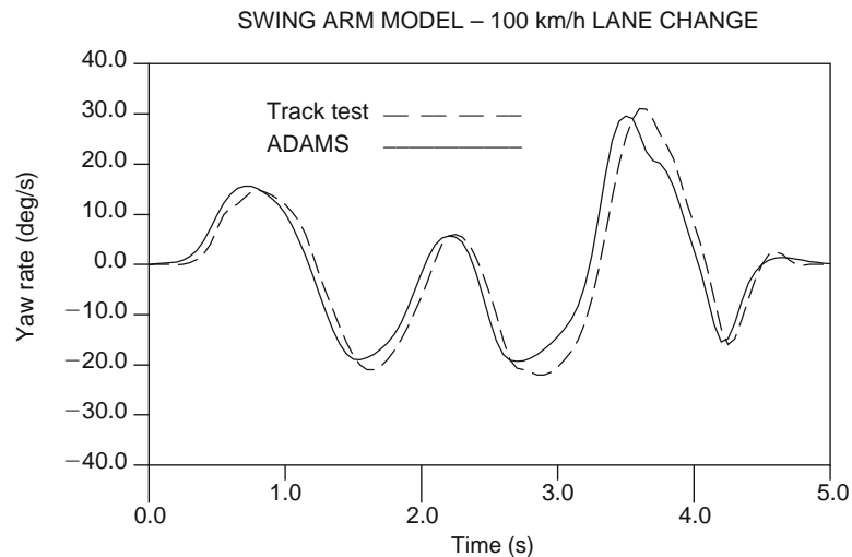
Fig. 15.1-54 Yaw rate comparison – swing arm model and test. (This material has been reproduced from the Proceedings of the Institution of Mechanical Engineers, K2 Vol. 214 ‘The modelling and simulation of vehicle handling. Part 4: handling simulation’, M.V. Blundell, page 80, by permission of the Council of the Institution of Mechanical Engineers.)
