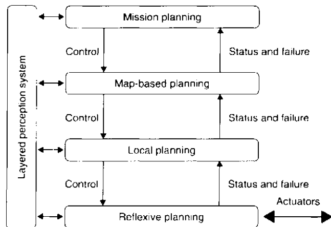
Fig. 14.2-3 Payton's architecture.
