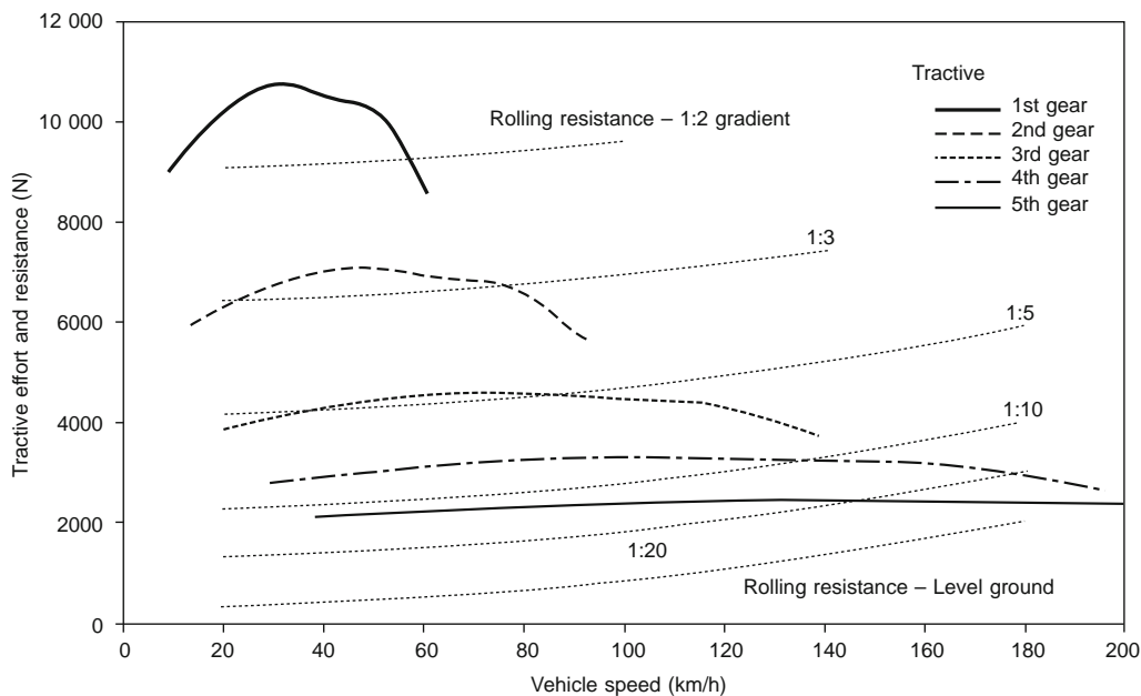
Fig. 5.1-5 Graph of tractive effort and rolling resistance vs road speed.
