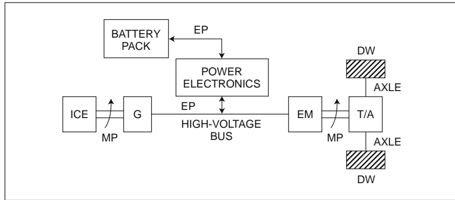
Fig. 4.1-20 SHV representation.
