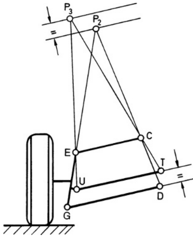
Fig. 9.1-45 Suspension control arms, which are parallel to one another in the design position of the vehicle, have to have a tie rod in the same position.
