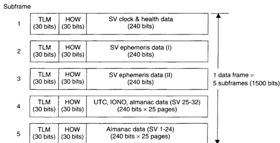
Fig. 14.1-1 Navigation message. TLM, telemetry word; HOW, handover word.
