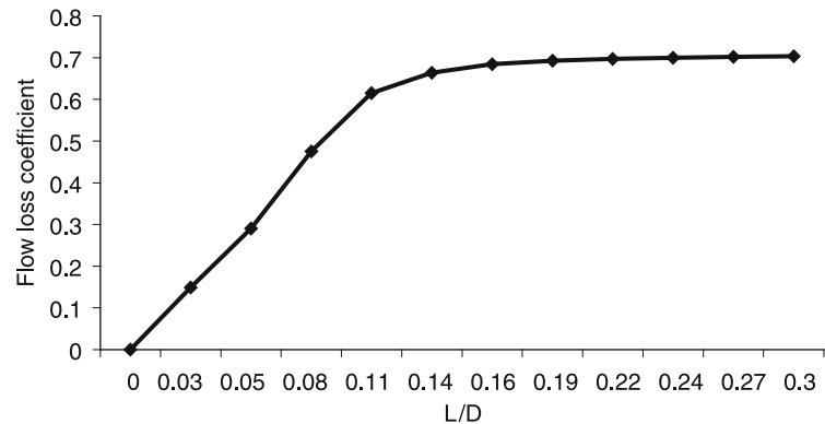
Fig. 22.1-9 Exhaust port flow loss coefficient (AVL, 2000).
