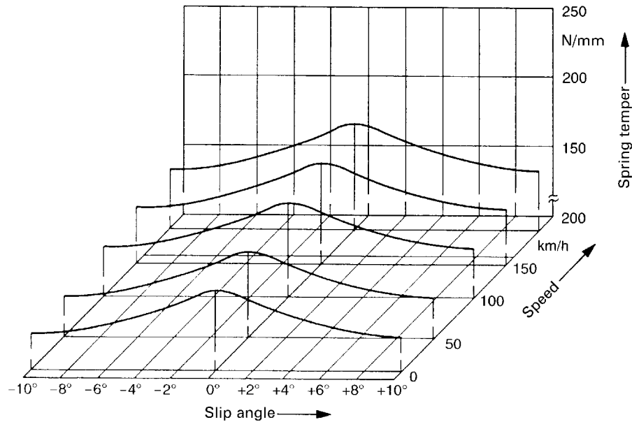
Fig. 10.1-28 Tyre springing rate as a function of slip angle and road speed, measured on a radial tyre 185/70 R 13 86 S at p_T = 2.1 bar. Speed increases the springing rate as the belt stands up due to the centrifugal force. However, the slip angle makes it softer because the belt is pushed away to the side and the shoulders take over part of the springing effect.
