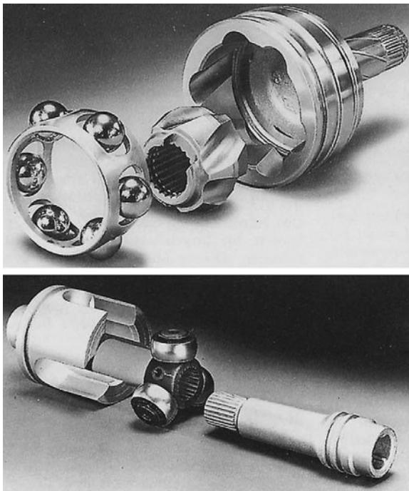
Fig. 8.1-17 Constant velocity sliding joints by GKN Automotive. In front-drive vehicles, considerable articulation angles of the drive axles occur, sometimes even during straight running, as a result of the installation situation, short propshafts and lifting movements of the body due to torque steer effects. These result in force and moment non-conformities and losses which lead to unwanted vibration. The full-load sliding ball joint
