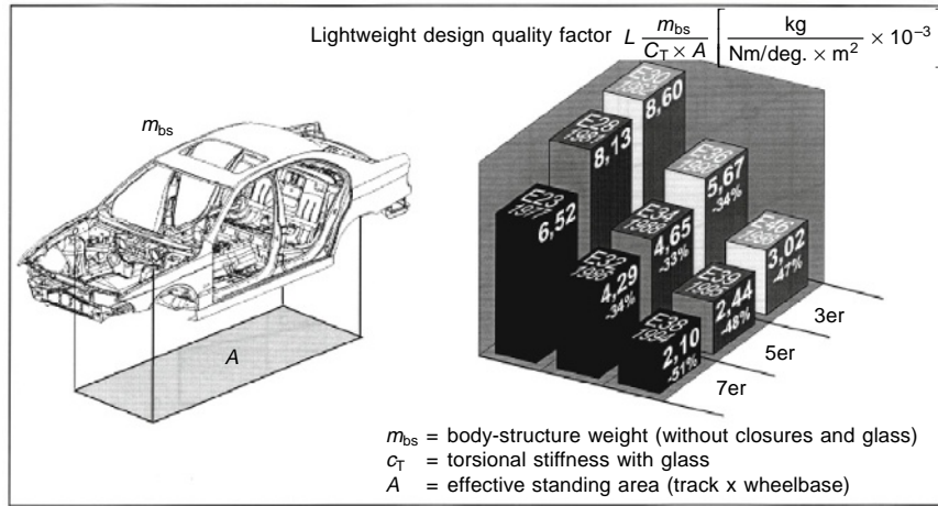
Fig. 18.1-15 Design efficiency as defined by functional optimization and size, over three generations of vehicles. 6
