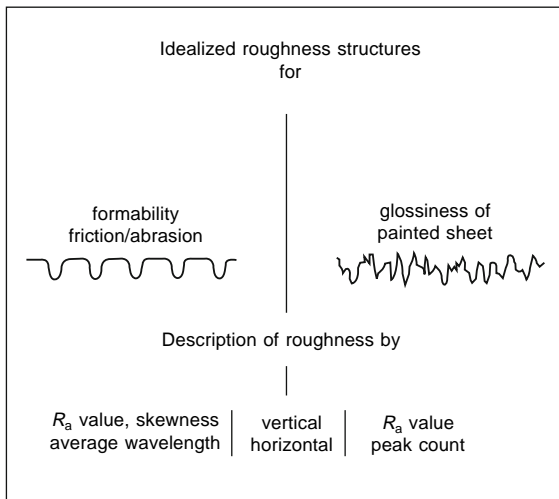
Fig. 18.2-8 Surface roughness profiles suited to forming and painting.
