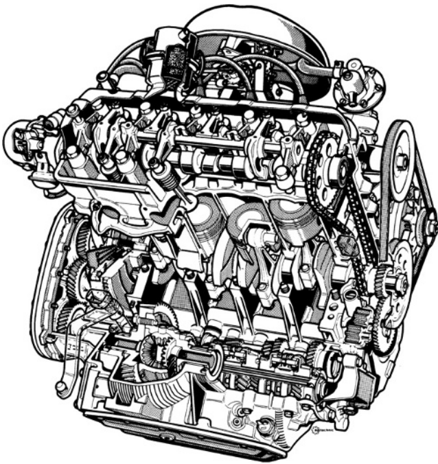
Fig. 8.1-52 Arrangement of the gearbox beneath the motor, which is inclined towards the rear, and the differential gear placed behind it. A single oil-economy undertakes the supply, in this case, of the driving unit, narrow in its design (Works Illustr. Fa Peugeot).
