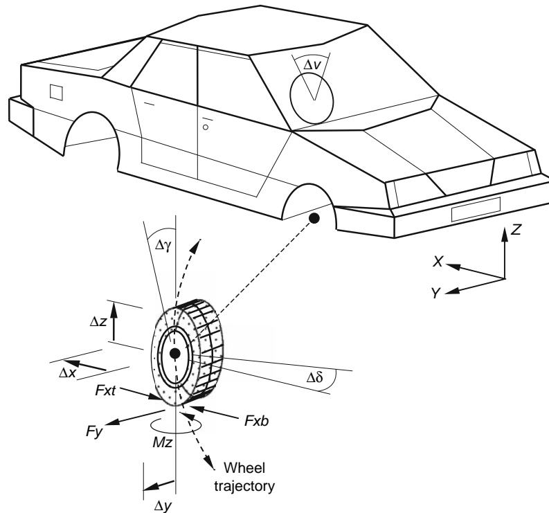
Fig. 15.1-12 Concept suspension system model schematic.
