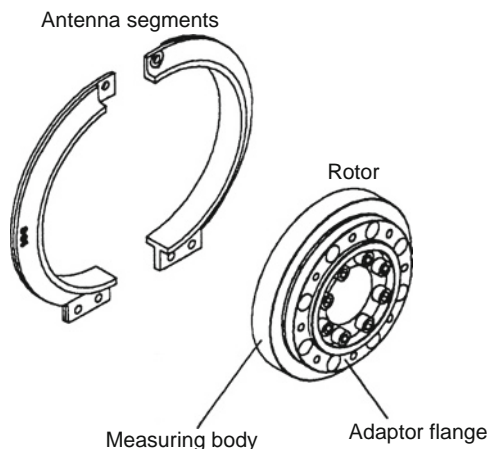
Fig. 2.1-5 Shaft-line components of a torque flange.
