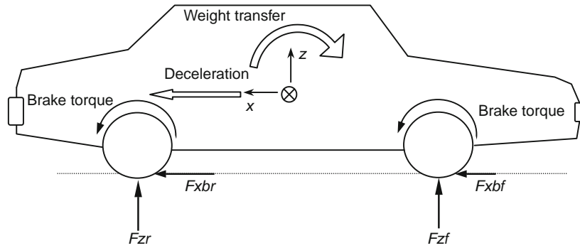
Fig. 15.1-26 Braking of a full vehicle.
