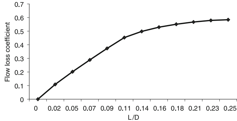
Fig. 22.1-8 Intake port flow loss coefficient (AVL, 2000).
