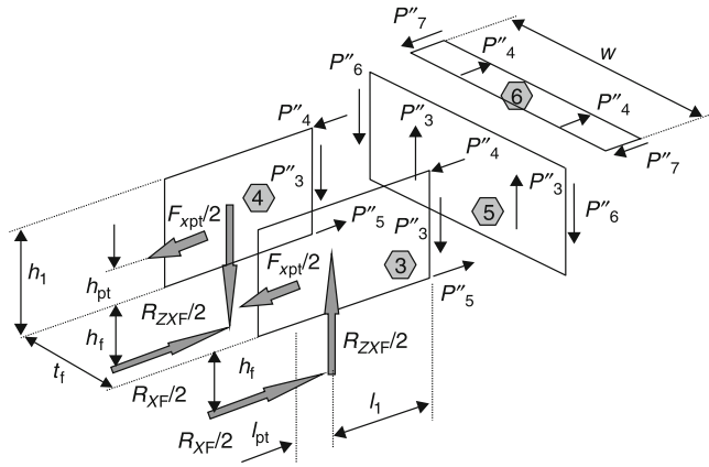
Fig. 16.2-31 Baseline model (front structure) – braking loads.
