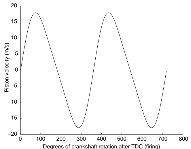
Fig. 22.1-11 Piston velocity, 4000 rev min -1 .
