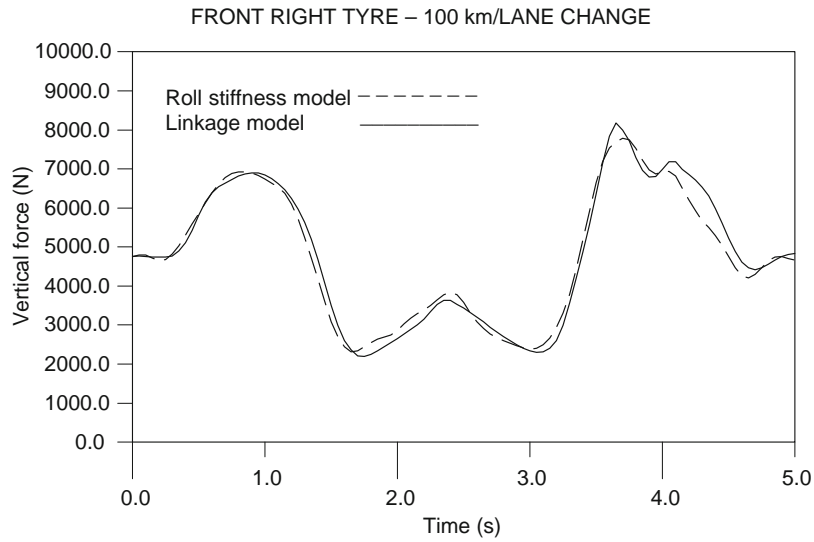
Fig. 15.1-57 Vertical tyre force comparison – linkage and roll stiffness models.
