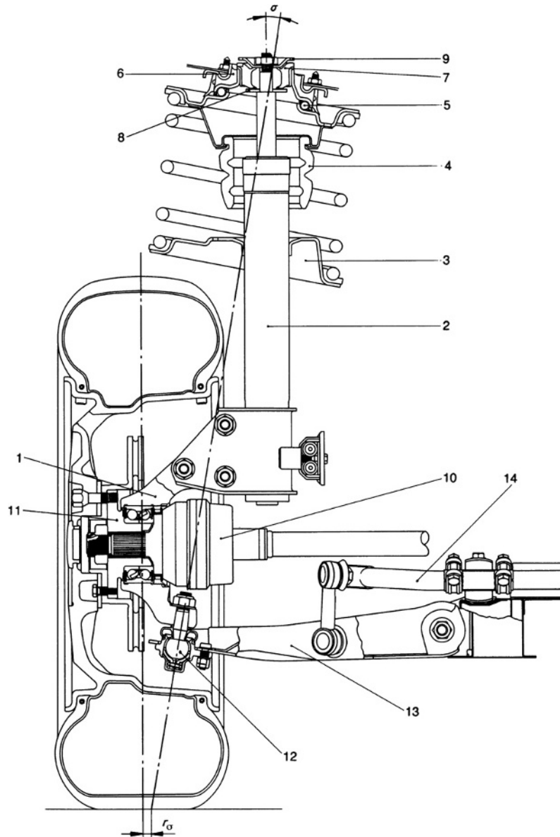
Fig. 8.1-56 Lancia front axle. The McPherson strut consists of the wheel hub carrier 1 and the damping part 2; the two are connected by three screws. The lower spring seat 3 sits firmly on the outer tube and also acts as a buffer for the supplementary spring 4. This surrounds the outer tube 2 giving a longer bearing span (path l-o , Fig. 8.1-11). The supporting bearing 5 is arranged diagonally and thus matches the position of the coil spring which is offset to reduce damping friction. The rubber bearing 6 absorbs the spring forces, and the rubber bearing 7 absorbs the forces generated by the damping. Disc 8 acts as a compression buffer and plate 9 acts as a rebound buffer for this elastic bearing. Both parts come into play if the damping forces exceed certain values. The centre of the CV joint 10 lies in the steering axis and the wheel hub 11 fits onto a two-row angular (contact) ball bearing. Guiding joint 12 sits in a cone of the wheel hub carrier 1 and is bolted to the lower transverse control arm 13. Inelastic ball joints provide the connection to the anti-roll bar 14. The steering axis inclination \sigma between the centre point of the upper strut mount and guiding joint 12 and the (here slightly positive) kingpin offset at ground (scrub radius) r_\sigma are included.
