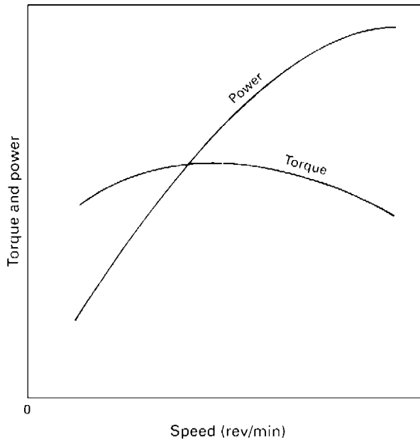
Fig. 1.1-11 Torque and power variation over engine speed range.
