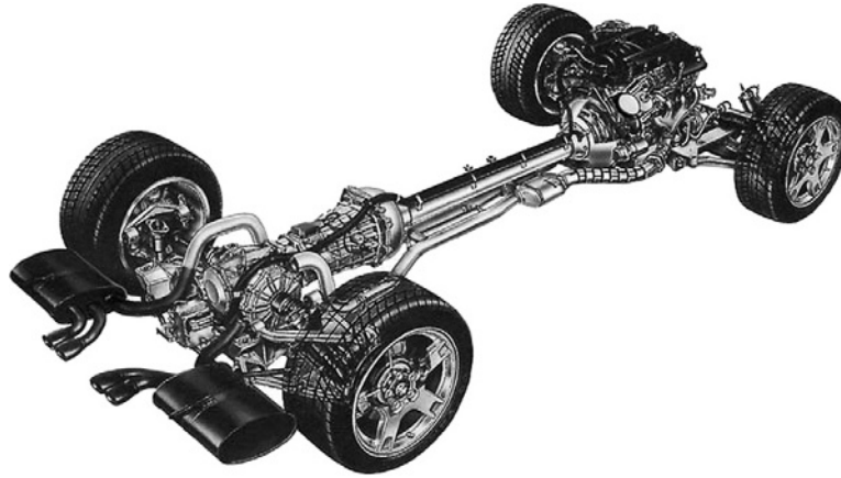
Fig. 8.1-33 Chevrolet Corvette (1998). In order to achieve balanced axle-load distribution, a more rigid overall system (necessary on account of the greater flexibility of the plastic bodywork) and more leg room, the gearbox is integrated with the rear-axle differential. Compared with standard drives, the cardan shaft turns higher (with engine speed) but is subject to correspondingly less torque. The front and rear axles have plastic (fibreglass) transverse leaf springs. Compared with the previous model, unwanted vibration, particularly on an uneven road surface, is reduced as a result of the shorter length of the wheel spindles of 63 mm and the small steering-axle angle of 8.8^\circ . Owing to the combination of a castor angle of 6.5^\circ with a castor trail of 36 mm (previous model: 5.9^\circ , 45 mm), a good compromise is achieved between high lateral rigidity of the axle and good feedback properties.
