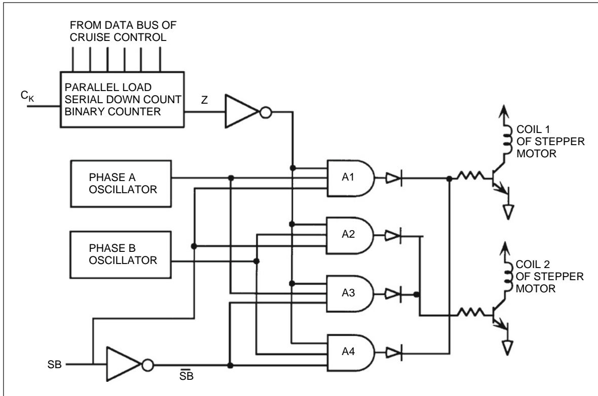
Fig. 13.1-9 Stepper motor actuator for cruise control.
