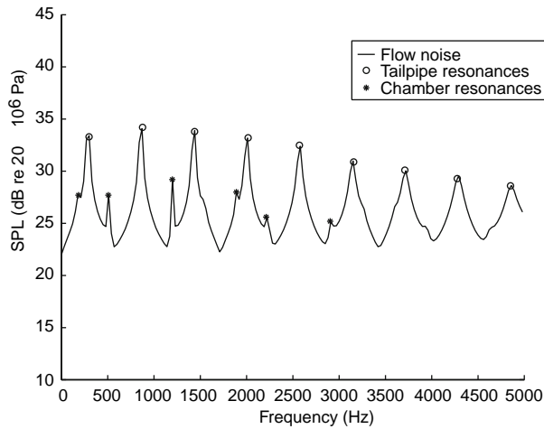
Fig. 22.1-18 Predicted levels of flow noise from a simple silencer element using the method of Davies and Holland (1999) . The exhaust tailpipe and chamber resonances have been marked as in Davies (1981) .
