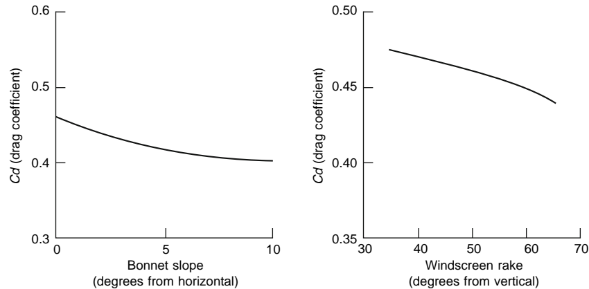
Fig. 19.1-3 Drag reduction by changes to front body shape.
