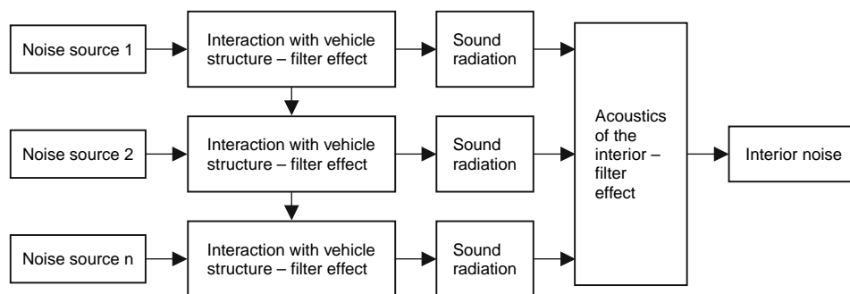
Fig. 21.1-1 Schematic showing the origin of interior noise.
