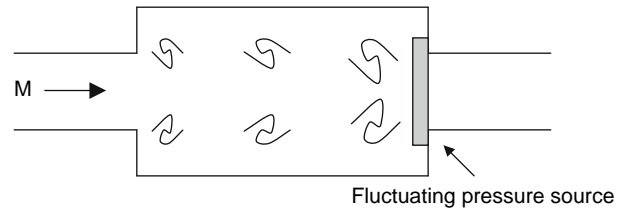
Fig. 22.1-17 Prediction of a common flow noise source (after (Davies and Holland, 1999)). M denotes a flow with a finite Mach number.
