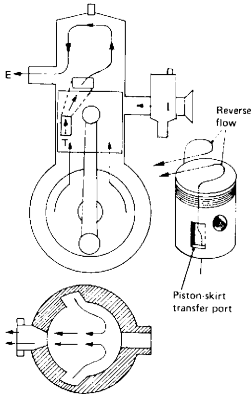
Fig. 1.1-6 Reverse flow or Schnuerle scavenging.
