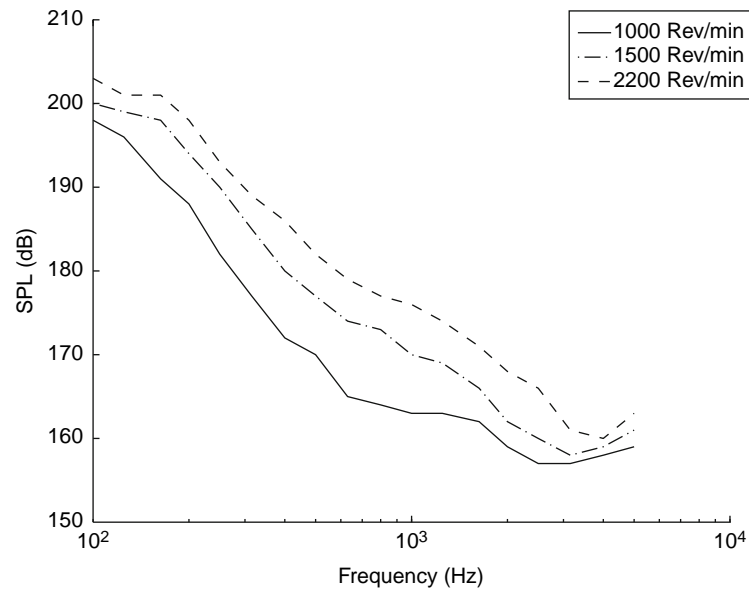
Fig. 21.1-6 Effect of engine speed on cylinder pressure spectra. NA-DI diesel engine at full load: data obtained from Nelson (1987) and Russell (1979).
