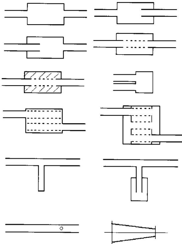
Fig. 22.1-22 Simple and complex silencing units used for intake and exhaust systems.
