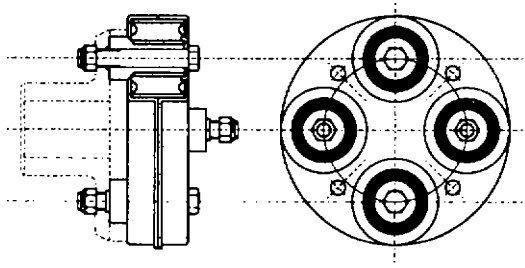
Fig. 2.1a-8 Rubber bush type torsionally resilient coupling.
