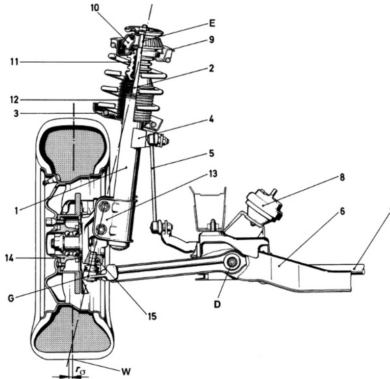
Fig. 8.1-8 Rear view of the left-hand side of the McPherson front axle on the Opel Omega (1999) with negative kingpin offset at ground (scrub radius) r_{\sigma} and pendulum-linked anti-roll bar. The coil spring is offset from the McPherson strut to decrease friction between piston rod 2 and the rod guide. Part 2 and the upper spring seat 9 are fixed to the inner wheel house panel via the decoupled strut mount 10.
