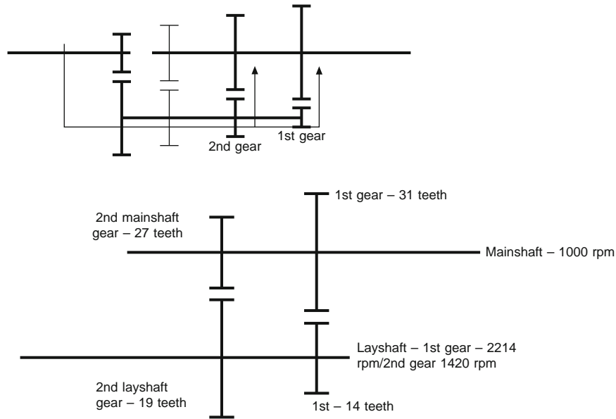
Fig. 5.1-11 Diagram to show the gears involved and ratio implications of a gearchanging between 1st and 2nd gear.
