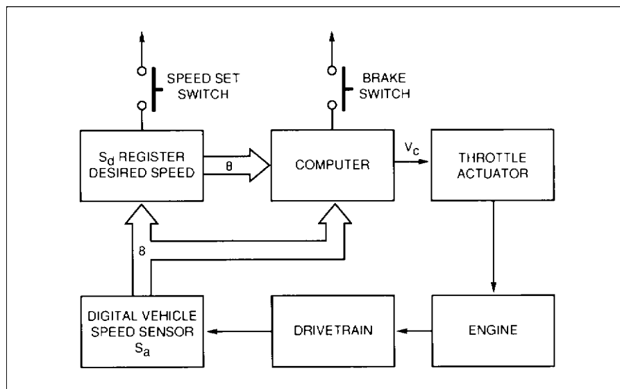
Fig. 13.1-4 Digital cruise control system.
