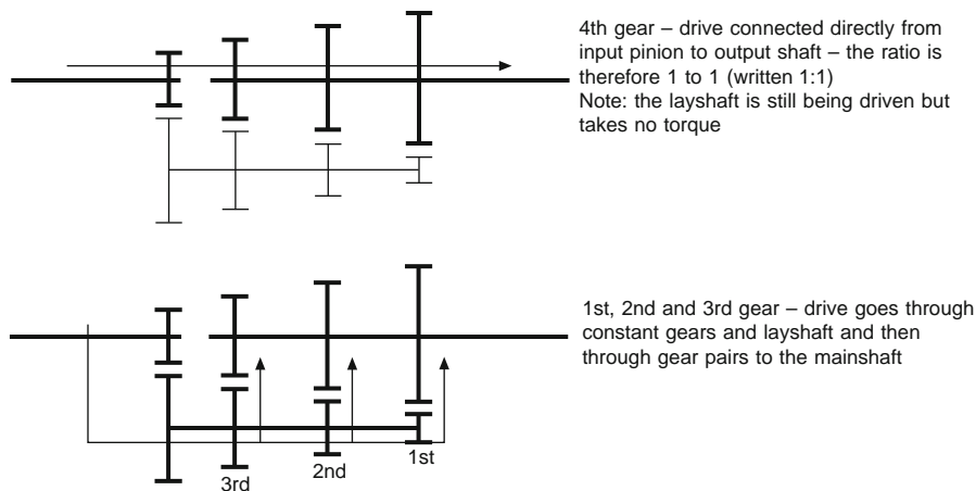
Fig. 5.1-10 Diagrams to illustrate different gears selected in a simplified gearbox.
