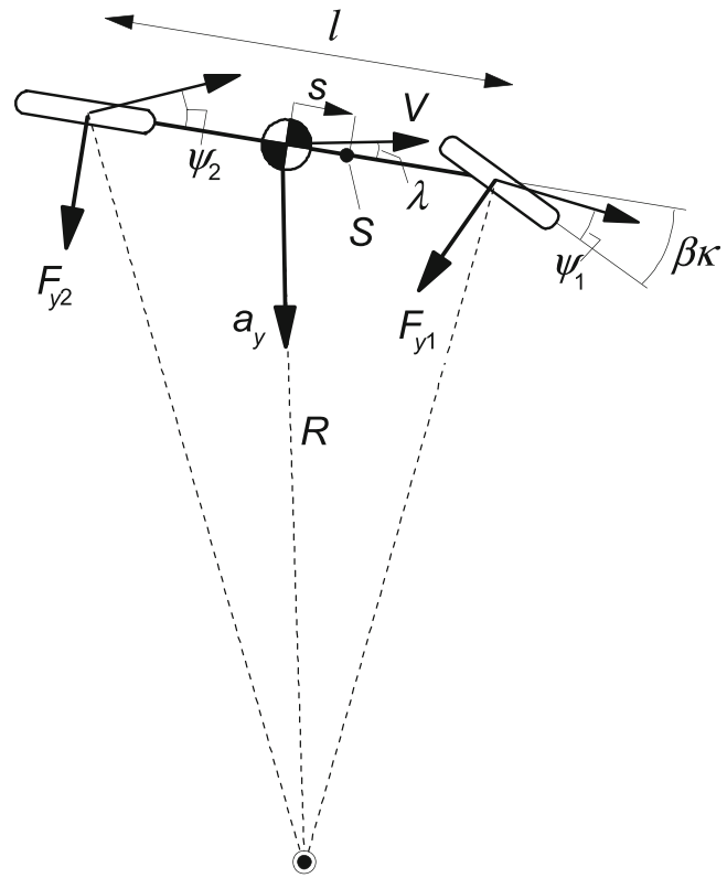
Fig. 11.1-11 Two-wheel vehicle model in a cornering manoeuvre.
