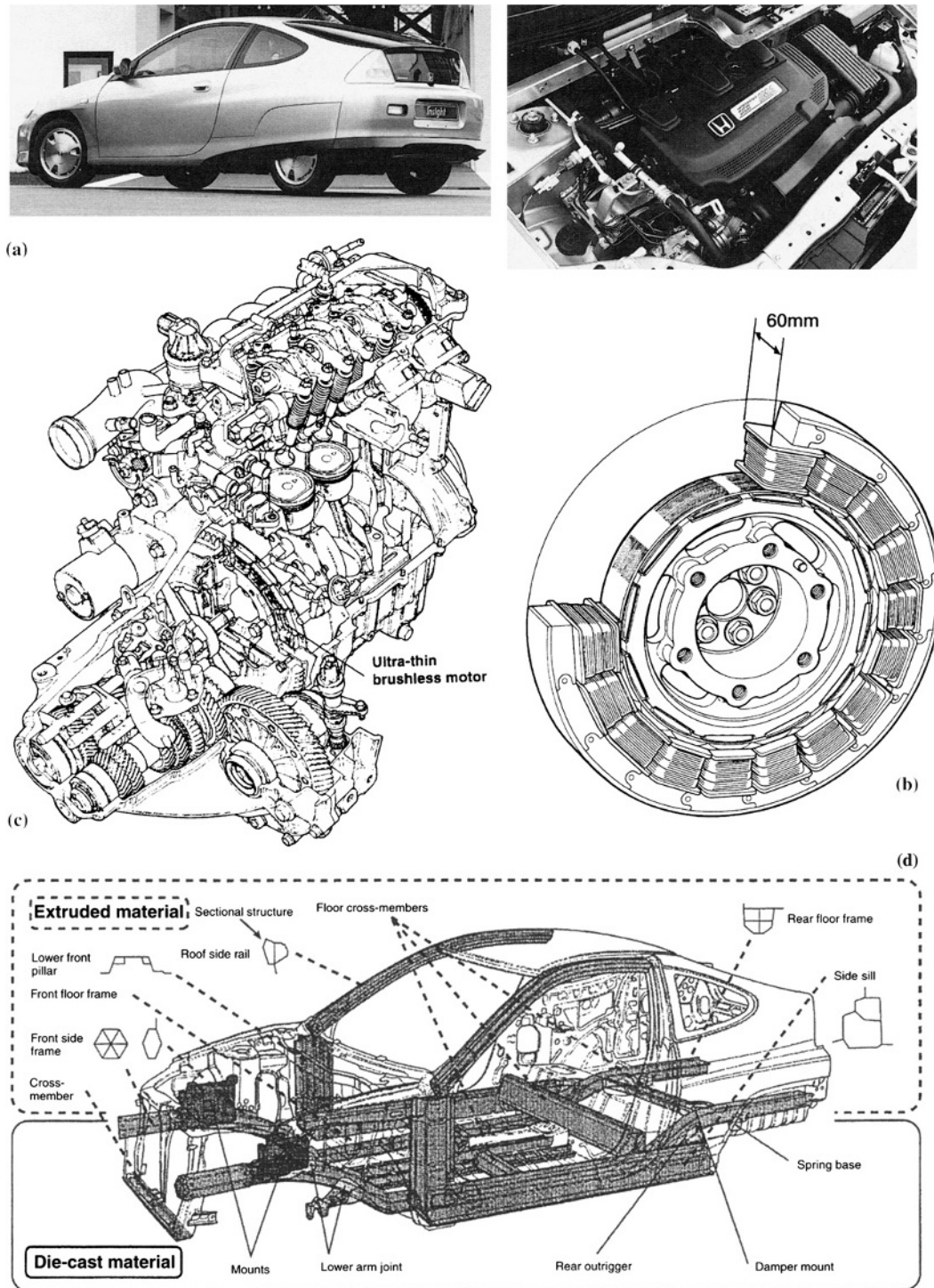
Fig. 7.1-16 Honda Insight hybrid: (a) aerodynamic tailed body and underbonnet power unit; (b) motor; (c) motor installation; (d) body structure.
