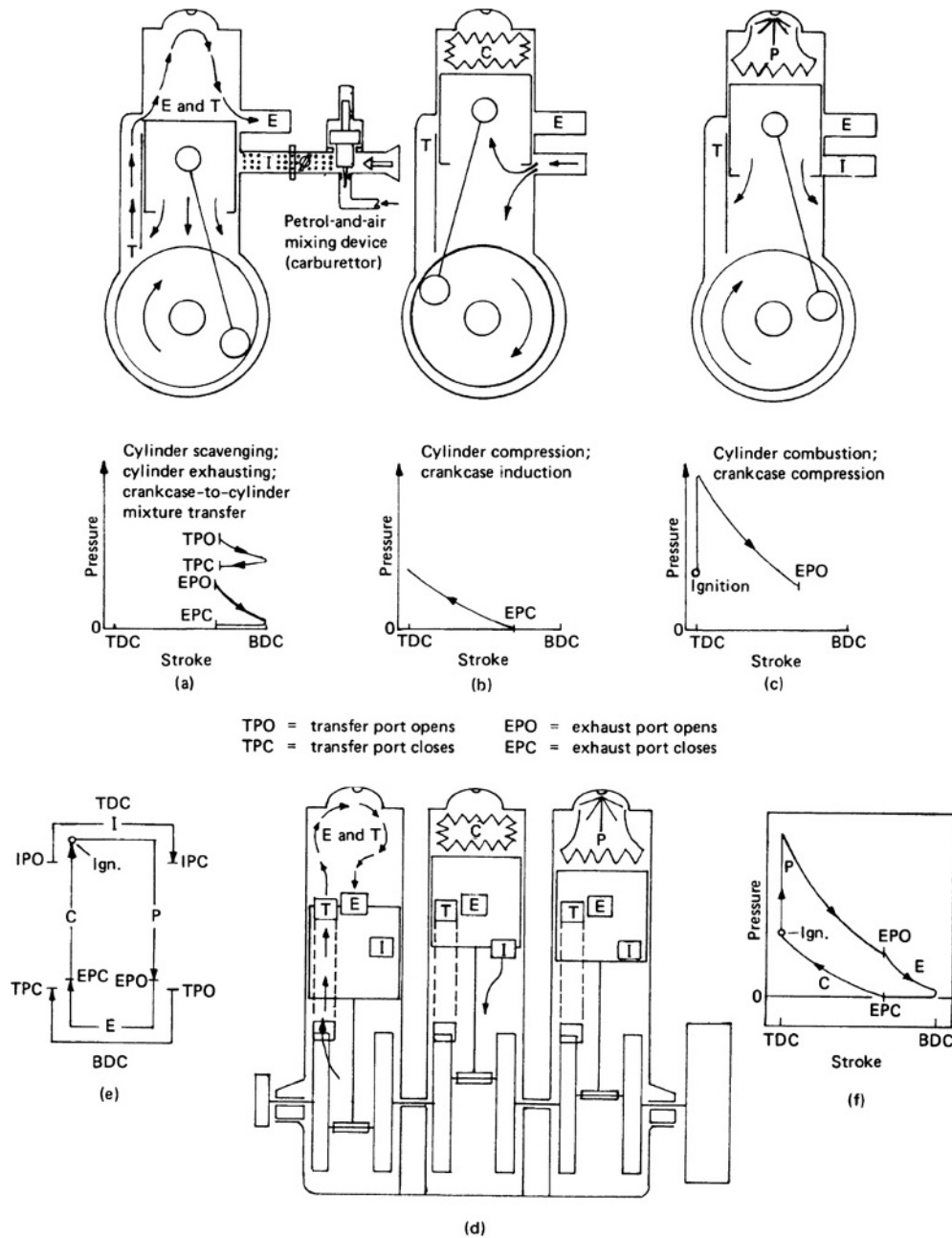
Fig. 1.1-5 Two-stroke-cycle petrol engine.
