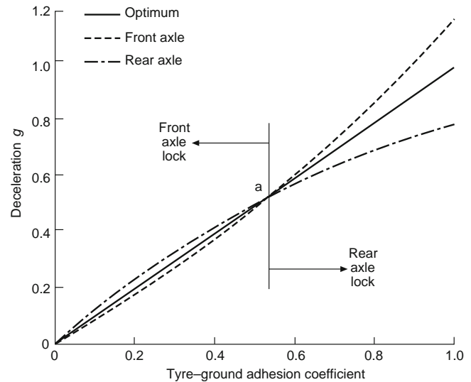
Figure 12.1-11 Deceleration as a function of tyre-ground adhesion.
