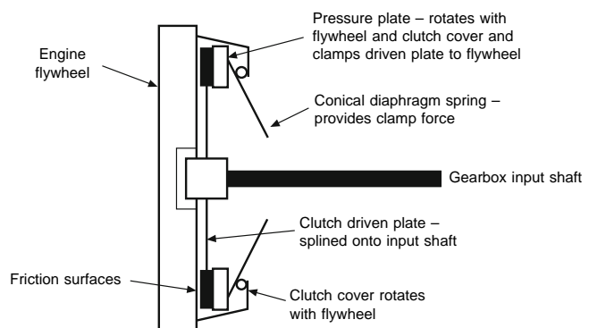
Fig. 5.1-13 Diagram of a conventional single-plate clutch.
