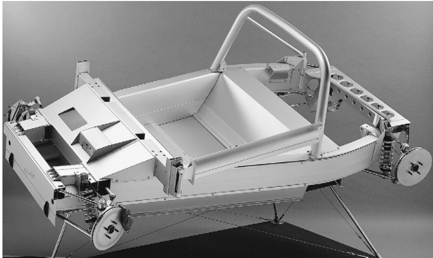
Fig. 16.1-19 Punt chassis (courtesy of Lotus Cars Ltd).
