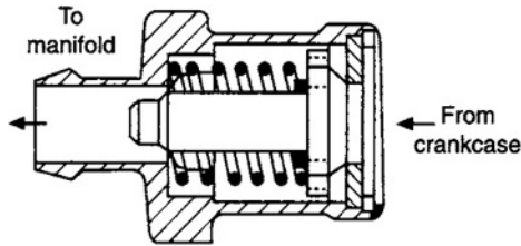
Fig. 3.1-7 AC-Delco crankcase ventilation control valve. With zero depression in the manifold, the valve seats on the right-hand orifice and with maximum depression on the left-hand one. In normal running it floats between the two.
