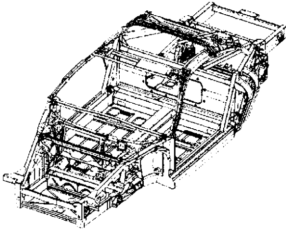
Fig. 18.1-26 Ferrari 360 Modena design.
