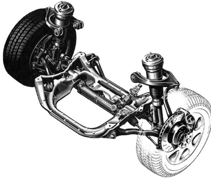
Fig. 8.1-39 Multi-link front suspension of the Mercedes-Benz model W220 (S class, 1998). Based on a double wishbone axle, two individual links (tension strut and spring link) are used instead of the lower transverse link in order to control the steering axle nearer to the middle of the wheel. As a result, the kingpin offset and disturbing force lever arm are reduced and vibrations are caused by tyre imbalances and brake-force fluctuations is consequently minimized. Crash performance is also improved by the more open design. The air-spring struts with integrated shock absorber proceed directly from the spring link. The laterally rigid rack and pinion steering in front of the middle of the wheel leads to the desired elastokinematic understeer effect during cornering owing to the laterally elastic spring link bearings. The manufacturing tolerances are kept so small by means of punched holes that the adjustment of camber and camber angles in production is not necessary.
