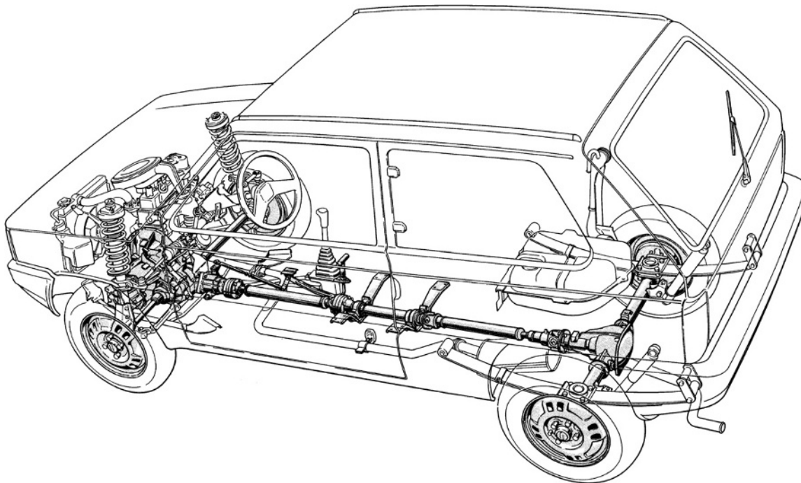
Fig. 8.1-68 The Fiat Panda Treking 4 × 4, a passenger car based on front-wheel drive with transverse engine. The vehicle has McPherson struts at the front and a rigid axle with longitudinal leaf springs at the back. The propshaft leading to it is divided into three to be able to take the rotational movements of the rigid axle around the transverse ( y ) axis during drive-off and braking and to absorb movements of the drive unit. The Fiat Panda is an estate car with the ratio:
