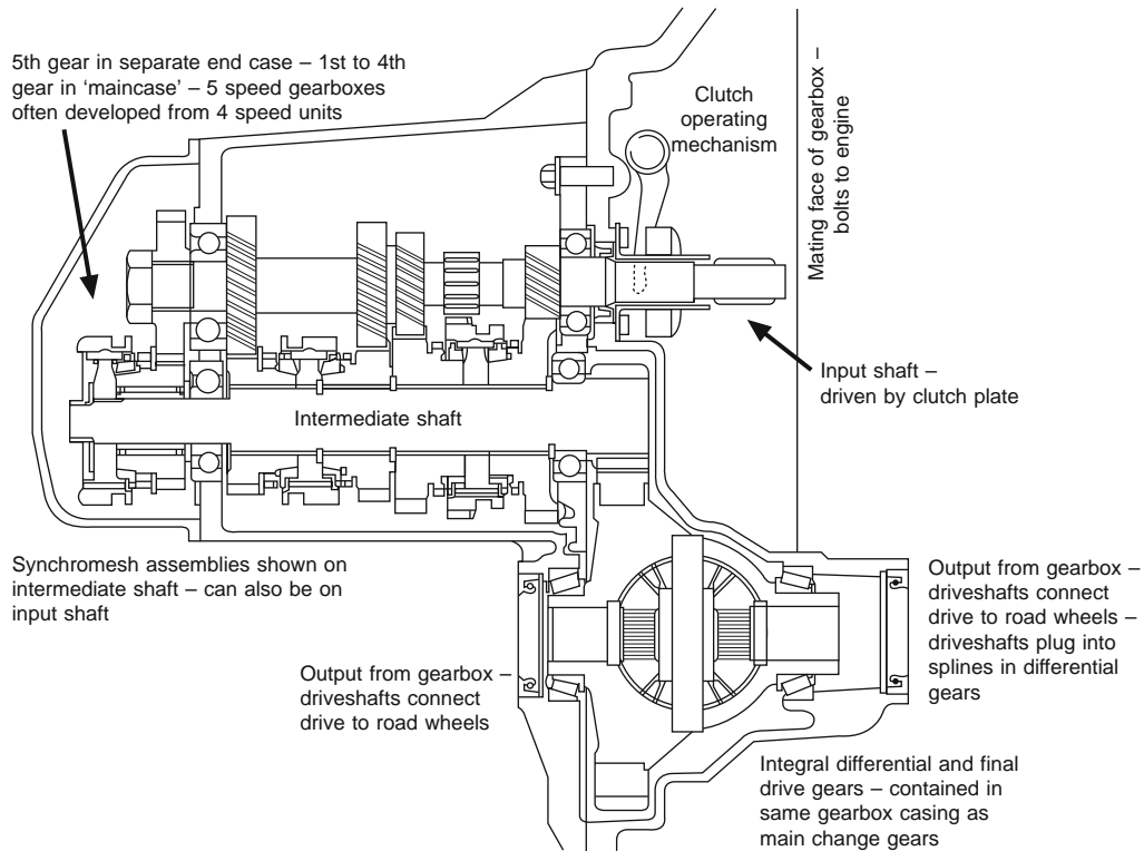
Fig. 5.1-6 Cross section of a front-wheel-drive manual gearbox.
