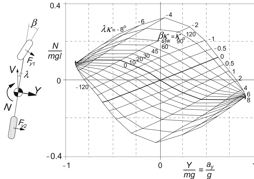
Fig. 11.1-27 The MMM diagram portraying the car's potential manoeuvring capacity.
