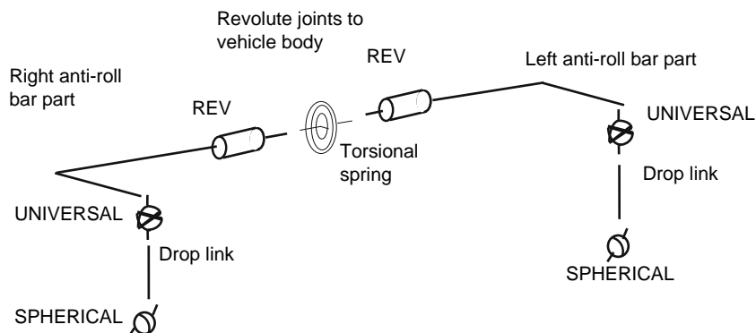
Fig. 15.1-17 Modelling the anti-roll bars using drop links. (This material has been reproduced from the Proceedings of the Institution of Mechanical Engineers, K2 Vol. 213 'The modelling and simulation of vehicle handling. Part 2: vehicle modelling', M.V. Blundell, page 131, by permission of the Council of the Institution of Mechanical Engineers.)
