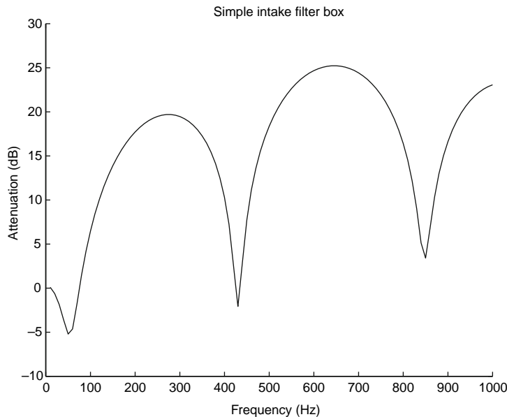
Fig. 22.1-29 Attenuation of a simple intake filter box calculated using APINEX software.
