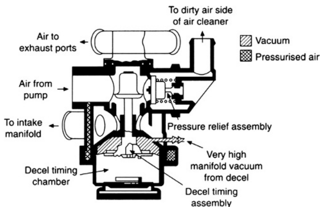
Fig. 3.1-10 Air intake control valve. Some of the air is also diverted into the induction manifold to reduce CO and HC output in the exhaust.
