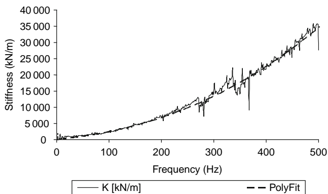
Fig. 21.1-3 Measured engine mount stiffness (Verstraeten, 2003).
