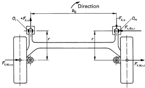
Fig. 8.1-31 The lateral forces F_{Y,W,r,o} and F_{Y,W,r,i} occurring at the centres of tyre contact during cornering are absorbed at the bearing points O_1 and O_{rs} . This results in a moment M_y = (F_{Y,W,r,o} + F_{Y,W,r,i})Xr = F_{X,o} b_0 which (depending on the elasticity of the rubber bearing) can cause 'lateral force oversteering'. The longer the control arms (distance r ) and the closer the points O_1 and O_{rs} (distance b_0 ), the greater the longitudinal forces \pm F_{X,o} .
