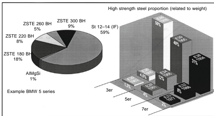
Fig. 18.1-16 Increasing proportion of high strength steel used in BMW body structures. 7
