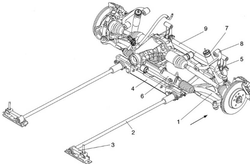
Fig. 8.1-81 Front suspension and drive axle of the Mercedes-Benz off-road vehicle of the M series. In off-road vehicles, rigid axles are mostly used. Instead of these, Mercedes-Benz installs double wishbone suspensions at the front and rear. In this way, the proportion of unsprung masses can be reduced by approximately 66%; driving safety and riding comfort are increased. For space reasons, torsion-bar springs are used for the suspension of the front axle.
