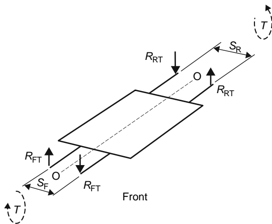
Fig. 16.2-8 Vehicle in pure torsion.
