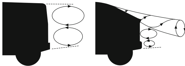
Fig. 19.1-4 (a) 'Squareback' large-scale flow separation. (b) 'Hatchback/fastback' vortex generation.
