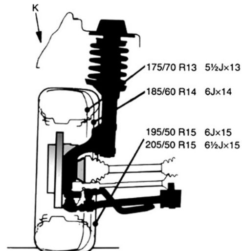
Fig. 10.1-8 Tyre sizes and associated rims used on the VW Golf III. All tyres fit flush up to the outer edge of the wing (wheel house outer panel) K. To achieve this, differing wheel offsets (depth of dishing) e are used on disc-type wheels with the advantage of a more negative rolling radius r_{\sigma} on wider tyres. A disadvantage then is that snow chains can no longer be fitted and steering sensitivity changes very slightly.
