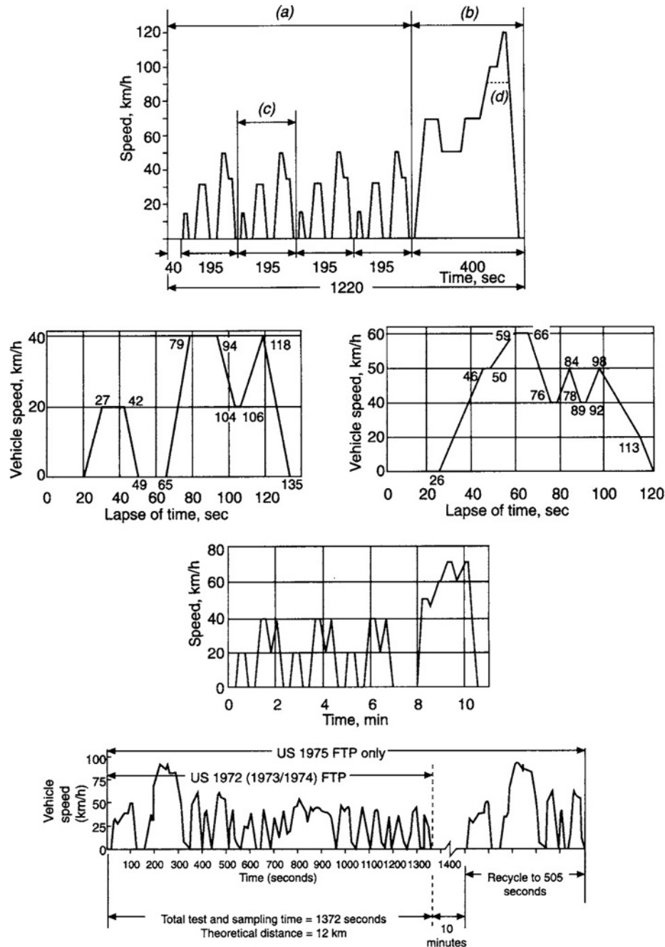
Fig. 3.1-2 Top, in 1992, a hot transient mode, (b) was added to the earlier EEC test cycle, (a). Sampling begins after 40 s. The lower limit, (d) is for vehicles incapable of attaining the higher maximum speed. Mid-left, the Japanese 10 mode cycle, which has to be run through 6 times. Mid-right, the Japanese 11 mode cycle to be run through 4 times. Below, Japanese hot transient test introduced in the early 1990s, comprising 24 s idle, the first three modes of its predecessor and a 15 mode high speed, or hot, test. Bottom, US Federal Test Program (FTP).
