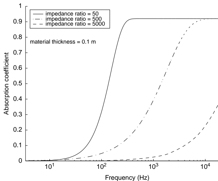
Fig. 21.1-8 Typical absorption characteristics of a porous material: adapted from data provided by Bies and Hansen (1996). Impedance ratio is the specific acoustic impedance of the material divided by the characteristic impedance of the air.
