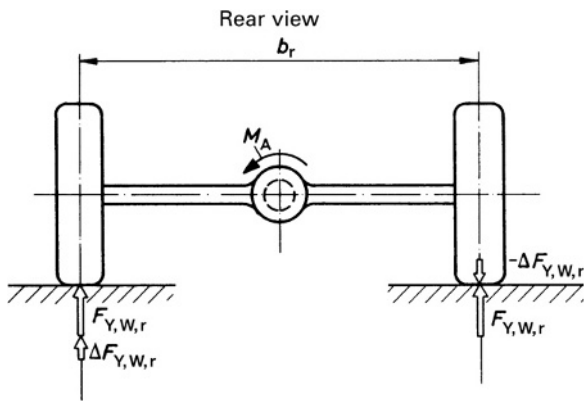
Fig. 8.1-22 If the differential is located in the body of the rigid axle, the driving torque M_A coming from the engine is absorbed at the centres of tyre contact, resulting in changes to vertical force \pm \Delta F_{y,w,r} .
