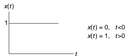
Fig. B21.1-1 The unit step function.
