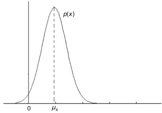
Fig. C21.1-1 The Gaussian distribution.
