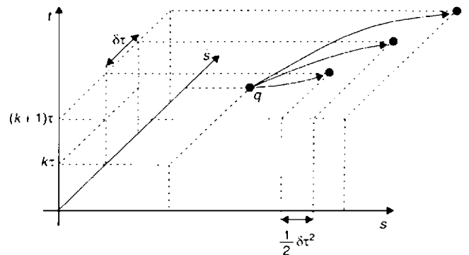
Fig. 14.2-26 G , the graph embedded in ST .
