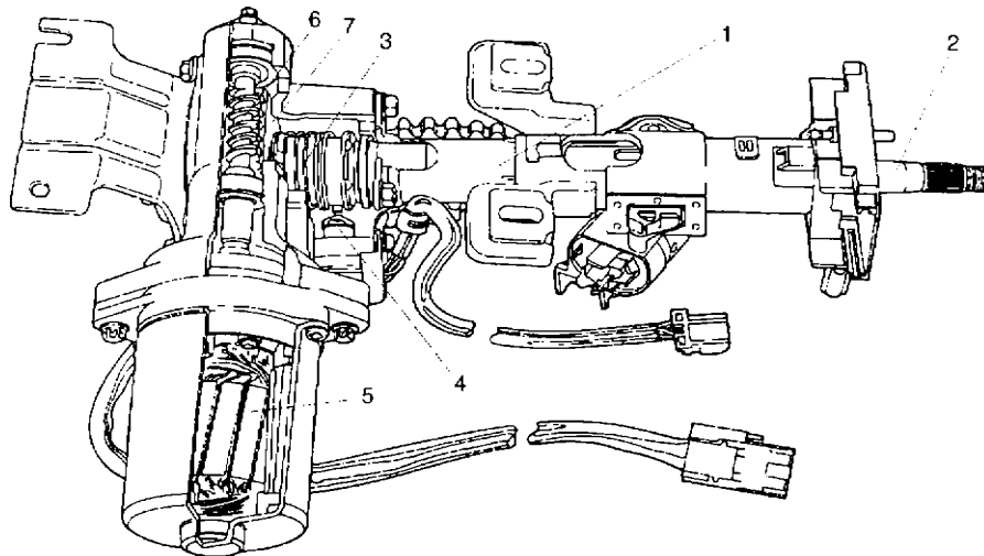
Fig. 9.1-20 Steering column with power-steering assembly of the Opel Corsa (1997). The individual components are:
