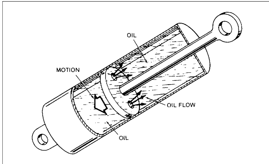
Fig. 13.1-20 Adjustable shock absorber.
