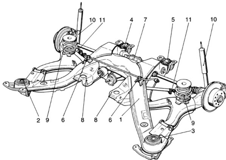
Fig. 8.1-15 Tilted-(Multiple) Staff Steering Rear Axle of the Opel Omega (1999), a further development of the tilted shaft steering axle. The differential casing of the rear-axle drive is above three elastic bearings, noise-isolated, connected with subframe (1), and this subframe is again, with four specially developed elastomer bearings on the installation (pos. 2–5). On top of part seated are the bearings (6) for the back of the stabilizer. Both of the extension arms (8) take up the inner bearings of the tilted shafts, which carry the barrel-shaped helical springs (9). In order to get a flat bottom of the luggage trunk, they were transferred to the front of the axle drive shafts. The transmission i_{Sp} (wheel to spring, becomes thereby with 1.5 comparatively large. The shock absorbers (10) are seated behind the centre of the axle, the transmission is with i_D = 0.86 favourable.
