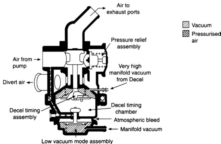
Fig. 3.1-12 The Rochester normal diverter valve diverts air from the oxidising converter to the air cleaner for operation at heavy load.
