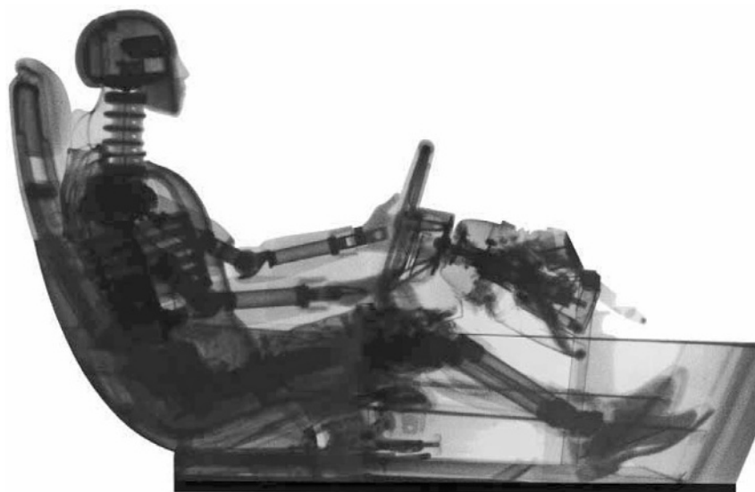
Fig. 17.1-1 MIRA has developed a method of X-ray imaging of tests at a rate of 1000 frames per second, which enables them to view regions which conventional cameras cannot access, for example around the pedals.
