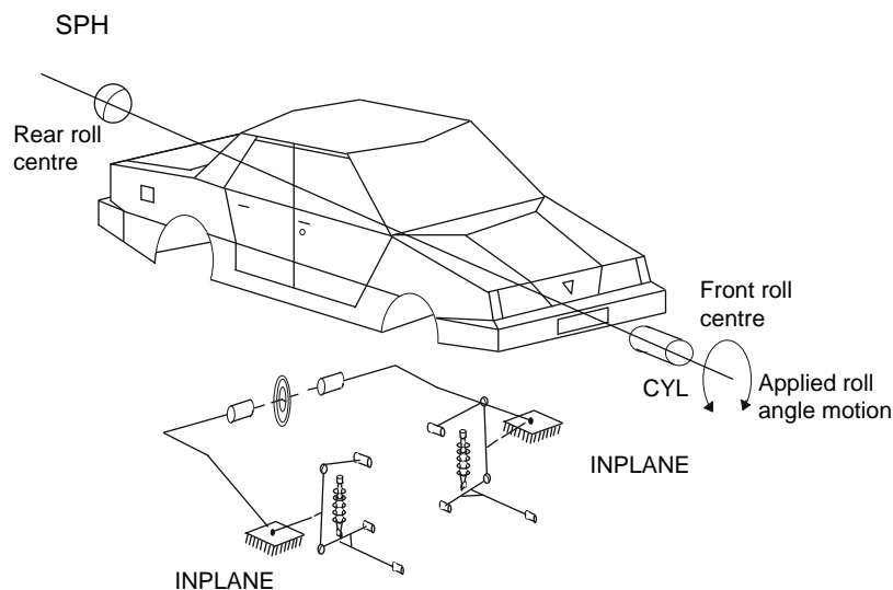
Fig. 15.1-21 Determination of front end roll stiffness. (This material has been reproduced from the Proceedings of the Institution of Mechanical Engineers, K2 Vol. 213 'The modelling and simulation of vehicle handling. Part 2: vehicle modelling', M.V. Blundell, page 127, by permission of the Council of the Institution of Mechanical Engineers.)
