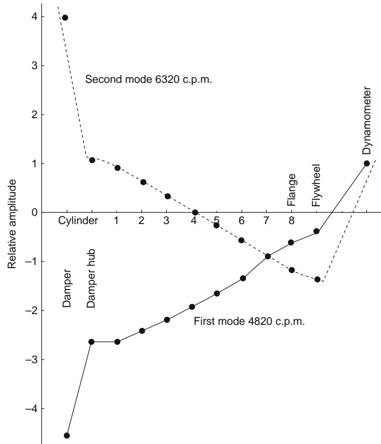
Fig. 2.1a-5 Normal elastic curves for a particular 16 cylinder V engine coupled to a hydraulic dynamometer (taken from an actual investigation).
