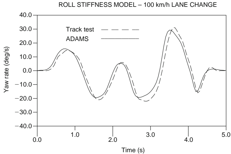
Fig. 15.1-55 Yaw rate comparison – roll stiffness model and test. (This material has been reproduced from the Proceedings of the Institution of Mechanical Engineers, K2 Vol. 214 'The modelling and simulation of vehicle handling. Part 4: handling simulation', M.V. Blundell, page 81, by permission of the Council of the Institution of Mechanical Engineers.)
