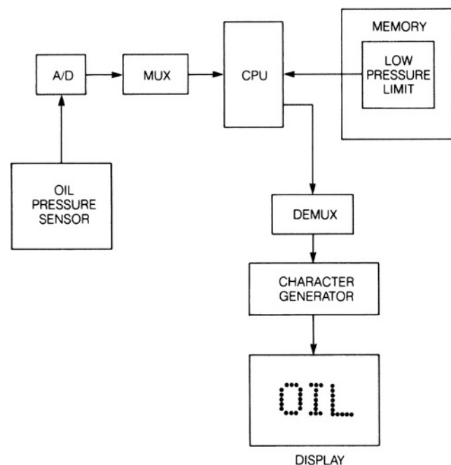
Fig. 23.1-13 Oil pressure measurement.
