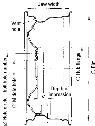
Fig. 10.1-23 The sheet metal disc-type wheel used in series production vehicles consists of a rim and disc. To avoid fatigue fractures, the wheel hub flange diameter should be greater than the dish contact surface. Wheel offset e (depth of impression) and kingpin offset at ground r_{\sigma} are directly correlated. A change in e can lead to an increase or a reduction in r_{\sigma} . The dome-shaped dish leading to the negative kingpin offset at ground is clearly shown (diagram: Hayes Lemmerz).
