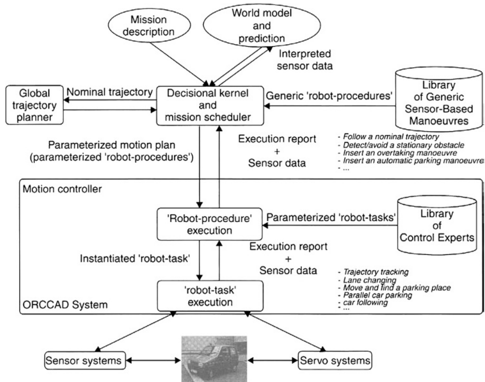
Fig. 14.2-10 Sharp control and decisional architecture.
