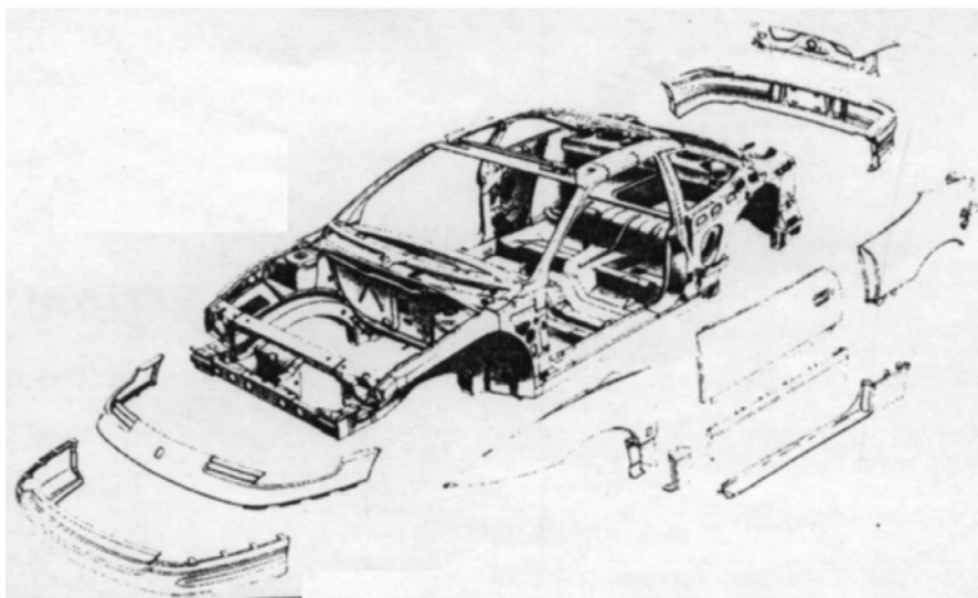
Fig. 18.1-25 Saturn spaceframe showing polymer panels on a four-door sedan. 10
