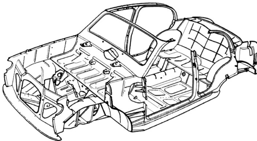
Fig. 18.1-5 Base structure of the Austin A30.
