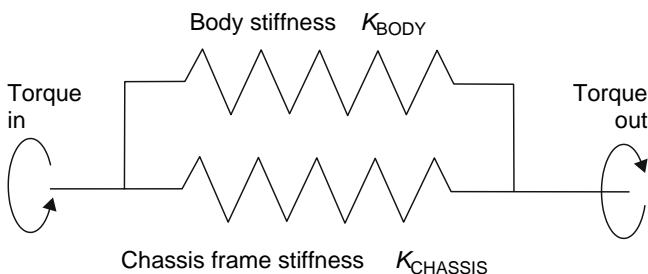
Fig. 16.1-6 Springs in parallel.
