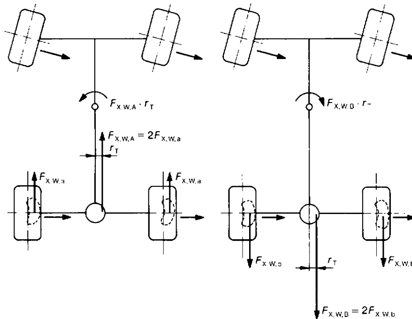
Fig. 10.1-53 The deformation of the tyre contact area during cornering results in aligning torque of the lateral forces which is further intensified by tractive forces and produces an understeering yawing moment. If there is a change in load, the braking forces produce an oversteering yawing moment.
