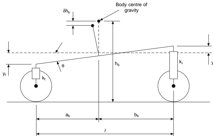
Figure 12.1-16 Determination of vehicle body pitch angle.
