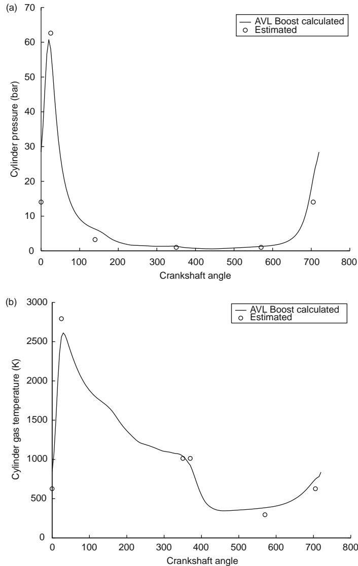
Fig. 22.1-43 Estimates of in-cylinder gas pressure and temperature made using simplified assumptions detailed in Section 22.1.3.14.2. Comparison is made with the results obtained from a full engine simulation of a 2.0-litre gasoline engine at 5000 rev min -1 using AVL Boost
