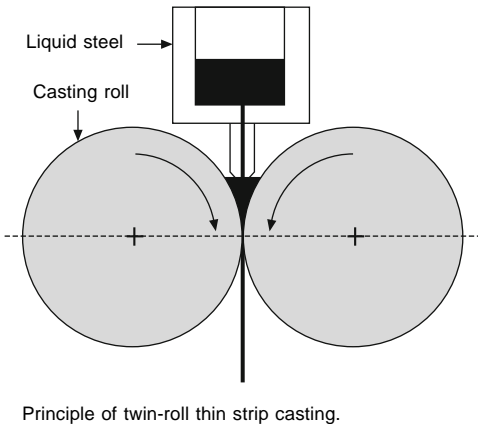
Fig. 18.2-5 Principle of direct process of casting thin strip from molten steel.
