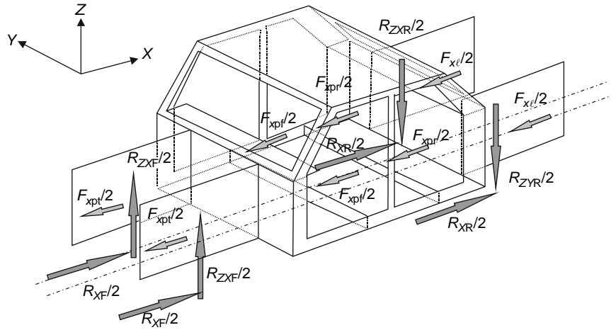
Fig. 16.2-29 Baseline model – braking loads.
