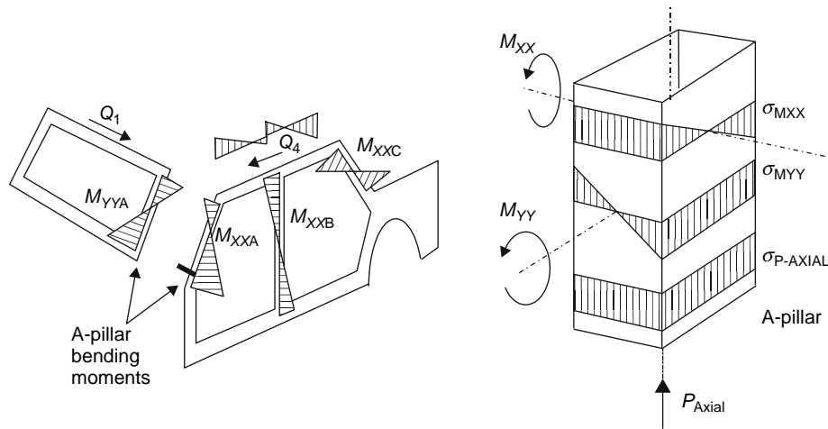
Fig. 16.2-17 Stresses in shared pillar.
