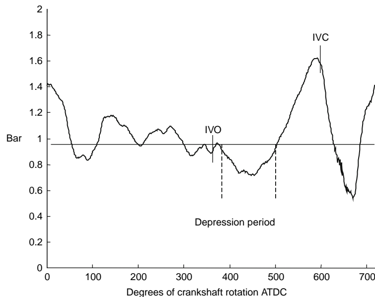
Fig. 22.1-12 Intake port pressure trace, 3/4 rated speed, full load (Dunkley, 1999).
