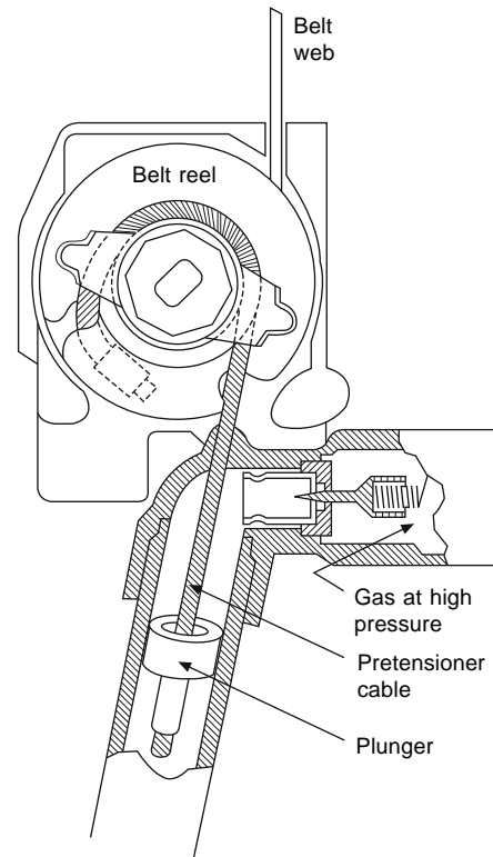
Fig. 17.1-16 Toyota automatic seat belt tensioner. In the event of an impact, gas is discharged from the horizontal cylinder on the right, into the chamber above the plunger, which it forces downwards. Dragging the pre-tensioner cable with it, the plunger thus pre-tensions the seat belt for the duration of the impact, after which the tension is progressively released as the gas escapes through the clearances round the cable and plunger.
