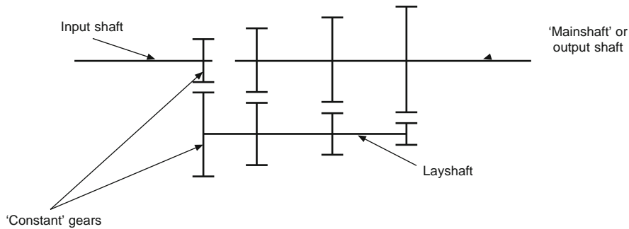
Fig. 5.1-9 Schematic of a gear train layout in a rear-wheel-drive gearbox.
