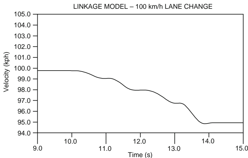
Fig. 15.1-33 Loss in velocity as vehicle 'drifts' through the lane change manoeuvre.
