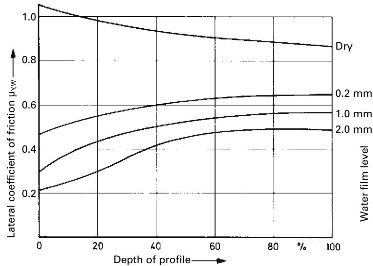
Fig. 10.1-47 Possible lateral friction coefficients \mu_{Y,W} of a steel radial tyre 155 R 13 78 S depending on the depth of the tyre profile as a percentage (starting from 8 mm = 100%) at p_T = 1.8 bar, \alpha = 10^\circ , v = 60 km/h and varying water film levels in mm. The improved grip of the treadless tyre on a dry road can be seen clearly as can its significantly poorer grip in the wet; a fact which also applies to the coefficient of friction in the longitudinal direction (see Section 10.1.7.2).
