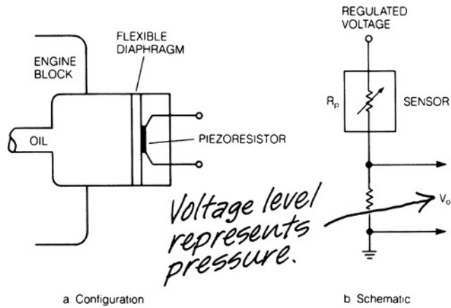
Fig. 23.1-14 Oil pressure sensor.
