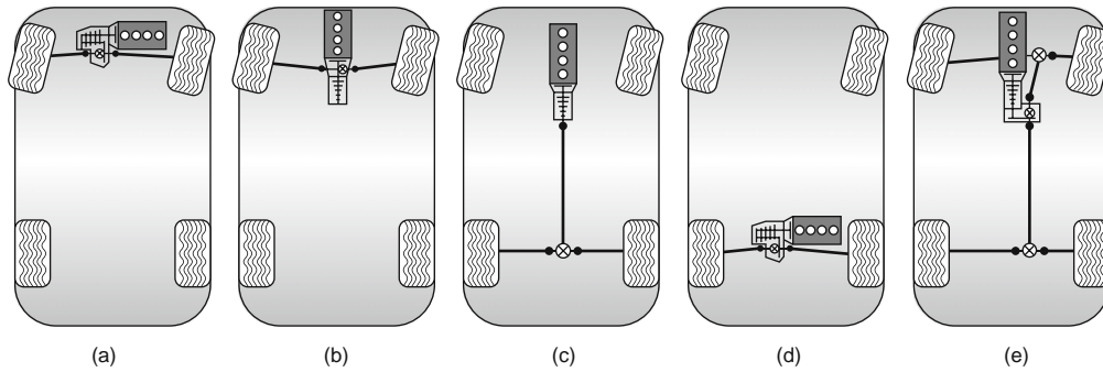
Fig. 5.1-1 Some typical vehicle/powertrain configurations.
