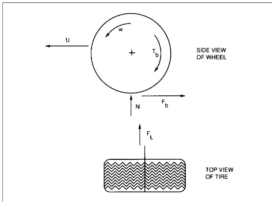
Fig. 13.1-13 Forces during braking.
