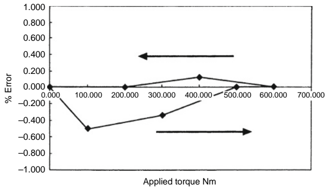
Fig. 2.1-6 Dynamometer calibration error as percentage of applied torque.
