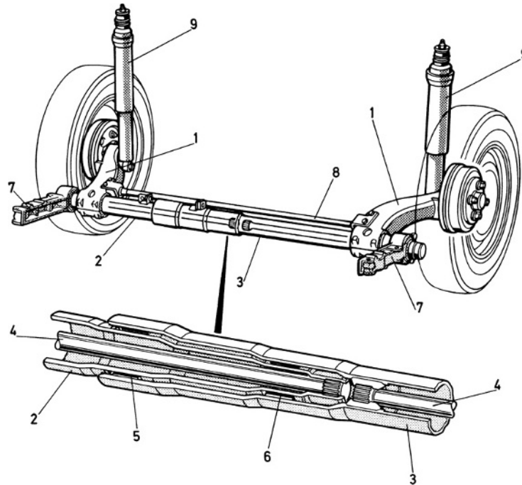
Fig. 8.1-63 Compact trailing arm rear axle, fitted by Renault to less powerful medium-sized vehicles. The short torsion bar springs grip into the guide tubes 2 and 3 in the centre of the vehicle. Parts 2, 3 and 4 are jointly subjected to torsional stresses and so the torsional stiffness of the transverse tubes contributes to the spring rate. On the outside, the cast trailing arms 1 are welded to the transverse tubes, which (pushed into each other) support each other on the torsionally elastic bearings 5 and 6. This creates a sufficiently long bearing basis, which largely prevents camber and toe-in changes when forces are generated.
