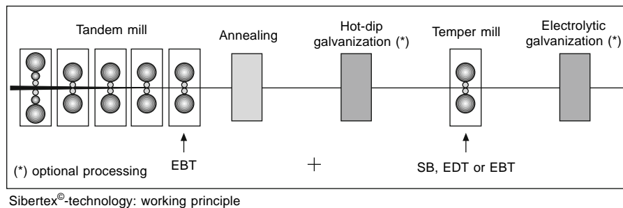
Fig. 18.2-12 Tandem and temper mill treatments offered by the Sibertex process. (Courtesy of Sidstahl.).
