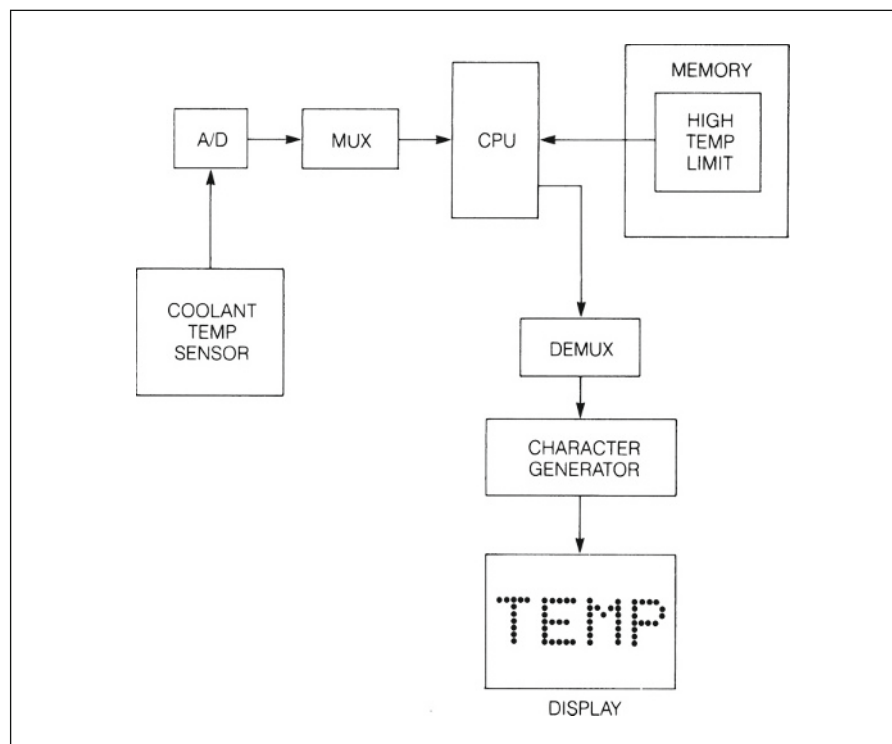
Fig. 23.1-11 Coolant temperature measurement.
