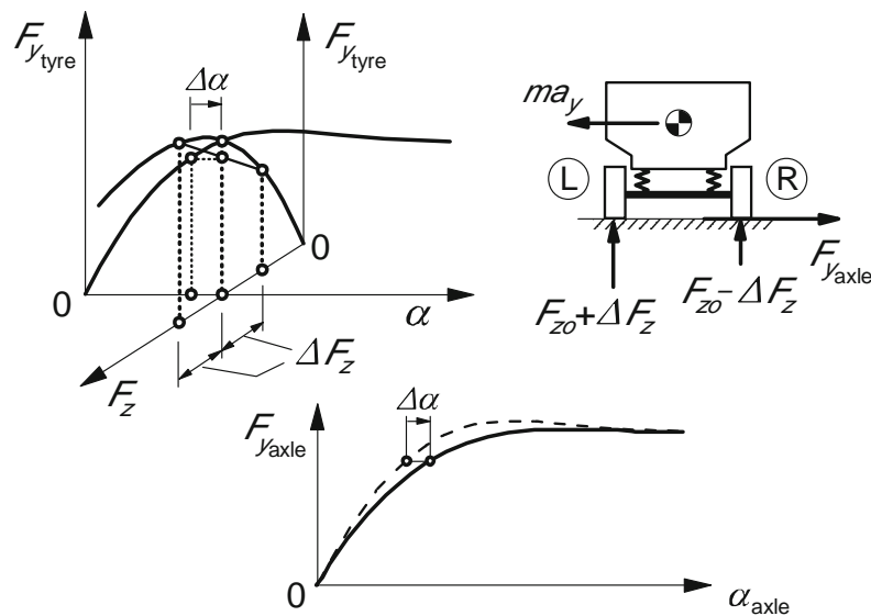
Fig. 11.1-7 The influence of load transfer on the resulting axle characteristic.
