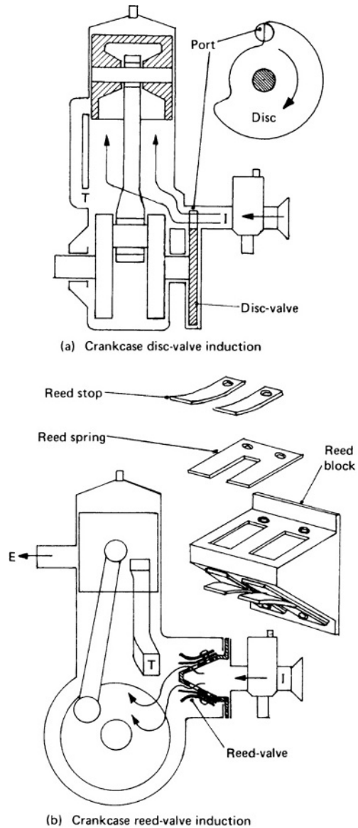
Fig. 1.1-7 Crankcase disc-valve and reed-valve induction.
