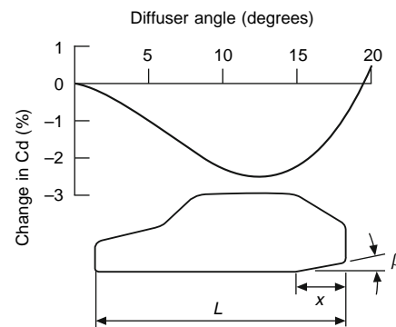
Fig. 19.1-8 Rear, underbody diffusion.
