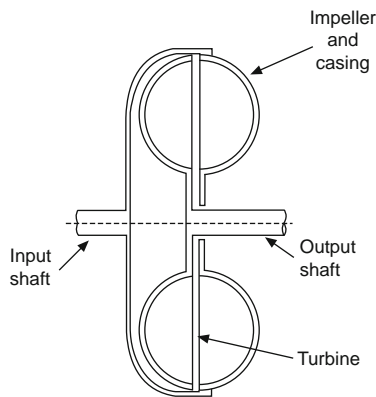
Fig. 5.1-17 Fluid coupling and characteristics.
