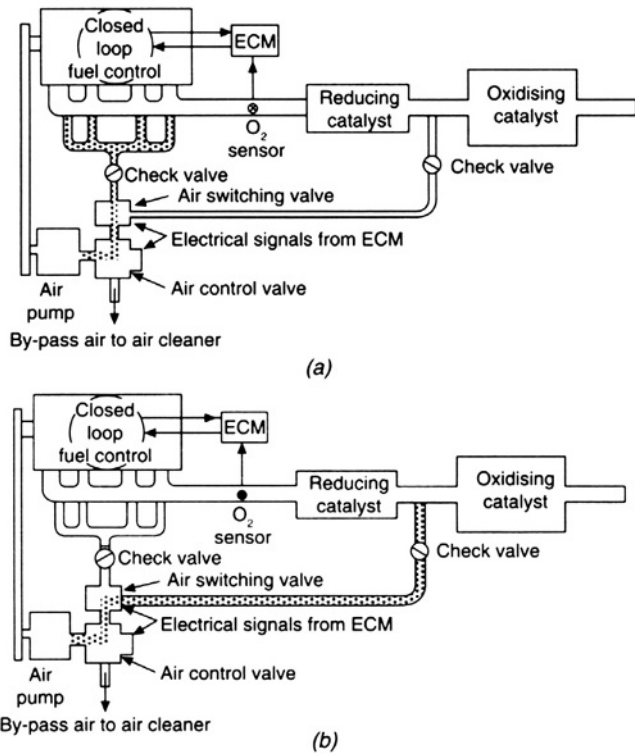
Fig. 3.1-11 System for switching air from the manifold (a) for open-loop operation to the oxidising catalytic converter, (b) for closed-loop operation.
