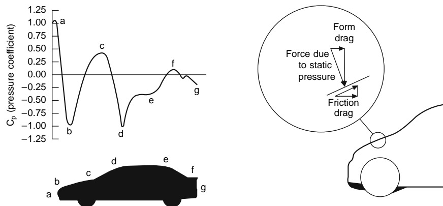
Fig. 19.1-2 (a) Typical static pressure coefficient distribution; (b) The force acting on a surface element.
