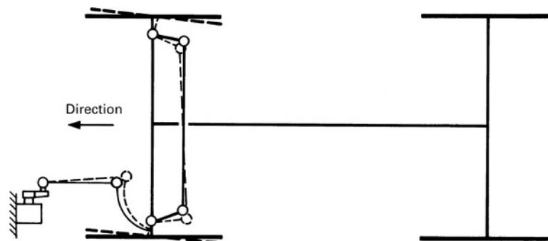
Fig. 9.1-7 If the movement curve 7 of the axle housing and curve 9 of the rear steering rod joint do not match when the body bottoms out, the wheels can turn and therefore an unwanted self-steering effect can occur.
