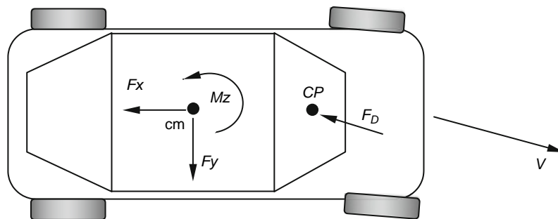
Fig. 15.1-25 Application of aerodynamic drag force.
