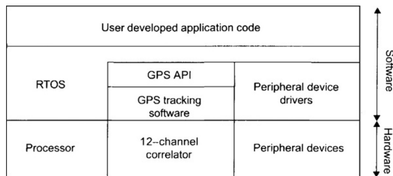
Fig. 14.1-8 GPS-enabled application software architecture.
