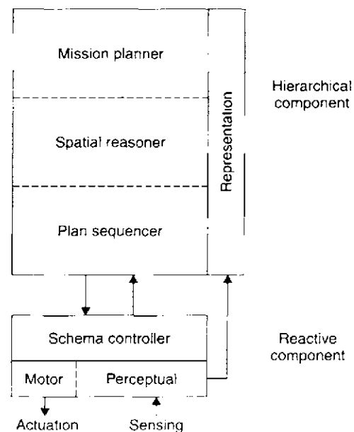
Fig. 14.2-5 AuRA architecture (Arkin).
