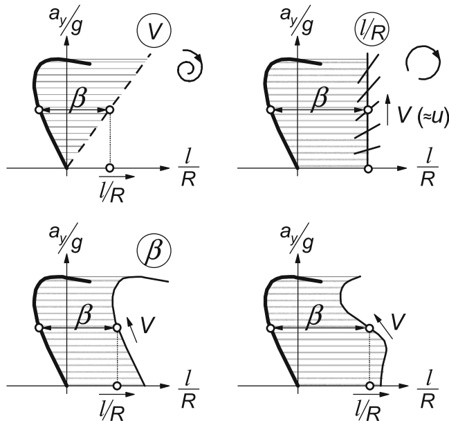
Fig. 11.1-19 Types of quasi-steady-state manoeuvres.
