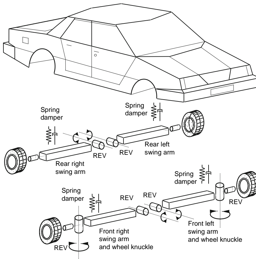
Fig. 15.1-9 Swing arm model approach.
