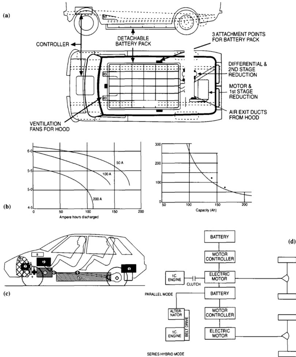
Fig. 6.1-11 Lucas electric and hybrid drive vehicles: (a) GM Griffon; (b) terminal volts per 6 V module and discharge current in amps; (c) Lucas Chloride hybrid car; (d) bi-mode drive system.
