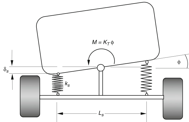
Fig. 15.1-23 Calculation of roll stiffness due to road springs.
