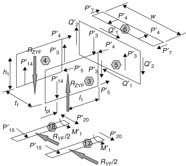
Fig. 16.2-26 Baseline model (front structure) – lateral loading.
