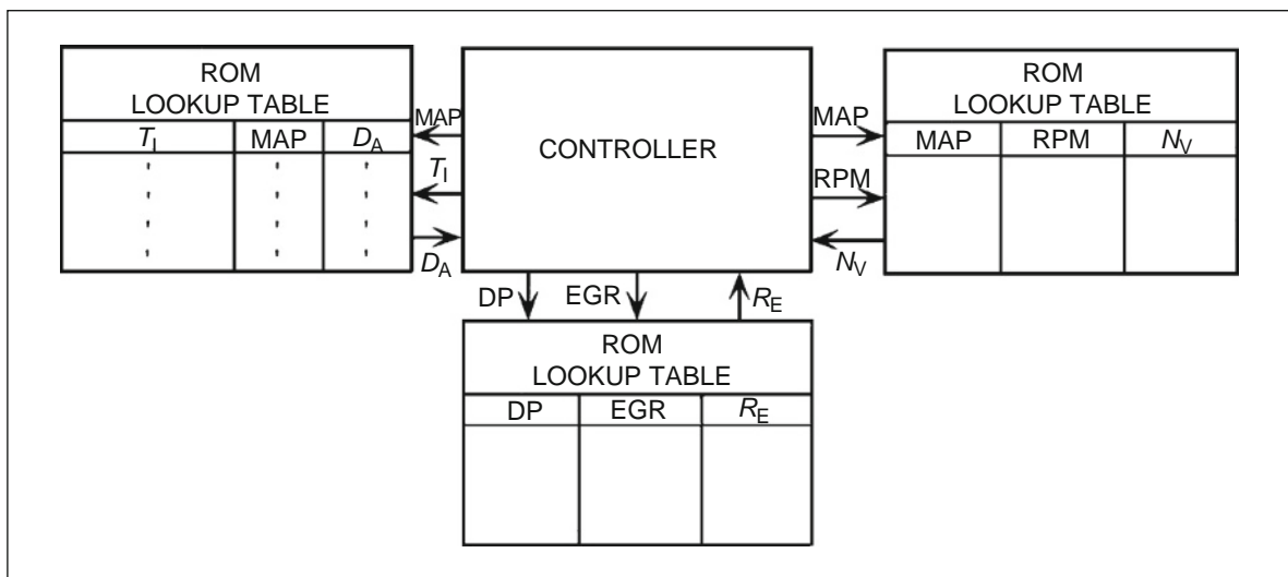
Fig. 4.1-5 Lookup table determination of d_a , R_E , and n_v .
