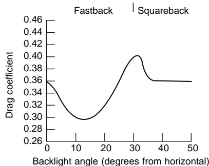
Fig. 19.1-5 The influence of backlight angle on drag coefficient.
