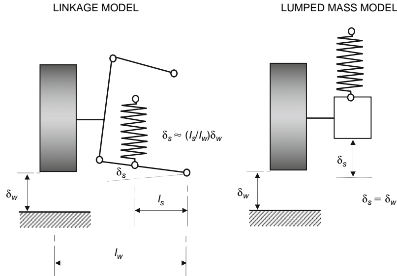
Fig. 15.1-13 Road spring in linkage and lumped mass models.
