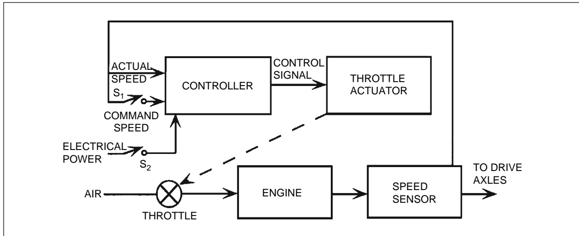
Fig. 13.1-1 Cruise control configuration.
