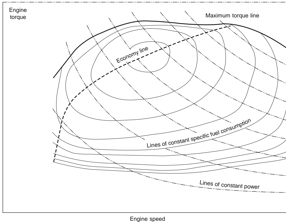
Fig. 5.1-26 A typical petrol engine torque speed characteristic.
