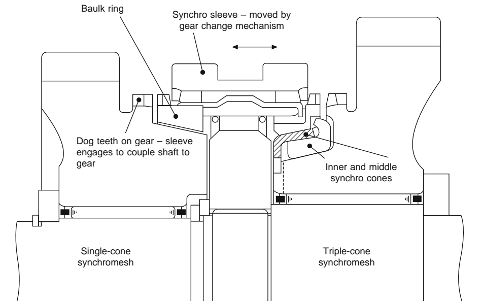
Fig. 5.1-12 Cross section of a synchromesh.
