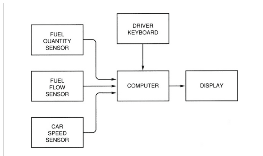
Fig. 23.1-27 Trip information system.
