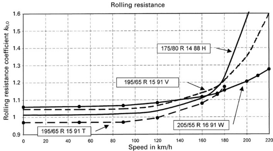
Fig. 10.1-31 Rolling resistance coefficients k_{R,0} , average values of radial tyres as a function of the speed, measured on a drum test rig. Tyres authorized up to 210 \text{ km h}^{-1} have a lower rolling resistance below 160 \text{ km h}^{-1} (than the V and W designs), whilst the value rises sharply above this speed (measurements: Continental). Asphalted roads cause k_{R,0} to increase by around 20% as k_R and rough concrete to at least 30%. The ratios i_R are then 1.2 or 1.3 to 1.4 and the actual value of k_R is: k_R = i_R \times k_{R,0} (2.4a)
