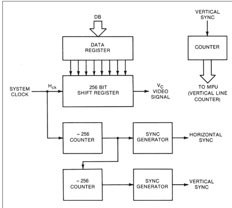
Fig. 23.1-25 Video signal generation.
