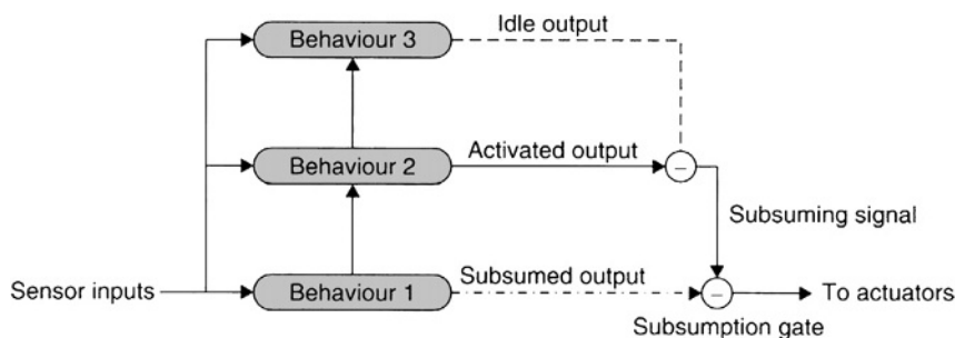
Fig. 14.2-1 Principle of the subsumption architecture (Brooks).
