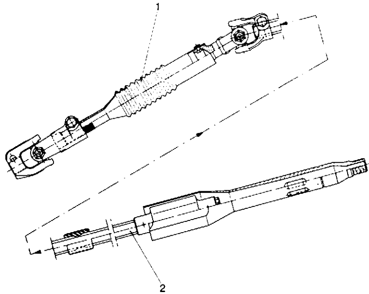
Fig. 9.1-28 Volvo steering column. Both the corrugated tube 1 in the intermediate shaft and the collapsible steering tube 2 meet the safety requirements. To save weight, the universal joints are made of aluminium alloy Al Mg Si 1 F31 (illustration: Lemförder Fahrwerktechnik).
