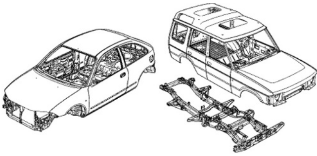
Fig. 18.1-1 Illustration of unitary and chassis body architecture. 3
