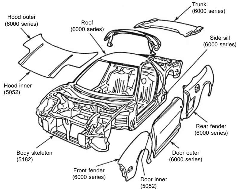
Fig. 18.1-23 Aluminium alloys used for NSX body panels. 9
