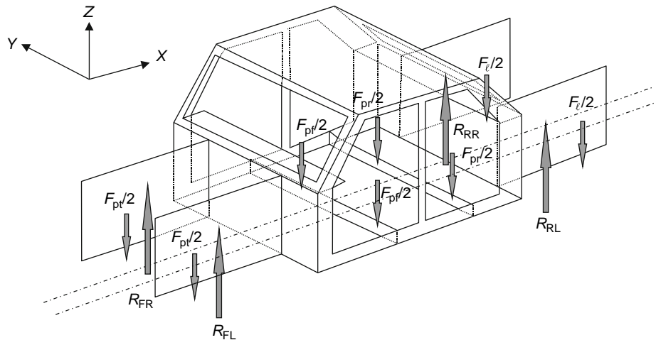
Fig. 16.2-2 Baseline model – bending loads.
