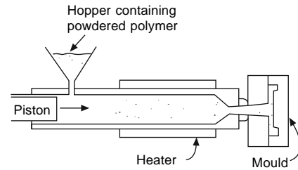
Fig. 18.2-16 Injection moulding process.
