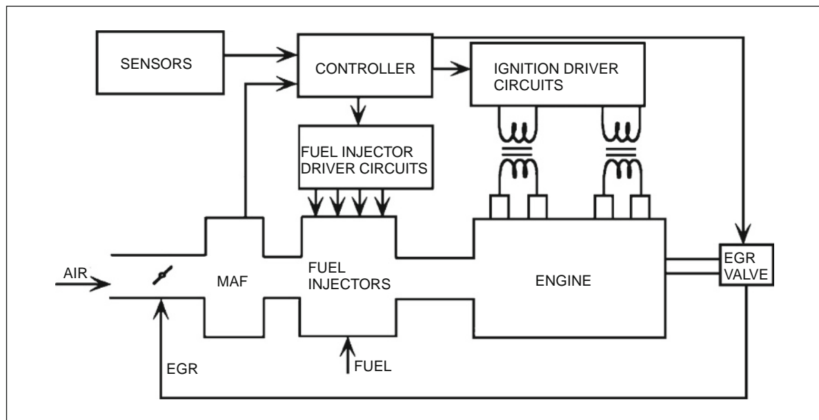
Fig. 4.1-1 Components of an electronically controlled engine.
