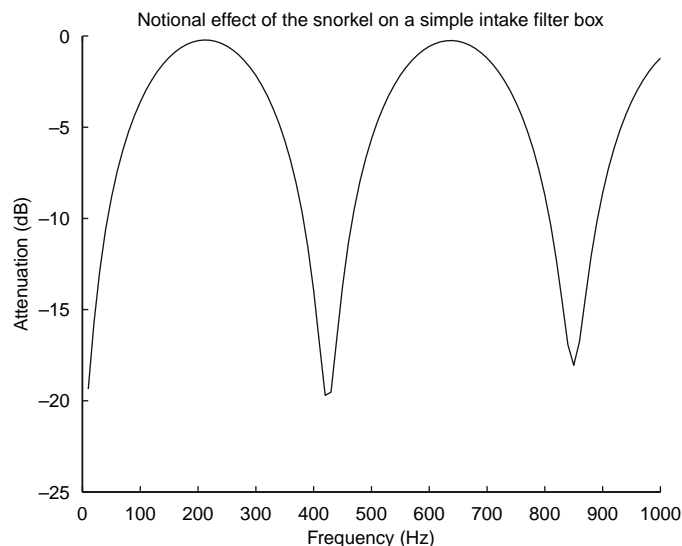
Fig. 22.1-31 Attenuation of the contraction section of a simple intake filter box calculated using APINEX software.
