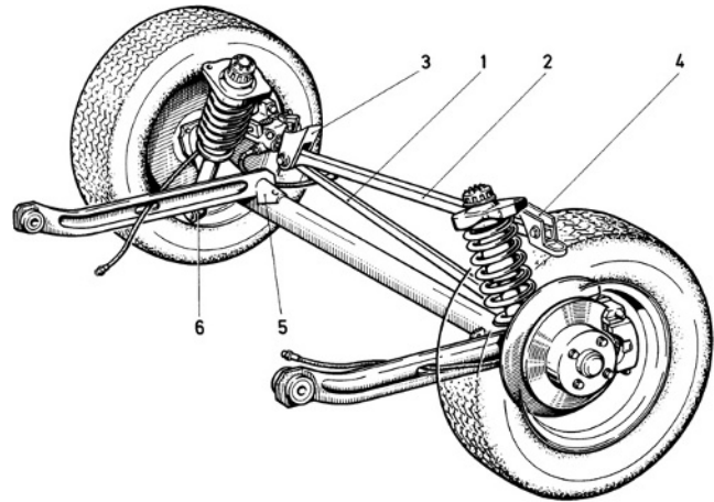
Fig. 8.1-61 Torsion crank axle on the Audi A6 (Audi 100, 1991) with spring dampers fixed a long way out at points 6 and which largely suppress body roll vibrations.
