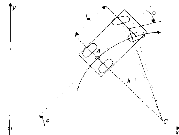
Fig. 14.2-29 A car-like robot.
