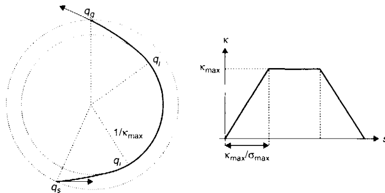
Fig. 14.2-31 A CC turn and its curvature profile.
