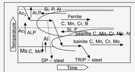
Influence of alloying elements on transformation behaviour
