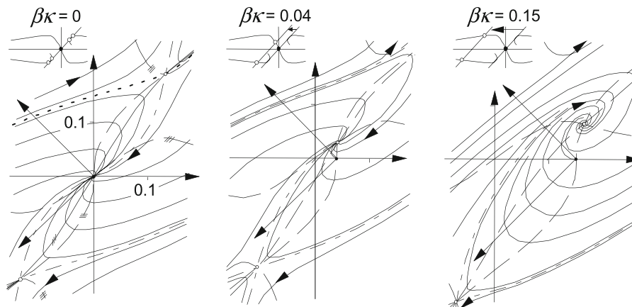
Fig. 11.1-24 Influence of steering on the stability margin (system of Fig. 11.1-20 (bottom)).
