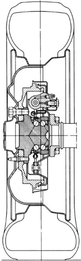
Fig. 8.1-59 Rear+wheel bearing on the Fiat Panda with a third-generation, two-row angular (contact) ball bearing. The wheel hub and inner ball bearing ring are made of one part, and the square outer ring is fixed to the rigid axle casing with four bolts (picture: SKF).
