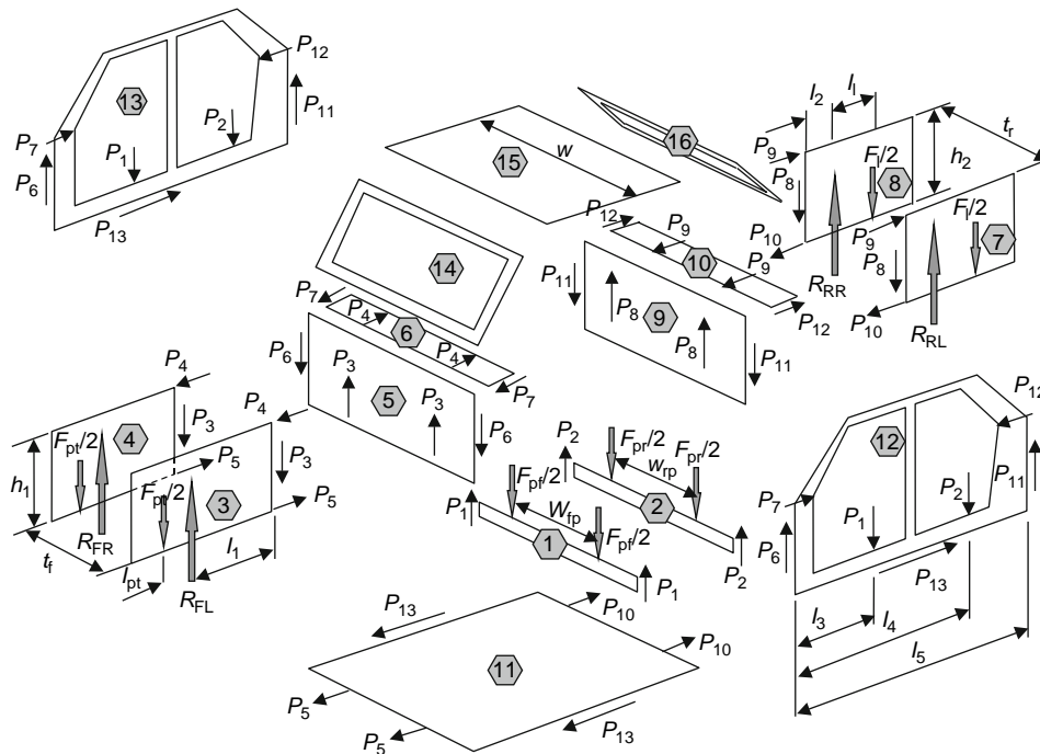
Fig. 16.2-4 Baseline model – bending case, end and edge loads.
