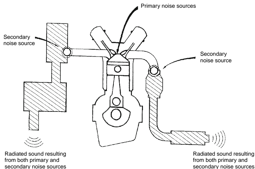
Fig. 22.1-15 Primary and secondary sources of intake and exhaust noise.
