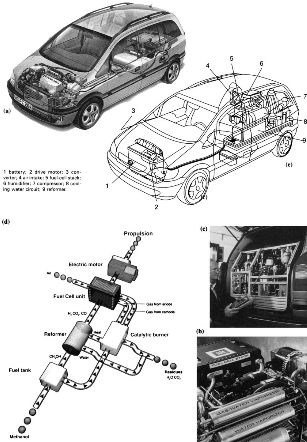
Fig. 6.1-23 GM fuel-cell developments: (a) Zafira conversion package; (b) under-bonnet power-pack; (c) reformer and cells; (d) flow diagram; (e) latest package with on-board hydrogen storage.
