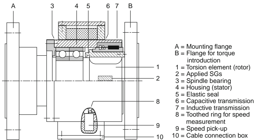
Fig. 2.1-4 Brushless torque-shaft for mounting in shaft-line between engine and 'brake'.
