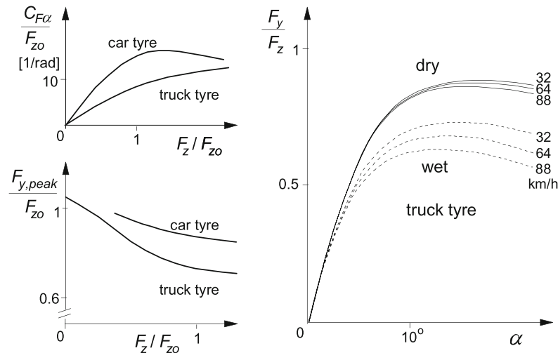
Fig. 11.1-3 Typical characteristics for the normalised cornering stiffness, peak side force and side force vs normalised vertical load and slip angle, respectively. F_{z0} is the rated load.
