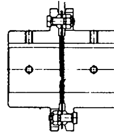
Fig. 2.1a-7 Multiple steel disc type flexible coupling.
