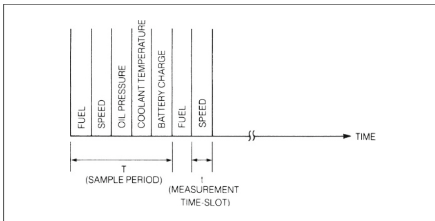
Fig. 23.1-8 Sequential sampling.
