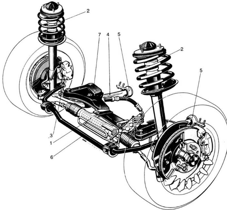
Fig. 8.1-40 Spring strut front axle of the BMW Roadster Z3, which Lemförder Fahrwerktechnik produce in the USA and supply directly to the assembly line there. The additional springs 2 are positioned in the coil springs (Fig. 8.1-11) which are offset at an angle in order to reduce friction. The stabilizer 6 is connected to the lower links by the struts 3.
