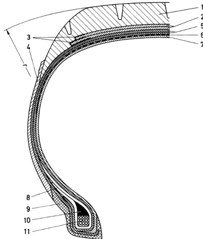
Fig. 10.1-5 Radial design passenger car tyres in speed category T (Fig. 10.1-12); the number of layers and the materials are indicated on the sidewall (see Fig. 10.1-18). The components are: 1 running tread; 2 steel belt; 3 edge protection for the belt, made of rayon or nylon; 4 sidewall; 5 substructure with two layers; 6 cap; 7 inner lining; 8 flipper; 9 bead profile; 10 core profile; 11 bead core.
