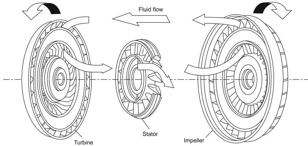
Fig. 5.1-18 Torque converter 3D with flow path.
