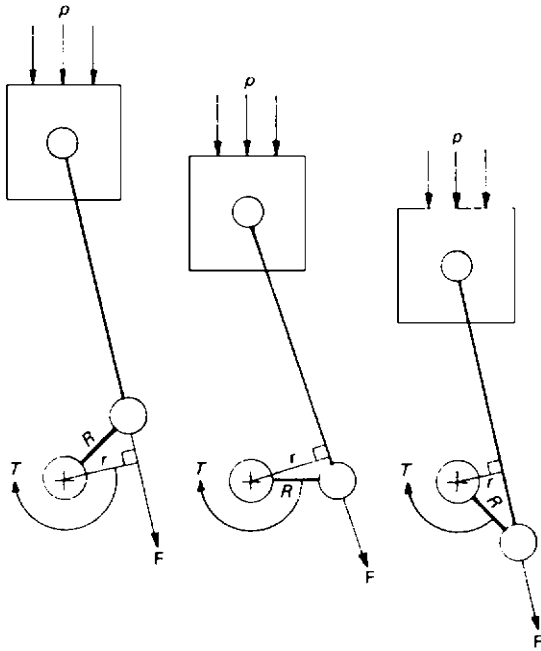
Fig. 1.1-10 Torque variation during crankshaft rotation ( p = cylinder gas pressure; F = connecting-rod thrust; R = crank-throw; r = effective crank radius; T = turning-effort or torque).
