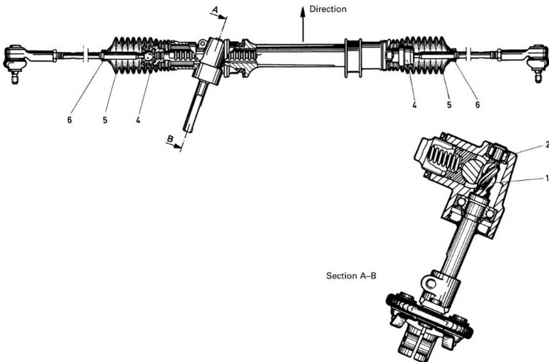
Fig. 9.1-9 Rack and pinion steering on the Vauxhall Corsa (1997). The tie rod axial joints 4 bolted to the side of the steering rack and the sealing gaiters 5 can be seen clearly. To stop them from being carried along when the toe-in is set (which is done by rotating the middle part of the rod) it is necessary to loosen the clamps 6.
