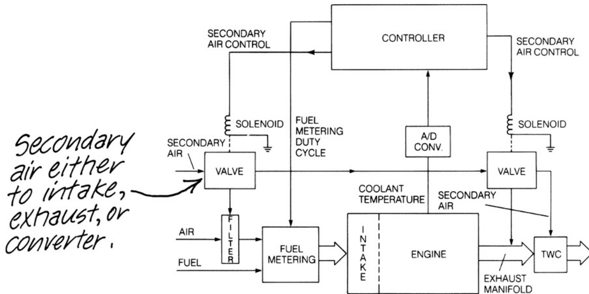
Fig. 4.1-17 Secondary air control system.
