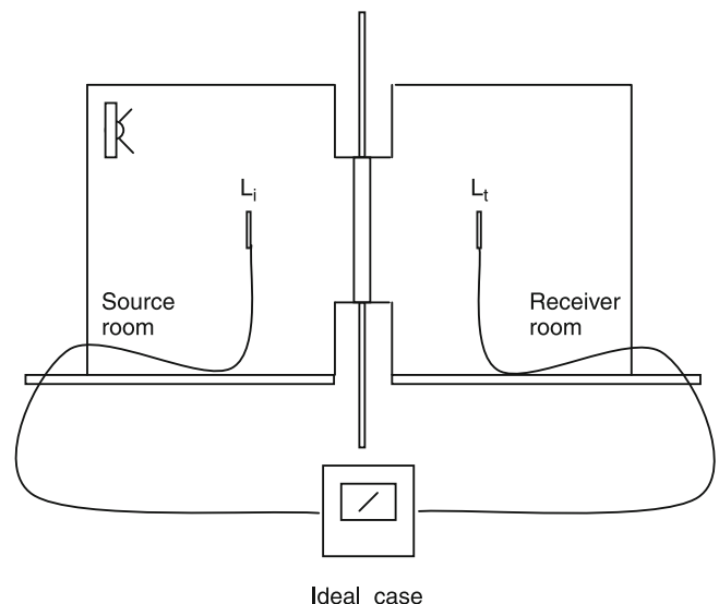
Fig. 21.1-15 The transmission suite.
