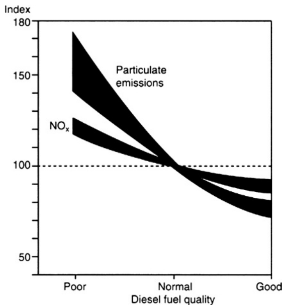
Fig. 3.1-24 Relationship between particulate emissions and fuel quality, as established by Volvo.
