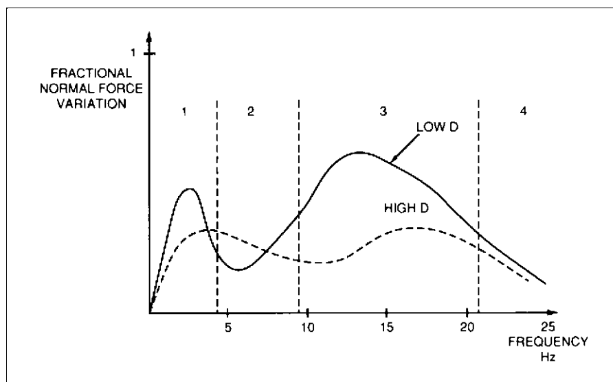
Fig. 13.1-18 Tire force variation.
