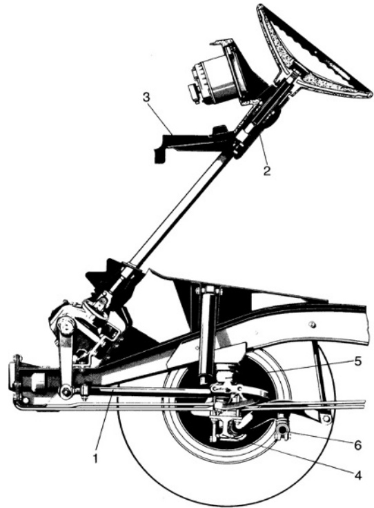
Fig. 8.1-37 The front rigid axle on the Mercedes-Benz light commercial vehicle of the 207 D/308 series with recirculating ball steering gear and steering rod 1 parallel to the two-layer parabolic spring. This rod has to be slightly shorter than the front side of the spring, so that both parts take on the same motion curve when the axle bottoms out (see also Fig. 9.1-6). The brace 3, running from the steering column jacket 2 to the body, bends on impact. The T-shaped axle casing 4, which is cranked downwards and to which the springs are fastened, can be seen in the section. The elastomer spring 5 sits on the longitudinal member of the frame and the two front wheels are joined by the tie rod 6. The safety steering wheel has additional padding.
