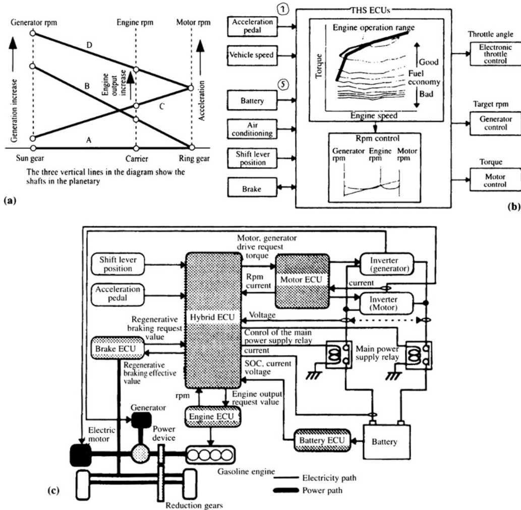
Fig. 7.1-15 Power-split control: (a) power interaction diagram; (b) THS control system; (c) ECU schematic.
