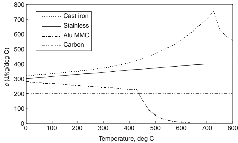
Fig. 15.1-28 Specific heat capacity, c , versus temperature, T .
