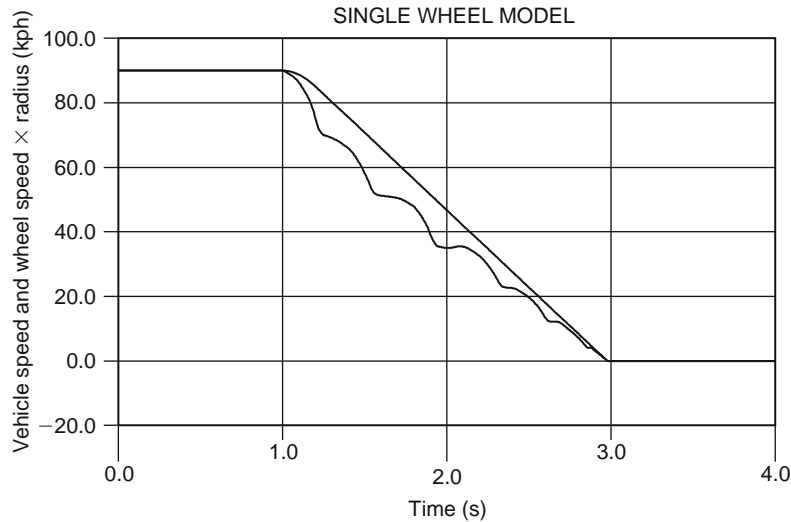
Fig. 15.1-32 Plot of vehicle speed and wheel speed during ABS braking simulation.
