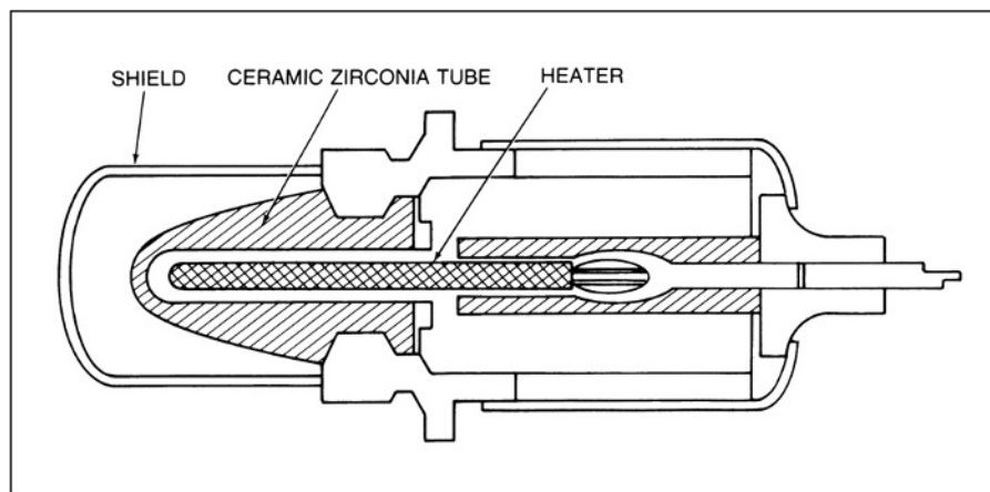
Fig. 4.1-18 Heated EGO sensor.
