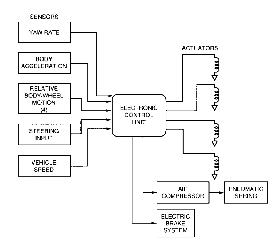
Fig. 13.1-22 Electronic suspension system.
