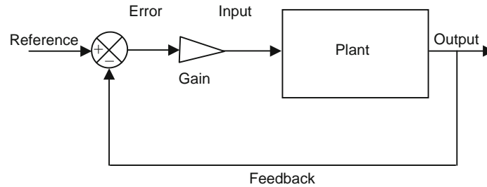
Fig. 15.1-41 An open-loop system, in black, is a subset of a closed-loop system, in grey.
