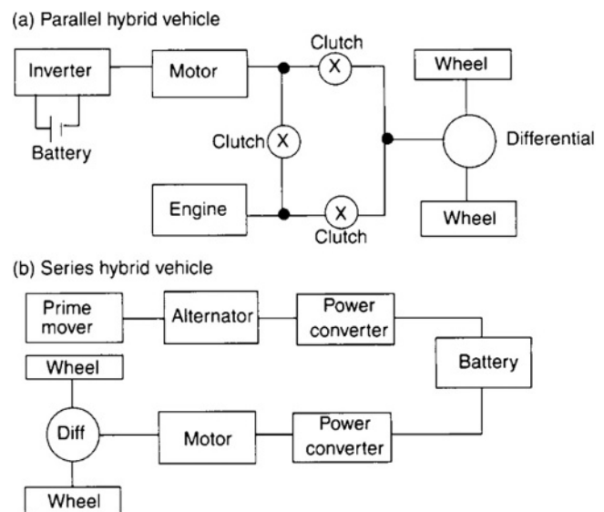
Fig. 7.1-1 Types of hybrid drive.
