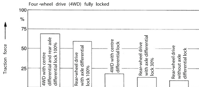
Fig. 8.1-66 Influence of the type of drive and differential lock on the propulsion force with \mu split', in other words, a slippery road surface with \mu_{x,w} = 0.1/0.8 on one side only. 100% locking of the rear axle differential gives most benefits. Some car manufacturers offer this option as ASR (or EDS) or using a hydraulic manual selection clutch. However, only 25% to 40% locking is provided on the multi-disc limited-slip differentials that have usually been fitted on vehicles to date.
