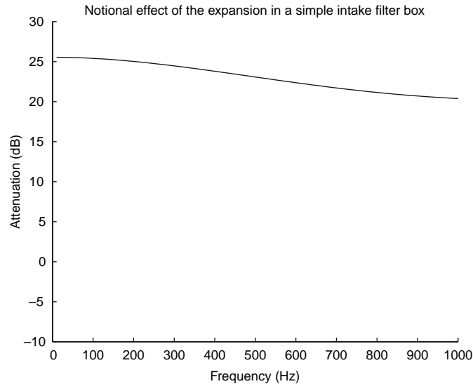
Fig. 22.1-30 Attenuation of the expansion section of a simple intake filter box calculated using APINEX software.
