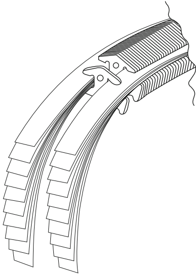
Fig. 5.1-28 The Van Doorne metal belt construction.
