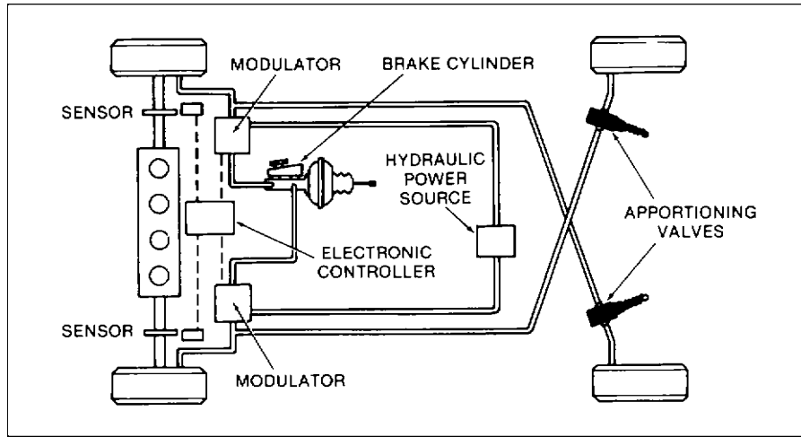
Fig. 13.1-12 Antilock braking system.
