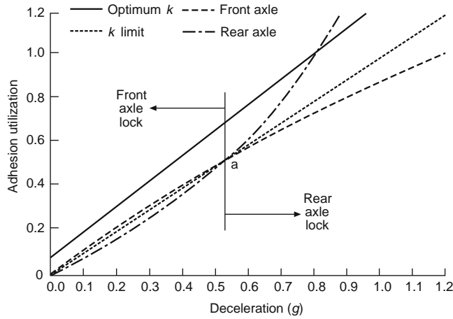
Figure 12.1-13a Adhesion utilization, datum prototype vehicle.
