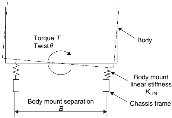
Fig. 16.1-8 Laterally positioned pair of body mountings.
