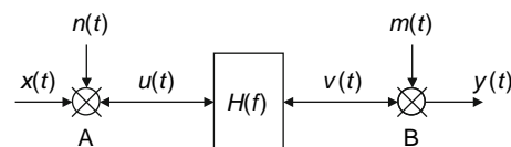
Fig. 21.1-2 Halvorsen and Bendat's single input/single output problem (1975).
