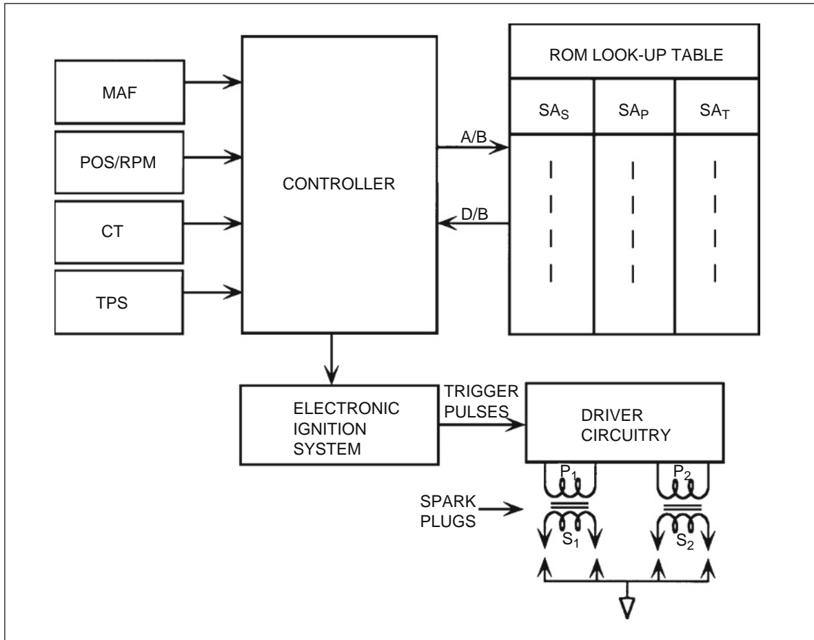
Fig. 4.1-9a Distributorless ignition system.
