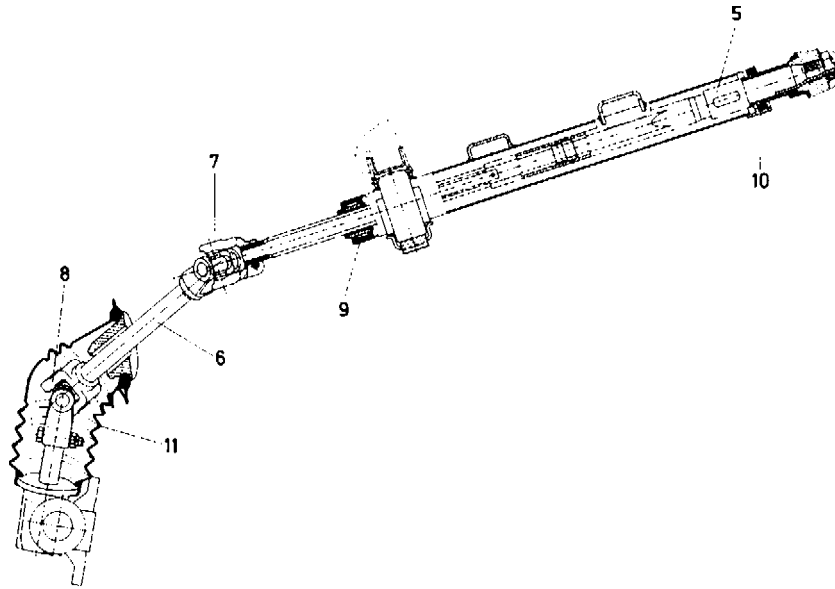
Fig. 9.1-26 Steering column of the VW Golf III and Vento (1996). The collapsible steering tube (Fig. 9.1-27) is carried from the bottom by the needle bearing 9 and through the top by the ball bearing 10 in the jacket tube; the spigot of the steering lock grips into part 5. The almost vertical pinion gear of the rack and pinion steering is linked to the inclined steering tube via the intermediate shaft 6 with the universal joints 7 and 8. The dashpanel is sealed by the gaiter 11 between this and the steering gear (illustration: Lemförder Fahrwerktechnik).
