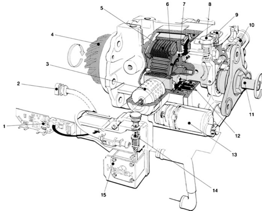
Fig. 8.1-73 Multi-disc clutch of the Swedish company Haldex, used in the Golf 4motion (1998) and Audi TT Quattro (1998). When there is a difference in speed between the front and rear axles, the disc cam 6 on the output shaft activates the working elements of the axial-piston pump 12 by means of the rollers 7. Via the control valve 14, the pressure produced activates the working piston which moves the discs. The torque transmitted is adjusted continuously by the control unit up to the maximum value, depending on the driving situation described by the wheel sensors, the signals from the slip and brake-power control systems, the position of the accelerator pedal, the engine speed etc. The clutch is disengaged when the ABS function is used. 1 electronic control unit, 2 connector vehicle (voltage, CAN, K leads), 3 oil filter, 4 shaft bevel wheel exit (rear axle gearing), 5 lamella, 6 cam plate, 7 coil, 8 relief valve, 9 pressure regulating valve, 10 accumulator, 11 input shaft, 12 axial piston pump, 13 pre-load pump, 14 control valve, 15 intermittent or step motor.
