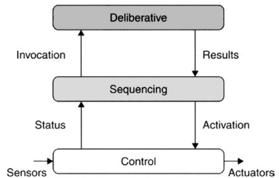
Fig. 14.2-7 ATLANTIS architecture (Gat).
