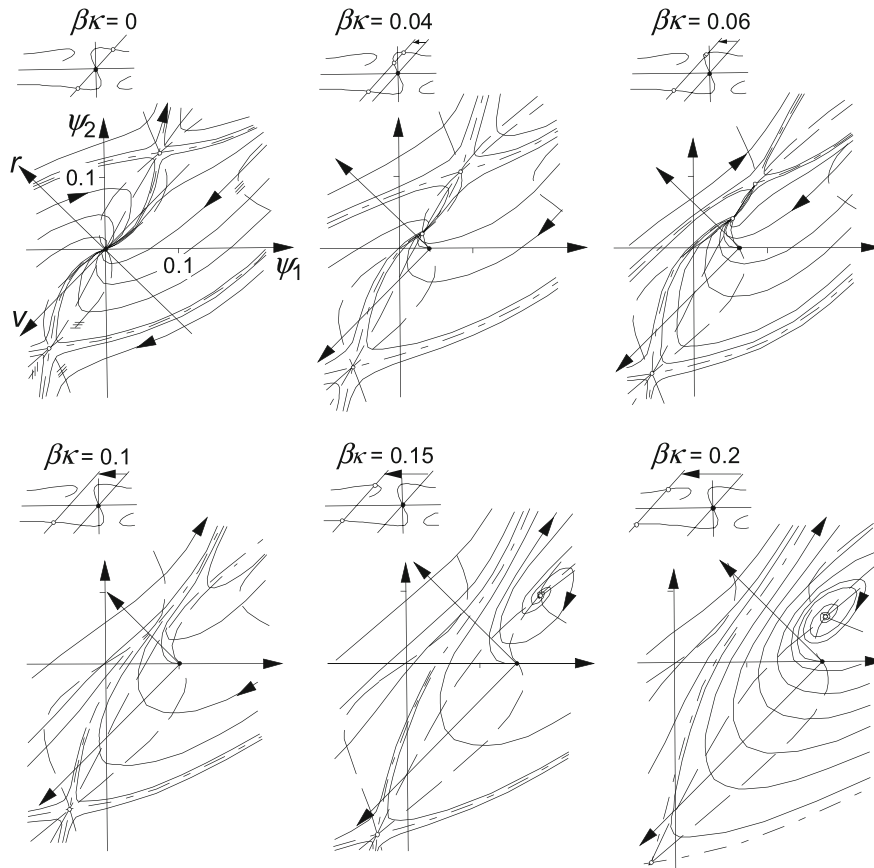
Fig. 11.1-23 Influence of steering on the stability margin (system of Fig. 11.1-20 (top)).
