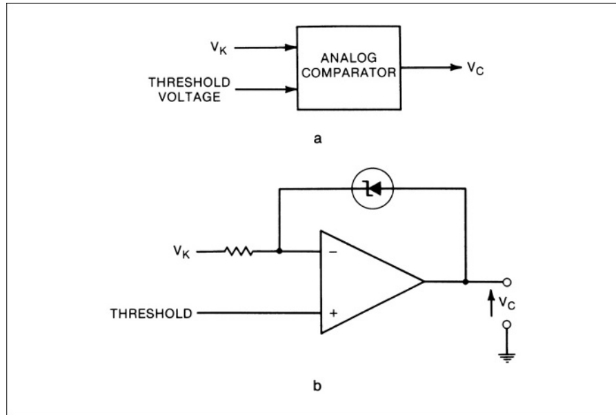
Fig. 4.1-14 Knock level detector circuit.
