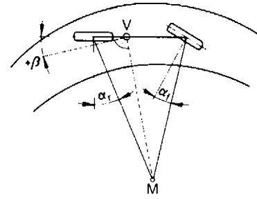
Fig. 10.1-42 If there is a greater slip angle \alpha_r on the rear wheels than on the front ( \alpha_f ), the vehicle oversteers. The positive angle describes the angle between the vehicle longitudinal axis and its speed at the centre of gravity.
