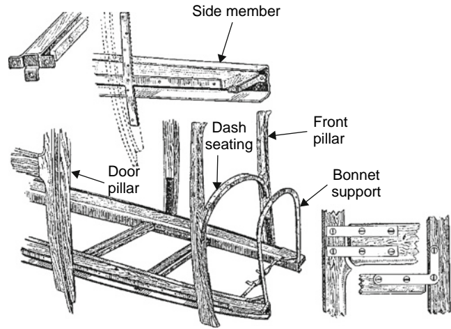
Fig. 16.1-7 Construction details of a timber framed 'fabric body'.
