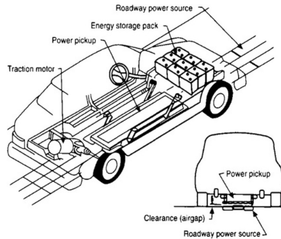
Fig. 6.1-13 Road-induced electricity.
