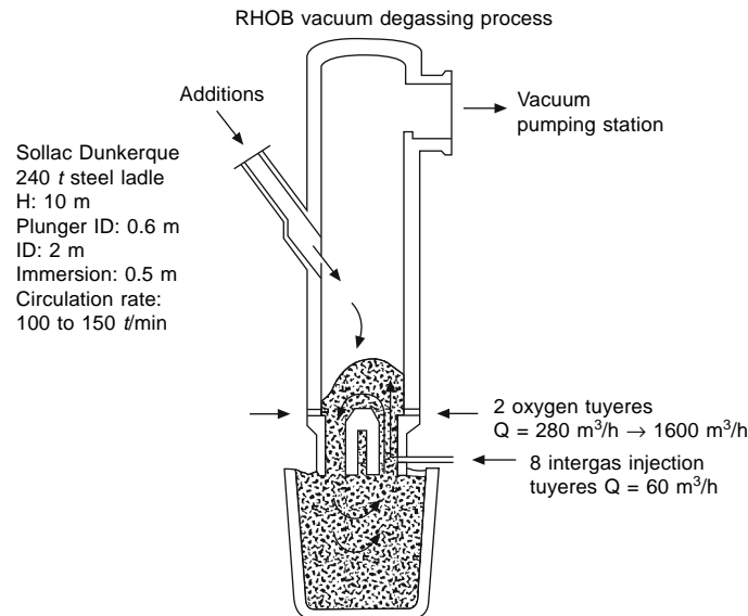
Fig. 18.2-3 Vacuum degassing in the steelmaking process. 3
