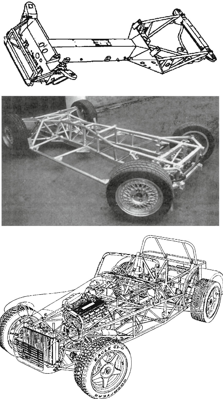
Fig. 18.1-4 Selection of alternative chassis designs. 2
