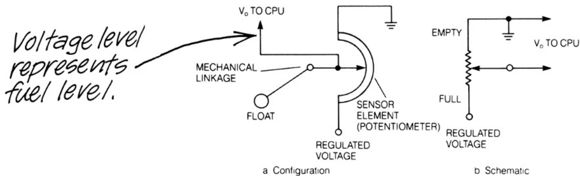
Fig. 23.1-10 Fuel quantity sensor.
