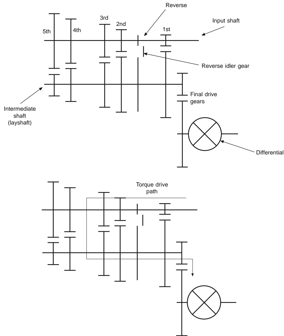
Fig. 5.1-7 Schematic of a front-wheel-drive gearbox gear layout.
