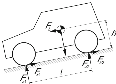
Fig. 11.1-26 The automobile subjected to longitudinal forces and the resulting load transfer.
