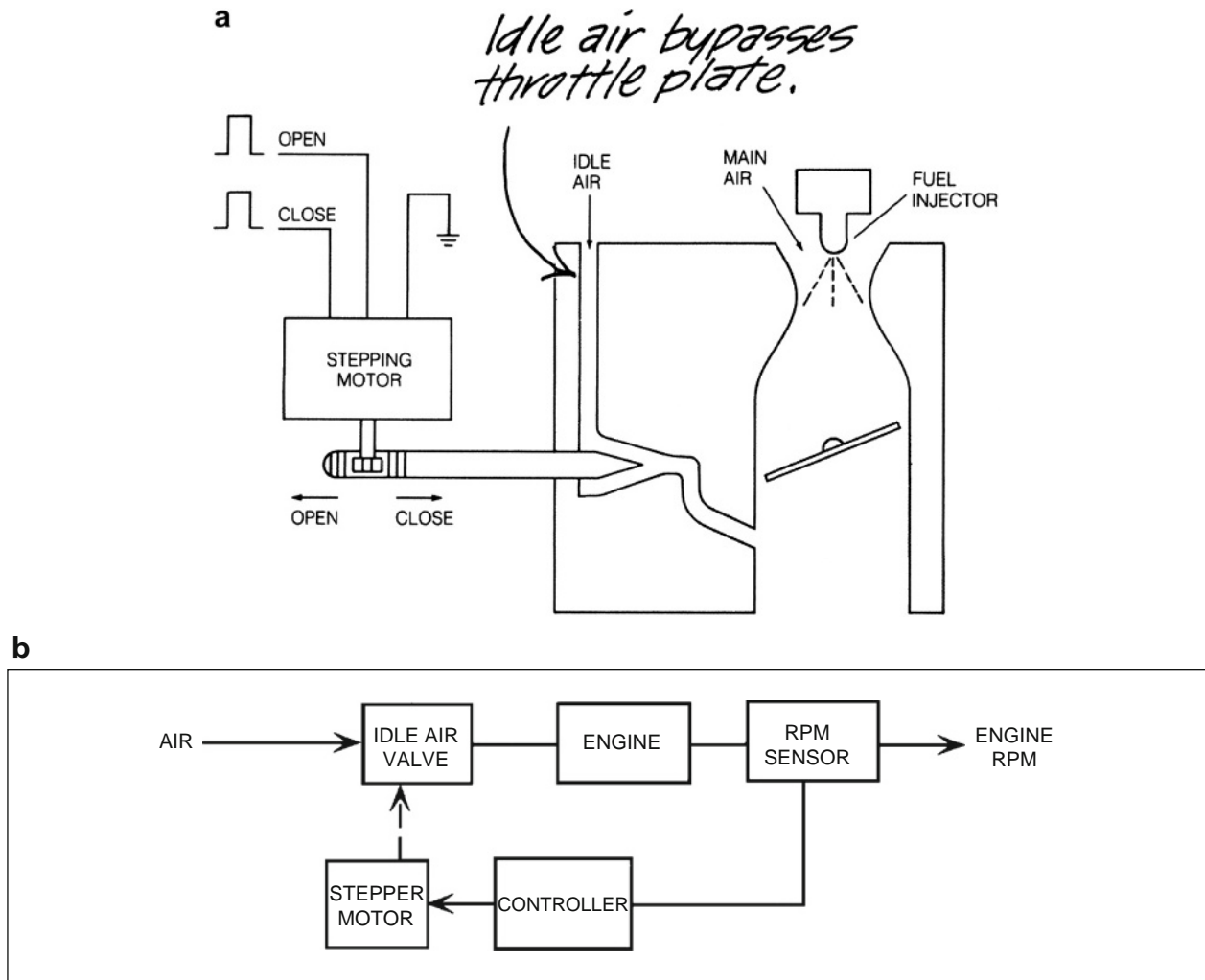
Fig. 4.1-7 Idle air control.
