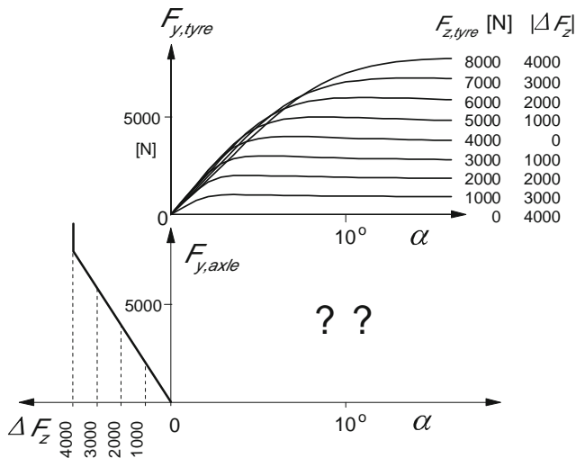
Fig. 11.1-8 The construction of the resulting axle cornering characteristics at load transfer (Exercise 11.1.1).
