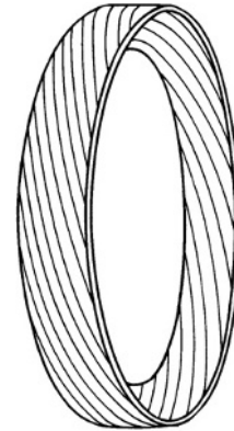
Fig. 10.1-4 The belt of the radial tyre sits on the substructure. The threads are at angles of between 15^\circ and 25^\circ to the plane of the tyre centre.
