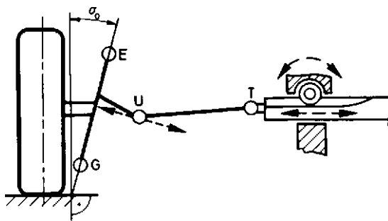
Fig. 9.1-34 When viewed from the rear, the inner tie rod joint T on rack and pinion steering moves parallel to the ground, whereas the outer tie rod joint U moves on an arc running vertical to the steering axis EG. Any caster angle \tau must also be considered.
