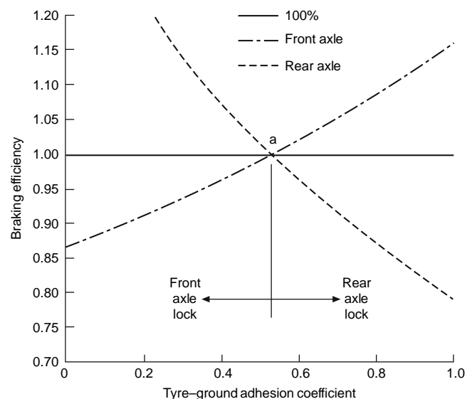
Figure 12.1-12 Efficiency as a function of tyre-ground adhesion.
