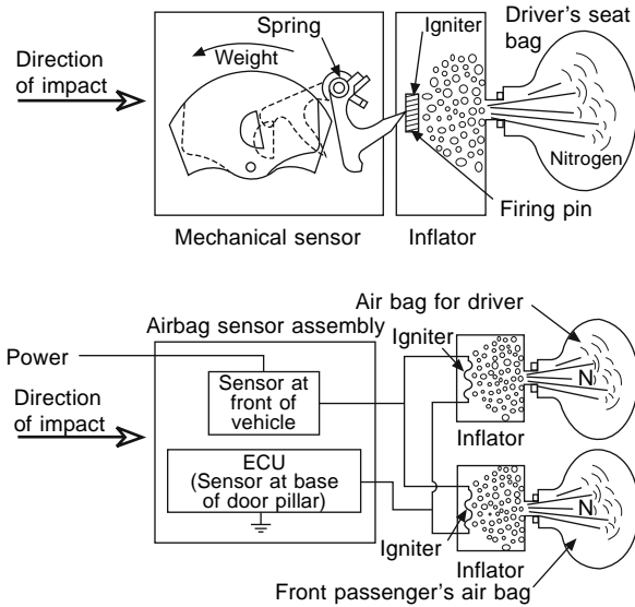
Fig. 17.1-12 Top , mechanically actuated bag firing mechanism; bottom , electrically actuated alternative. The latter has the advantages of greater compactness of the parts that may have to be accommodated in the steering wheel hub and the sensors and electronic control unit can be sited in the most appropriate positions.
