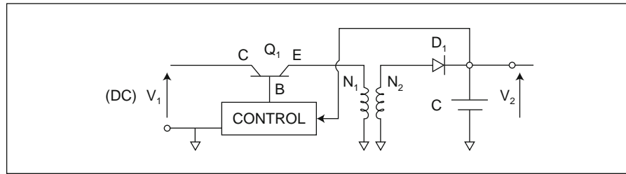
Fig. 4.1-23 DC to DC converter.
