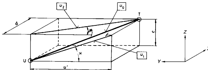
Fig. 9.1-32 On independent wheel suspensions, the tie rod UT is spatially inclined. The path u' (i.e. the lateral distance of points U and T from one another) or the angle \kappa must be determined when viewed from the rear. From the top view, the distance d or the angle \omega_0 is more important; the projected lengths which appear in both views are u_1 and u_2 . The true tie rod length is then: u_0 = (u'^2 + c^2 + d^2)^{1/2} .
