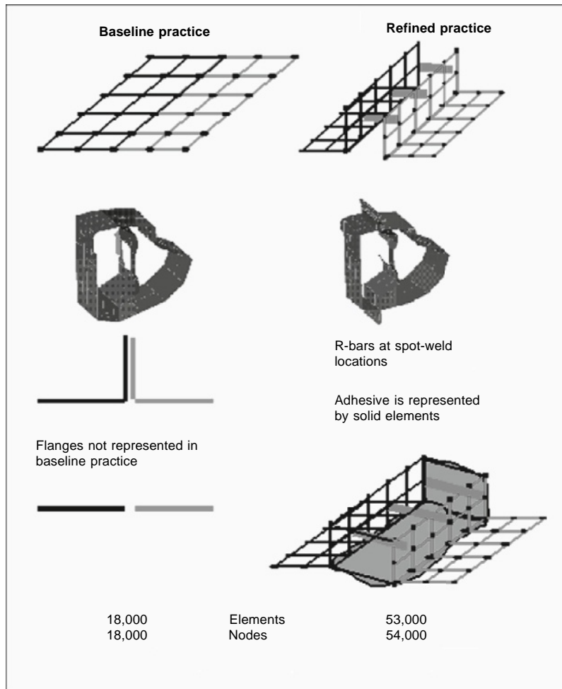
Fig. 18.1-37 FE representation of joints. 16 (Reprinted with permission from SAE paper 1999-01-3181 Copyright 1999 Society of Automotive Engineers Inc.)
