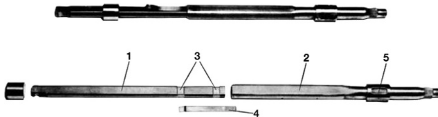
Fig. 9.1-27 Telescopic collapsible steering tubes consist of a lower part 1, which is flattened on the outside, and a hollow part 2, which is flattened on the inside. The two will be fitted together; the two plastic bushes 3 ensure that the assembly does not rattle and that the required shear-off force in the longitudinal direction is met. The tab 4 fixed to part 1 ensures the passage of electric current when the horn is operated. The spigot of the steering wheel lock engages with the welded-on half shells 5 (illustration: Lemförder Fahrwerktechnik).
