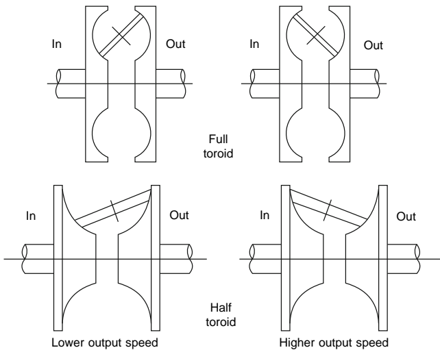
Fig. 5.1-31 The toroidal drive concept (full and half).
