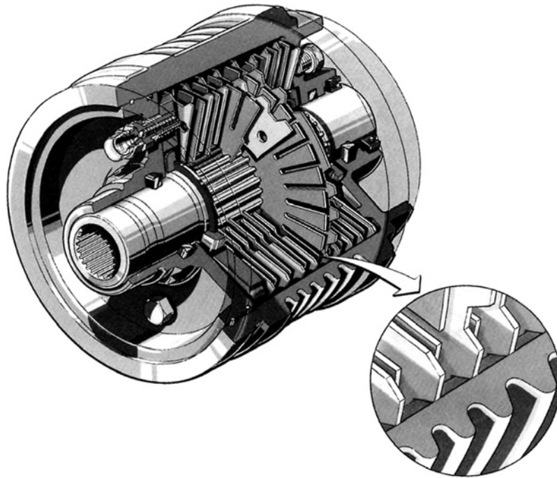
Fig. 8.1-74 Visco clutch with slip-dependent drive moment distribution. Two different packages sit in the closed drum-shaped housing: radially slit steel discs, which are moved by the serrated profile of the hollow shaft, and perforated discs which grip (as can be seen below) into housing keys. The shaft is joined with the differential and the casing with the propshaft going to the rear axle. The discs are arranged in the casing so that a perforated disc alternates with a slit one. The individual parts have no definite spacing but can be slid against one another axially. The whole assembly is filled with viscous silicone fluid and the torque behaviour (therefore the locking effect) can be adjusted via the filling level.
