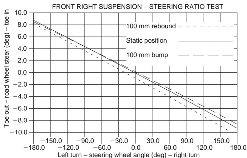
Fig. 15.1-40 Results of steering ratio test for MSC.ADAMS front right suspension model.
