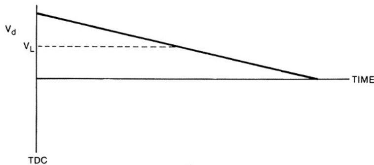
Fig. 4.1-12 Instrumentation and waveforms for closed-loop ignition control.
