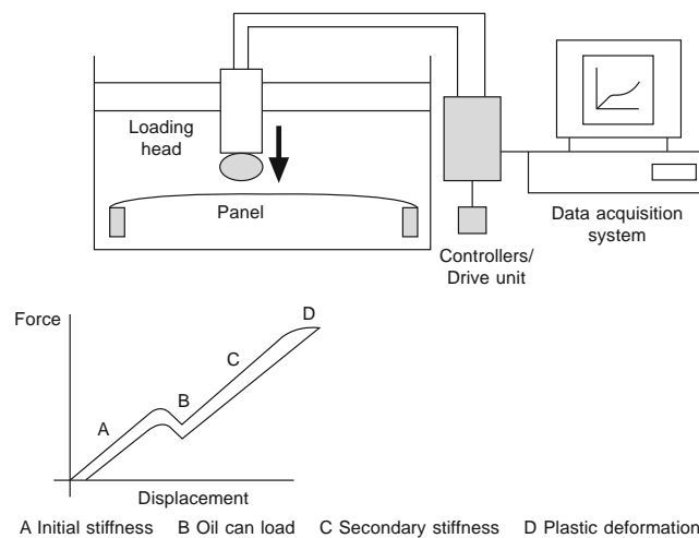
Fig. 18.1-20 Test rig for measurement of panel dent resistance and stiffness.
