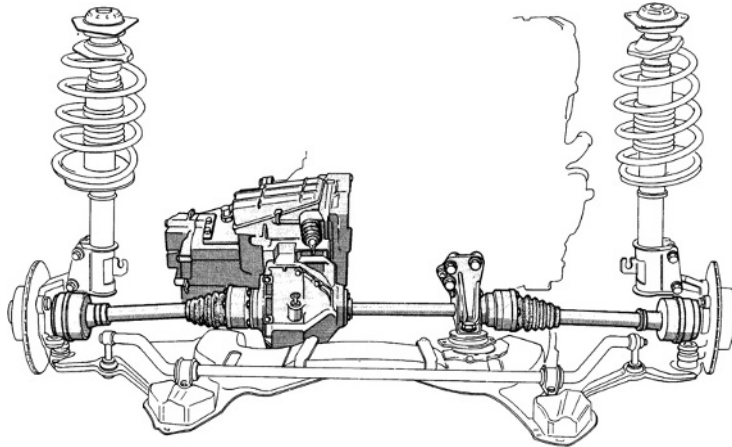
Fig. 8.1-51 Gearbox unit on the Lancia Thema, located beside the transverse engine and between the front axle McPherson struts. Owing to the high engine performance, the design features two equal-length axle shafts joined by an intermediate shaft. There are also internally ventilated disc brakes.
