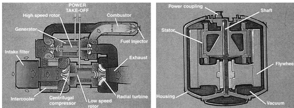
Fig. 6.1-8 Chrysler Patriot flywheel energy storage system: left, turbine; right, flywheel.
