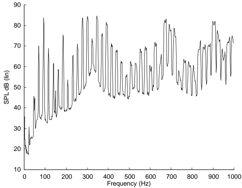
Fig. 22.1-19 Sound pressure levels recorded 100 mm from the intake orifice of a 1.6-litre four-cylinder gasoline engine running full load at 2800 rev min -1 .
