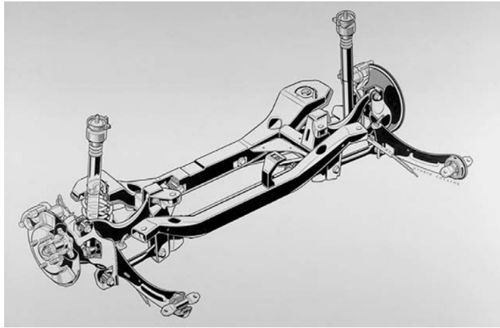
Fig. 8.1-18 Multi-link suspension of Ford Werke AG. Derived from the Mondeo Turnier model series, multi-link suspension is used by Ford for the first time in the Focus models (1998) in the segment of C class vehicles. This is called the ‘control sword axle’ after the shape of the longitudinal link. As there are five load paths available here, instead of the two that exist in twist-beam axles and trailing arm axles, there is great potential for improvement with regard to the adjustment of riding comfort, driving safety and noise and vibration insulation. As a result of a very elastic front arm bush, the high level of longitudinal flexibility necessary for riding comfort is achieved. At the same time, very rigid and accurate wheel control for increased driving safety is ensured by the transverse link, even at the stability limit. The longitudinal link is subject to torsional stress during wheel lift and to buckling stress when reversing. By using moulded parts, it was possible to reduce the unsprung masses by 3.5 kg per wheel.
