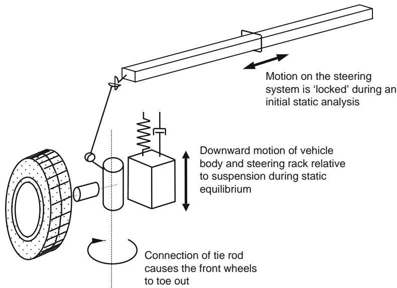
Fig. 15.1-37 Toe change in front wheels at static equilibrium for simple models. (This material has been reproduced from the Proceedings of the Institution of Mechanical Engineers, K2 Vol. 213 'The modelling and simulation of vehicle handling. Part 2: vehicle modelling', M.V. Blundell, page 129, by permission of the Council of the Institution of Mechanical Engineers.)
