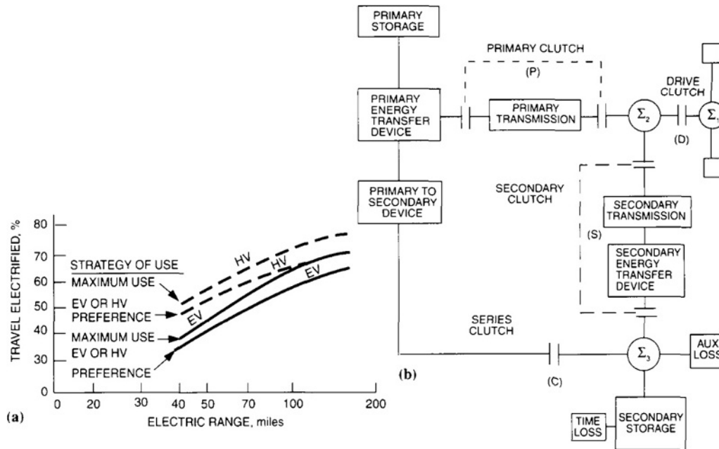
Fig. 7.1-4 Justifying the hybrid: (a) EV traffic potential; (b) combined series-parallel mode.
