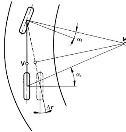
Fig. 8.1-29 If a rigid rear axle steers with the angle \Delta r towards understeer, the tail moves out less in the bend and the driver has the impression of more neutral behaviour. Moreover, there is increased safety when changing lanes quickly at speed. The same occurs if the outside wheel of an independent wheel suspension goes into toe-in and the inside wheel goes into toe-out.
