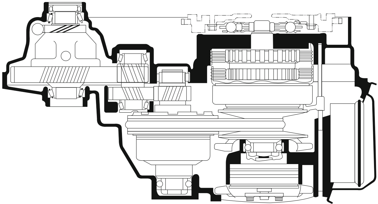
Fig. 5.1-30 A complete push belt transmission.
