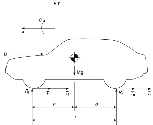
Figure 12.1-9 Free body diagram of the decelerating vehicle.
