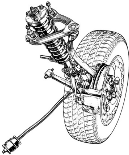
Fig. 8.1-55 Double wishbone front suspension on the Honda models, Prelude and Accord, with short upper wishbones with widely spaced bearings, lower transverse control arms and longitudinal rods whose front mounts absorb the dynamic rolling stiffness of the radial tyres. The spring shock absorbers are supported via fork-shaped struts on the transverse control arms and are fixed within the upper link mounts. This point is a good force input node. Despite the fact that the upper wheel carrier joint is located high, which gives favourable wheel kinematics, the suspension is compact and the bonnet can be low to give aerodynamic advantages. The large effective distance c between the upper and lower wheel hub carrier joints seen in Fig. 8.1-5 results in low forces in all mounts and therefore less elastic deflection and better wheel control.
