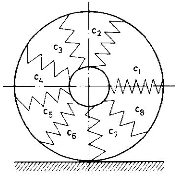
Fig. 10.1-30 The tyre spring rate can fluctuate depending on the manufacturing process, shown as c_1 to c_8 .
