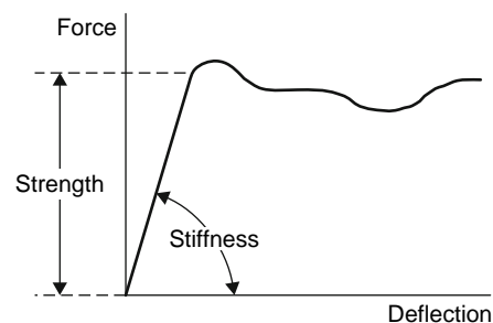
Fig. 16.1-1 The concepts of stiffness and strength.
