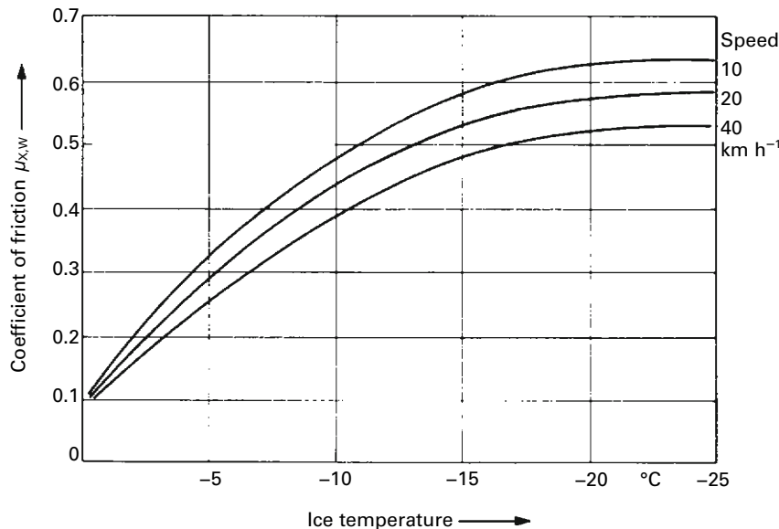
Fig. 10.1-36 Influence of ice temperature and car speed on the coefficient of friction \mu_{x,w} of an 82 series winter tyre; the extremely low values at 0°C can be seen clearly.
