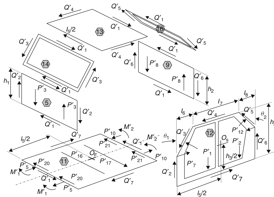
Fig. 16.2-28 Baseline model (torsion box) – lateral loading.
