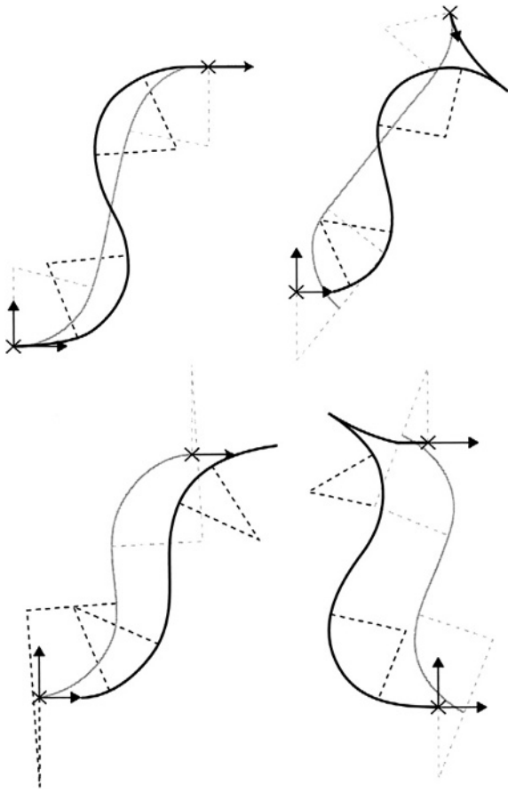
Fig. 14.2-32 RS (in grey) versus CC paths (in black).
