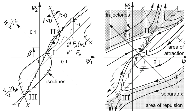
Fig. 11.1-22 Isoclines for the construction of trajectories in the phase-plane. Also shown: the three singular points I, II and III (cf. Fig. 11.1-17) and the separatrices constituting the boundary of the domain of attraction. Point I represents the stable cornering motion at steer angle \delta .
