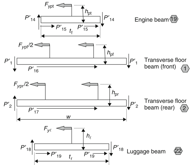
Fig. 16.2-25 Baseline model cross-beams – lateral loading.
