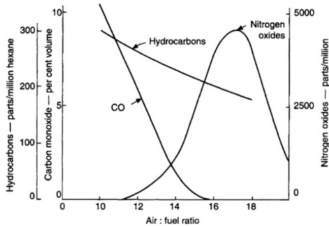
Fig. 3.1-1 Effect of air:fuel ratio on exhaust emissions.
