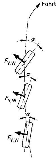
Fig. 10.1-39 Increasing lateral forces F_{Y,W} during cornering caused by the centrifugal force F_{c,v} leads to increasing slip angles \alpha .
