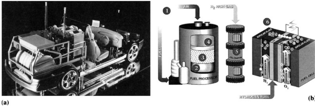
Fig. 6.1-25 Liquid hydrogen or reformed fuel: (a) Renault cryogenic storage: (b) Arthur D. Little reformer.
