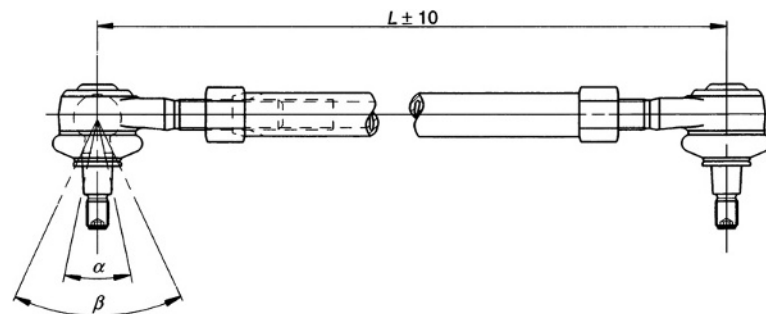
Fig. 9.1-13 Configuration of an adjustable tie rod with pre-lubricated joints and buckling-resistant central tube, the interior of which has a right-hand thread on one side and a left-hand thread on the other. It can usually be continuously adjusted by \pm 10 mm. When toe-in has been set, the length on the right and left tie-rod may differ, resulting in unequal steering inputs and different size turning circles; for this reason, the central tube should be turned the same amount on the left and right wheel. The configuration shown in the illustration is used on rigid front axles and as a drag link (illustration: Lemförder Fahrwerktechnik).
