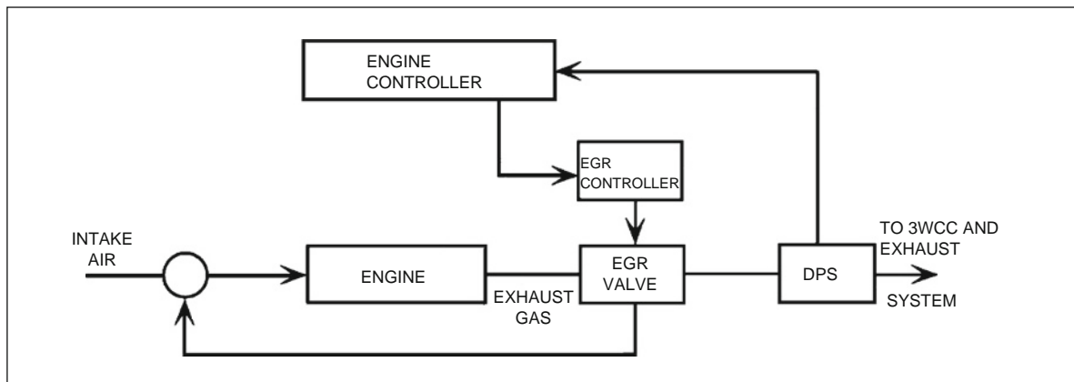
Fig. 4.1-8a EGR control.
