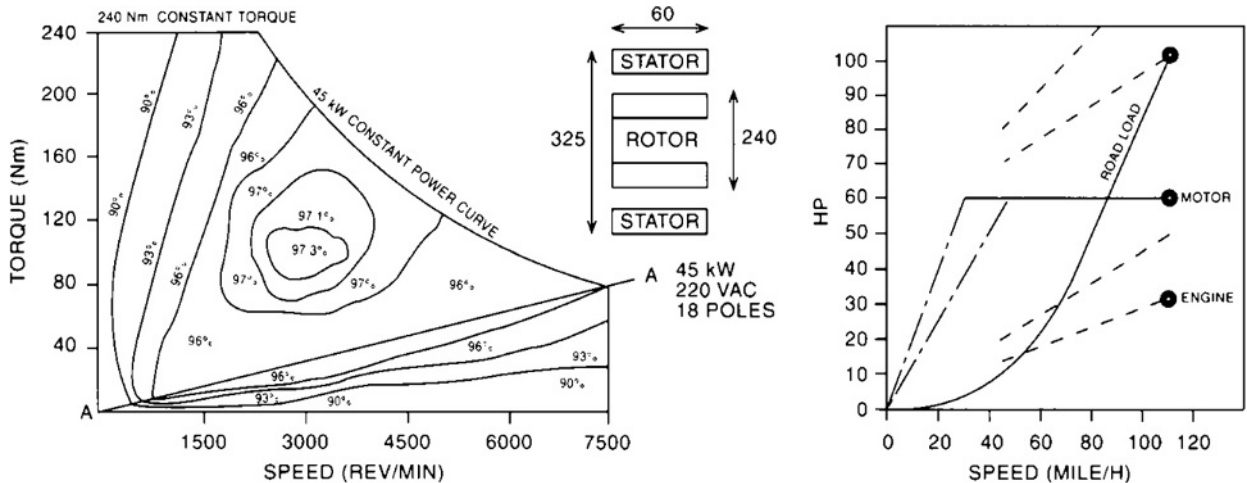
Fig. 7.1-6 Efficiency map, torque/speed curves and load matching.
