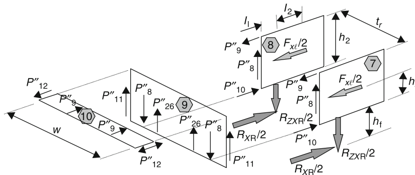
Fig. 16.2-32 Baseline model (rear structure) – braking loads.
