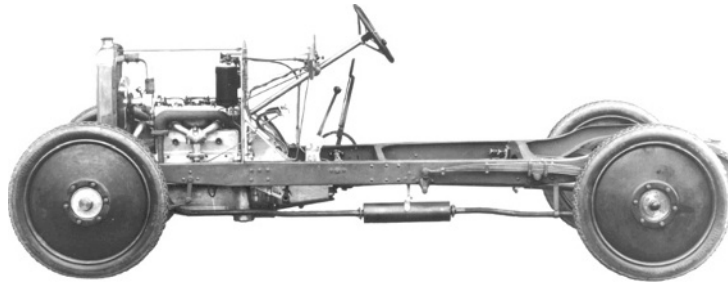
Fig. 16.1-2 Open section ladder frame chassis of the 1920s (courtesy of Vauxhall Archive Centre).
