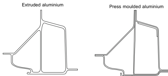
Fig. 18.1-22 Sill sections produced from pressed parts compared with extruded sections. 9
