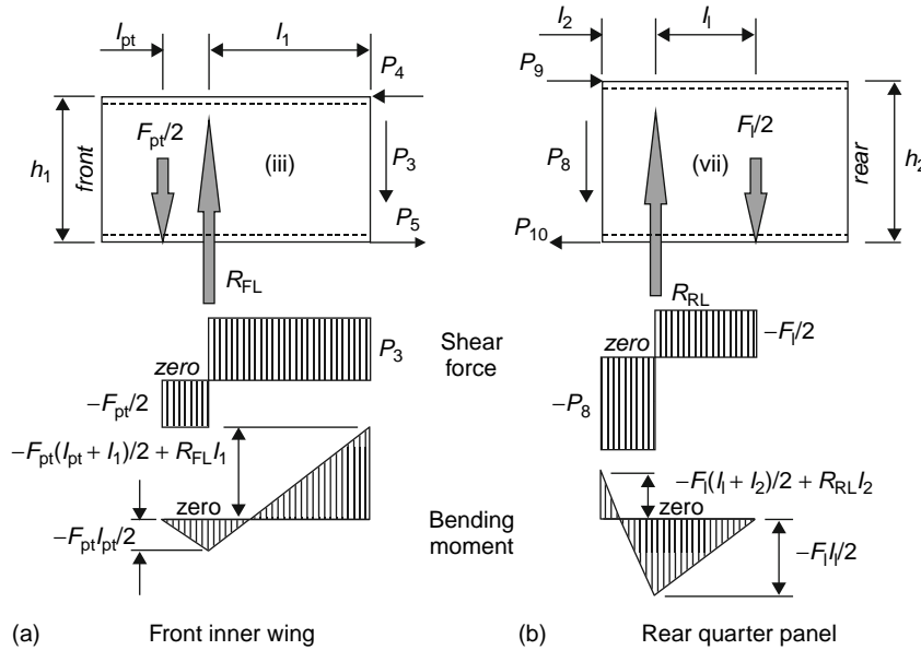
Fig. 16.2-6 Shear force and bending moment diagrams.
