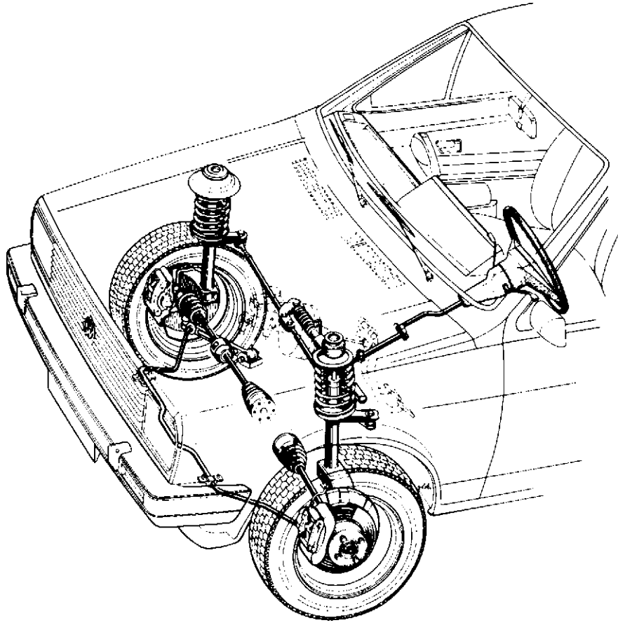
Fig. 9.1-1 Damper strut front axle of a VW Polo (up to 1994) with 'steering gear', long tie rods and a 'sliding clutch' on the steering tube; the end of the tube is stuck onto the pinion gear and fixed with a clamp. The steering arms, which consist of two half shells and point backwards, are welded to the damper strut outer tube. An 'additional weight' (harmonic damper) sits on the longer right drive shaft to damp vibrations. The anti-roll bar carries the lower control arm. To give acceptable ground clearance, the back of it was designed to be higher than the fixing points on the control arms. The virtual pitch axis is therefore in front of the axle and the vehicle's front end is drawn downwards when the brakes are applied.
