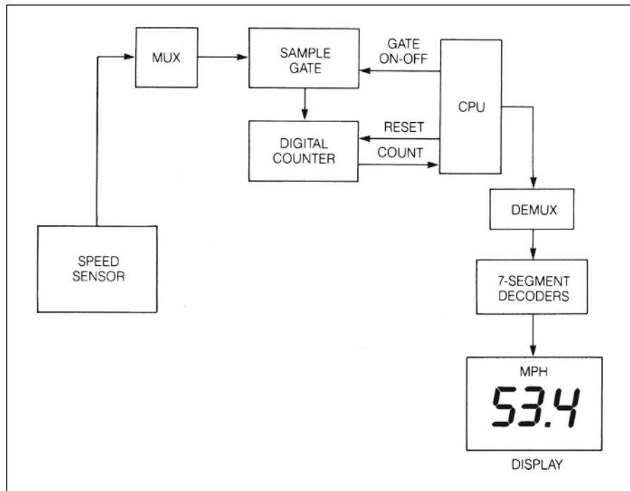
Fig. 23.1-15 Vehicle speed measurement.
