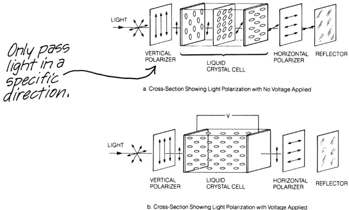
Fig. 23.1-17 Liquid crystal polarization.
