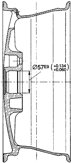
Fig. 10.1-24 Hayes Lemmerz alloy wheel for the Audi 80, made of the aluminium alloy GK-Al Si 7 Mg wa. The wheel has a double-hump rim (H2) and middle centring and is fixed with four spherical collar bolts. The different wall thicknesses, which are important for the strength, the shape of the bolt hole, the different shape of the drop-rim and the position of the valve hole are clearly shown. At high speeds the snap-fit valve (Fig. 10.1-6) is pressed outwards by the centrifugal force and supported below the rim base.
