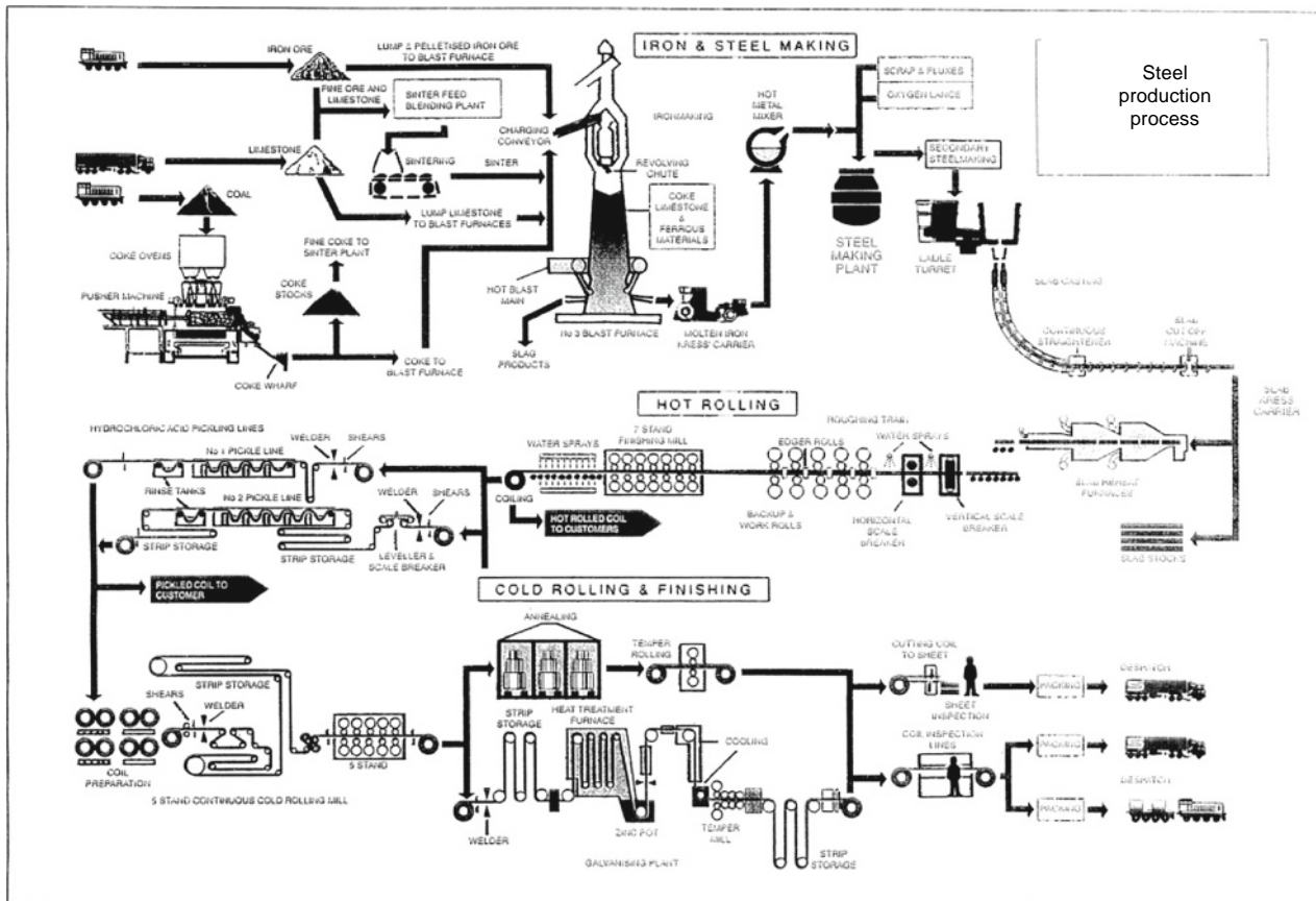
Fig. 18.2-2 (a) Typical sheet metal steel manufacturing process.
