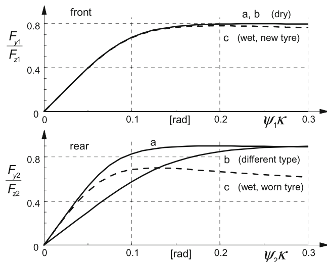
Fig. 11.1-21 Three sets of hypothetical axle cornering characteristics (Exercise 11.1.3).
