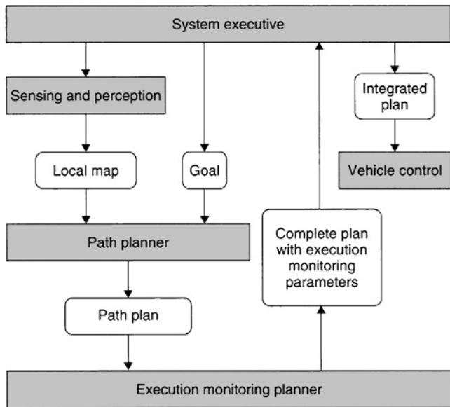
Fig. 14.2-2 JPL exploratory robot architecture (Gat).
