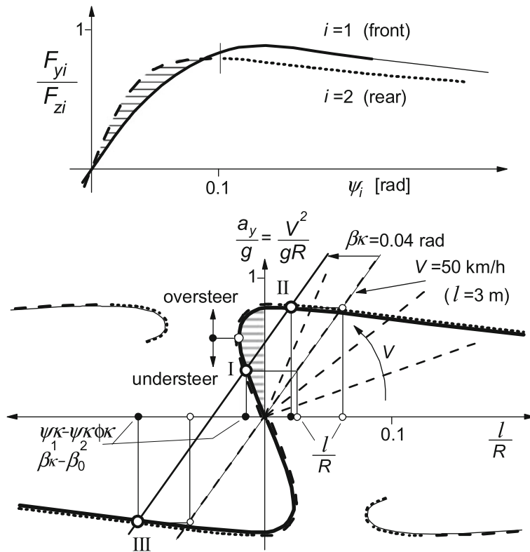
Fig. 11.1-17 Handling diagram resulting from normalised tyre characteristics. Equilibrium points I, II and III (steady turns) of which only I is stable, arise for speed V = 50 km/h and steer angle \delta = 0.04 rad. From the different line types the manner in which the curves are obtained from the upper diagram may be retrieved.
