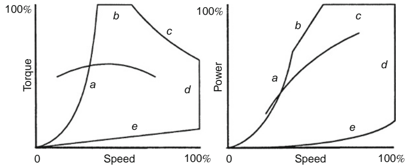
Fig. 2.1-13 Engine torque curves plotted on hydraulic dynamometer torque curves.
