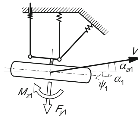
Fig. 11.1-5 Wheel suspension and steering compliance resulting in additional steer angle \psi_1 .
