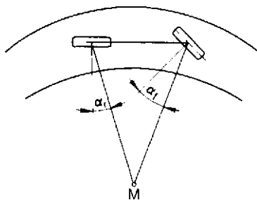
Fig. 10.1-41 If there is a greater slip angle \alpha_f on the front wheels than \alpha_r on the rear, the vehicle understeers.
