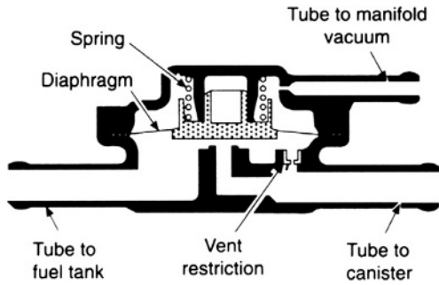
Fig. 3.1-19 Fuel tank pressure control valve. When the engine is not running, the valve is closed by the spring and the tank is then vented only through the restriction.
