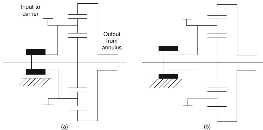
Fig. 5.1-21 Single epicyclic sun locked to carrier and sun locked to frame. (a) Sun shaft locked to carrier shaft, (b) sun shaft held stationary.
