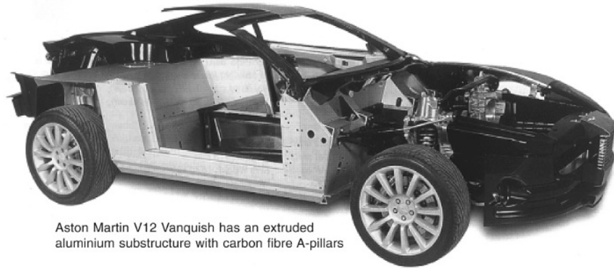
Fig. 18.1-33 Side view of Vanquish.
