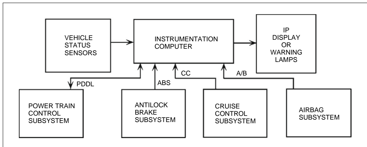
Fig. 23.1-2 Computer-based instrumentation system.
