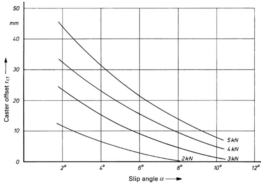
Fig. 10.1-50 Caster offset of tyre r_{\tau,T} calculated from Figs. 10.1-45 and 10.1-49 for 175/70 R 13 82 S steel radial tyres at p_T = 2.0 bar. The higher the vertical force F_{Z,W} (in kN) and the smaller the angle \alpha , the longer is r_{\tau,T} .
