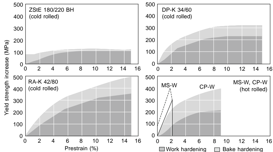
Fig. 18.2-13 Contribution of work hardening and bake hardening in HSS. (Diagram courtesy of TK5.)
