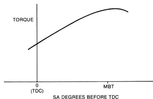
Fig. 4.1-10 Torque versus SA for typical engine.
