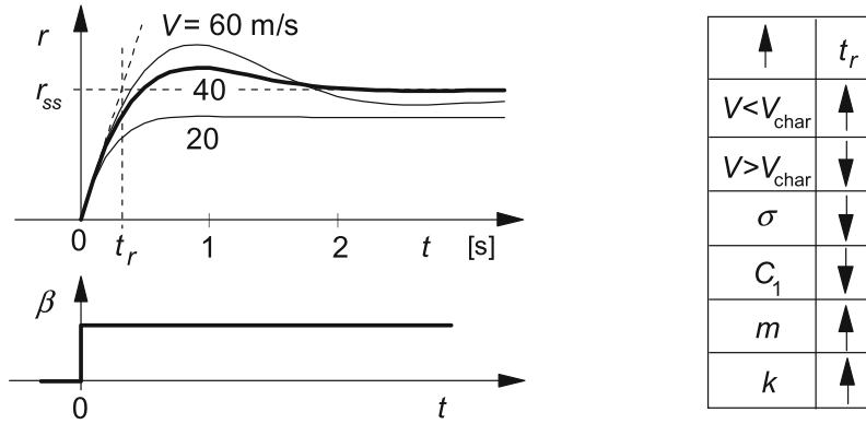
Fig. 11.1-14 Step response of yaw rate to steer angle. Parameters according to Table 11.1-1. Parameter influence on the rise time t_r .
