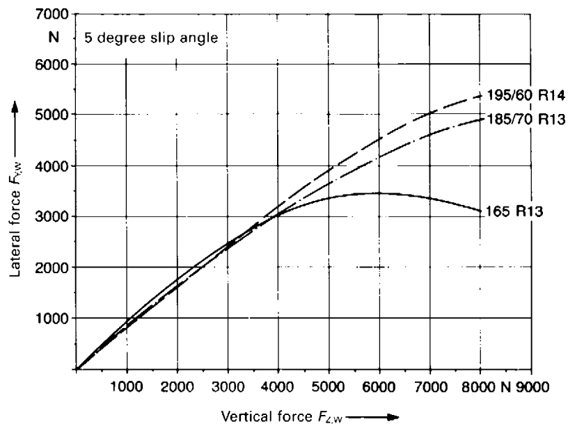
Fig. 10.1-46 Lateral force F_{y,w} dependent on vertical force F_{z,w} and tyre sizes of different H/W ratios: 165 R 13 82 H, 185/70 R 13 85 H and 195/60 R 14 85 H. Up to F_{z,w} = 4000 N the curves are more or less the same, but at higher loads the more favourable lateral cornering properties of the wide tyre are evident.
