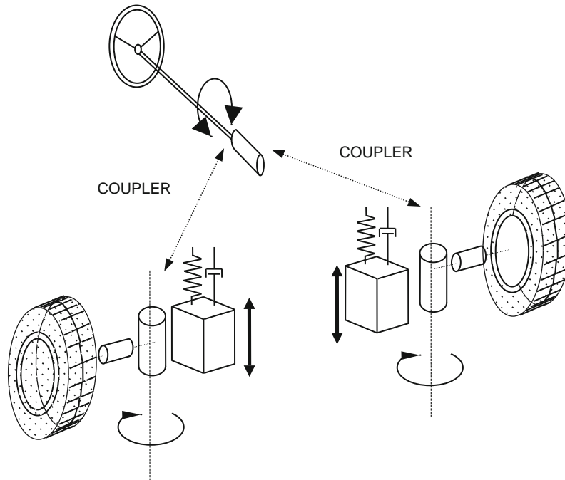
Fig. 15.1-38 Coupled steering system model. (This material has been reproduced from the Proceedings of the Institution of Mechanical Engineers, K2 Vol. 213 'The modelling and simulation of vehicle handling. Part 2: vehicle modelling', M.V. Blundell, page 130, by permission of the Council of the Institution of Mechanical Engineers.)
