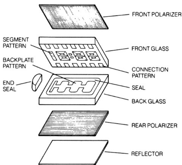
Fig. 23.1-16 Typical LCD construction.
