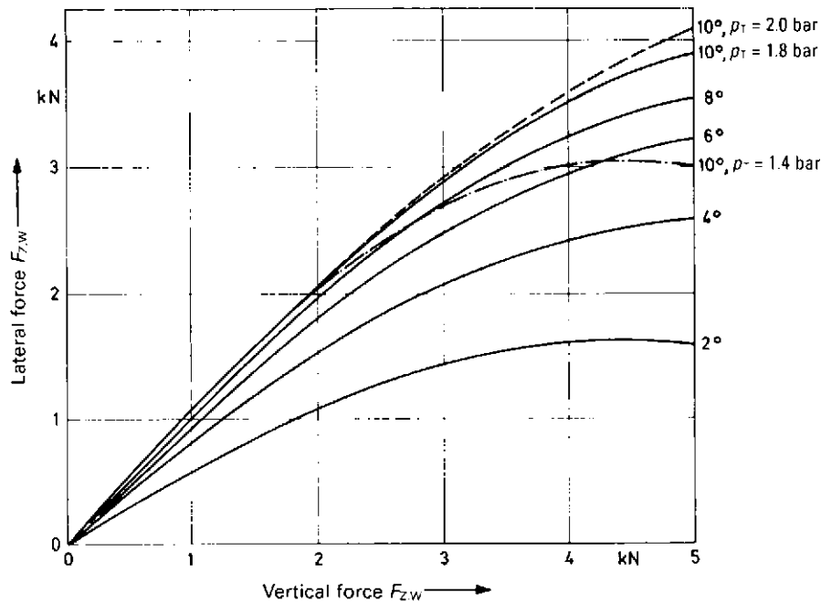
Fig. 10.1-44 Lateral cornering forces of the 155 R 13 78 S '82 series' steel radial tyre, measured on a dry drum at p_T = 1.8 bar. The load capacity at this pressure is around 360 kg, corresponding to a vertical force F_{Z,W} = 3.53 kN. Also shown are the forces at \alpha = 10^\circ and P_T = 1.4 bar and 2.0 bar to indicate the influence of the tyre pressure on the lateral cornering properties.
