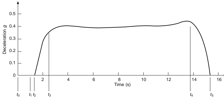
Figure 12.1-4 Typical measured deceleration time history.
