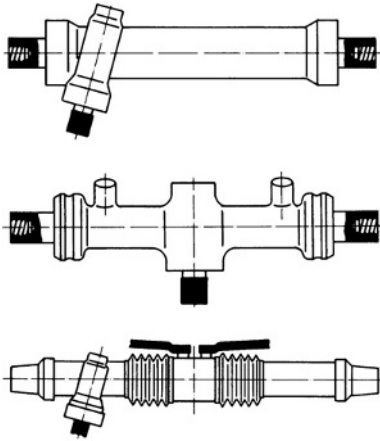
Fig. 9.1-8 The three most common types of rack and pinion steering on left-hand drive passenger cars; right-hand drive vehicles have the pinion gear on the other side on the top and bottom configurations (shown in Fig. 9.1-39). The pinion gear can also be positioned in the centre to obtain longer steering rod travel.
