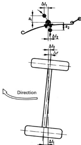
Fig. 8.1-28 Angled longitudinal leaf springs fixed lower to the body at the front than at the back cause the rigid rear axle to self-steer towards understeering (so-called roll pitch understeering). Where there is body roll, the wheel on the outside of the bend, which is compressing along the path s_1 , is forced to accommodate a shortening of the wheel base \Delta l_1 , whilst the wheel on the inside of the bend, which is extending by s_2 , is forced to accommodate a lengthening of the wheel base by \Delta l_2 . The axle is displaced at the steering angle \Delta r .
