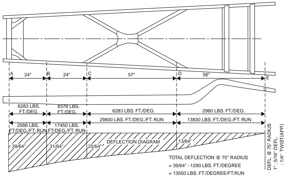
Fig. 16.1-10 Cruciform-braced chassis frame (Booth 1938 by permission Council of I.Mech.E.).
