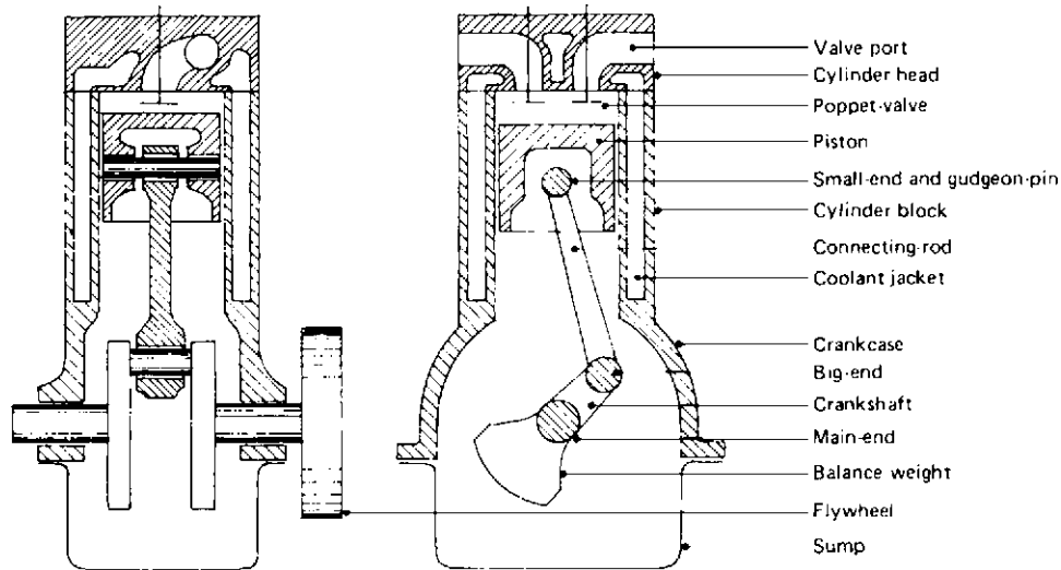
Fig. 1.1-2 Sectional view of the basic engine.
