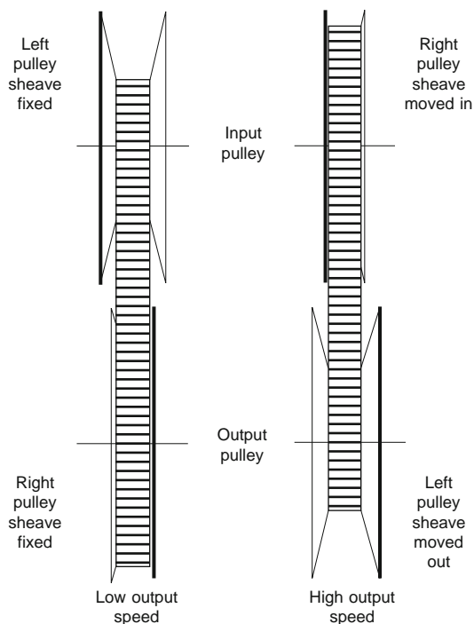
Fig. 5.1-27 Variable pulley drive concept.
