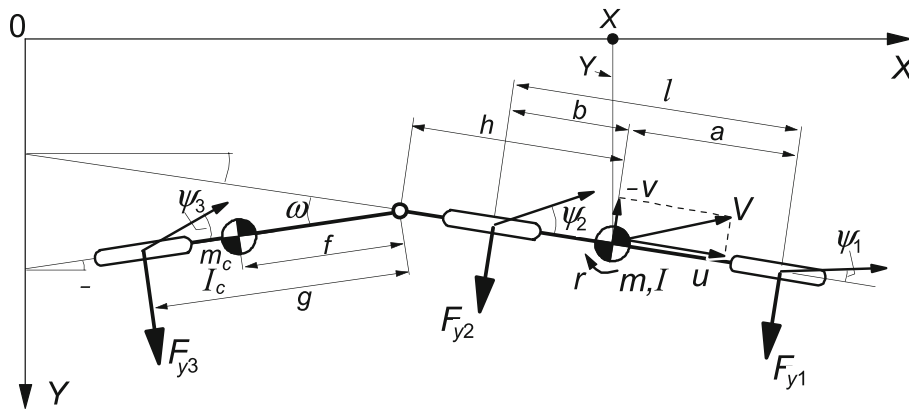
Fig. 11.1-29 Single-track model of car trailer combination.
