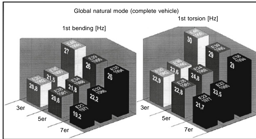
Fig. 18.1-9 Progressive improvement in dynamic stiffness with successive generations of BMW vehicles.
