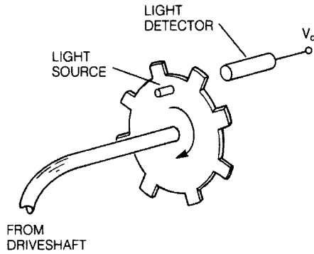
Fig. 13.1-5a Digital speed sensor.
