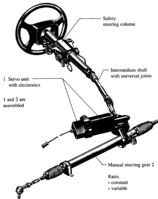
Fig. 9.1-21 Electrical power steering system by ZF. The servo unit acts directly upon the pinion of the rack and pinion steering. Consequently, the amount of stress to which the pinion is subjected increases by the amount of steering boost, compared with a mechanical or hydraulic power steering system.
