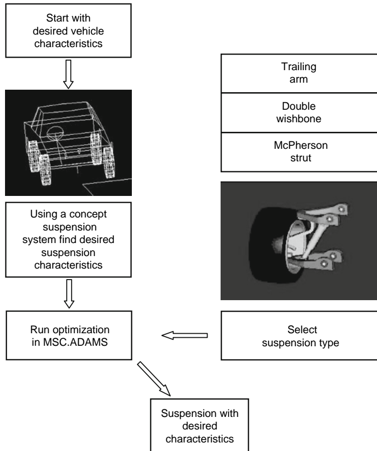
Fig. 15.1-11 Application of a concept suspension model (provided courtesy of MSC.Software).
