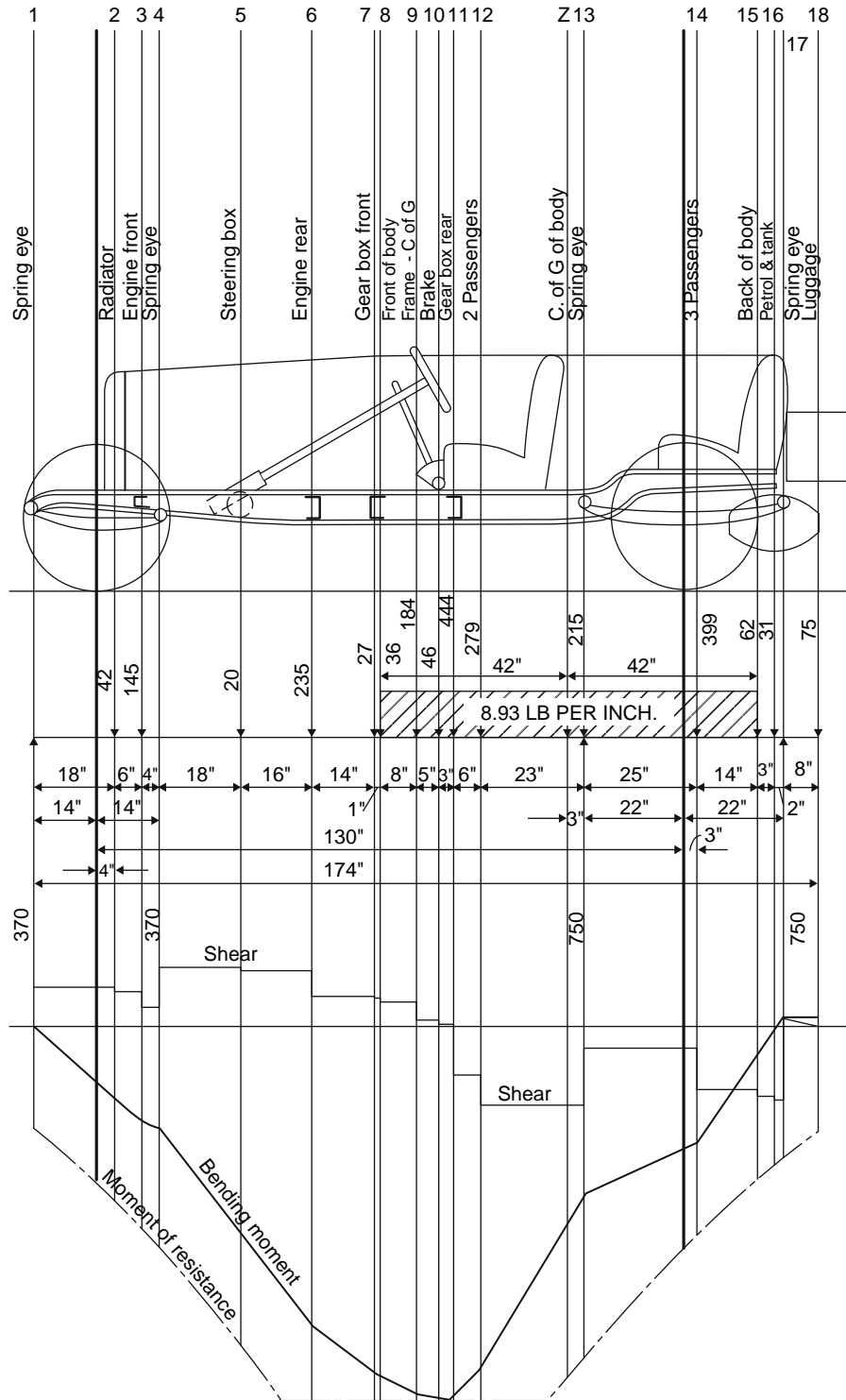
Fig. 16.1-4 Chassis structural analysis diagram (Donkin 1925).
