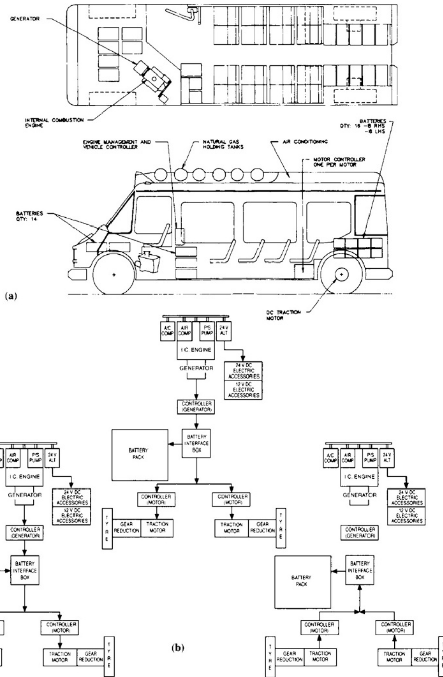
Fig. 7.1-18 Unique Mobility small hybrid bus: (a) Unique Mobility midibus; (b) power flow charts.
