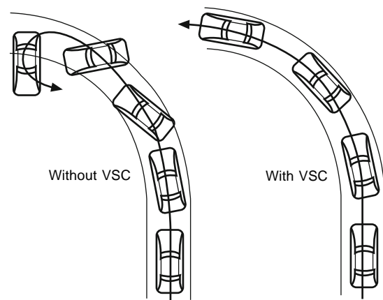
Fig. 17.1-18 Left , diagram showing the path typical of an oversteering car driven beyond the limit of adhesion of the wheels on the road, compared with, right , one driven in the same manner but equipped with vehicle stability control.
