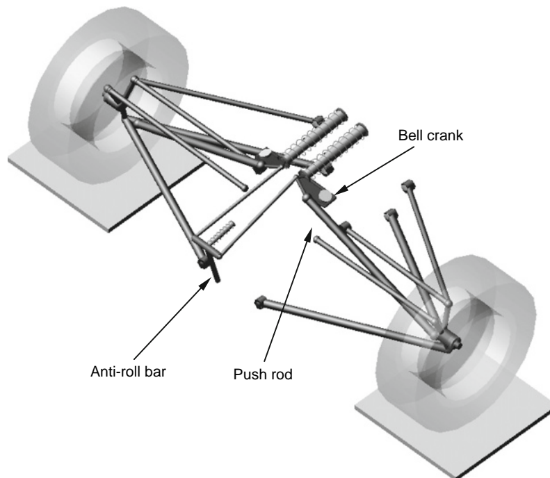
Fig. 15.1-19 Graphic of anti-roll bar in typical student race vehicle (provided courtesy of MSC.Software).
