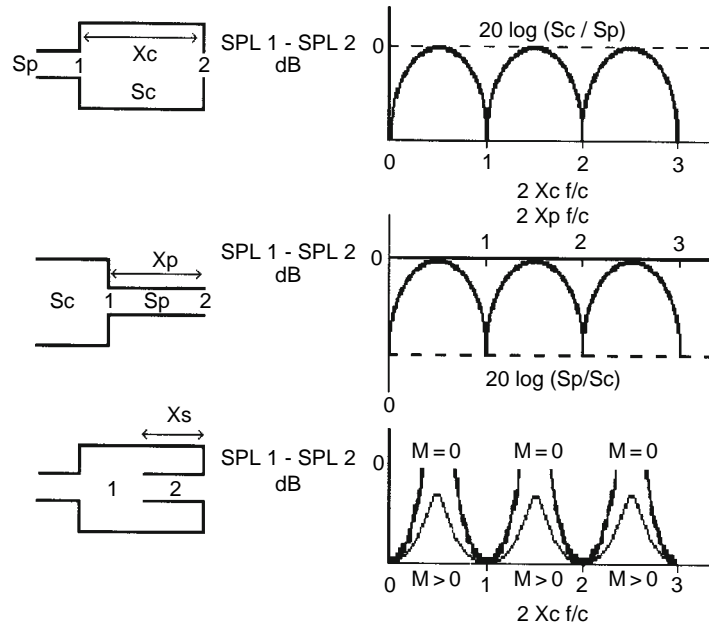
Fig. 22.1-21 The performance of silencer elements in the absence of flow or temperature gradients.
