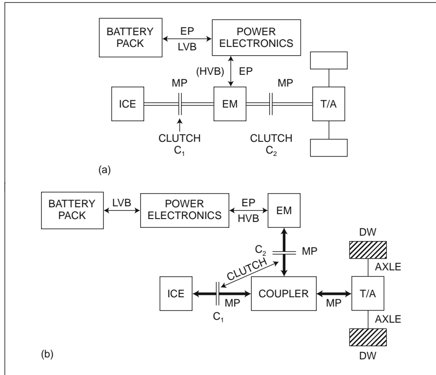
Fig. 4.1-21 Parallel hybrid schematic.
