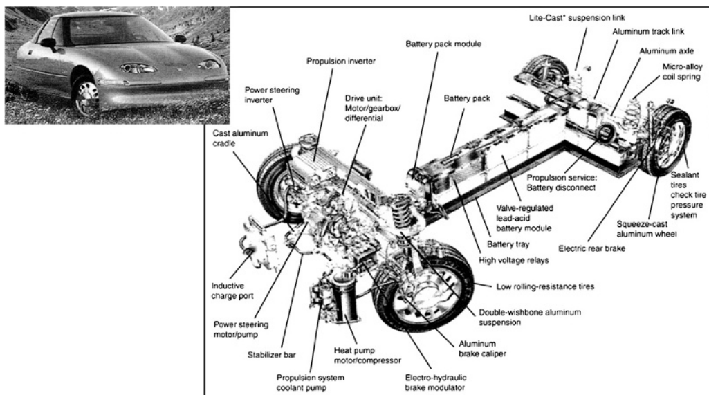
Fig. 6.1-15 GM EVI and Impact prototype, inset.
