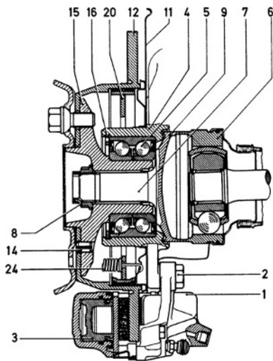
Fig. 8.1-44 Rear axle wheel hub carrier with wheel and brake. The drive shaft 7 is butt-welded to the CV slip joint 6. The drive shaft transmits the driving torque to the wheel hub 15 via a serrated profile. Part 15 is carried by the maintenance-free, two-row angular (contact) ball bearing 5. The one-part outer ring is held in the hub carrier 4 by the snap ring 16. The seal rings on both sides sit in the permanently lubricated bearing unit. The covering panel 11 (that surrounds the brake disc 12) acts as additional dirt-protection outside, as does collar 9 of the CV joint on the inside. This grips into a cut-out in the wheel hub carrier 4 and creates a cavity. The centrifugal effect of the bell-shaped joint housing prevents ingress of dirt and water. The brake disc 12 is pulled from outside against the flange 15 and fixed by dowel 14 until the wheel is mounted. The jaws 20 of the drum brake acting as a handbrake act on the inside of part 12. At the lower end, the illustration shows the fixed calliper 1 of the disc brake. Two hexagonal bolts (item 2) fix it to the wheel hub carrier 4. Piston 3 and the outer brake pad are shown cut away (illustration: Mercedes-Benz).
