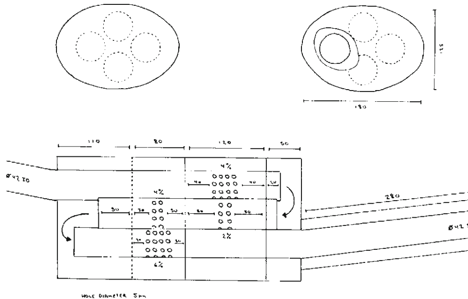
Fig. 22.1-42 The internals of a compact exhaust silencer element showing many distinct chambers and a flow path that is longer than the physical length of the element. Dimensions are in millimetres.
