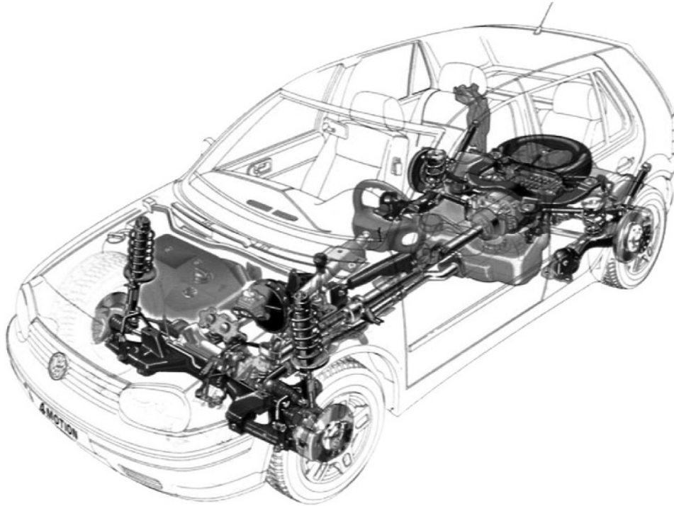
Fig. 8.1-72 Four-wheel-drive Golf 4motion (1998). In the four-wheel-drive vehicle, Volkswagen uses a multi-link suspension consisting of one longitudinal and two transverse links mounted on a subframe. The driving torque is transmitted to the rear axle via a wet multi-disc clutch by the Swedish company Haldex which is flange-mounted on the rear axle drive and runs in oil. This electronically controlled clutch can build up a coupling torque of up to 3200 N m even at small cardan-shaft rotation angles of 45° and can be combined to good effect with brake-power control systems. The drive train of the Audi TT Quattro (1998) built on the same platform is built to almost the same design.
