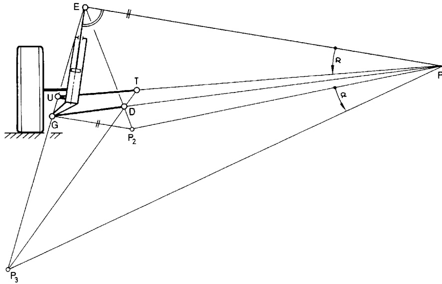
Fig. 9.1-47 On a McPherson strut with the joint G shifted to the wheel, the outer one, U of the tie rod, can lie in the plane of the steering axis (i.e. on the connecting line EG) when viewed from the rear. Extending the path UG is crucial for determining the virtual centre P_3 , whereas the direction of movement of the damper, i.e. a vertical on the piston rod in point E, must be the starting point for calculating P_1 .
