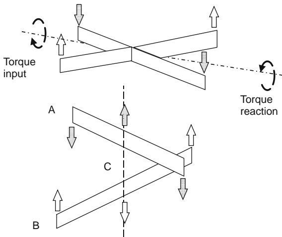
Fig. 16.1-11 Free body diagrams of cruciform brace members.
