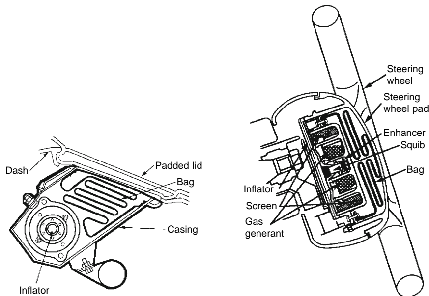
Fig. 17.1-11 Two Toyota gas bag installations: left , in the dash for the front seat passenger and right , in the steering wheel hub, for the driver. In both instances, an electrically fired squib generates the heat to fire the pellets which generate the gas. As the bags inflate, they push away the padded trim panels beneath which they are housed.
