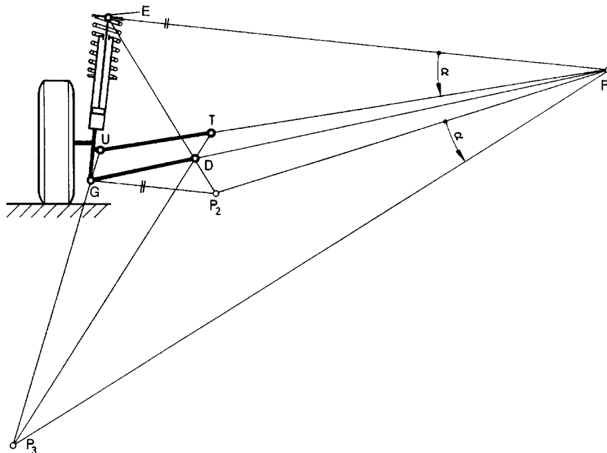
Fig. 9.1-46 On the McPherson strut or strut damper, the tie rod is above the lower control arm; the steering arms point inwards with the result that the outer joint U lies more to the vehicle centre.
