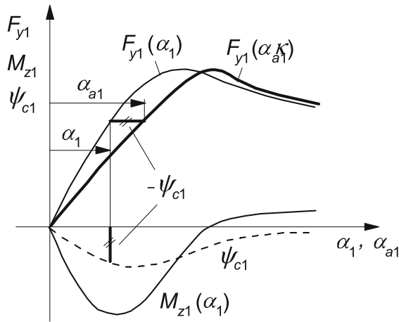
Fig. 11.1-6 Effective front axle characteristic F_{y1}(\alpha_{a1}) influenced by steering compliance.
