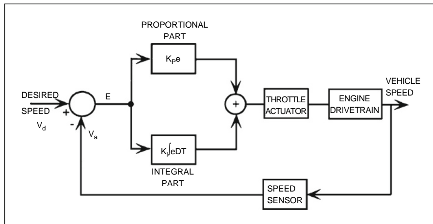
Fig. 13.1-2 Cruise control block diagram.
