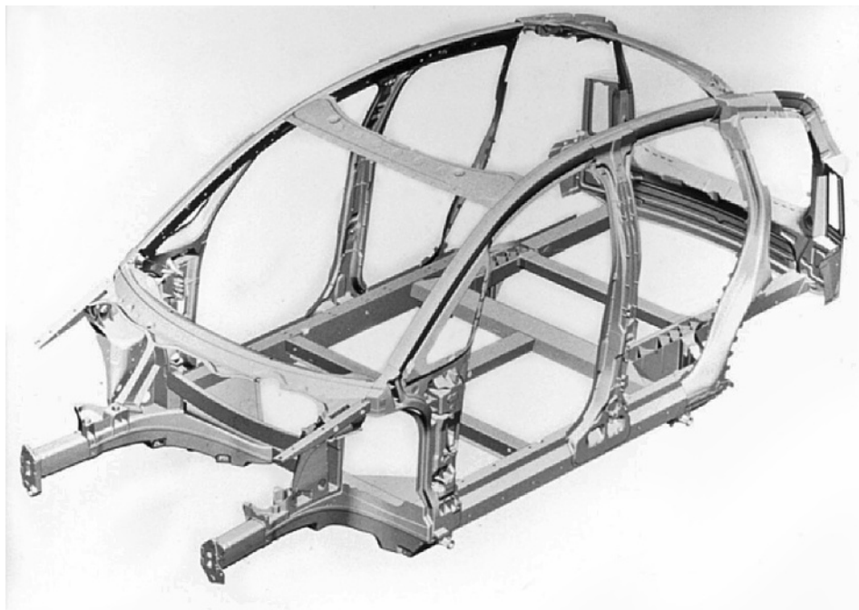
Fig. 16.1-20 Perimeter space frame (courtesy of Audi UK Ltd).
