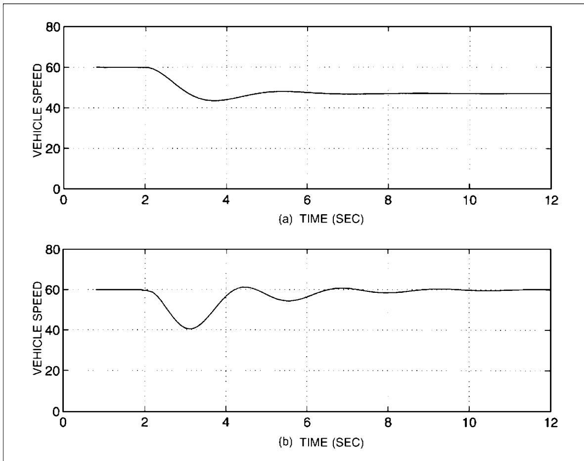
Fig. 13.1-3 Cruise control speed performance.
