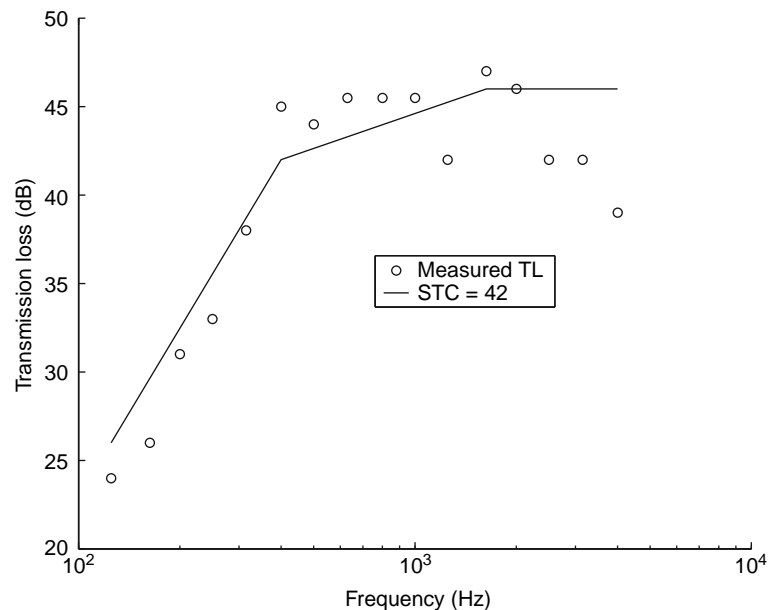
Fig. 21.1-17 STC curves: data after Kinsler et al. (1982).
