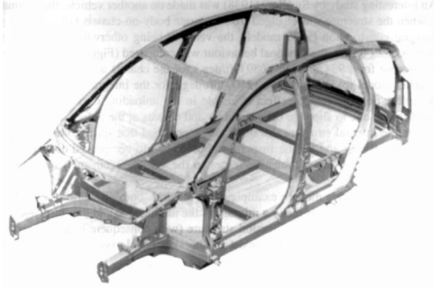
Fig. 18.1-29 Audi A2 body structure.
