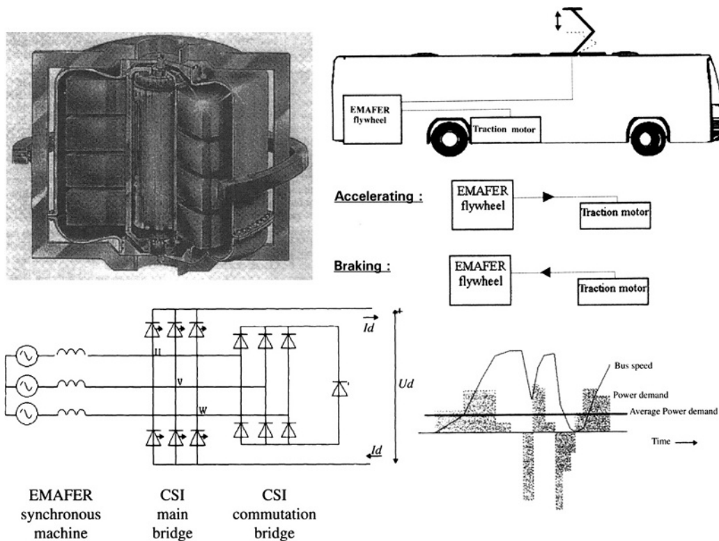
Fig. 7.1-12 Flywheel motor/generator: (a) Emafer flywheel/generator construction and electronic control; (b) power converter: shaded areas show power the Emafer has to supply/extract for accelerating or braking.
