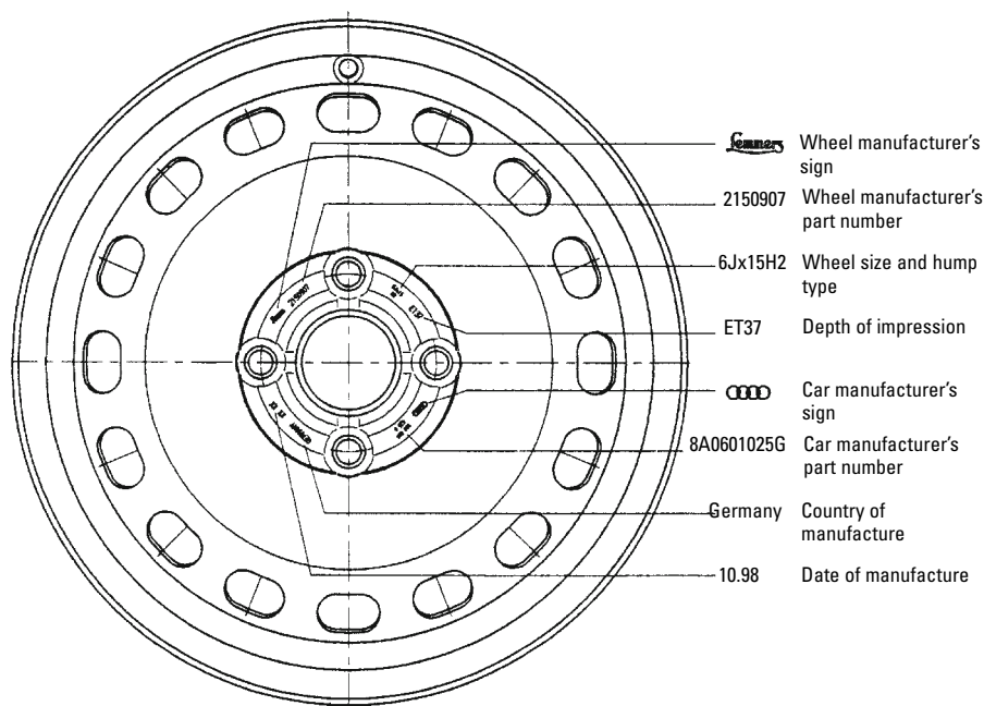
Fig. 10.1-25 Double-hump sheet metal disc-type wheel with openings for cooling the brakes. Also pictured is the stamp in accordance with the German standard DIN 7829, indicating manufacturer code, rim type and date of manufacture (week or month and year). Also specified is the wheel offset (ET37) and, in the case of special wheels with their own ABE (General operating approval), the allocation number of the KBA, the German Federal Vehicle Licensing Office. If there is not much space the stamp may be found on the inside of the dish. The date of manufacture also points to when the vehicle was manufactured (diagram: Hayes Lemmerz).
