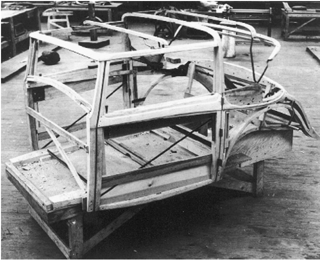
Fig. 16.1-5 Car body manufacture in the 1920s (courtesy of Vauxhall Archive Centre).
