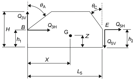
Fig. 16.2-15 Components of forces Q_3 and Q_5 .
