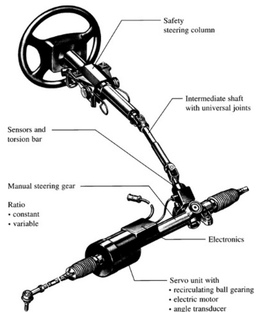
Fig. 9.1-22 Electrical power steering system by ZF. The servo unit acts on the gear rack itself. This system is suitable for high axle loads and steering forces. The maximum current strength is 105 A with a 12 V electric system; with a 42 V system, it is only 35 A.
