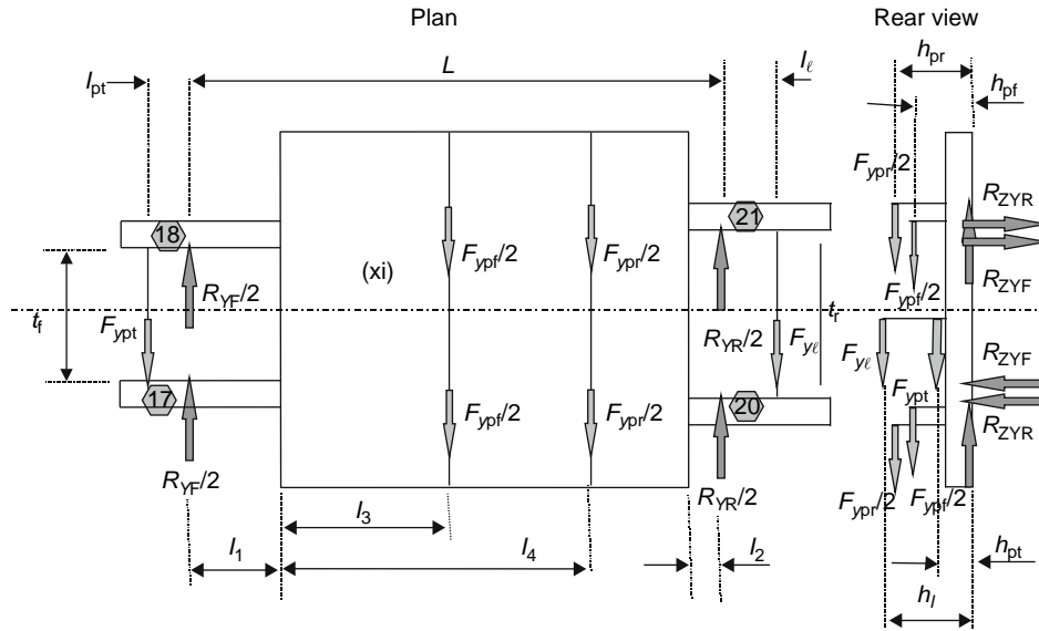
Fig. 16.2-24 Baseline model – lateral loading.
