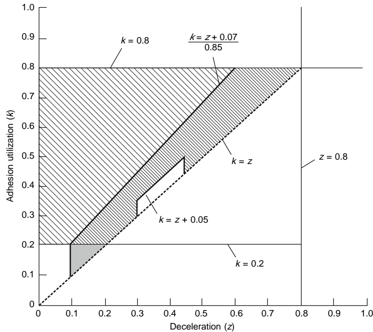
Figure 12.1-2 Adhesion utilization diagram for a category M_1 vehicle.
