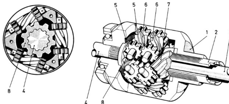
Fig. 8.1-71 Torsen central differential fitted in Quattro models (apart from the TT) by Audi. It consists of two worm gears, which are joined by spur gears and, depending on the traction requirement, can distribute the driving torque up to 75% to the front or rear axle. Under normal driving conditions 50% goes to each axle.
