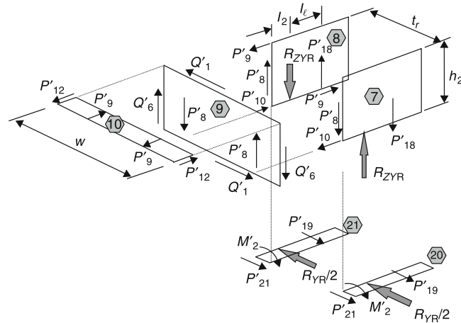
Fig. 16.2-27 Baseline model (rear structure) – lateral loading.
