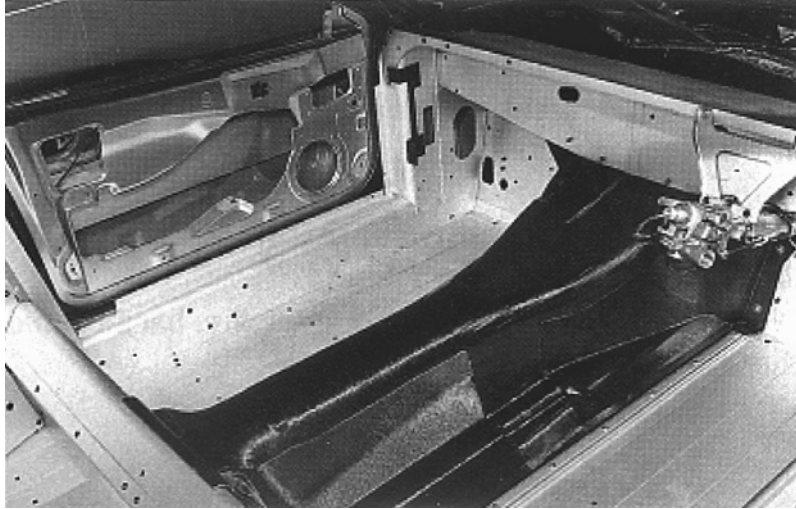
Fig. 18.1-32 Internal structure of Vanquish showing carbon fibre composite and extrusion construction.
