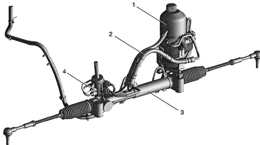
Fig. 9.1-18 Electro-hydraulic power steering system of the Opel Astra (1997). The individual components are: 1 electrically operated power-steering pump with integrated reserve tank ('power pack') 2 pump–steering valve hydraulic lines 3 rack and pinion steering gear with external drive, attached to auxiliary frame 4 steering valve.
