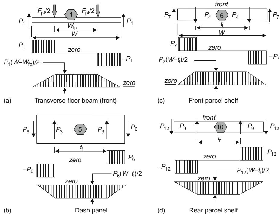
Fig. 16.2-5 Shear force and bending moment diagrams.
