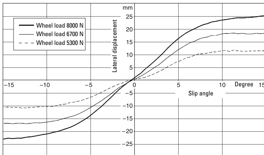
Fig. 10.1-51 Lateral displacement of normal (wheel load) point of application depending on slip angle and wheel load; measurements by Continental on a tyre of type 205/65 R 15 94 V ContiEcoContact CP.
