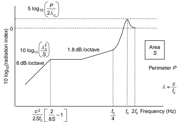
Fig. 21.1-5 Theoretical modal average radiation efficiency of a baffled rectangular panel: after Vér and Holmer (1971).
