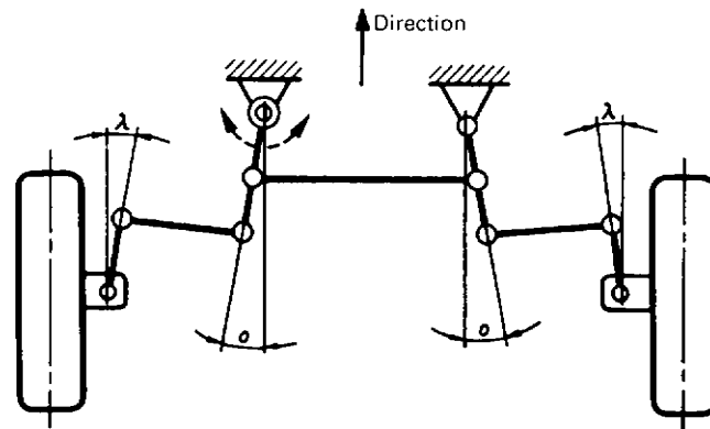
Fig. 9.1-37 'Opposed' 4-bar linkage located in front of the wheel centre. Steering arm and pitman arm rotate in opposite directions towards one another, similar to meshing gears. The tie rods are fixed directly to pitman and idler arms. For kinematic reasons, these can have the pre-angle \sigma (see also Fig. 8.1-7).
