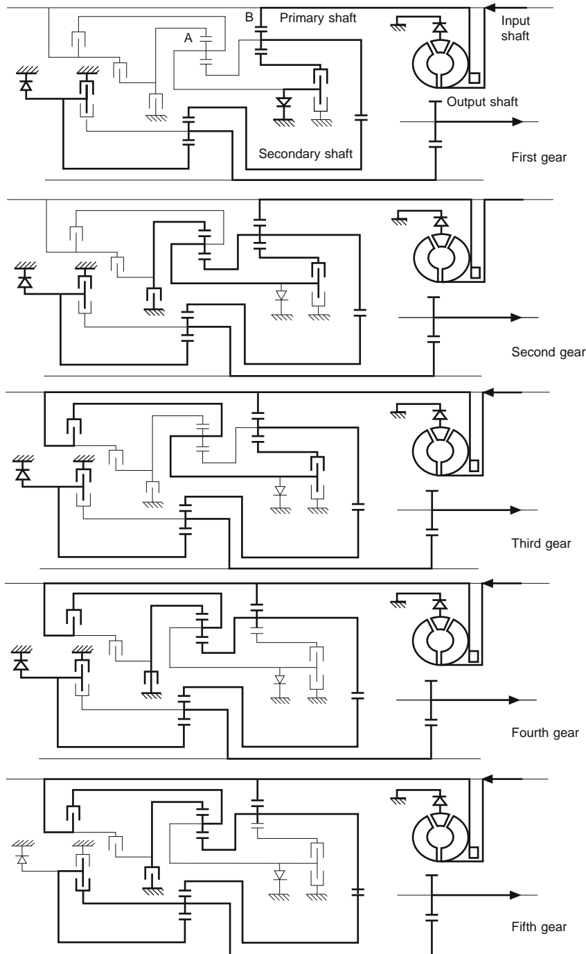
Fig. 5.1-22 Power flow paths for different gears in JF506E (courtesy of Jatco).
