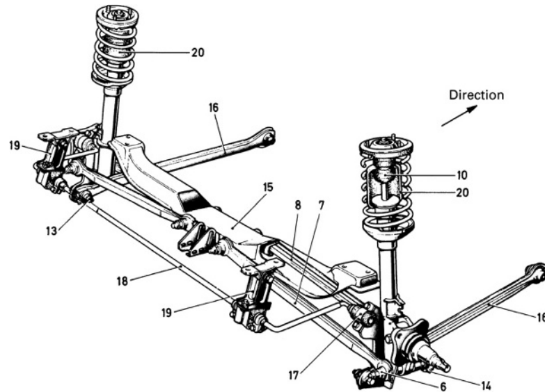
Fig. 8.1-12 The McPherson strut rear axle on the Lancia Delta with equal length transverse links of profiled steel trunnion-mounted close to the centre the cross-members 7 and 8. As large a distance as possible is needed between points 6 and 14 on the wheel hub carrier to ensure unimpaired straight running. The fixing points 13 of the longitudinal links 16 are behind the wheel centre, exactly like mounting points 17 of the anti-roll bar 18. The back of the anti-roll bar is flexibly joined to the body via tabs 19. The additional springs 10 attached to the top of the McPherson struts are covered by the dust tube 20. The cross-member 15 helps to fix the assembly to the body. An important criterion for dimensioning the control arm 16 is reverse drive against an obstruction.
