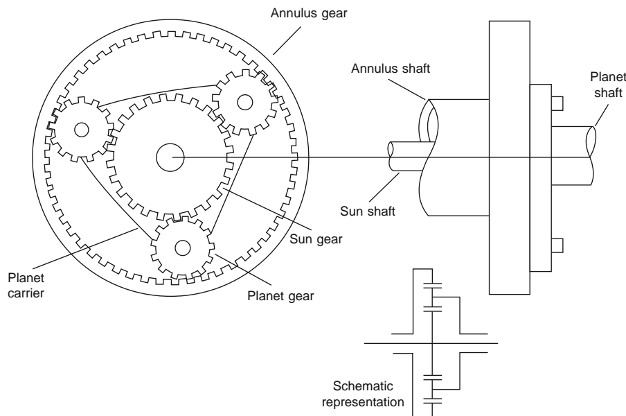
Fig. 5.1-20 An epicyclic gear and stick equivalent.
