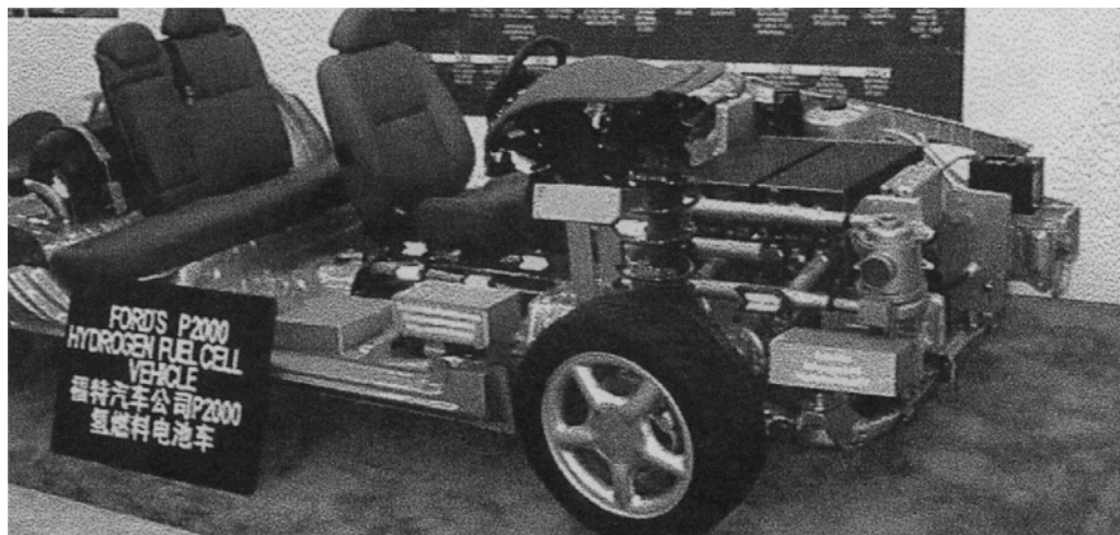
Fig. 6.1-24 Ford P2000 fuel cell platform with two 35 kW Ballard stacks.
