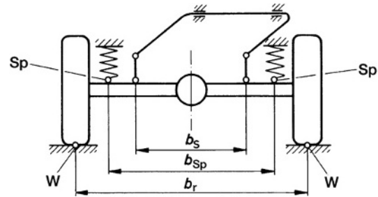
Fig. 8.1-23 When considering the roll pitch of the body with the rigid axle the distances b_{Sp} (of the springs F ) and b_S (of the anti-roll bar linkage points) are included in the calculation of the transfer with mutually opposed springing. i_\phi is squared to give the rate c_\phi :
