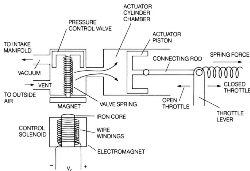
Fig. 13.1-7 Vacuum-operated throttle actuator.
