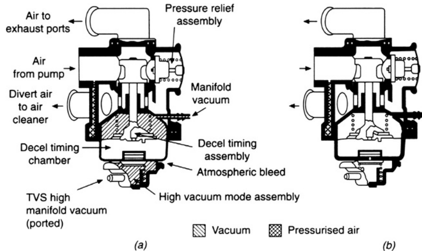
Fig. 3.1-13 This is what Rochester term their high vacuum air-control valve: (a) in the high vacuum mode; (b) in the low vacuum mode. On sudden closure of the throttle valve with the engine cold it operated in the same way as the standardised diverter valve in Fig. 3.1-8.
