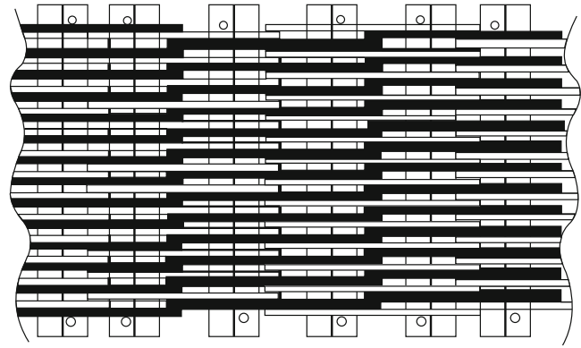
Fig. 5.1-29 The LuK-PIV chain construction.
