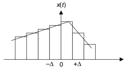
Fig. B21.1-3 x(t) represented as a continuum of impulses: after (Sinha, 1991).
