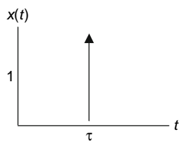
Fig. B21.1-2 The unit impulse at time t = \tau .
