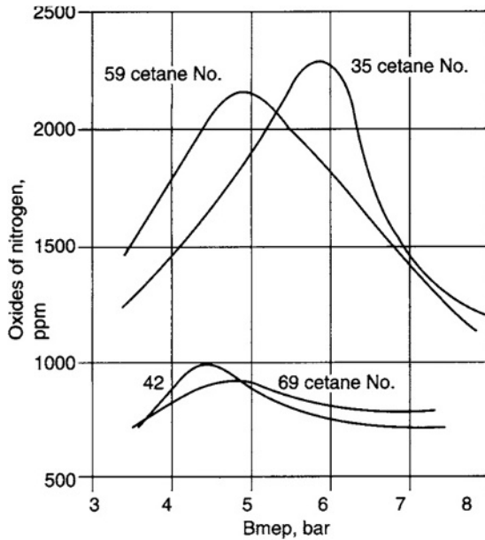
Fig. 3.1-22 \text{NO}_x emissions with direct and indirect injection.
