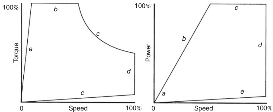
Fig. 2.1-15 Performance curve shapes of an eddy-current dynamometer.
