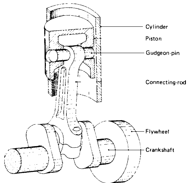
Fig. 1.1-1 Pictorial view of the basic engine.
