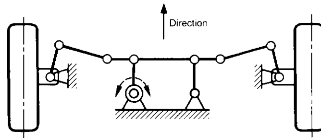
Fig. 9.1-36 'Synchronous' 4-bar linkage with steering arms pointing forwards. The inner joints are fixed to the sides of the intermediate rod.
