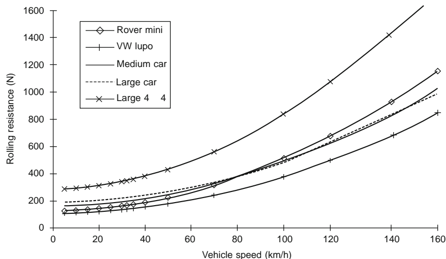
Fig. 5.1-2 Plot of total rolling resistance vs road speed (level road) – data shown for various vehicles.
