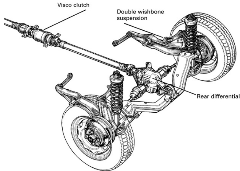
Fig. 8.1-77 Double wishbone rear axle of the Honda Civic Shuttle 4 WD. The visco clutch sits (held by two shaft bearings) in the centre of the divided propshaft. The rear axle differential has been moved forwards and is mounted to the rear on the body via a cross-member. Apart from the different type of wheel bearings and the lower transverse control arm positioned somewhat further back (to make it possible to bring the drive shafts through in front of the spring dampers), the axle corresponds to Fig. 8.1-62 and resembles the suspension shown in Fig. 8.1-1.
