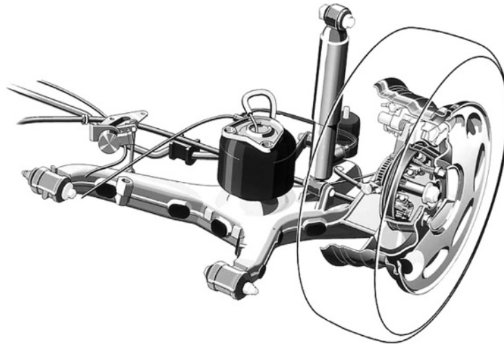
Fig. 8.1-16 Flat, non-driven air-suspended semi-trailing-arm rear axle of the Mercedes-Benz V class, whose driven front axle with spring-and-shock absorber strut has conventional coil springs. The air-spring bellows are supplied by an electrically powered compressor. The individual wheel adjustment permits the lowering or lifting of the vehicle as well as a constant vehicle height, regardless of – even onesided – loading. It is also possible to counteract body tilt during cornering. The damping properties of the shock absorbers are affected by spring bellow pressure depending on the load. The short rolling lobe air-spring elements make a low load floor possible; its rolling movement during compression and rebound results in self-cleaning. In the case of semi-trailing arm axles, roll understeer of the rear axle can be achieved by means of a negative vertical angle of pivot-axis inclination the kinematic toe-in alteration is also reduced.
