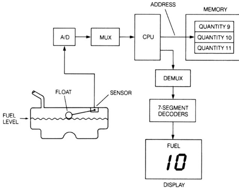
Fig. 23.1-9 Fuel quantity measurement.
