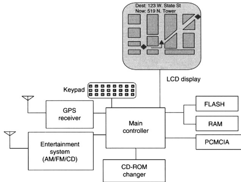
Fig. 14.1-10 Block diagram of basic GPS-enabled navigation system.
