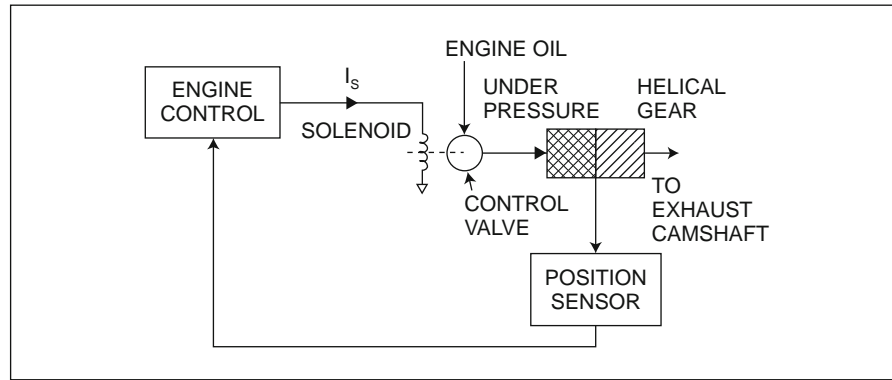
Fig. 4.1-8b Closed-loop control system.
