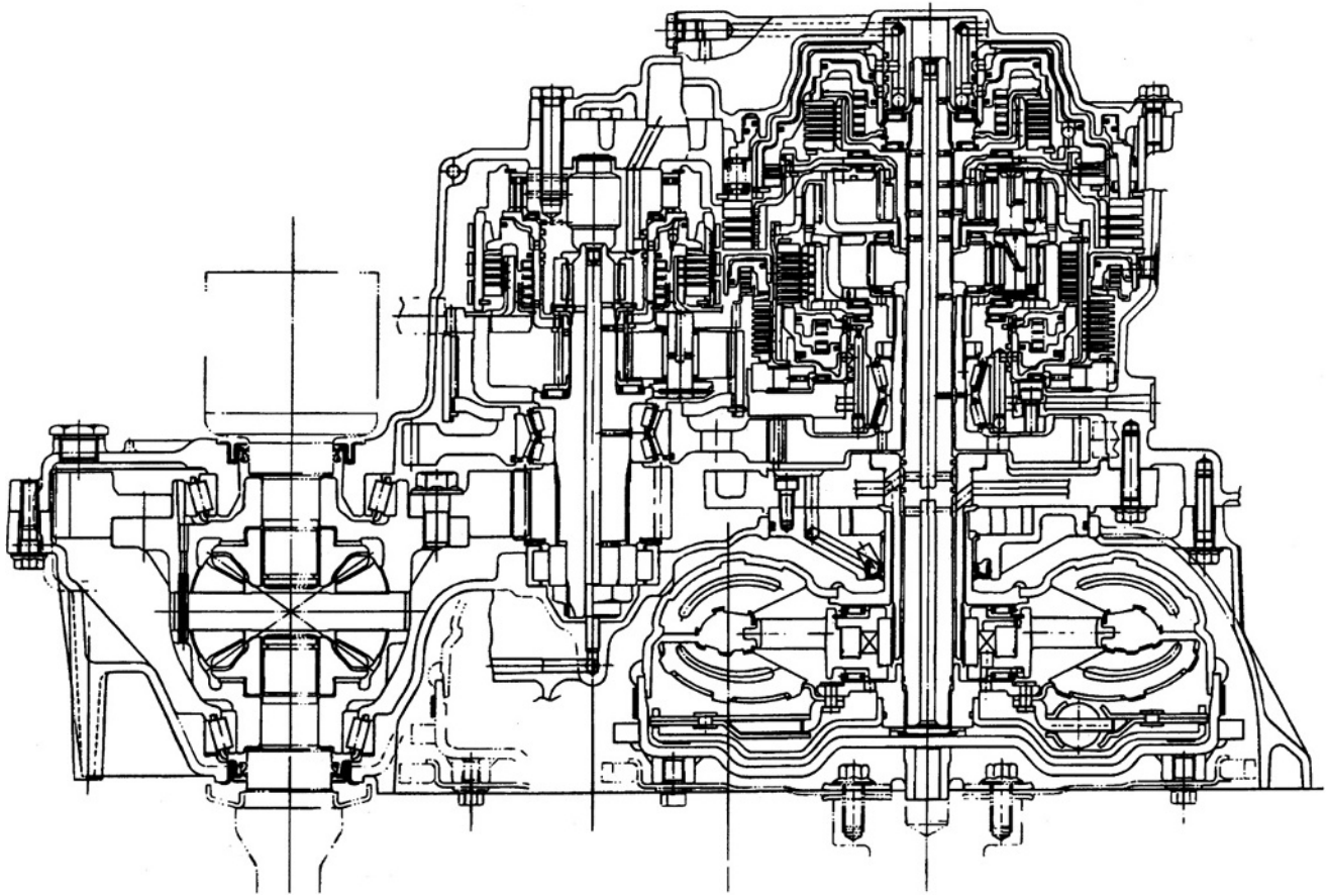
Fig. 5.1-16 Sectioned view of Jatco JF506E (courtesy of Jatco).
