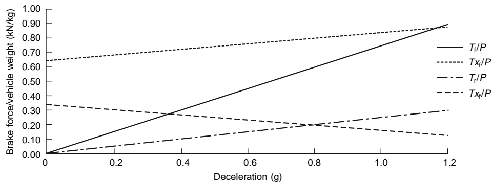
Figure 12.1-10 Normalized brake force against deceleration.
