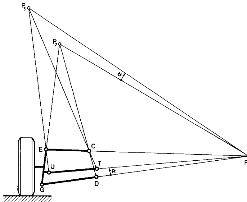
Fig. 9.1-42 Double wishbone suspension with steering arm pointing inwards. The tie rod is above the lower control arm.
