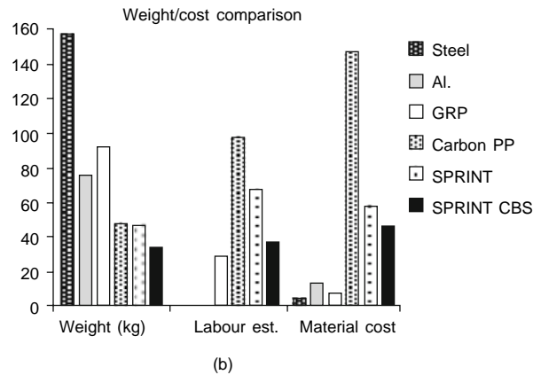
Fig. 18.2-17 (a) and (b) Nature of SPRINT material and comparative costs. (Courtesy of SP Systems.)
