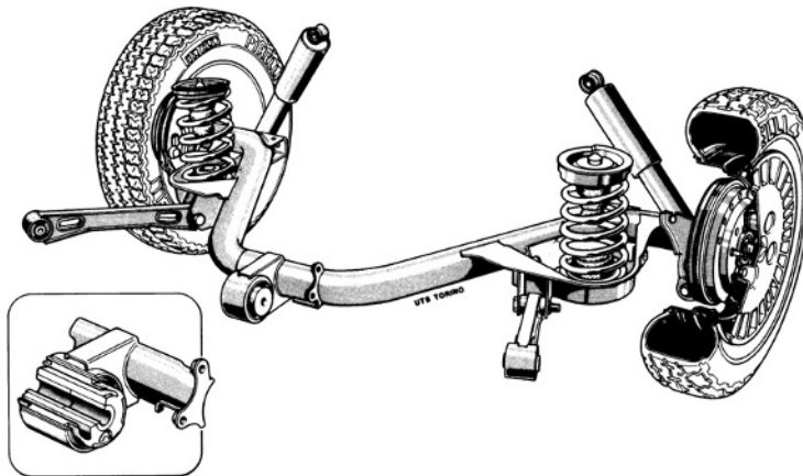
Fig. 8.1-60 'Omega' rear wheel suspension on the Lancia Y 10 and Fiat Panda, a trailing axle with a U-shaped tube, drum brakes, inclined shock absorbers and additional elastomer springs seated inside the low-positioned coil springs. The rubber element in the shaft axle bearing point, shown separately, has cut-outs to achieve the longitudinal elasticity necessary for comfort reasons; the same is true for the front bearings of the two longitudinal trailing links. The middle bearing point is also the body roll axis. The body roll centre is located in the centre of the axle but is determined by the level of the three mounting points on the body. The lateral forces are absorbed here. The angled position of the longitudinal trailing links is chosen to reduce the lateral force oversteering that would otherwise occur (shown in Fig 8.1-31). The coil springs are located in front of the axle centre and so have to be harder, with the advantage that the body is better supported on bends.
