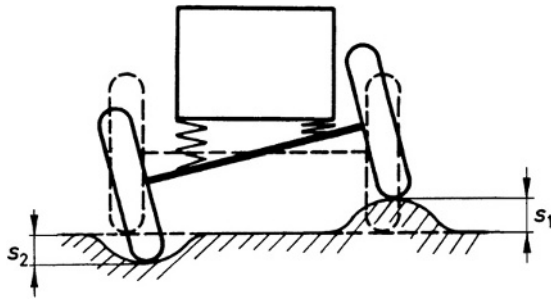
Fig. 8.1-21 Mutual influence of the two wheels of a rigid axle when travelling along a road with pot-holes, shown as 'mutually opposed springing'. One wheel extends along the path s_2 and the other compresses along the path s_1 .
