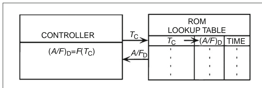
Fig. 4.1-3 Illustration of lookup table for desired air/fuel ratio.
