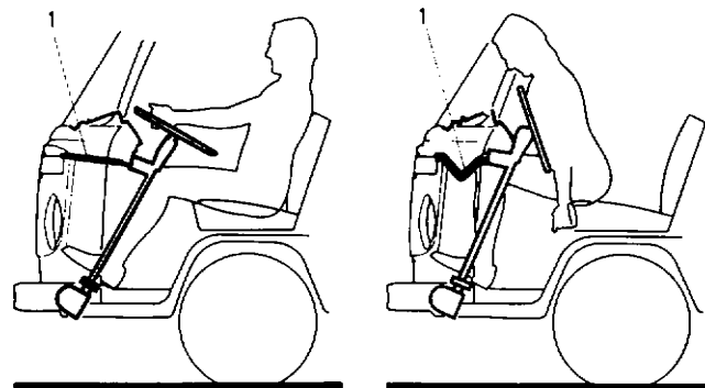
Fig. 9.1-31 The VW Bus Type II has an almost vertical steering column. In a head-on crash, first the steering wheel rim gives and then the retaining strut 1, which is designed so that a given force is needed to make it bend inwards.
