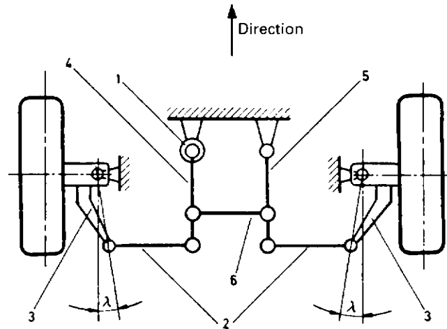
Fig. 9.1-3 Synchronous steering A-bar on the front suspension of a left-hand drive passenger car or light van; on the right-hand drive vehicle, the steering gear is on the other side. The steering arm (3) and the pitman arm (4) rotate in the same direction. The tie rods (2) are fixed to these arms.
