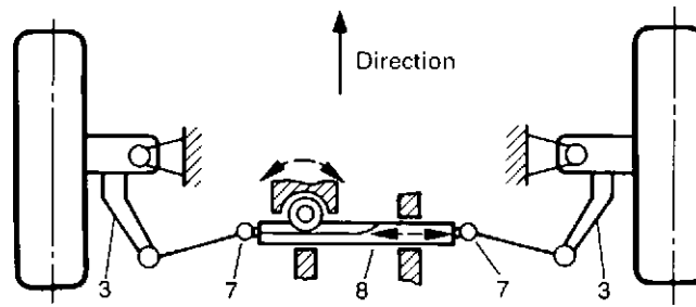
Fig. 9.1-4 Rack and pinion steering with the steering linkage 'triangle' behind the front axle. The spigots of the inner tie rod joints 7 are fixed to the ends of the steering rack 8 and the outside ones to the steering arms 3 (see also Figs. 8.1-40 and 8.1-54).
