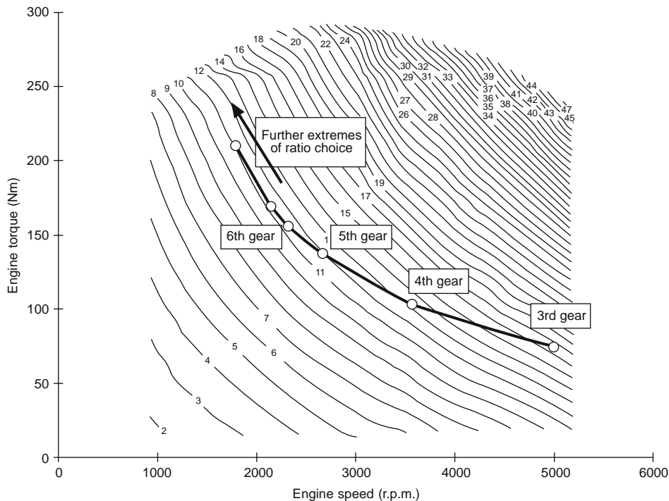
Fig. 5.1-4 Chart of fuel (mass) flow for a large petrol engine – also shows engine conditions for a range of gear ratios.
