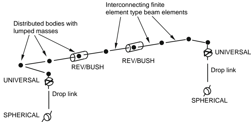
Fig. 15.1-18 Modelling the anti-roll bars using interconnected finite element beams.
