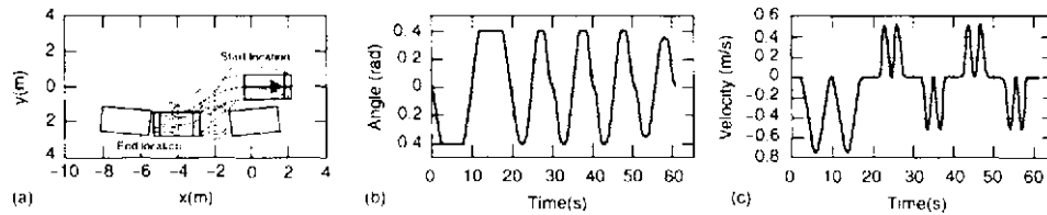
Fig. 14.2-20 Motion and control commands in the parallel parking scenario: (a) motion, (b) steering angle and (c) velocity controls applied.
