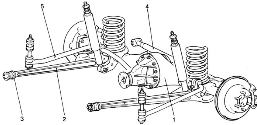
Fig. 8.1-43 The rear axle on the all-terrain, general-purpose passenger car, Mitsubishi Pajero. The rigid axle casing 1 is taken through the longitudinal control arms 2. These absorb the drive-off and braking forces (and the moments which arise) and transmit them to the frame. The rubber mountings 3 in the front fixing points 1, which also represent the vehicle pitch pole O_r , are designed to be longitudinally elastic to keep the road harshness due to the dynamic rolling hardness of the radial tyre away from the body. The Panhard rod 4 absorbs lateral forces. The anti-roll bar 5 is (advantageously) fastened a long way out on the frame (Fig. 8.1-23). The disc brakes, coil springs and almost vertical shock absorbers can be clearly seen.
