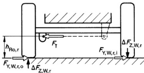
Fig. 8.1-25 On rigid axles the axle body absorbs the bending moments which arise as a result of lateral forces. Only the force F_T occurs between the suspension and the body, and its size corresponds to the lateral forces F_{Y,W,r,o} and F_{Y,W,r,i} . On a horizontal Panhard rod, the distance h_{Ro,r} is also the height of the body roll centre. The higher this is above ground, the greater the wheel force change \pm \Delta F_{Z,w,r} .
