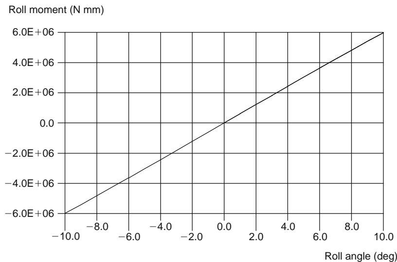
Fig. 15.1-22 Front end roll simulation.
