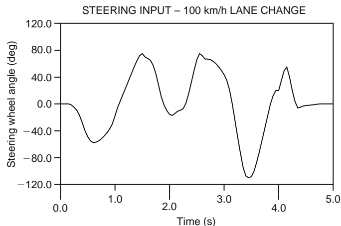
Fig. 15.1-50 Steering input for the lane change manoeuvre.
