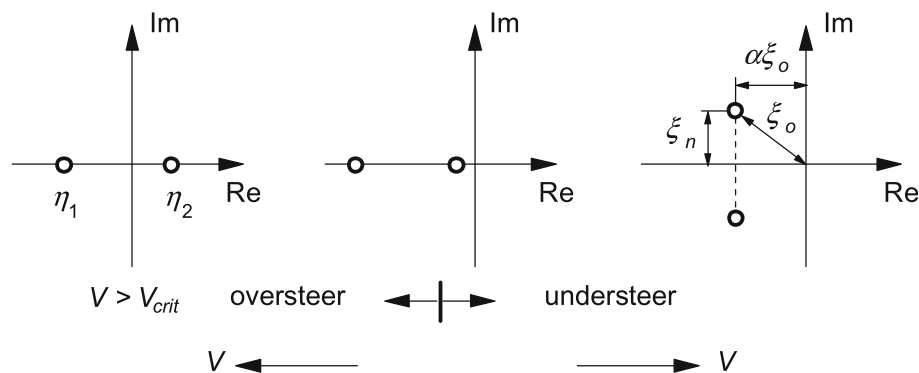
Fig. 11.1-12 Possible eigenvalues for the over and understeered car at lower and higher speeds.
