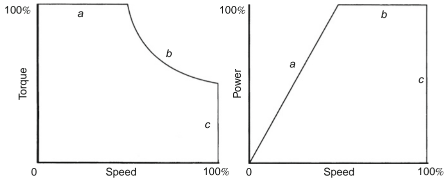
Fig. 2.1-14 Performance curve shapes of electrical motor-based dynamometers.
