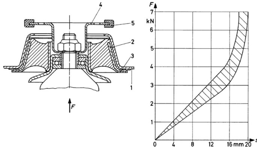
Fig. 8.1-9 McPherson strut mount on the VW Golf III with a thrust ball bearing, which permits the rotary movement of the McPherson strut whereas the rubber anchorage improves noise insulation. Initially, the deflection curve remains linear and then becomes highly progressive in the main work area, which is between 3 kN and 4 kN. The graph shows the scatter. Springing and damping forces are absorbed together so the support bearing is not decoupled (as in Fig. 8.1-10). In the car final assembly line the complete strut mount is pressed into a conical sheet metal insert on the wheel house inside panel 1. The rubber layer 2 on the outside of the bearing ensures a firm seat and the edge 3 gives the necessary hold in the vertical direction. The rubber ring 5 clamped on plate 4 operates when the wheel rebounds fully and so provides the necessary security (figure: Lemförder Fahrwerktechnik AG).
