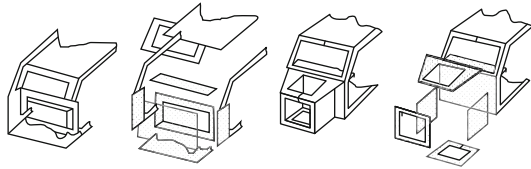
Fig. 16.2-20 Torsion stiffening by ‘boxing in’ localized regions of body.
