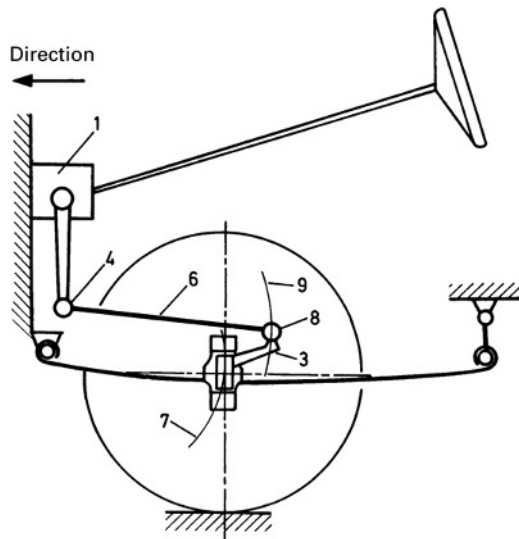
Fig. 9.1-6 Side view of a rigid front axle showing the movement directions 9 and 7 of the drag link and axle housing during bump and rebound-travel. The path of point 7 is determined by the front half of the leaf spring and can be calculated on a spring-balance by measuring the change in length when a load is added to and removed from the spring.
