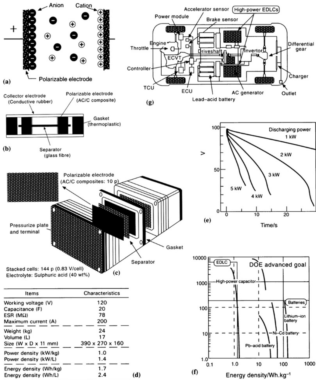
Fig. 6.1-7 Supercapacitors: (a) EDLC model; (b) cell; (c) high-power EDLC schematic; (d) HP EDLC specification; (e) constant power discharge characteristics; (f) power density, y-axis in W/kg, vs energy density for high-power EDLC; (g) ELCAPA configuration.
