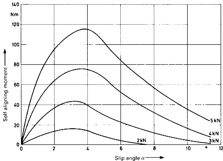
Fig. 10.1-49 Self-aligning torques of a 175/70 R 13 82 S steel radial tyre measured on a dry drum as a function of the slip angle at p_T = 2.0 bar. The vertical force F_{Z,W} in kilonewtons is used as a parameter. The torques increase sharply at low angles, reach a maximum at \alpha = 3\text{--}4^\circ and then reduce slowly. As the cornering speed increases, the tyre self-aligning torque decreases, while the kinematically determined torque increases.
