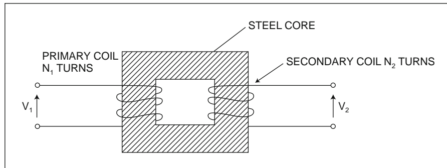
Fig. 4.1-22 Transformer structure and conversion of voltages.
