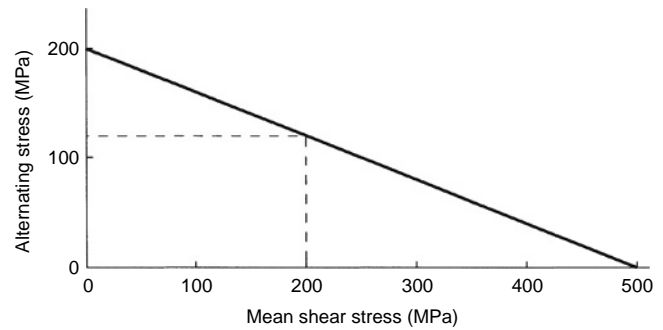
Fig. 2.1a-6 Goodman diagram, steel shaft in shear.
