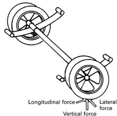
Fig. 8.1-26 Longitudinal leaf springs can absorb both forces in all directions and the drive-off, braking and lateral force moment.
