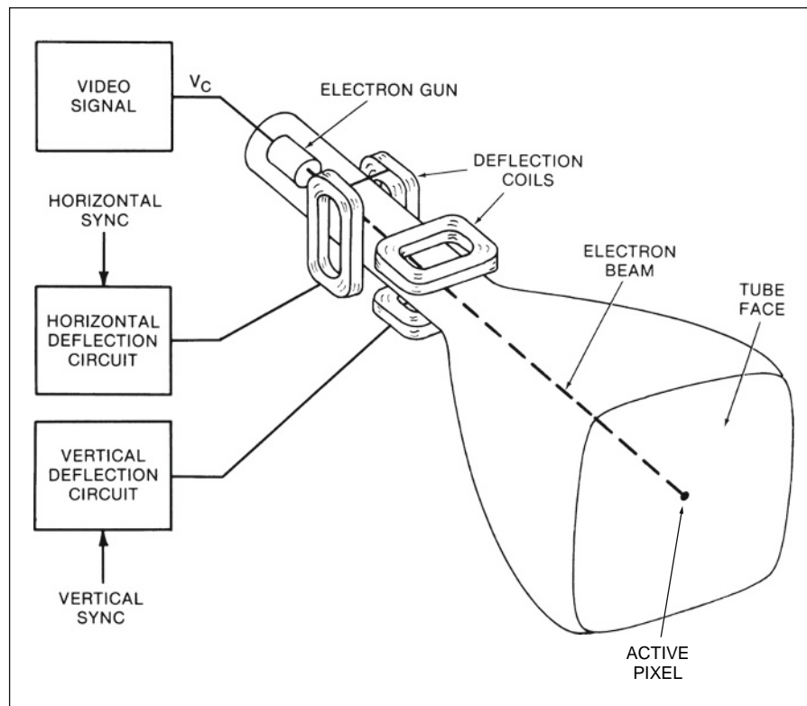
Fig. 23.1-20(a) CRT and associated circuitry.
