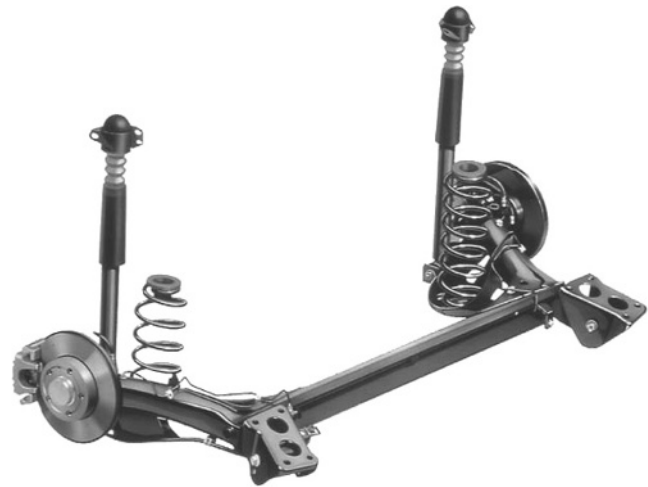
Fig. 8.1-30 Twist-beam suspension of the VW Golf IV (1997), VW Bora (1999) and Audi A3 (1996). The rubber-metal bearings of the axle body are set at 25^\circ to the transverse suspension of the vehicle in order to improve the self-steering properties of the suspension together with the rigidity of the bearings which varies in three directions in space. Compared with the previous model, it was possible to reduce unwanted lateral-force toe-out steer resulting from link deformation by 30% to approximately 1 mm per 500 N of lateral force. Fig. 8.1-72 shows the four-wheel-drive version of the VW Golf IV.
