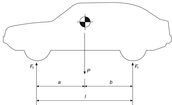
Figure 12.1-8 Static axle loads.
