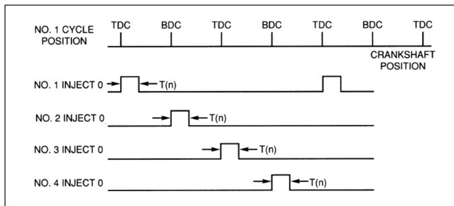
Fig. 4.1-19 Injector timing for 4-cylinder engine.
