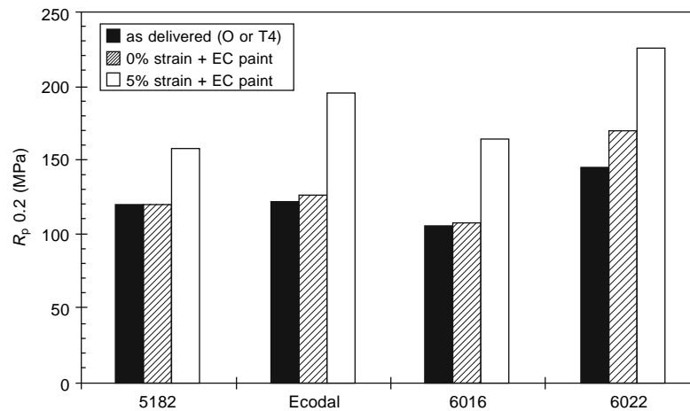
Fig. 18.2-15 Bake hardening response in 6000 series aluminium.
