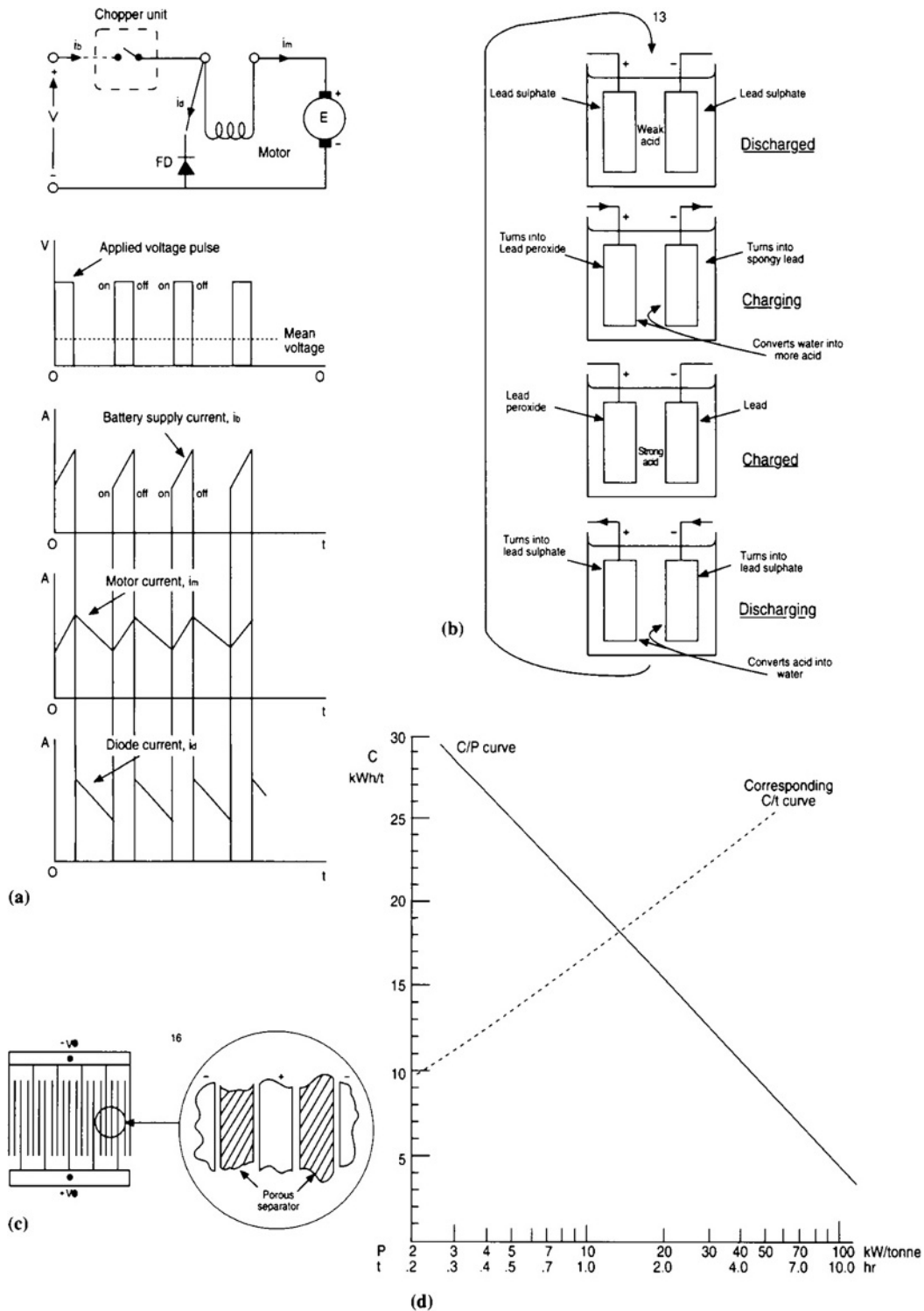
Fig. 6.1-10 Motor control and battery: (a) chopper circuit; (b) battery charge–discharge cycle; (c) cell arrangement; (d) battery time-of-discharge curves.
