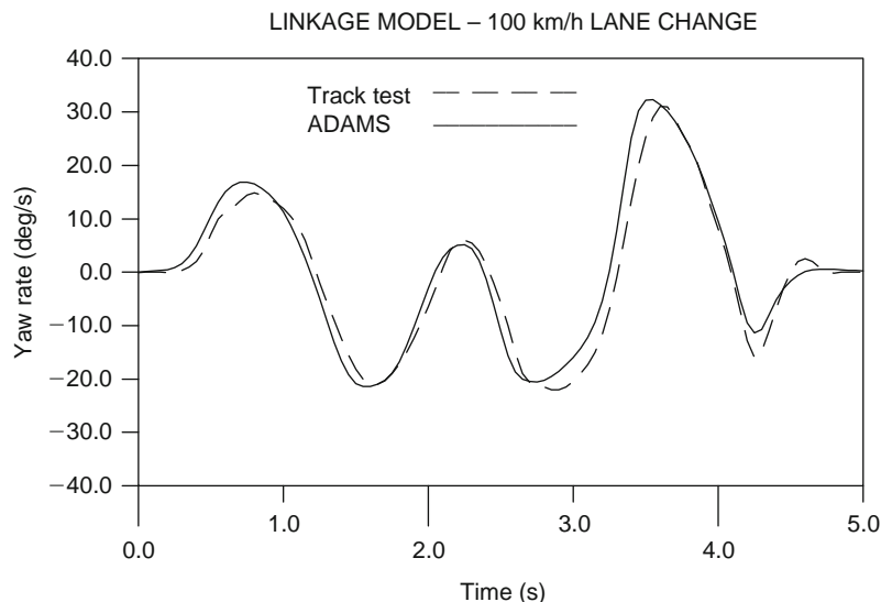
Fig. 15.1-56 Yaw rate comparison – linkage model and test. (This material has been reproduced from the Proceedings of the Institution of Mechanical Engineers, K2 Vol. 214 'The modelling and simulation of vehicle handling. Part 4: handling simulation', M.V. Blundell, page 81, by permission of the Council of the Institution of Mechanical Engineers.)
