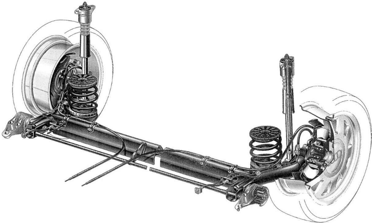
Fig. 8.1-58 Twist-beam suspension of the Audi A6 (1997). An advantageously large support width of the guide on the links – important for force application – was chosen because of the overhung arrangement. The flexurally resistant, but torsionally soft V section profile of the axle is in an upright position in order to ensure that the suspension has roll understeer properties through the high position of the centre of thrust of the profile. The instantaneous centre height is 3.7 mm and the toe-in alteration is 0.21 min/mm. Braking-torque compensation of 73% is reached. The stabilizer situated in front of the axis of rotation increases the lateral rigidity of the axle design, because it accepts tension forces upon the occurrence of lateral wheel forces. The linear coil springs mounted on noise-insulating moulded rubber elements on both sides are separated from the shock absorbers to allow the maximum loading width of the boot as a result of their location under the side rails. The gas-pressure shock absorbers support additional springs made of cellular polyurethane which act softly, through specific rigidity balancing, to avoid uncomfortable changes in stiffness when reaching the limits of spring travel. Owing to the rigid attachment of the shock absorbers to the bodywork, these also work at low amplitudes; so-called ‘parasitic’ springing resulting from the unwanted flexibility of wheel suspension or bodywork components is thereby reduced.
