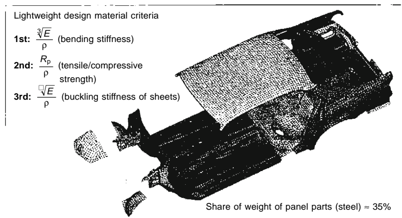
Fig. 18.1-18 Criteria used in the analysis of panel parts by BMW.
