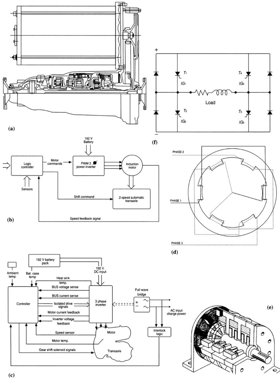
Fig. 6.1-16 AC drive systems: (a) transaxle motor; (b) controller arrangement; (c) controller drive system; (d) 3 phase induction motor stator; (e) air-gap type reluctance motor; (f) induction motor controller.
