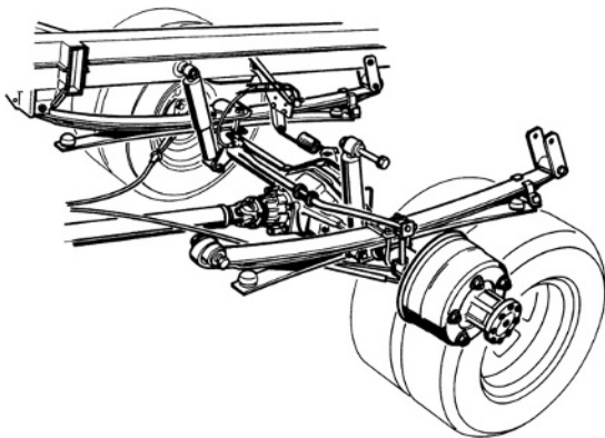
Fig. 8.1-20 Rear axle on the VW LT light commercial vehicle. The long, parabola-shaped rolled-out, dual leaf springs cushion the frame well and are progressive. The rubber buffers of the support springs come into play when the vehicle is laden. Spring travel is limited by the compression stops located over
