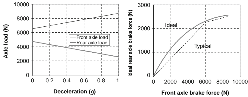
Fig. 15.1-30 Force distribution for ideal and typical braking events.
