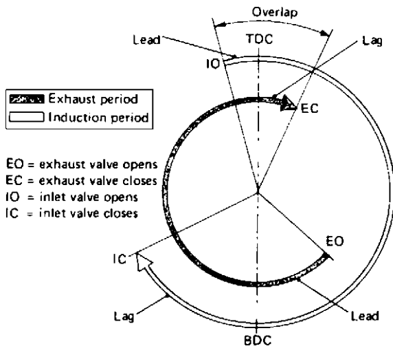
Fig. 1.1-4 Valve timing diagram.
