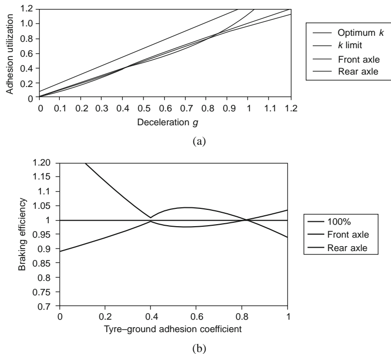
Figure 12.1-21 (a) Adhesion utilization, modified vehicle fitted with deceleration-sensitive pressure modulating valve, (b) brake system efficiency, modified vehicle fitted with deceleration sensitive.
