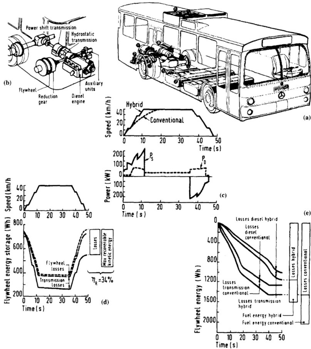
Fig. 7.1-19 Daimler-Benz OE 303 hybrid conversions: (a) diesel/electric hybrid package; (b) flywheel drive hybrid; (c) characteristics of flywheel hybrid; (d) flywheel losses; (e) diesel losses.
