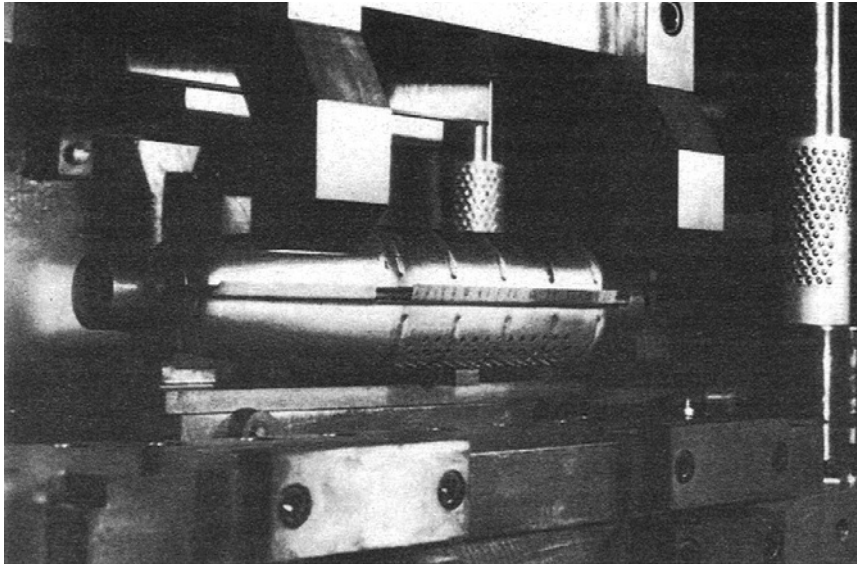
Fig. 3.1-3 The AC-Delco stainless steel housing for monolithic catalyst carriers is enclosed in an aluminised steel outer casing. Sandwiched between top halves of the outer and inner shells is heat insulation material. The perforations in the lower half of the outer shell, termed the grass shield, facilitate local cooling.
