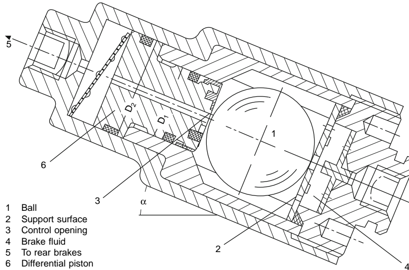
Figure 12.1-17 Deceleration-sensitive pressure limiting valve (Limpert, 1992).
