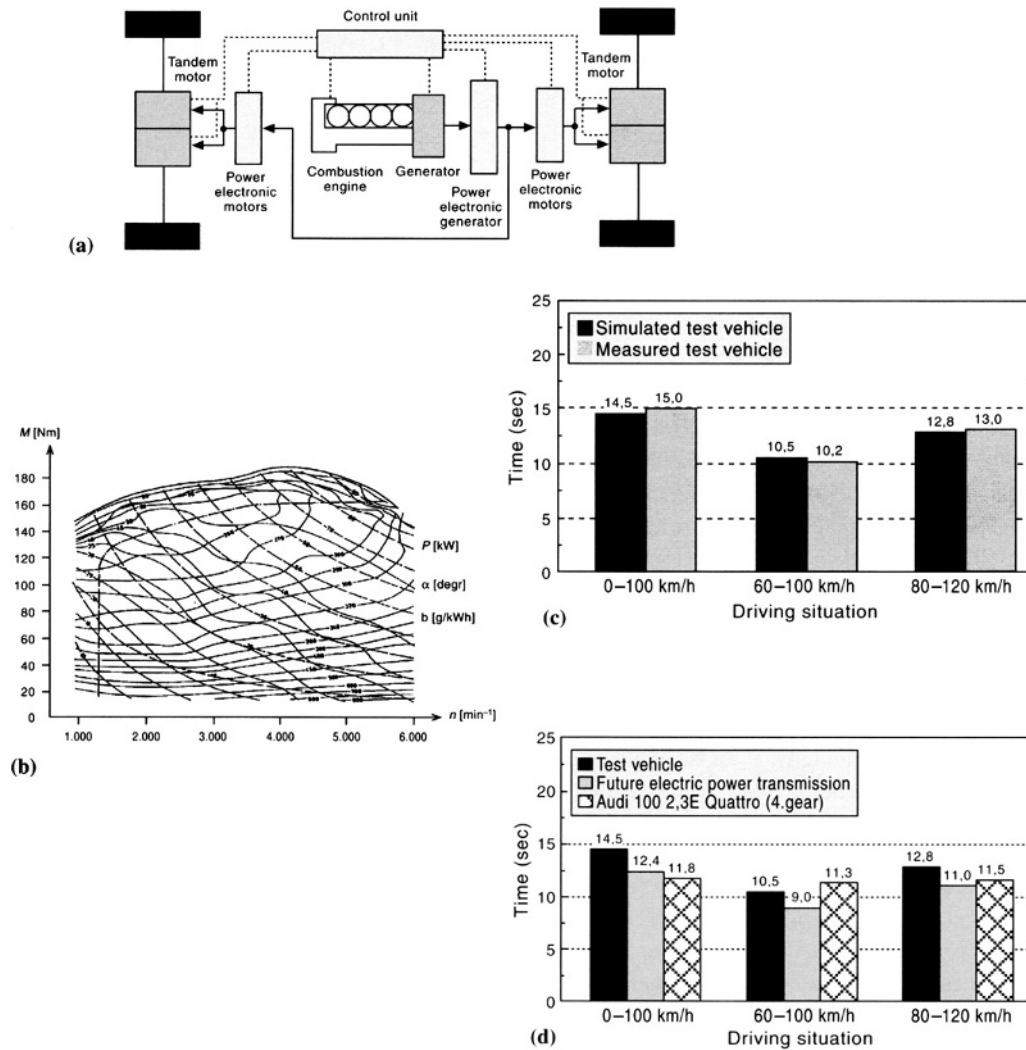
Fig. 7.1-9 Audi Quattro hybrid: (a) package; (b) speed/torque map; (c) simulated performance test; (d) estimated future performance.
