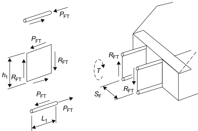
Fig. 16.2-9 Frontal structure.
