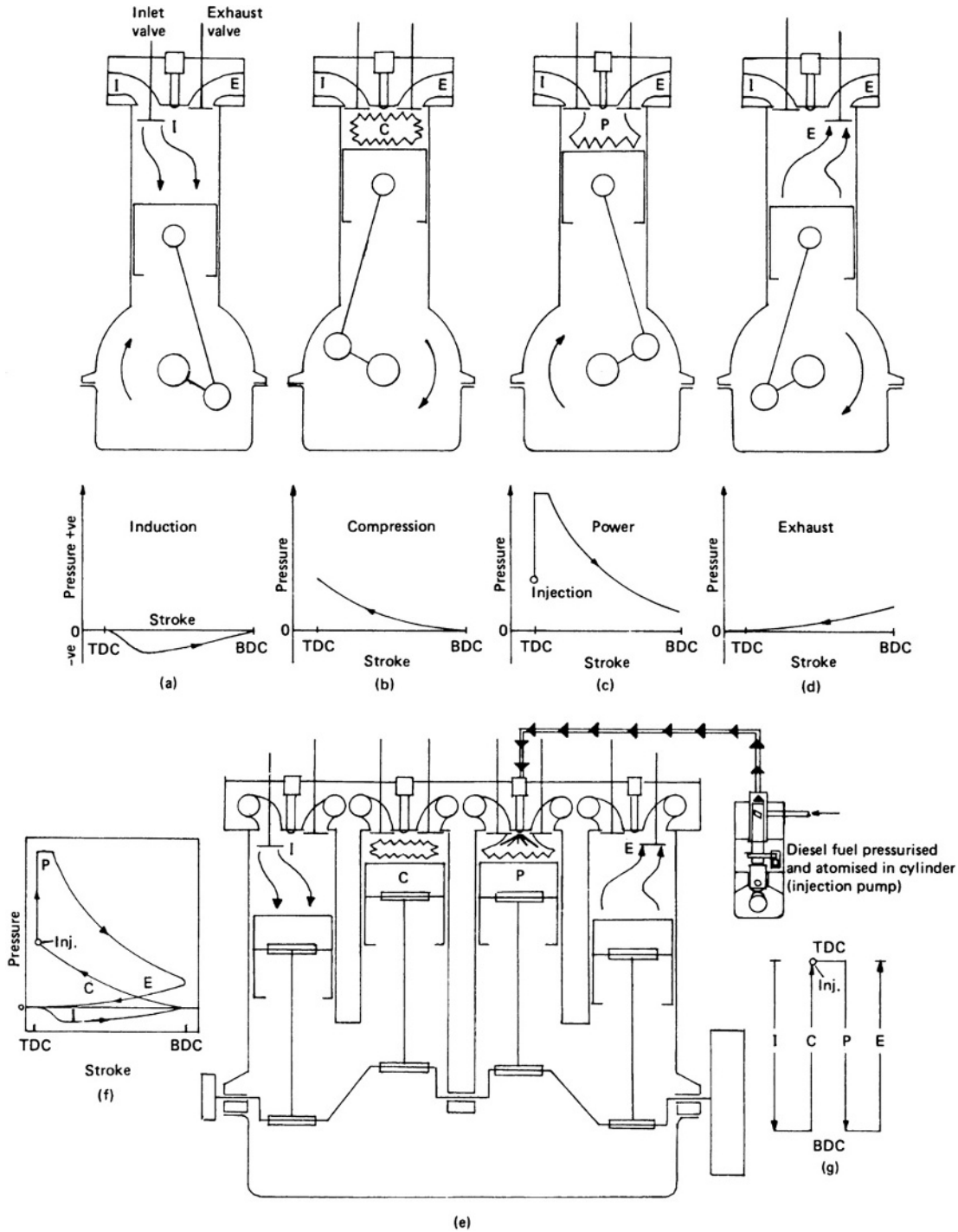
Fig. 1.1-8 Four-stroke-cycle diesel engine.
