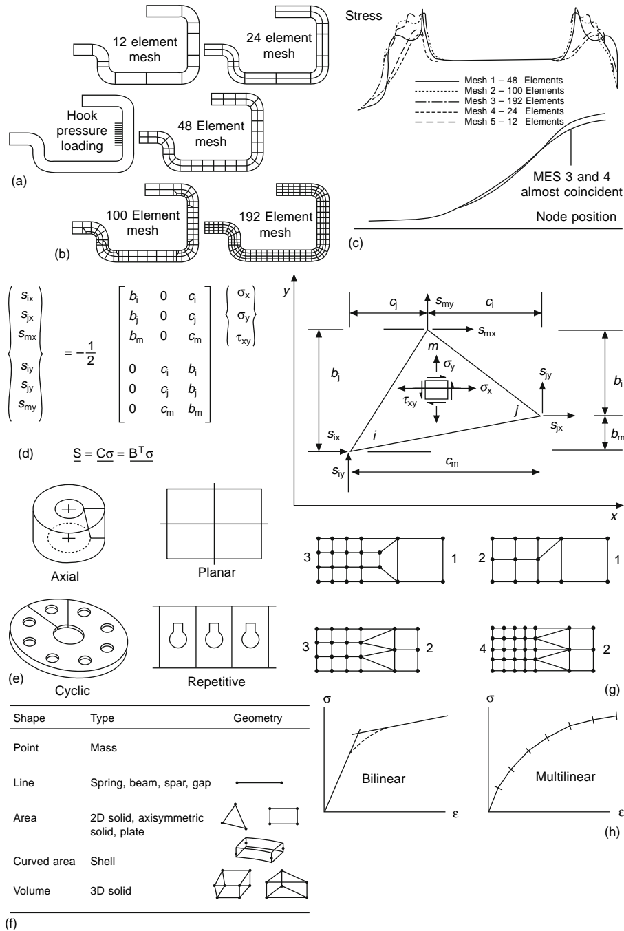
Fig. 18.1-6 Development of FEA: (a) towing hook as structural example; (b) various mesh densities; (c) FEA vs elasticity theory; (d) node equations in matrix form; (e) types of symmetry; (f) element shapes; (g) varying mesh densities; (h) stress–strain curve representation.
