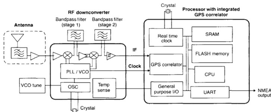
Fig. 14.1-7 Functional block diagram of GPS receiver.
