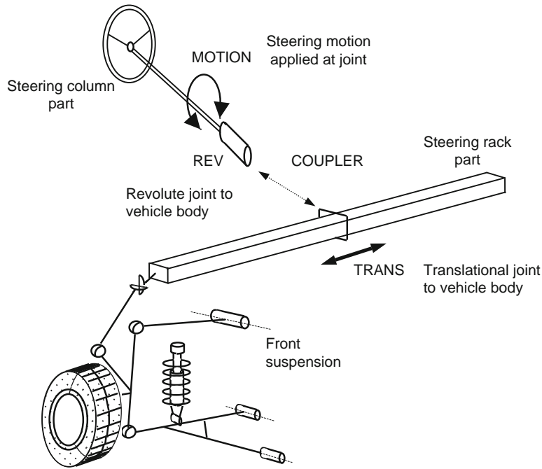
Fig. 15.1-36 Modelling the steering system. (This material has been reproduced from the Proceedings of the Institution of Mechanical Engineers, K2 Vol. 213 'The modelling and simulation of vehicle handling. Part 2: vehicle modelling', M.V. Blundell, page 129, by permission of the Council of the Institution of Mechanical Engineers.)
