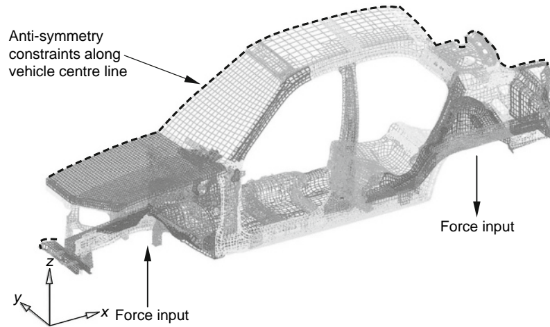
Fig. 15.1-4 Finite element model of body-in-white.
