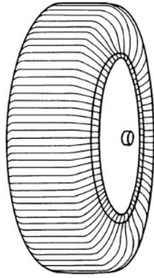
Fig. 10.1-3 Substructure of a radial tyre. The threads have a bias angle between 88^\circ and 90^\circ .
