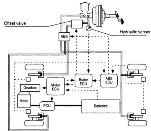
Fig. 6.1-14 Honda 'EV' electric car and Honda regenerative braking/coasting system.
