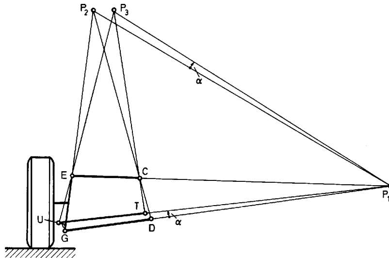
Fig. 9.1-43 In the case of a steering gear located in front of the wheel centre, the centre of the tie rod joint U lies outside the steering axis EG.
