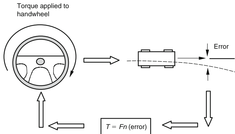
Fig. 15.1-43 Principle of a closed loop steering controller.
