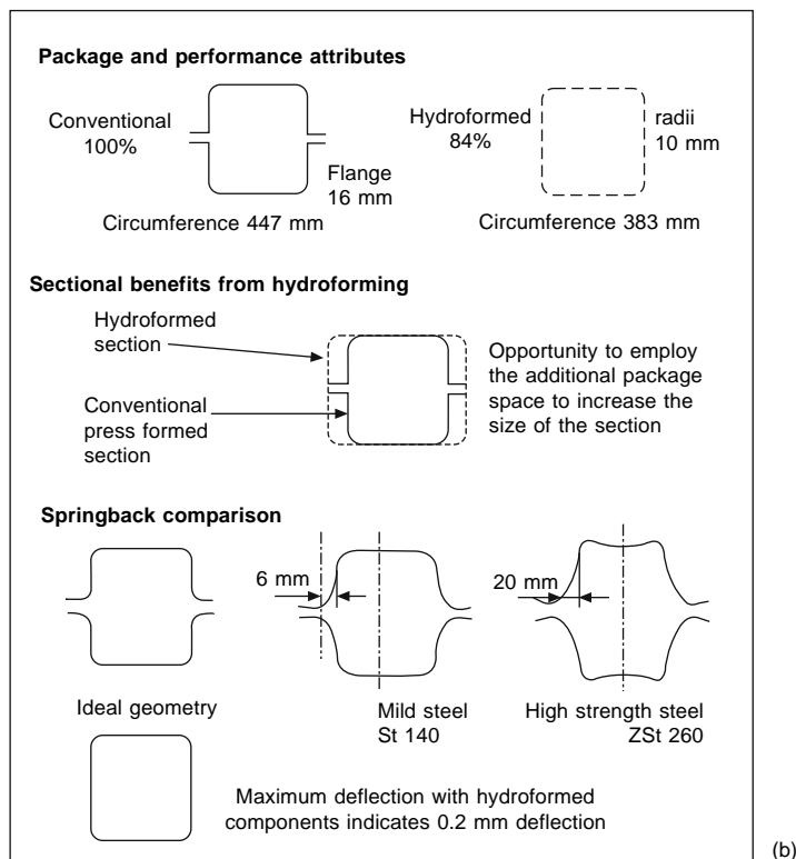
Fig. 18.1-35 Pre-development phases of ULSAB 40 and attributes of hydroformed sections. 16 (a) Pre-concept phases, (b) shape comparison with conventional sections. (Reprinted with permission from SAE paper 1999-01-3181 Copyright 1999 Society of Automotive Engineers Inc.)
