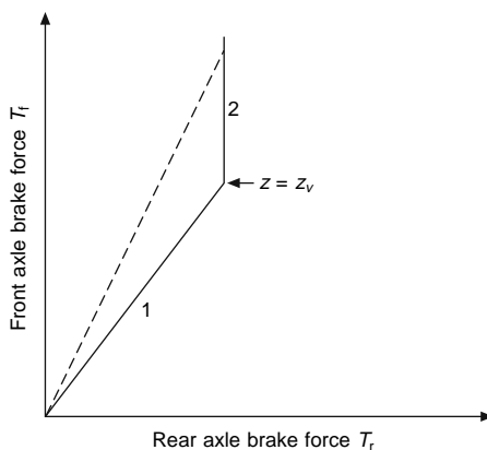
Figure 12.1-18 Typical limiting valve brake force distribution.
