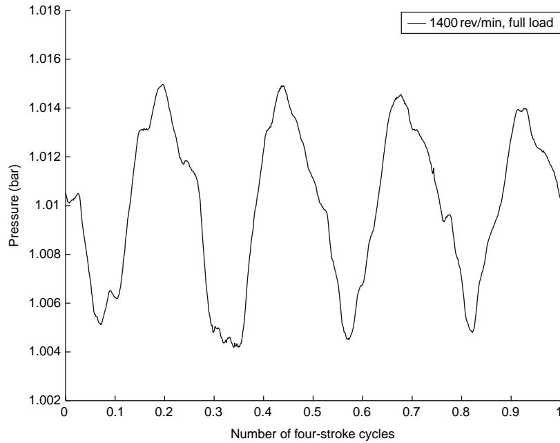
Fig. 22.1-14 Intake pressure trace for a four-cylinder engine.
