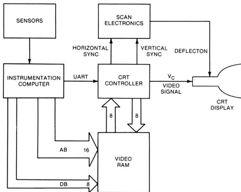
Fig. 23.1-22 Automotive CRT instrumentation system.
