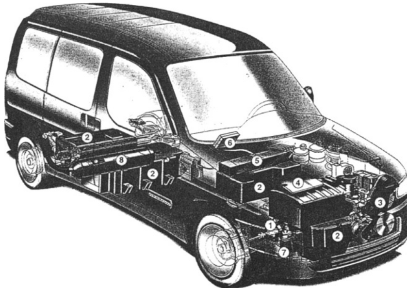
Fig. 6.1-18 Citroen Berlingo Dynavolt: 1. electric motor and drive; 2. traction battery pack; 3. generator set; 4. motor controller; 5. generator controller; 6. drive programme selector; 7. LPG regulator; 8. LPG storage tank.
