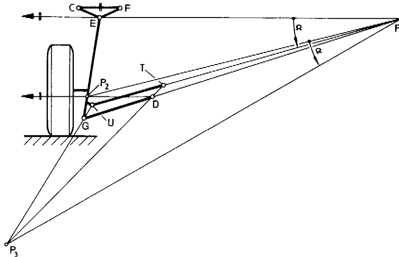
Fig. 9.1-49 Longitudinal transverse axle with the tie rod located above the lower control arm and the steering arm pointing inwards.
