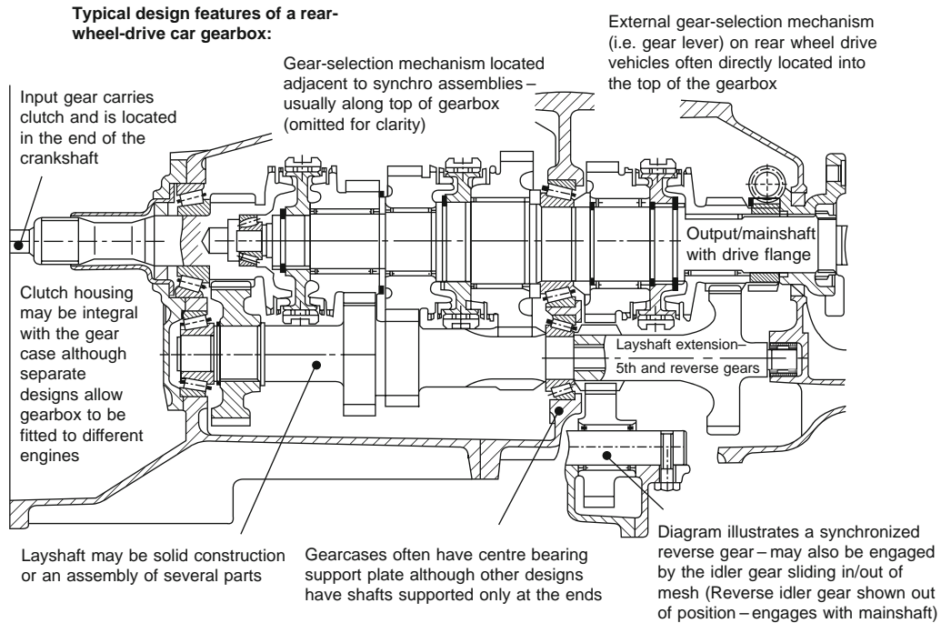
Fig. 5.1-8 Cross section of a rear-wheel-drive manual gearbox.
