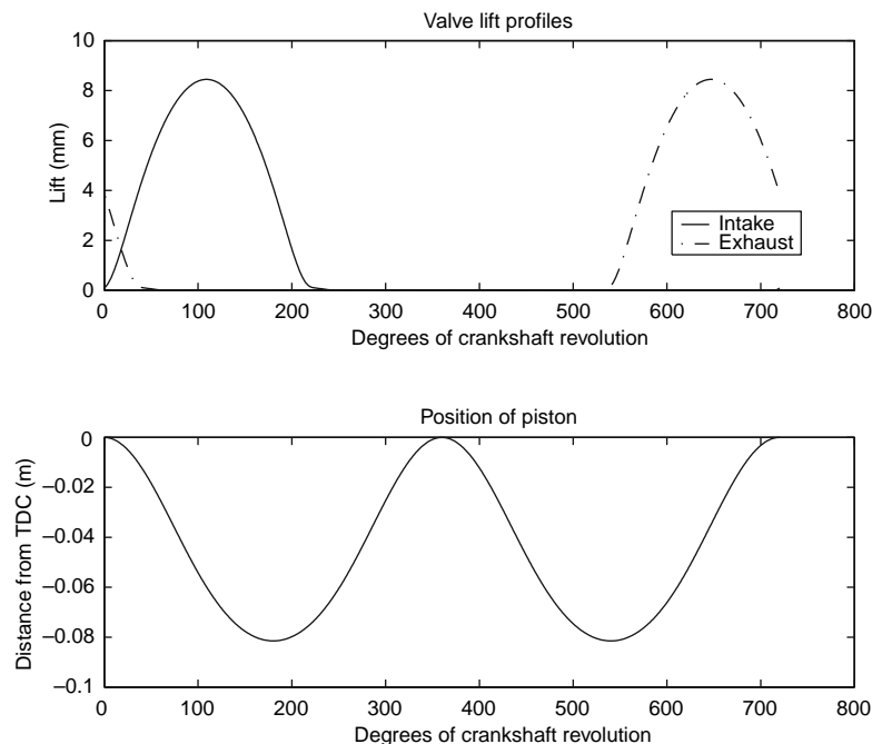
Fig. 22.1-6 Valve lift profiles and the instantaneous position of the piston.
