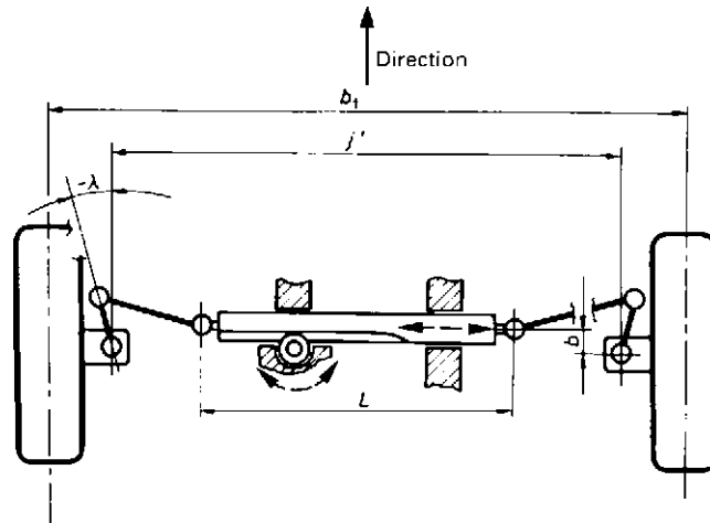
Fig. 9.1-41 Where rack and pinion steering and the steering triangle are shifted in front of the wheel centre, for kinematic reasons the steering arms must point outwards, making longer tie rods possible (see also Fig. 8.1-40).
