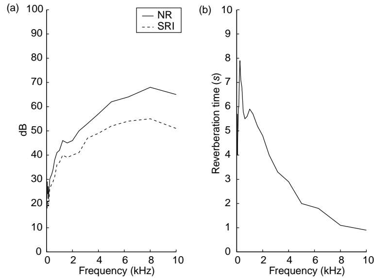
Fig. 21.1-16 Measured NR and SRI (TL) curves along with reverberation times.
