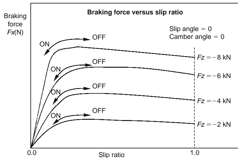
Fig. 15.1-31 Principle of a brake slip control model.
