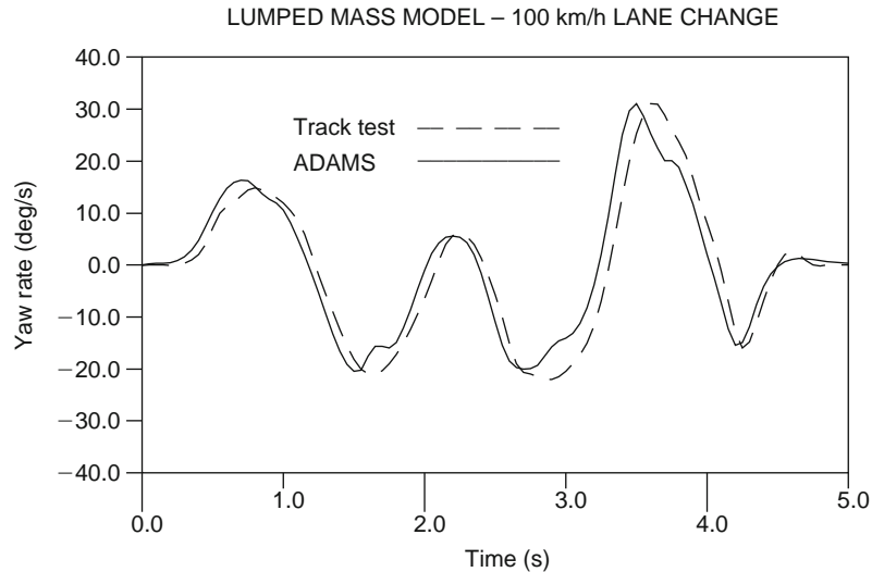
Fig. 15.1-53 Yaw rate comparison – lumped mass model and test. (This material has been reproduced from the Proceedings of the Institution of Mechanical Engineers, K2 Vol. 214 ‘The modelling and simulation of vehicle handling. Part 4: handling simulation’, M.V. Blundell, page 80, by permission of the Council of the Institution of Mechanical Engineers.)
