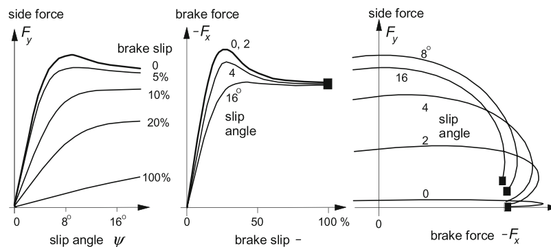
Fig. 11.1-2 Combined side force and brake force characteristics.
