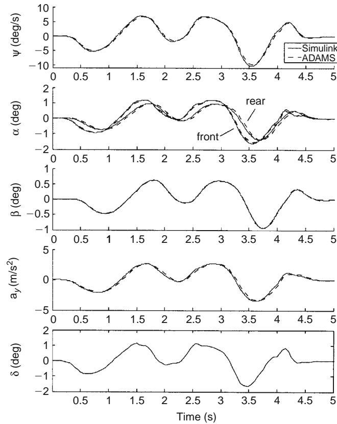
Fig. 15.1-63 Comparison of Simulink and MSC.ADAMS predictions of vehicle response.
