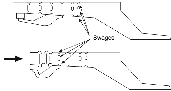
Fig. 17.1-13 Diagrammatic representation of front longitudinal frame member carrying the suspension and engine. The lengths of the swages, in each set of four (in the top, bottom and two sides of the frame), become progressively smaller, from the foremost to the rearmost, so that the frame will offer progressively increasing resistance to collapse in a frontal impact. The lower diagram shows it only partially collapsed.
