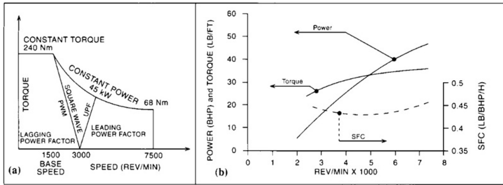
Fig. 7.1-7 System operation states (a), with performance curves of 300 cc fuel-injection Wankel engine (b).
