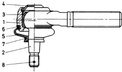
Fig. 9.1-14 Lemförder Fahrwerktechnik pre-lubricated tie rod joint, used on passenger cars and light vans. The joint housing 1 has a fine thread on the shaft (M14 × 1.5 to M22 × 1.5) and is made of annealed steel C35V; surface-hardenable steel 41Cr4V is used for the ball pivot 2.
