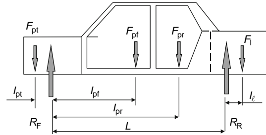
Fig. 16.2-3 Payload distribution.
