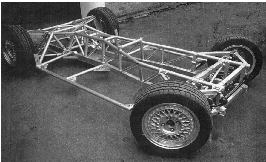
Fig. 16.1-15 Backbone chassis made of triangulated tubes (from author's collection, courtesy TVR Ltd).
