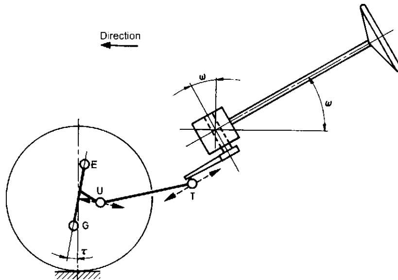
Fig. 9.1-33 The central points of the tie rod joints (T on the inside and U on the outside) change their position relative to one another, based on the wheel travel (vertical and horizontal) on independent wheel suspensions. The reasons for this are the different directions of movement of pitman arm and steering arm. The former depends on the inclined position of the steering gear (angle \omega ) and that of the point U from the inclination of the steering axis EG, i.e. the kingpin inclination \sigma and the caster angle \tau .
