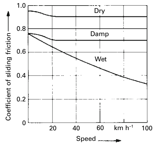
Fig. 10.1-34 Dependency of the coefficient of sliding friction \mu_{X,W,lo} on speed on different road conditions.
