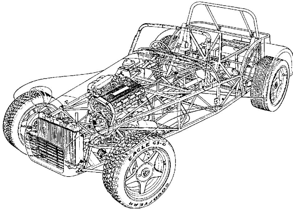
Fig. 16.1-16 Triangulated sports car structure (courtesy of Caterham Cars Ltd).
