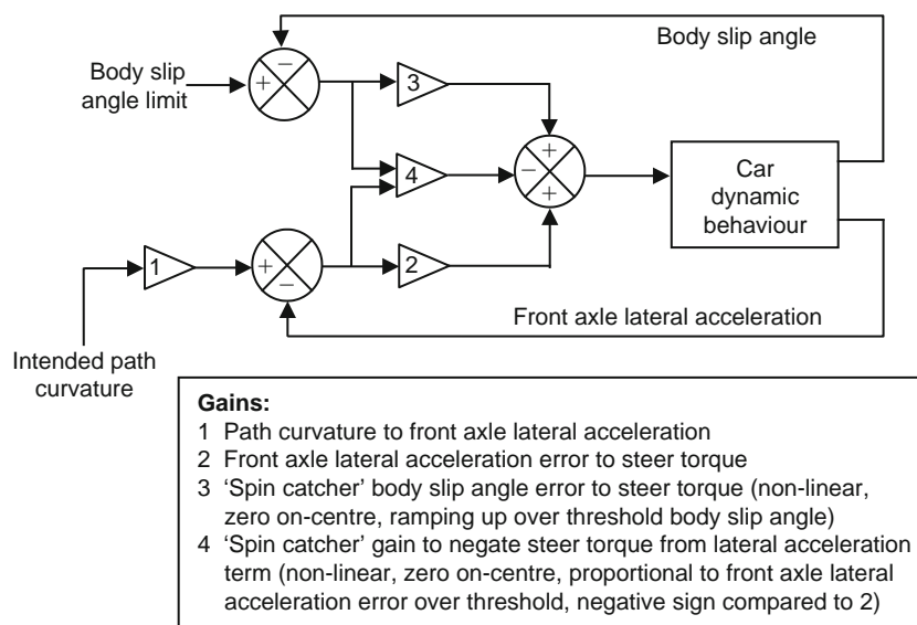
Fig. 15.1-48 A typical two-loop driver model.
