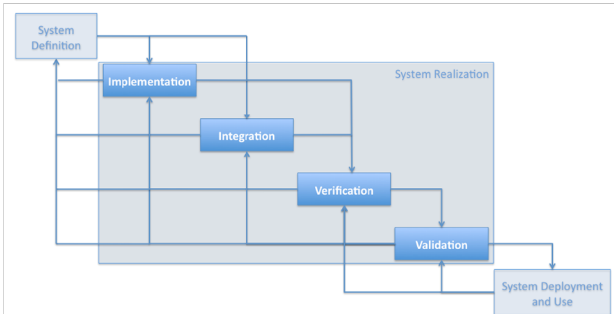
Figure 3. System Realization. (SEBoK Original)
