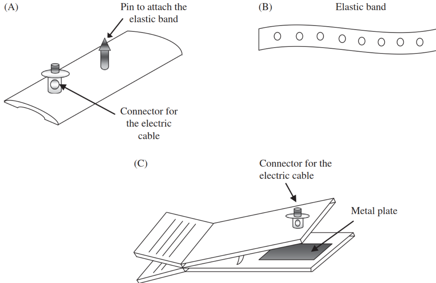
Figure 2.17 Limb electrodes: (A) curved plate, (B) fixation elastic bands and (C) plate electrode mounted in clip support.
