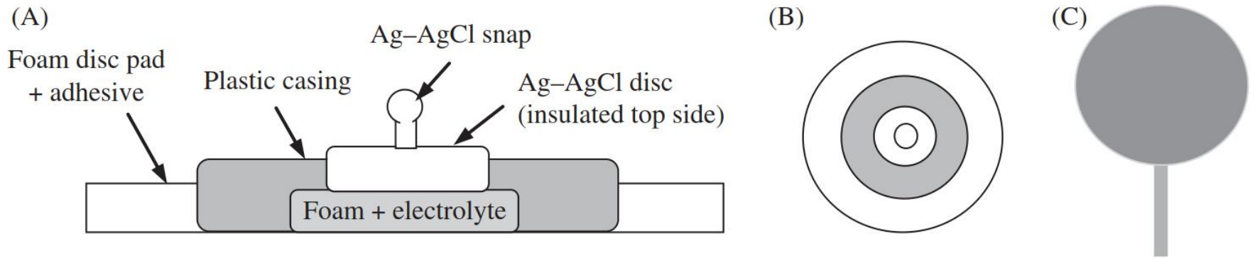
Figure 2.24 Schematic diagram of a disposable electrode with lead wire connector: (A) side section, (B) top view, and (C) electrode with soldered lead wire.
